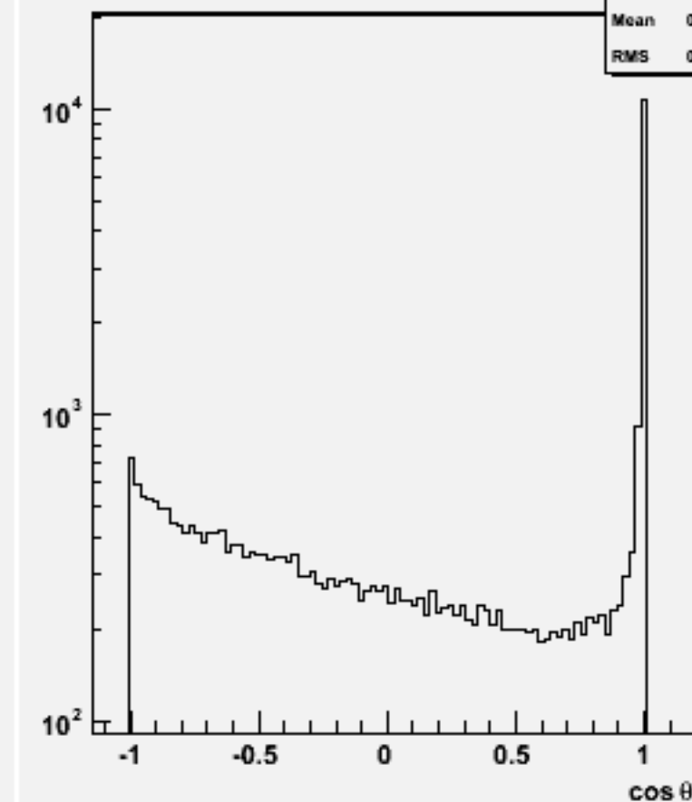
Jet cos \theta (All jets)w101478 n2n2cse1n1_o
