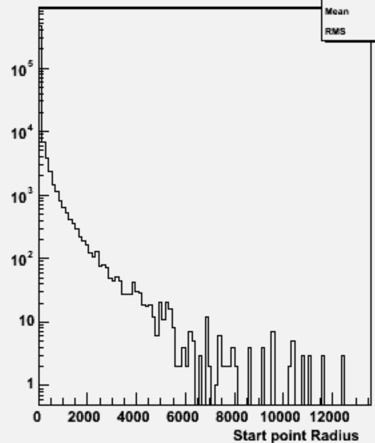
Start point R : w101478 n2n2cse1n1_o
