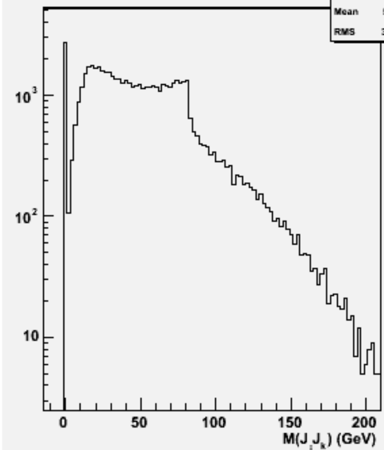
2jets mass(All comb)w101478 n2n2cse1n1_o
