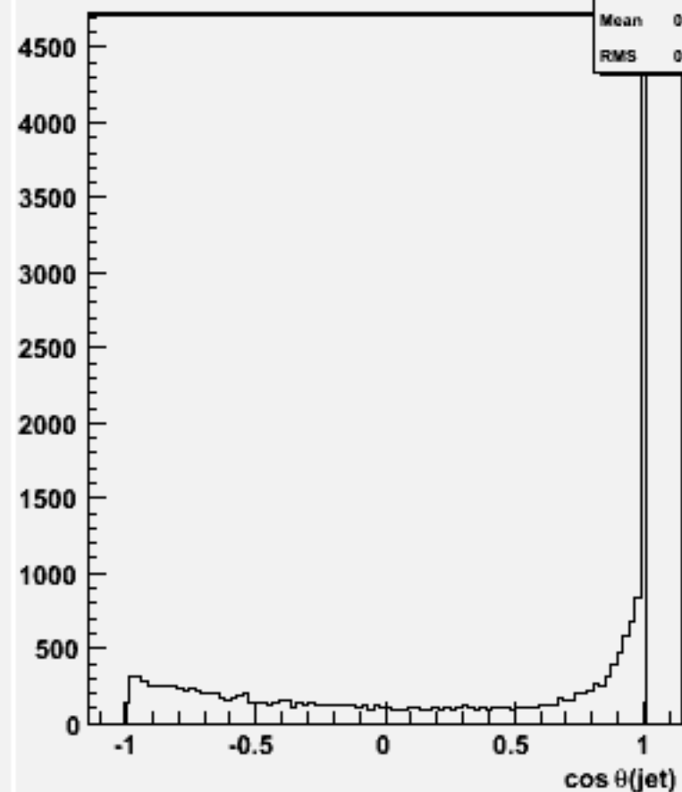
cos \theta for 2-jets :w101478 n2n2cse1n1_o
