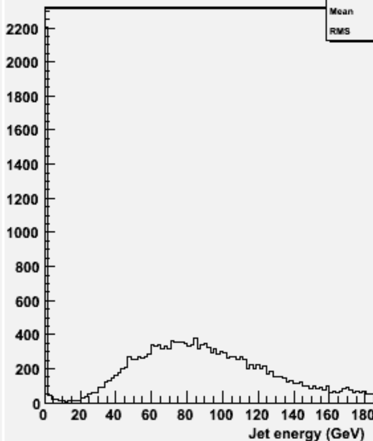
energy for 2-jets :w101478 n2n2cse1n1_o
