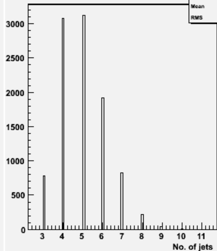
No. jets (ycut=0.001) : w101478 n2n2cse1n1_o
