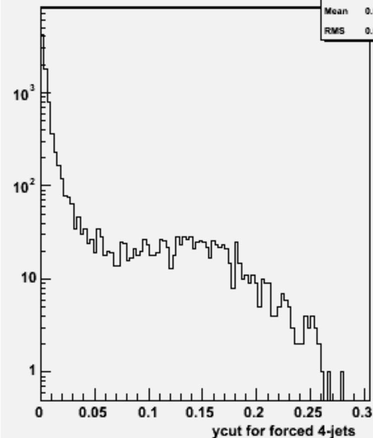
Ycut for 4-jets :w101478 n2n2cse1n1_o
