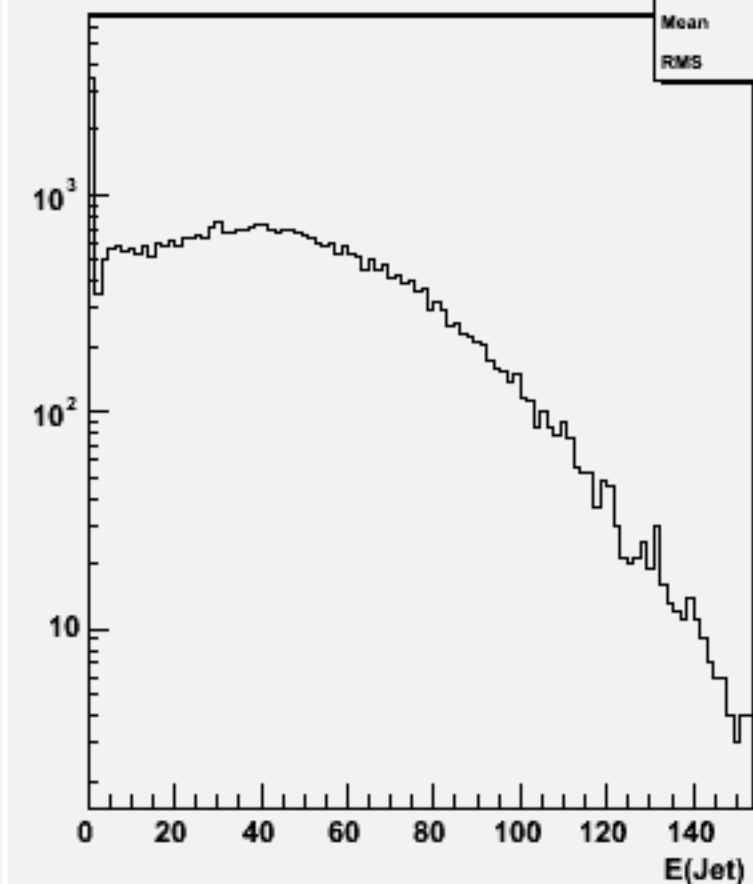
Jet energies(All jets)w101478 n2n2cse1n1_o
