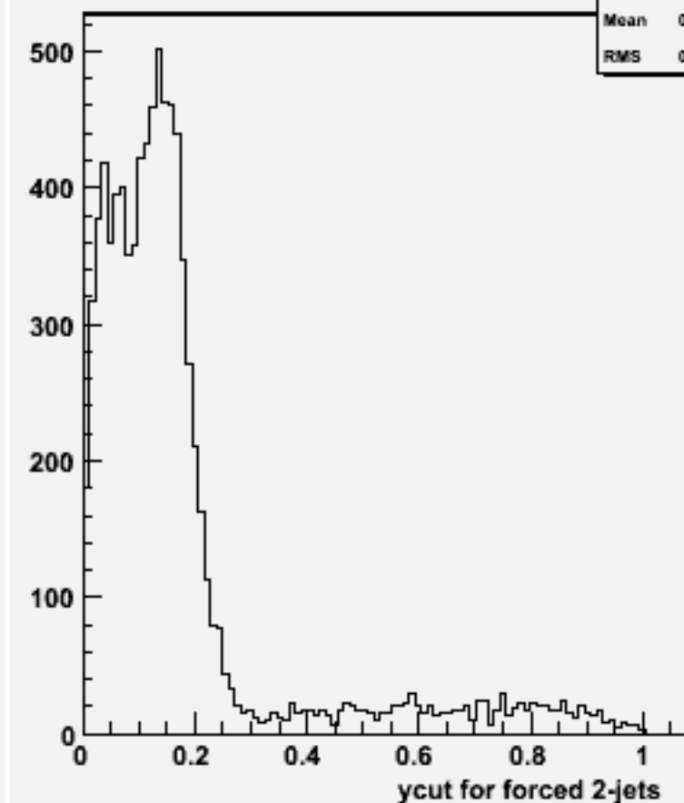
Ycut for 2-jets :w101478 n2n2cse1n1_o
