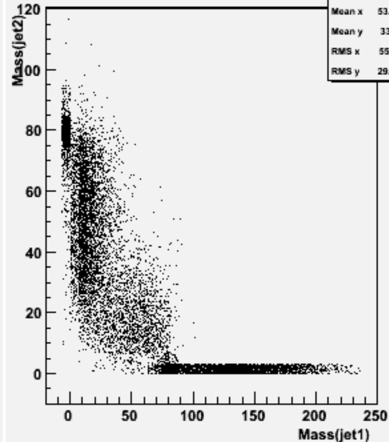
Jet mass for forced 2-jets : w101478 n2n2cse1n1_o
