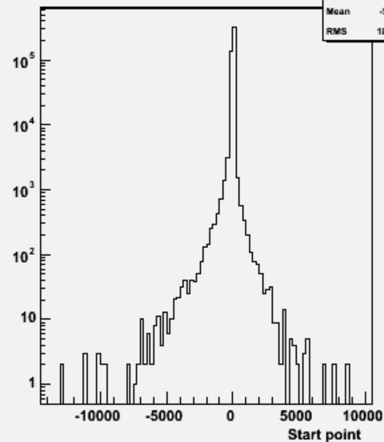
Start point Z : w101478 n2n2cse1n1_o
