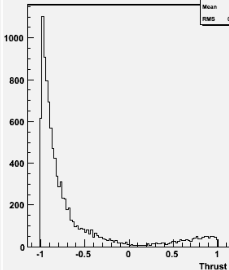
cos \Theta (thrust) w101478 n2n2cse1n1_o
