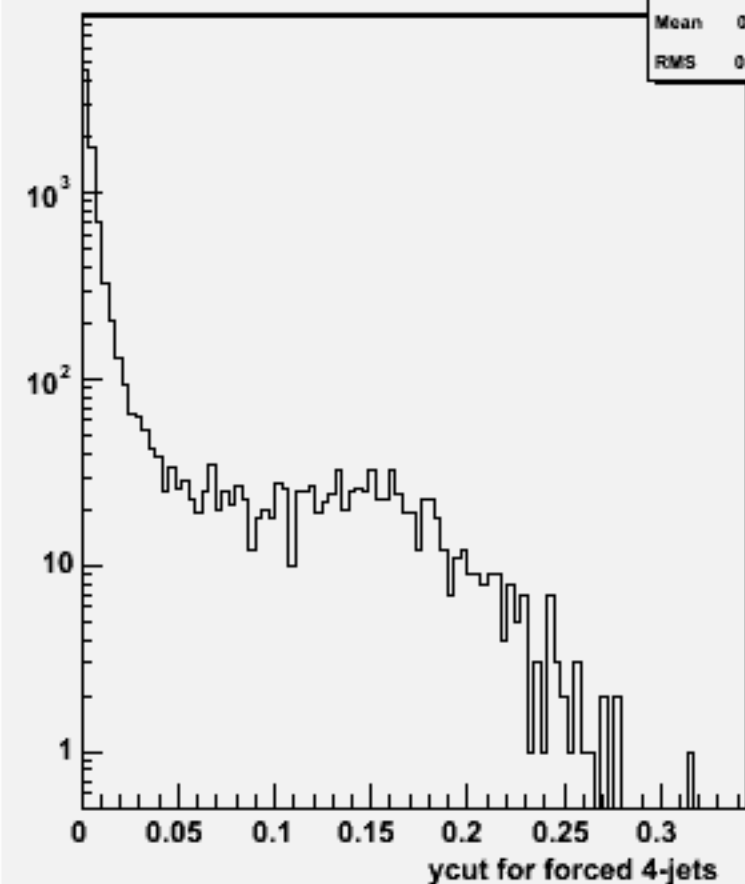
Ycut for 4-jets :w101476 n2n2cse1n1_o
