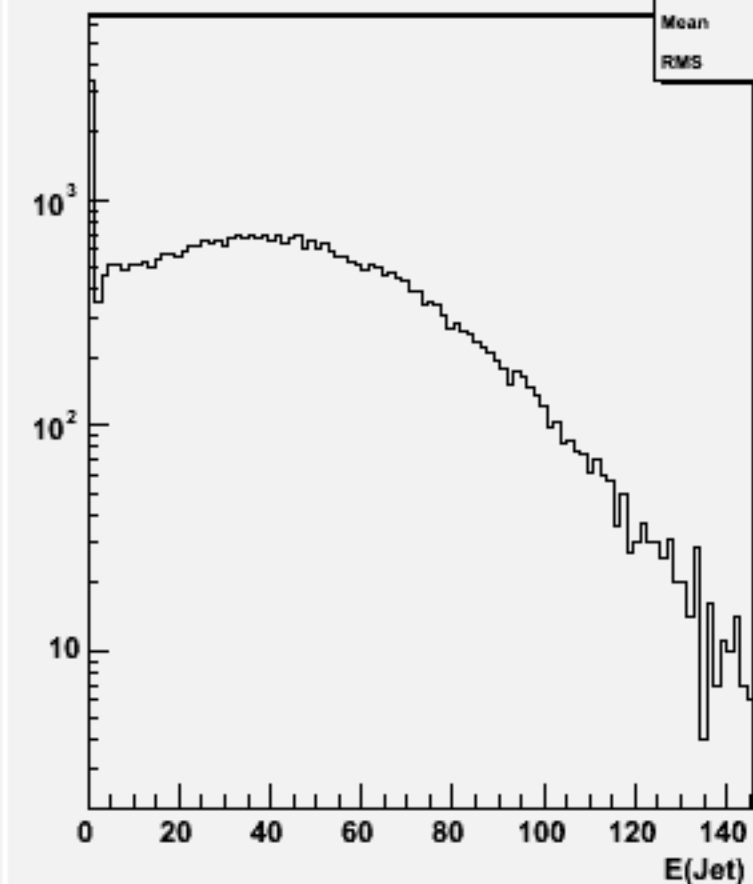
Jet energies(All jets)w101476 n2n2cse1n1_o
