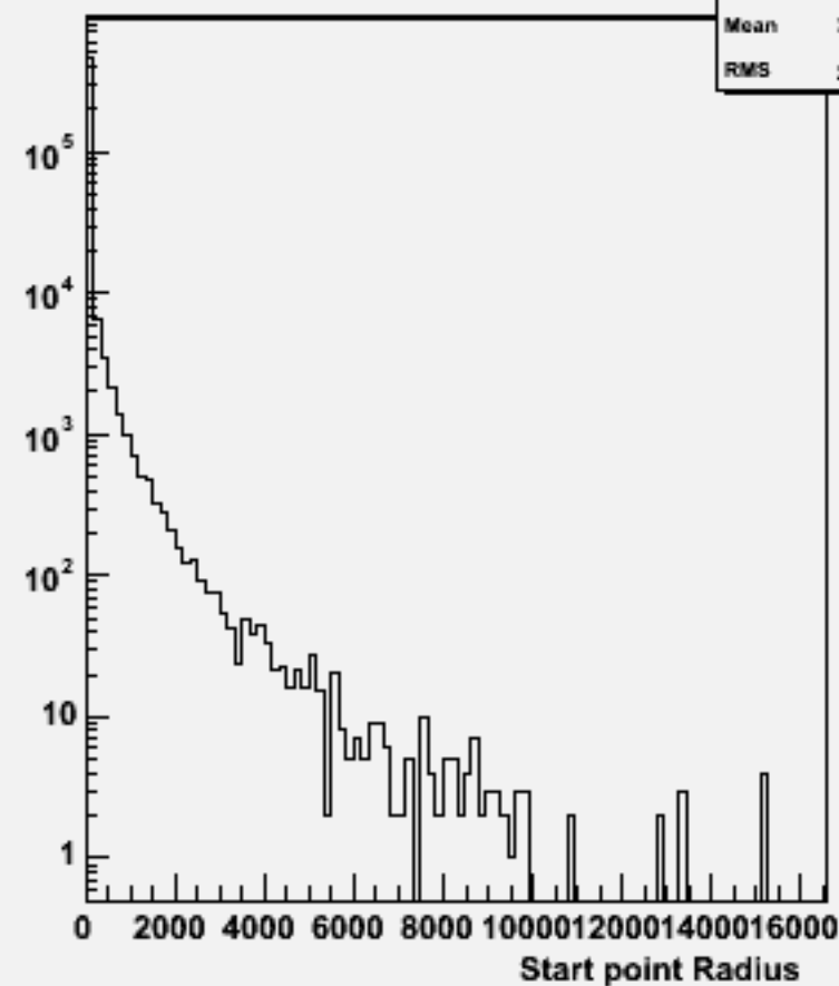
Start point R : w101476 n2n2cse1n1_o
