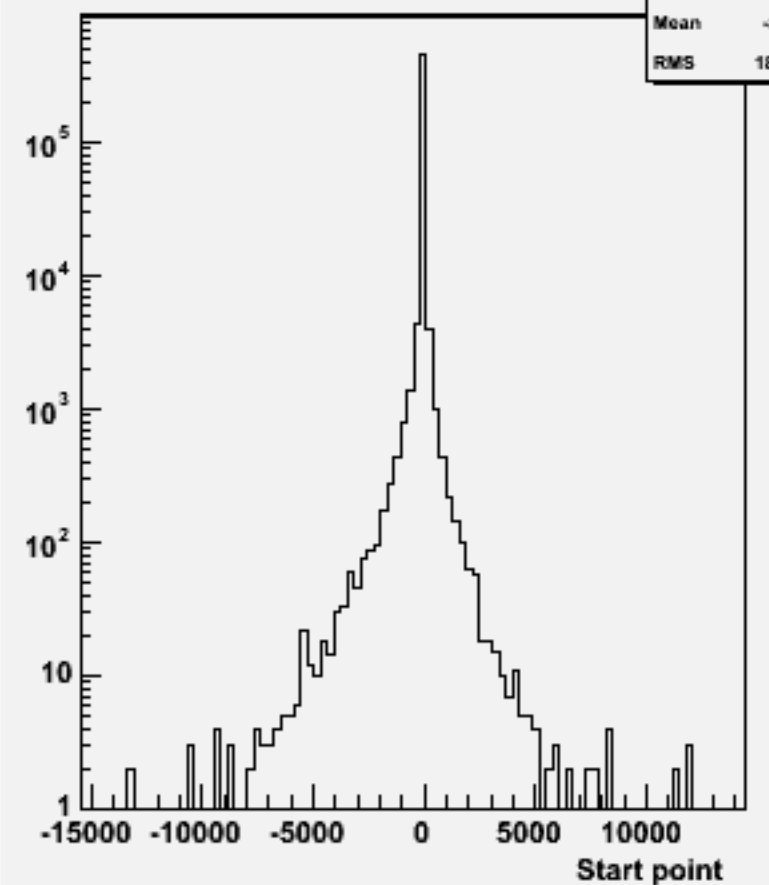
Start point Z : w101476 n2n2cse1n1_o
