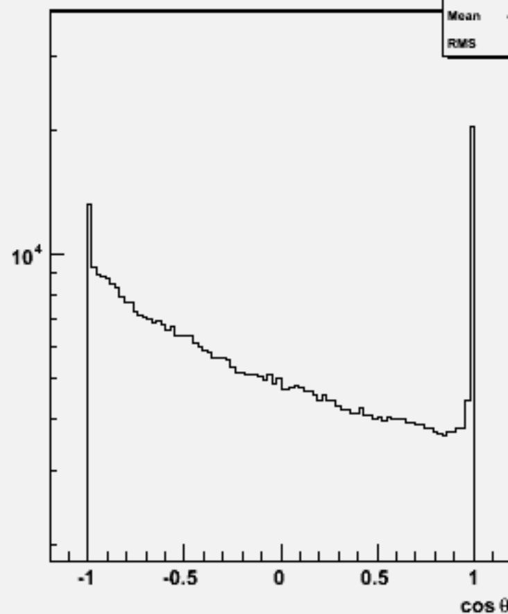
Particle cosθ : w101476 n2n2cse1n1_o
