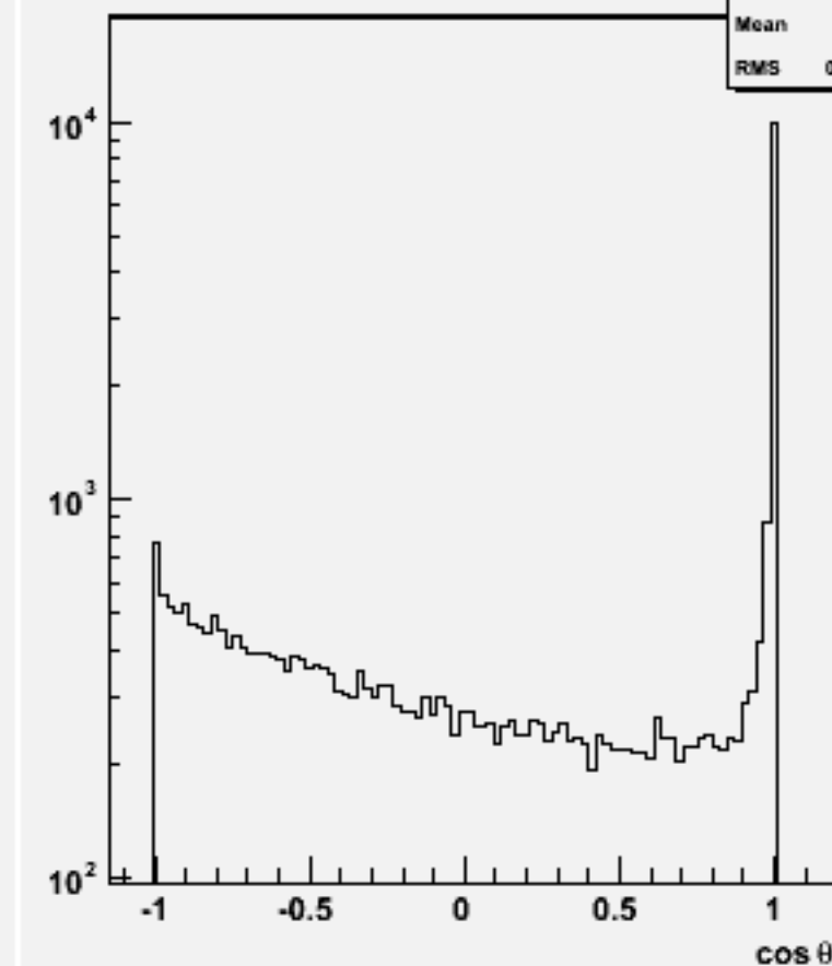
Jet cos \theta (All jets)w101476 n2n2cse1n1_o
