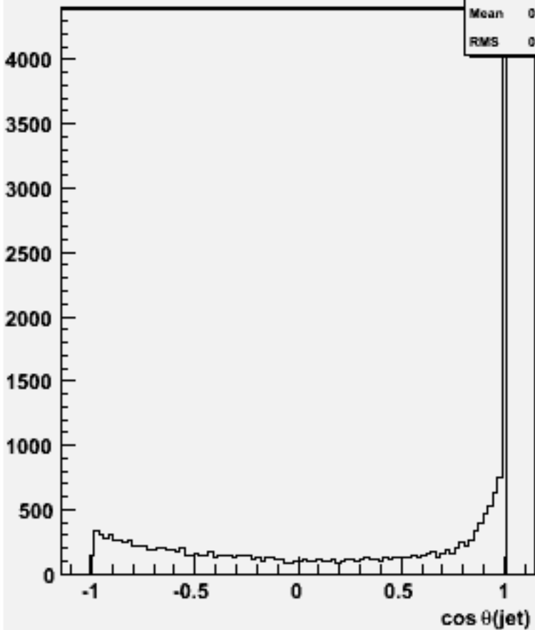
cos \theta for 2-jets :w101476 n2n2cse1n1_o
