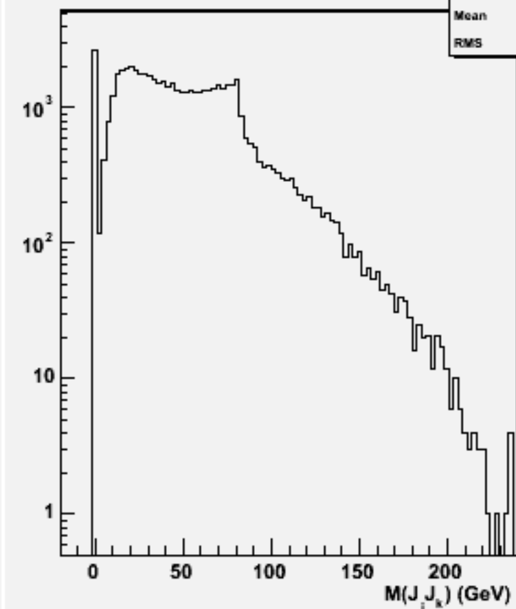
2jets mass(All comb)w101476 n2n2cse1n1_o
