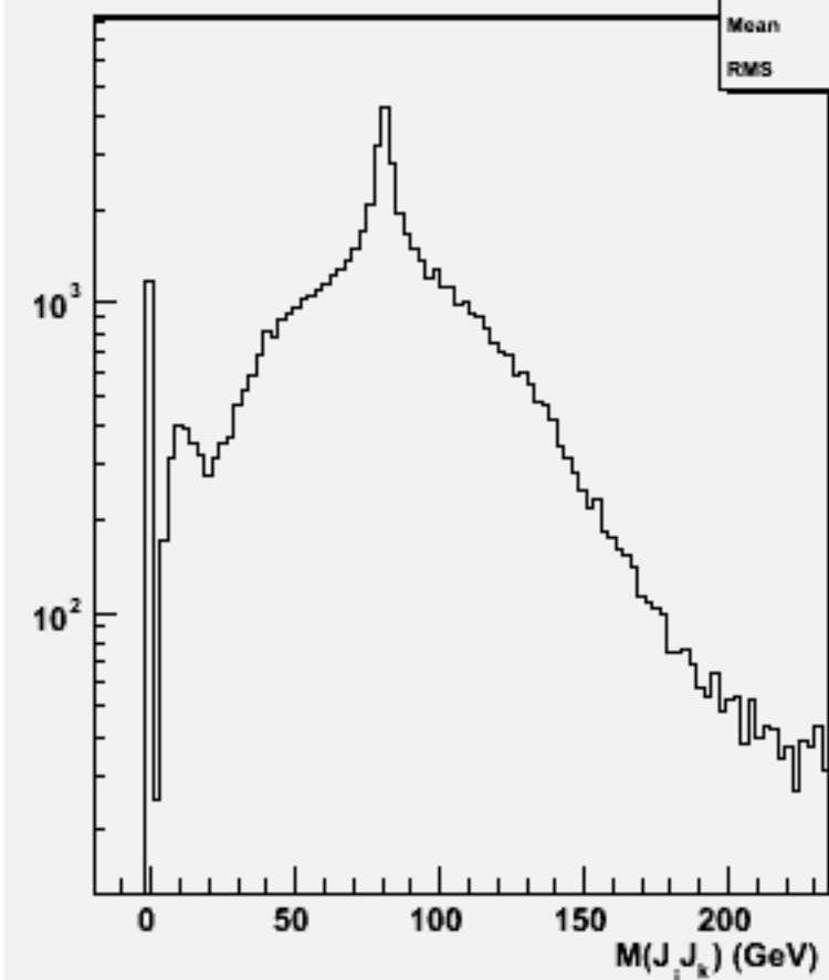
2jets mass(All comb)w101473 n2n2udsc_o
