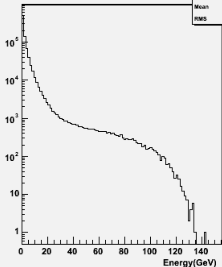
Particle Energy : w101473 n2n2udsc_o
