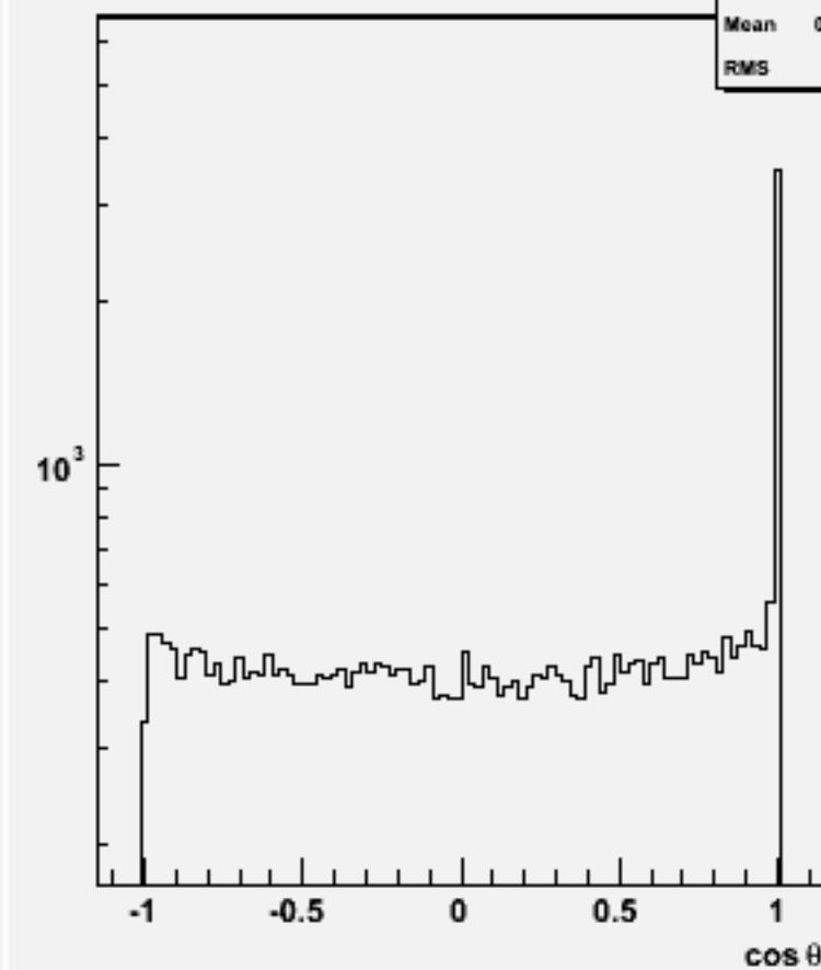
Jet cos \theta (All jets)w101473 n2n2udsc_o
