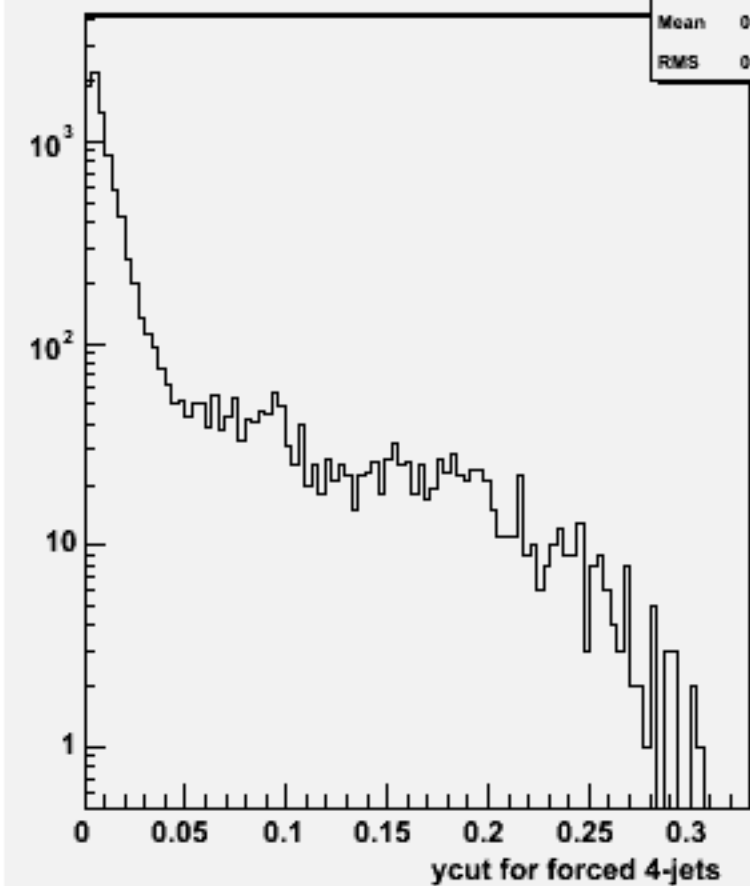
Ycut for 4-jets :w101473 n2n2udsc_o
