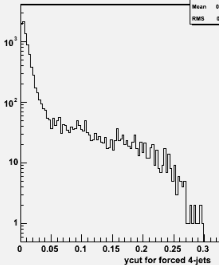
Ycut for 4-jets :w101472 n2n2udsc_o
