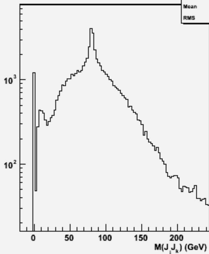
2jets mass(All comb)w101472 n2n2udsc_o
