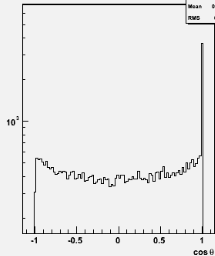
Jet cos \theta (All jets)w101472 n2n2udsc_o
