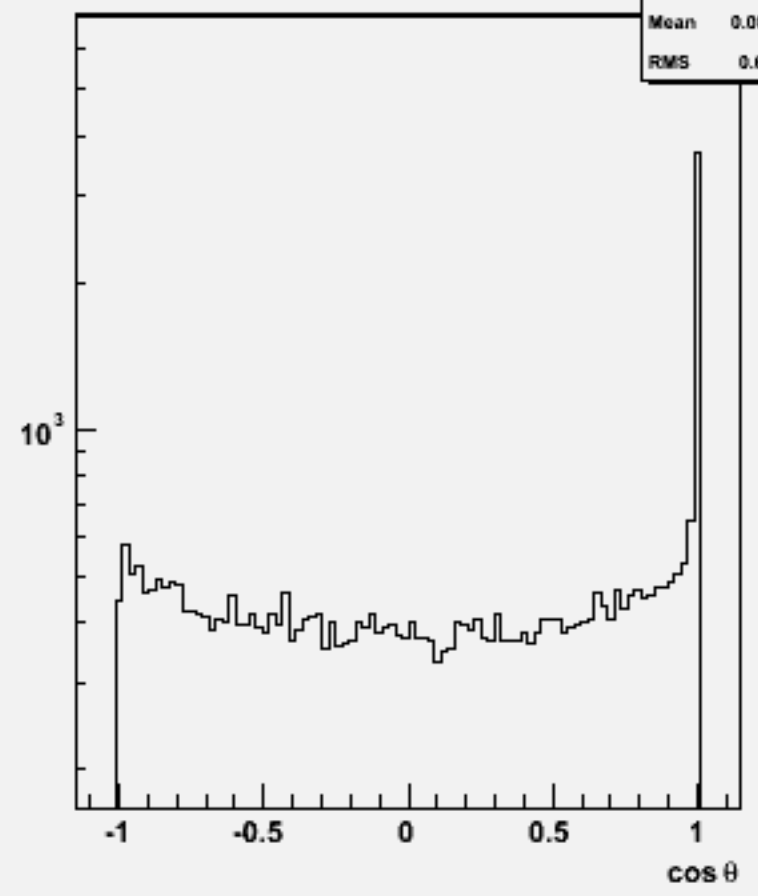
Jet cosθ (All jets)w101469 n2n2uddu_o
