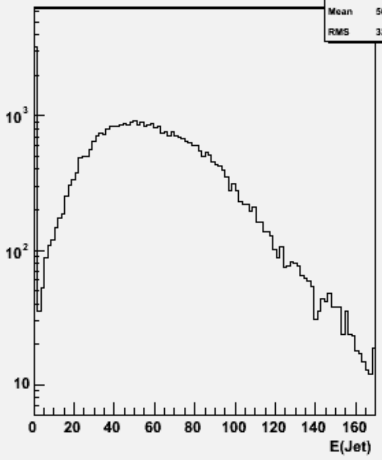
Jet energies(All jets)w101469 n2n2uddu_o
