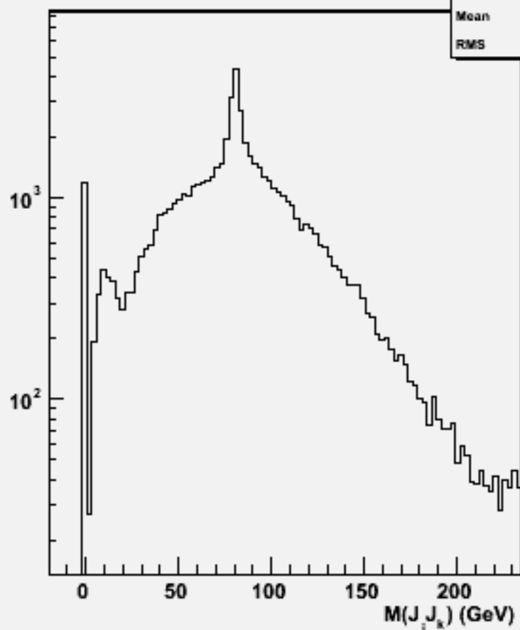
2jets mass(All comb)w101468 n2n2uddu_o
