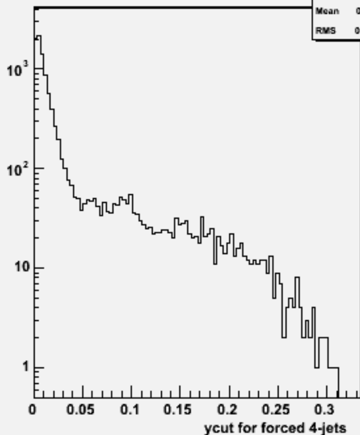
Ycut for 4-jets :w101468 n2n2uddu_o
