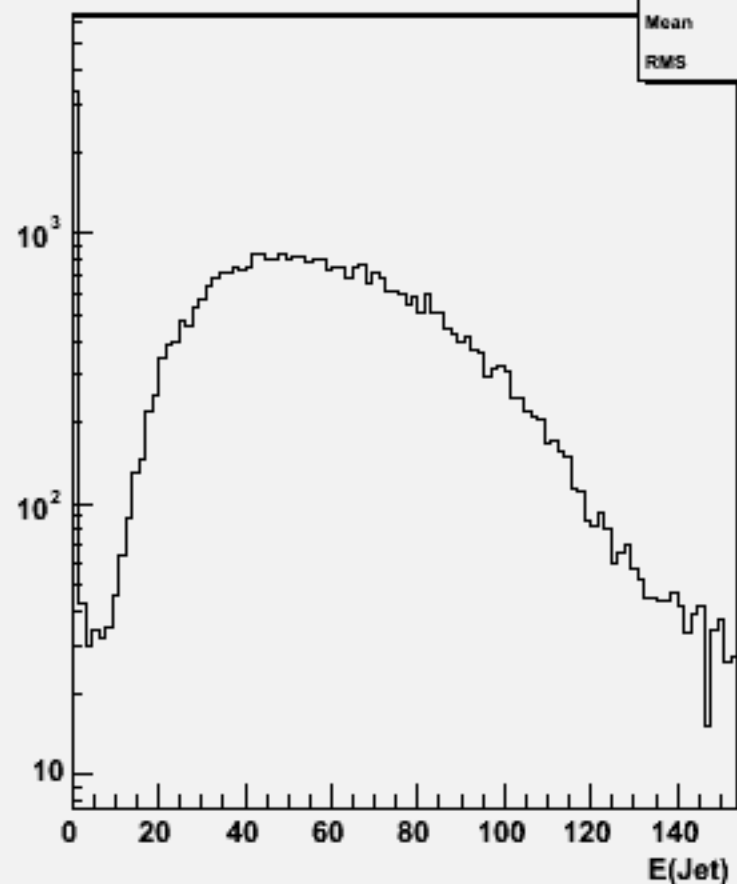
Jet energies(All jets)w101468 n2n2uddu_o
