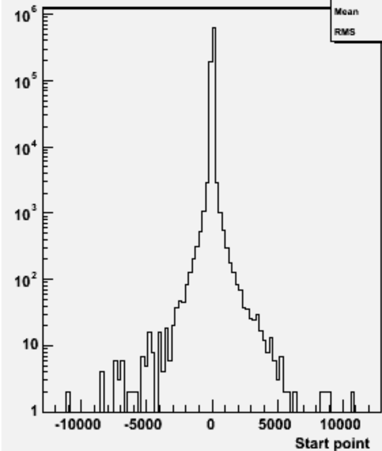
Start point Z : w101468 n2n2uddu_o
