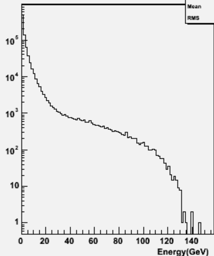
Particle Energy : w101468 n2n2uddu_o
