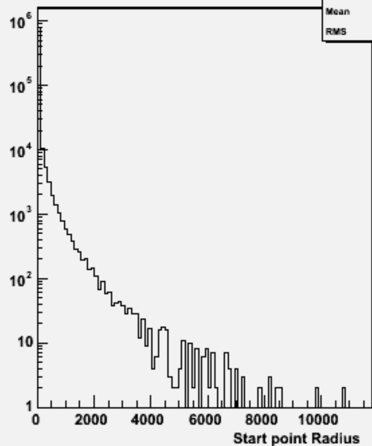
Start point R : w101468 n2n2uddu_o
