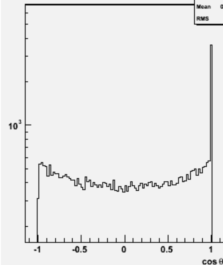
Jet cos \theta (All jets)w101468 n2n2uddu_o
