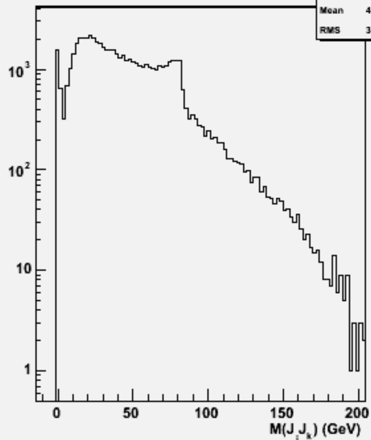
2jets mass(All comb)w101464 n2n2ude3n3_o
