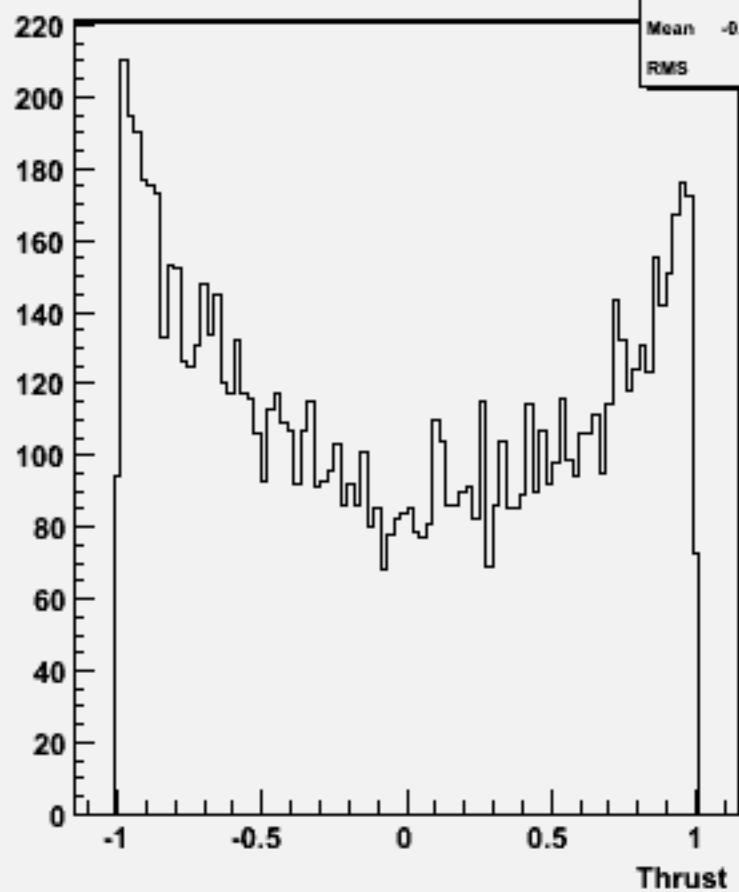
cos \Theta (thrust) w101464 n2n2ude3n3_o
