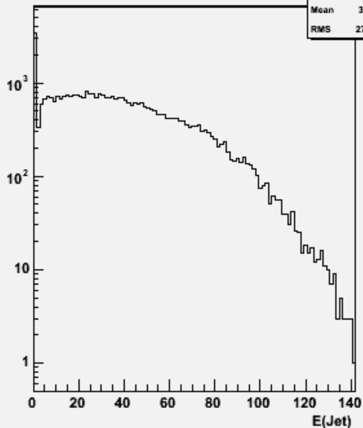
Jet energies(All jets)w101464 n2n2ude3n3_o
