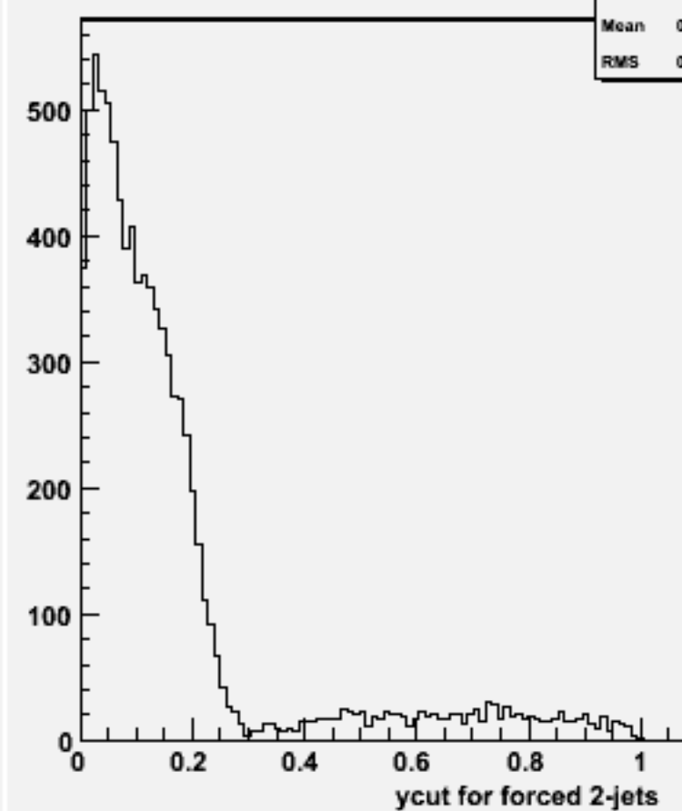
Ycut for 2-jets :w101464 n2n2ude3n3_o
