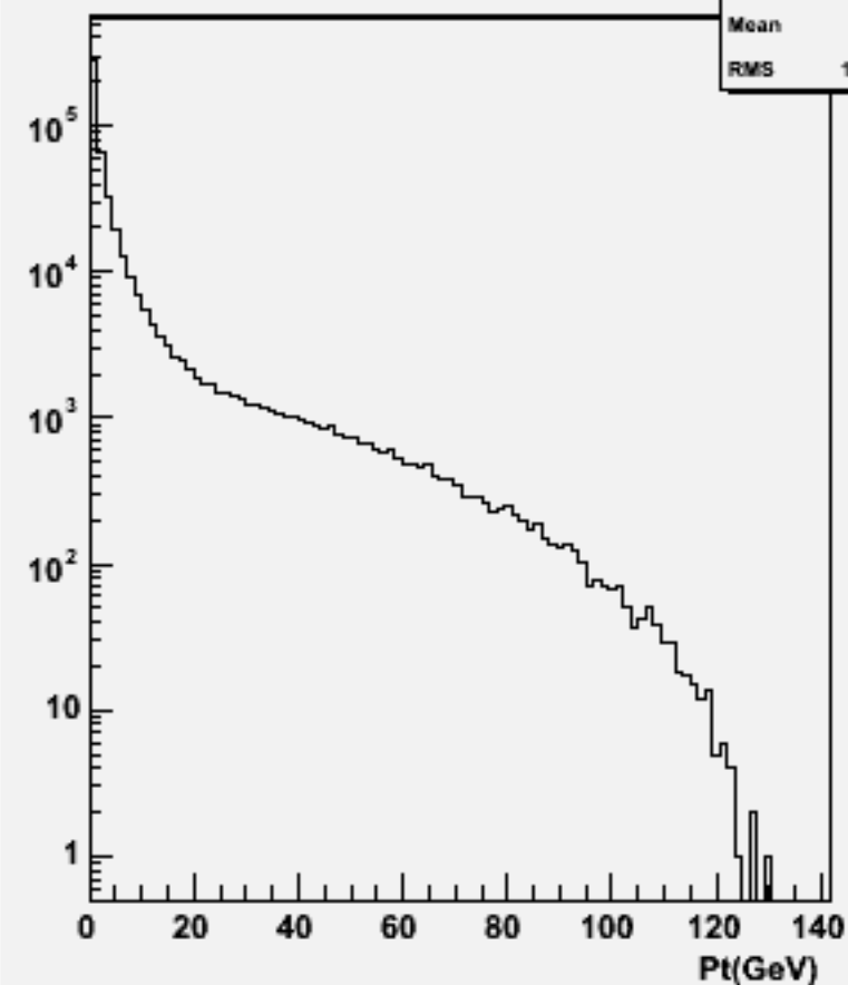
Start point Z : w101464 n2n2ude3n3_o
