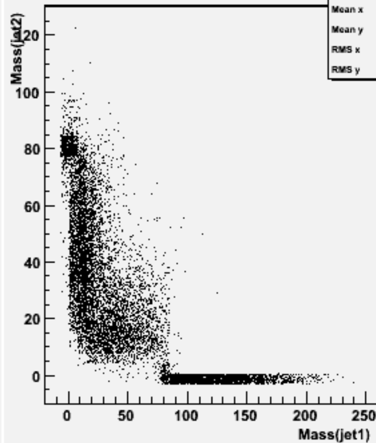
Jet mass for forced 2-jets : w101464 n2n2ude3n3_o
