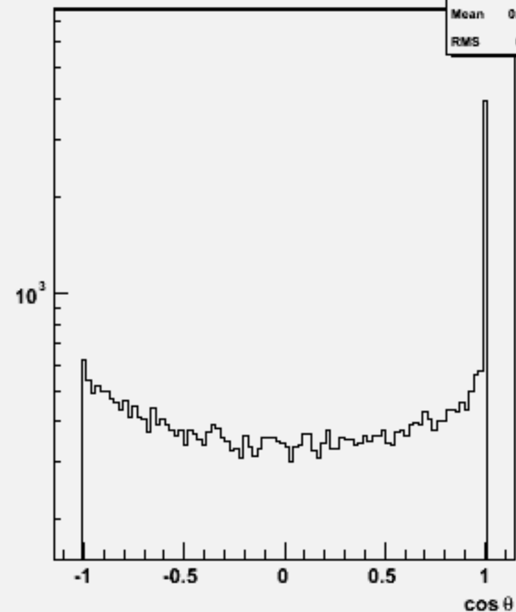
Jet cos \theta (All jets)w101464 n2n2ude3n3_o
