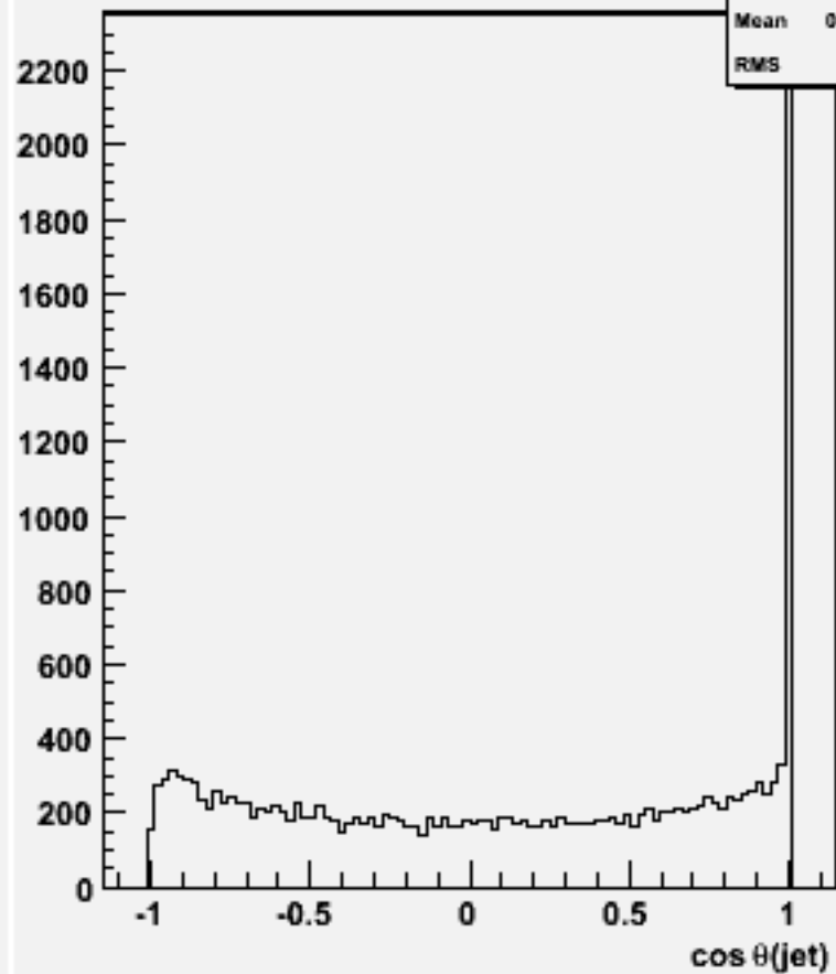
cos \theta for 2-jets :w101464 n2n2ude3n3_o
