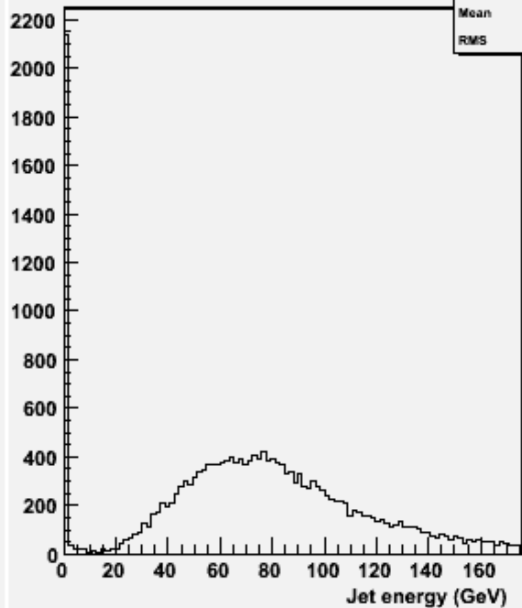
energy for 2-jets :w101464 n2n2ude3n3_o
