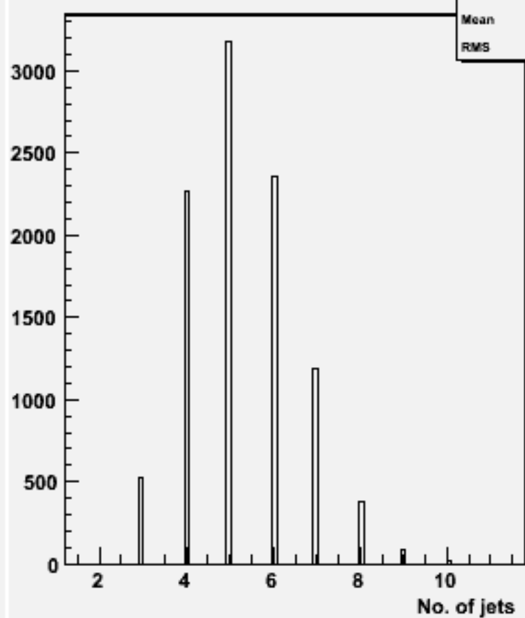
No. jets (ycut=0.001) : w101464 n2n2ude3n3_o
