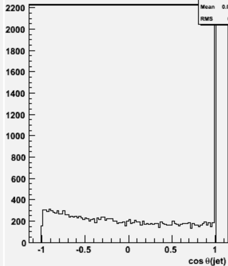
cos \Theta for 2-jets :w101461 n2n2ude2n2_o
