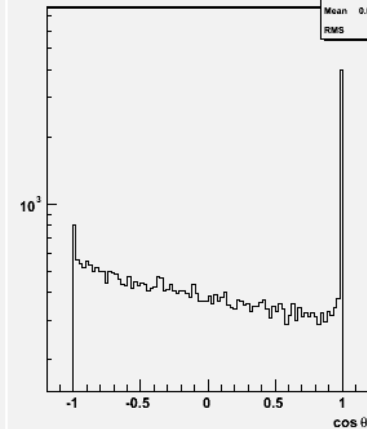
Jet cos \theta (All jets)w101461 n2n2ude2n2_o
