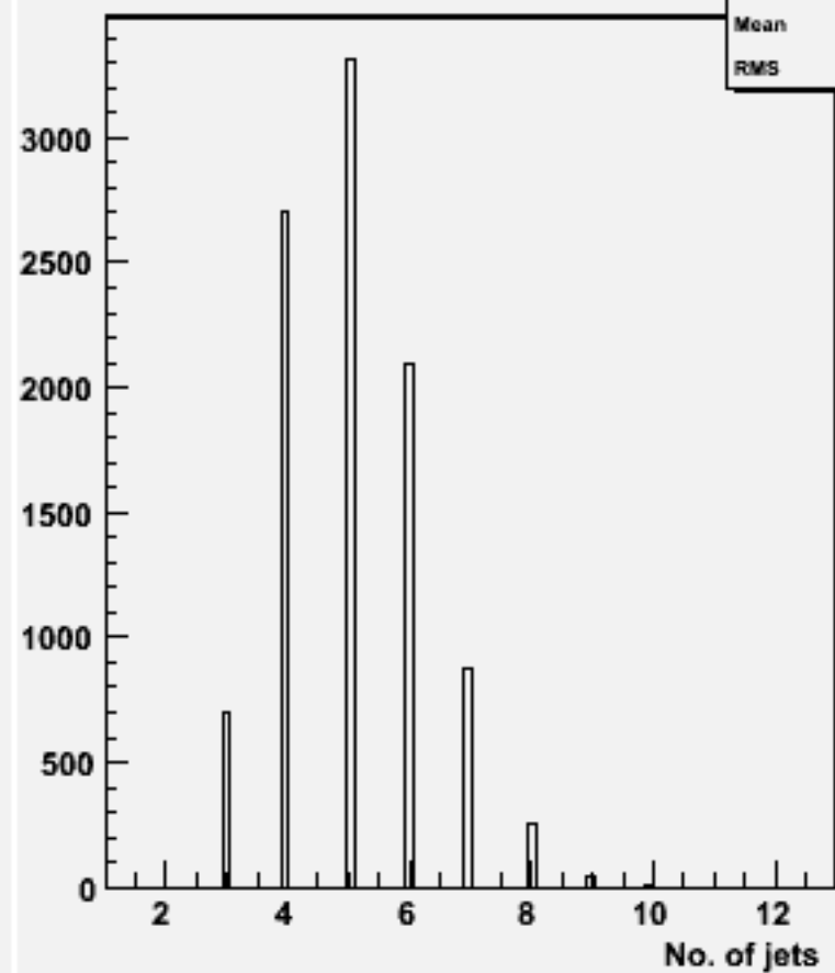
No. jets (ycut=0.001) : w101461 n2n2ude2n2_o
