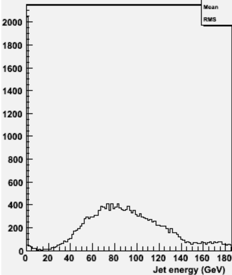
energy for 2-jets :w101461 n2n2ude2n2_o
