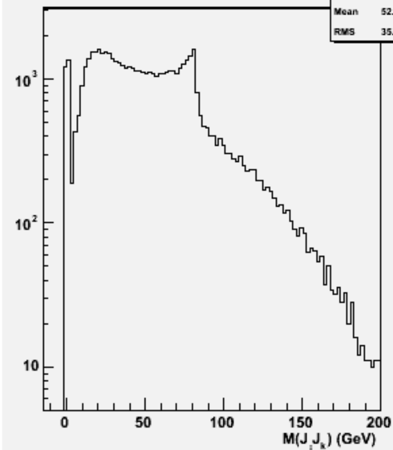
2jets mass(All comb)w101461 n2n2ude2n2_o
