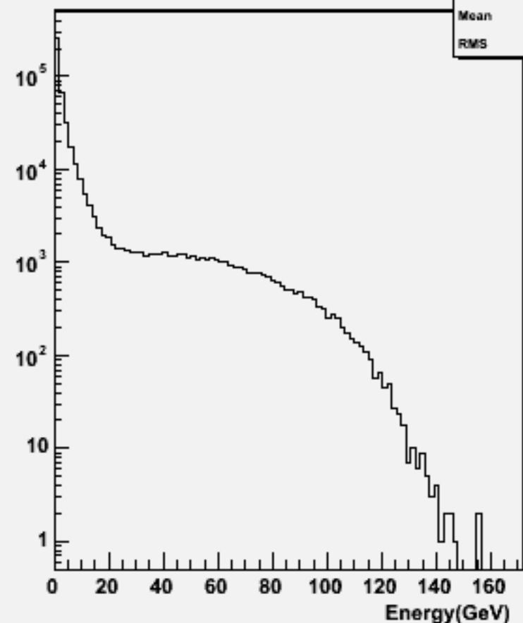
Start point R : w101461 n2n2ude2n2_o
