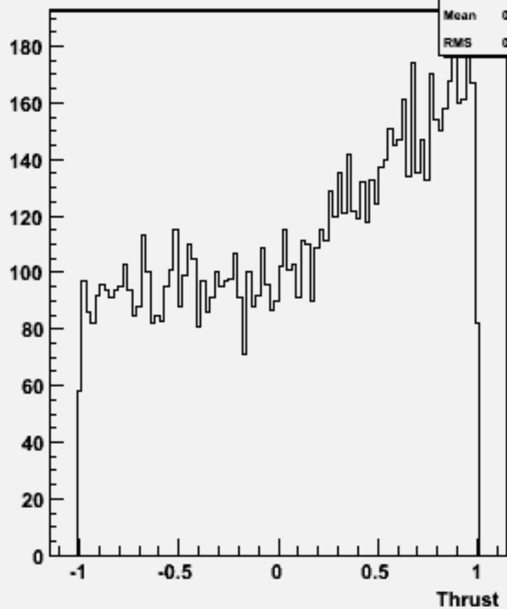
cos \Theta (thrust) w101461 n2n2ude2n2_o
