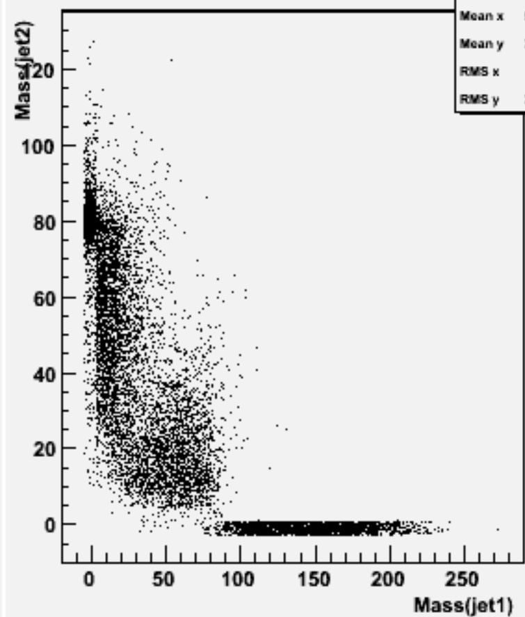
Jet mass for forced 2-jets : w101461 n2n2ude2n2_o
