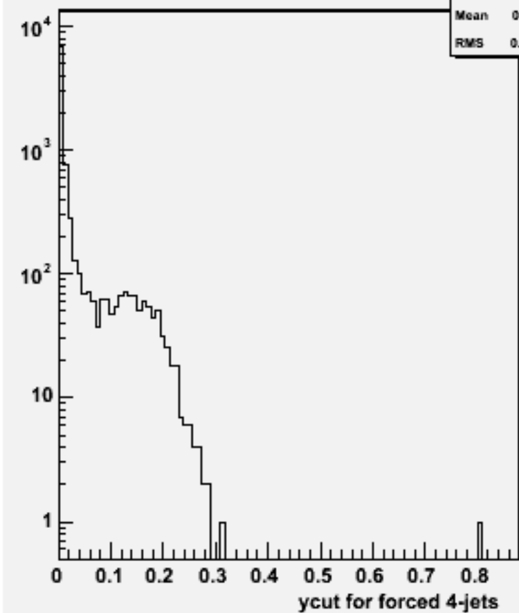
Ycut for 4-jets :w101461 n2n2ude2n2_o
