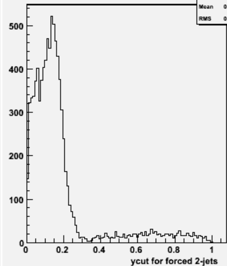
Ycut for 2-jets :w101461 n2n2ude2n2_o
