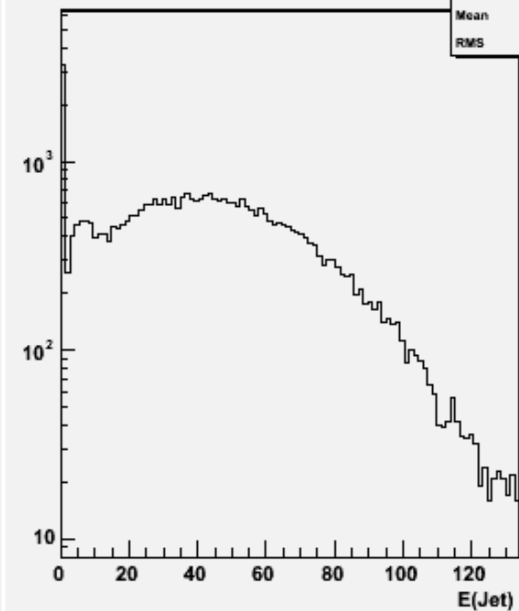
Jet energies(All jets)w101461 n2n2ude2n2_o
