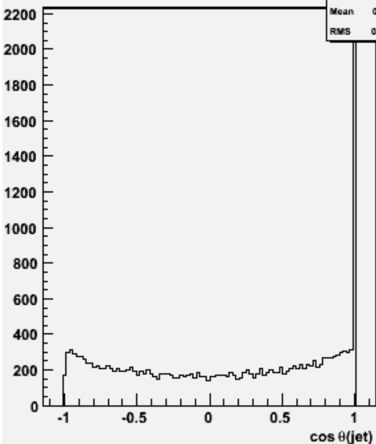
cos \Theta for 2-jets :w101460 n2n2ude2n2_o
