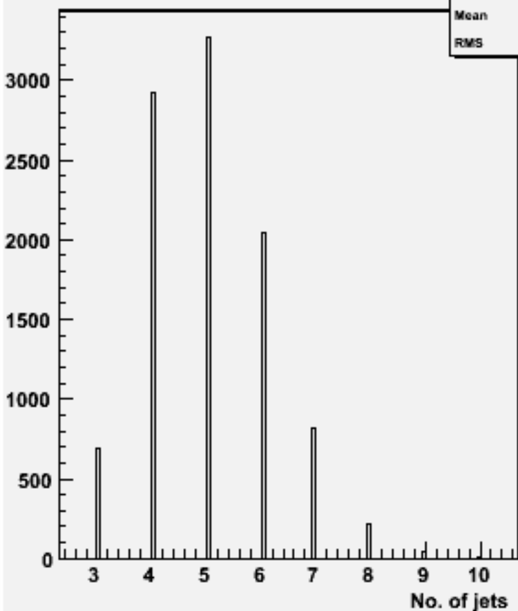
No. jets (ycut=0.001) : w101460 n2n2ude2n2_o
