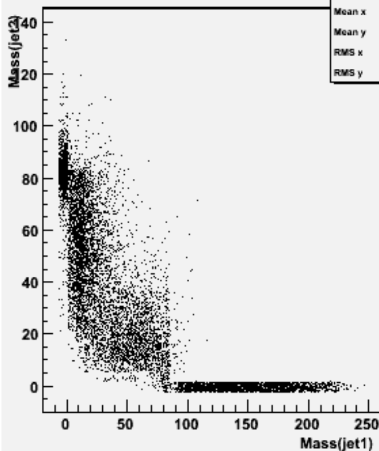
Jet mass for forced 2-jets : w101460 n2n2ude2n2_o
