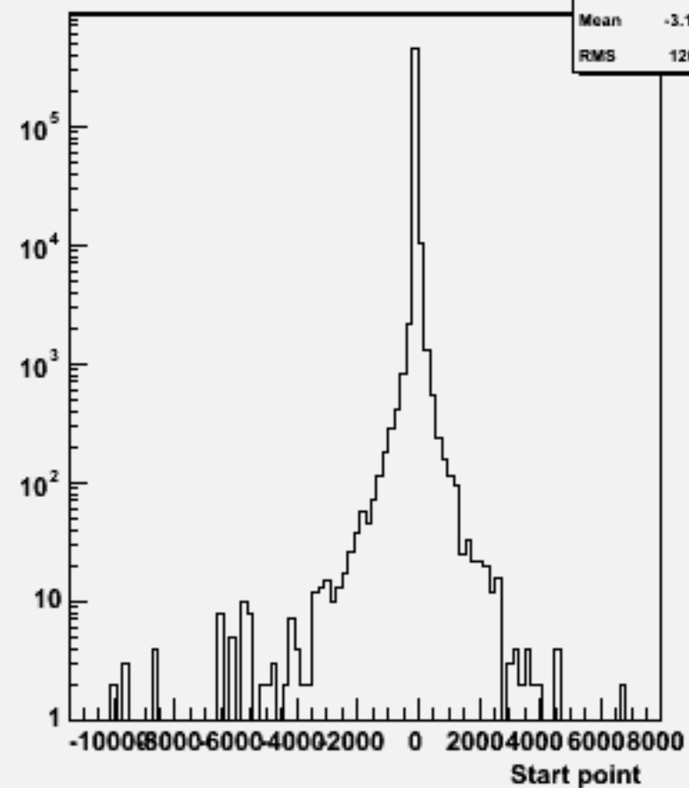
Start point Z : w101460 n2n2ude2n2_o
