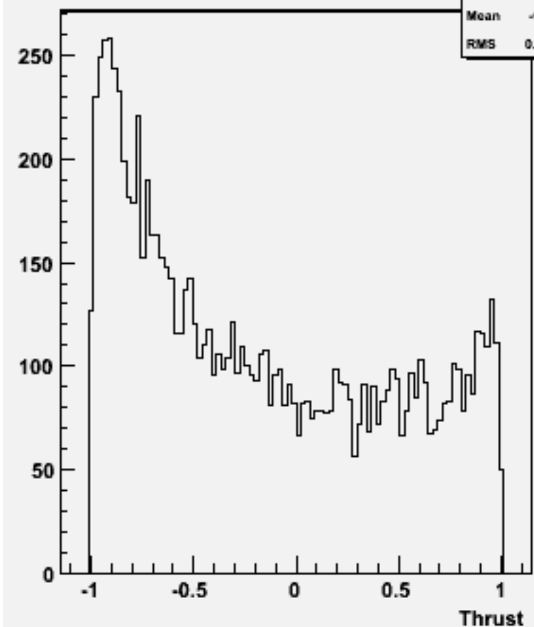
cos \Theta (thrust) w101460 n2n2ude2n2_o
