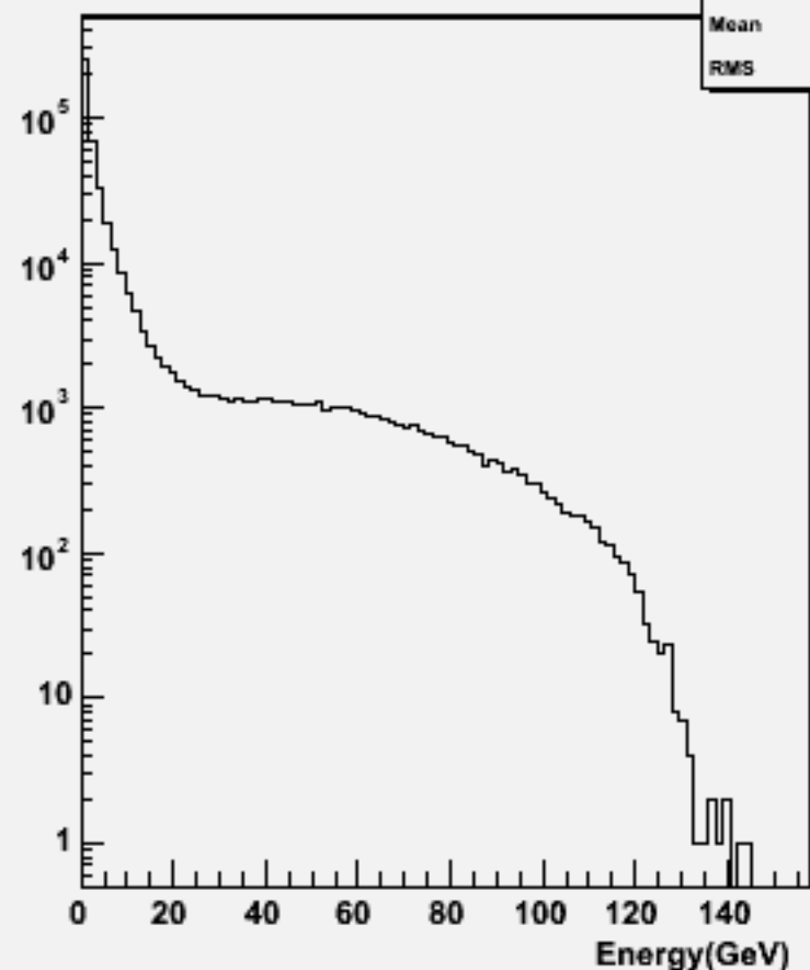
Start point R : w101460 n2n2ude2n2_o
