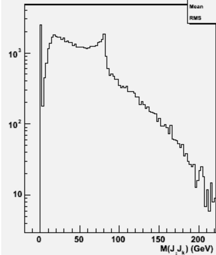
2jets mass(All comb)w101460 n2n2ude2n2_o
