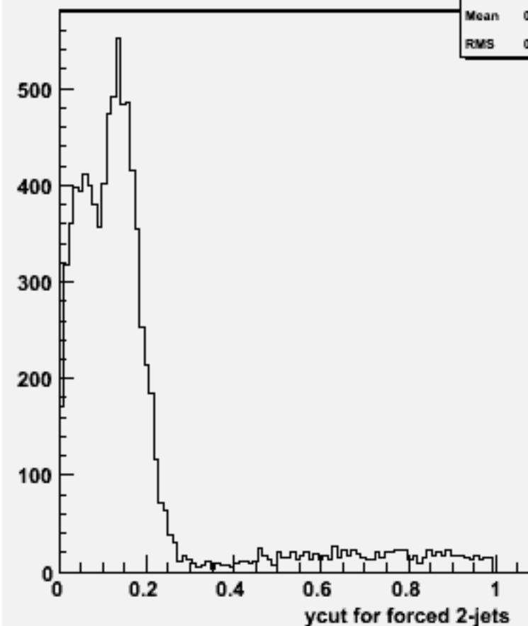
Ycut for 2-jets :w101460 n2n2ude2n2_o
