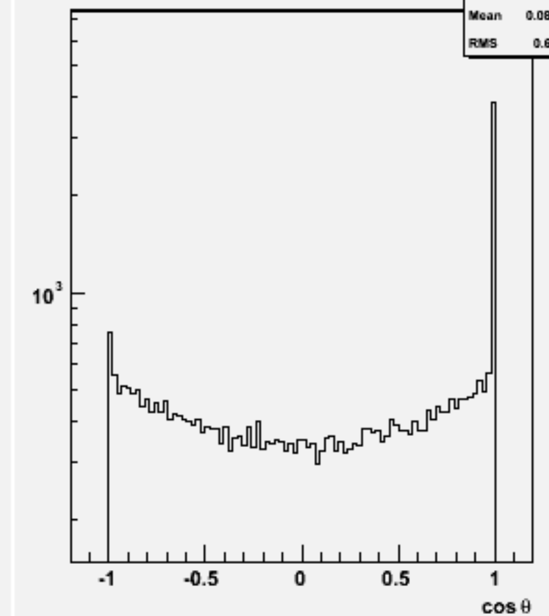
Jet cos \theta (All jets)w101460 n2n2ude2n2_o
