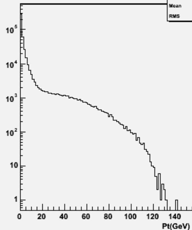
Start point Z : w101460 n2n2ude2n2_o
