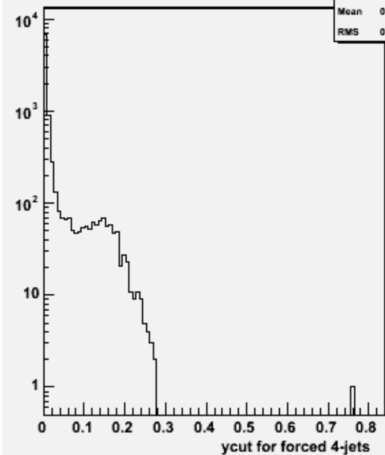
Ycut for 4-jets :w101460 n2n2ude2n2_o
