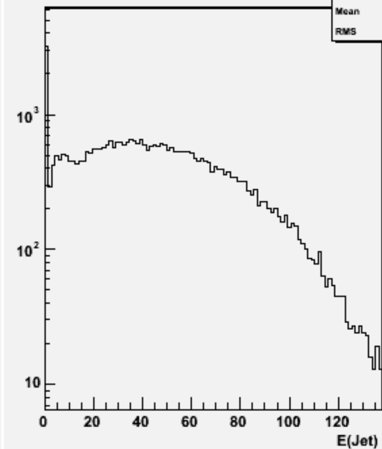
Jet energies(All jets)w101460 n2n2ude2n2_o
