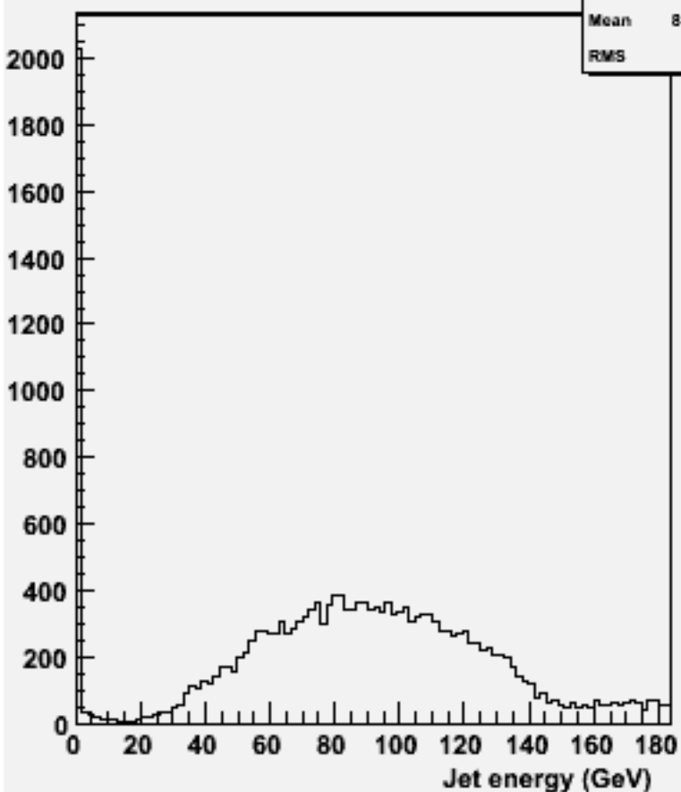
energy for 2-jets :w101460 n2n2ude2n2_o
