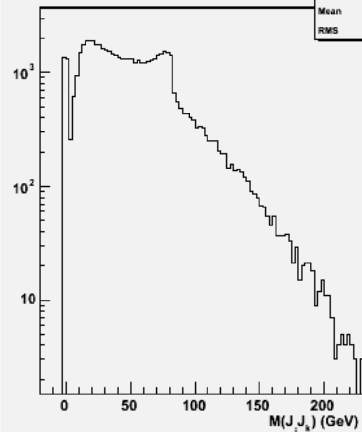
2jets mass(All comb)w101458 n2n2ude1n1_o
