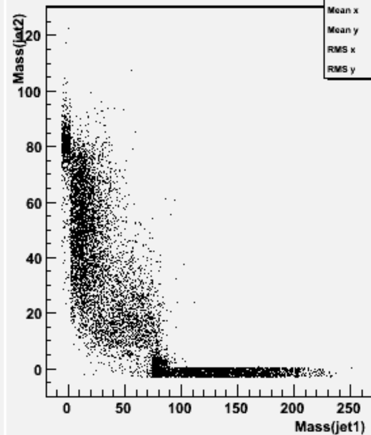
Jet mass for forced 2-jets : w101458 n2n2ude1n1_o
