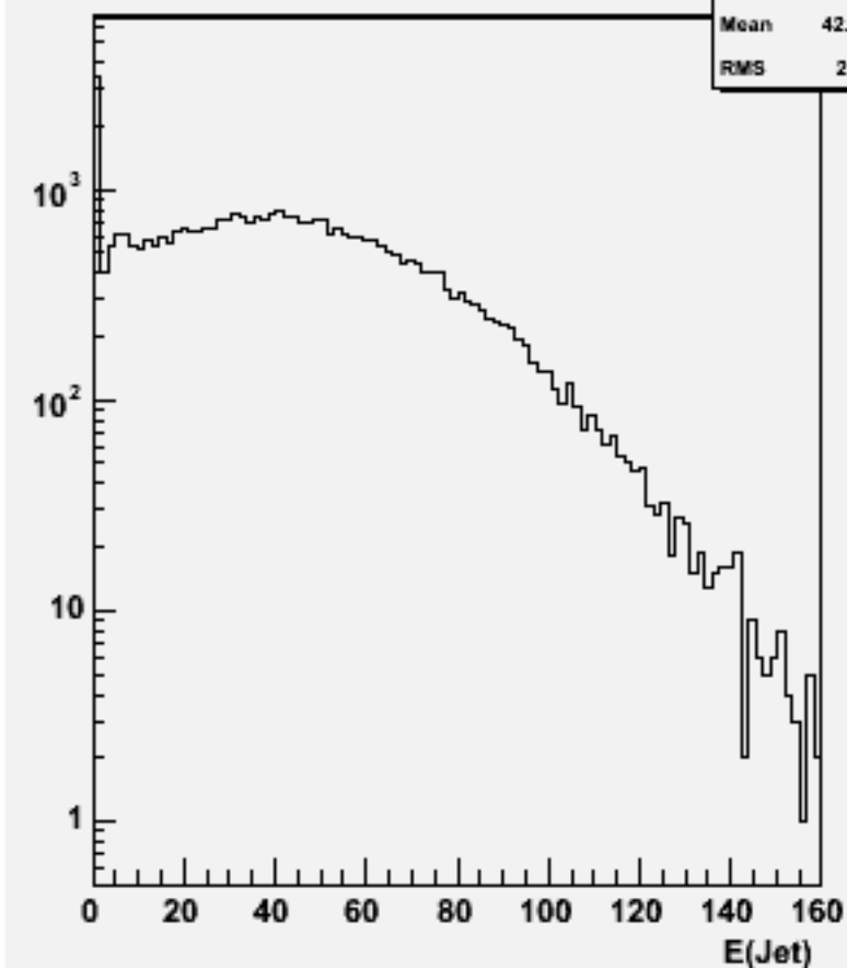
Jet energies(All jets)w101458 n2n2ude1n1_o
