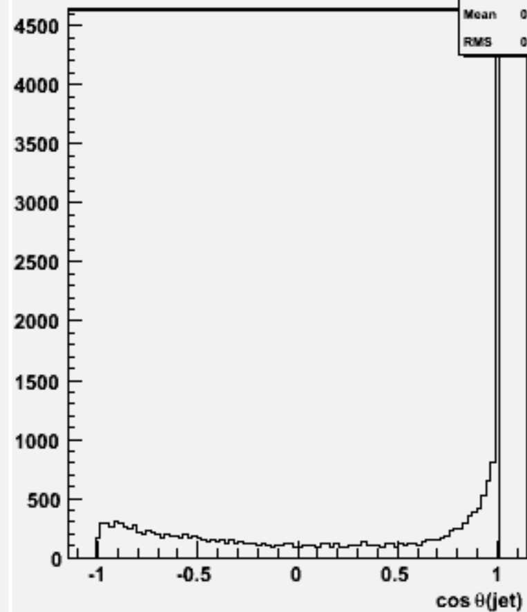
cos \theta for 2-jets :w101458 n2n2ude1n1_o
