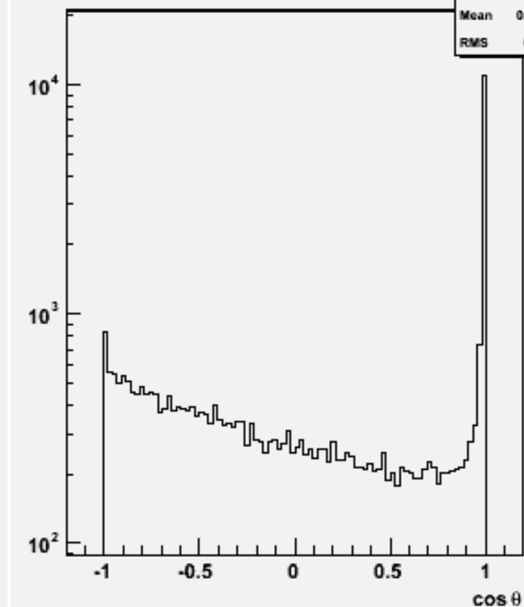
Jet cos \theta (All jets)w101458 n2n2ude1n1_o
