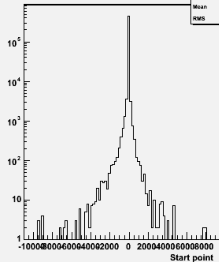
Start point Z : w101458 n2n2ude1n1_o
