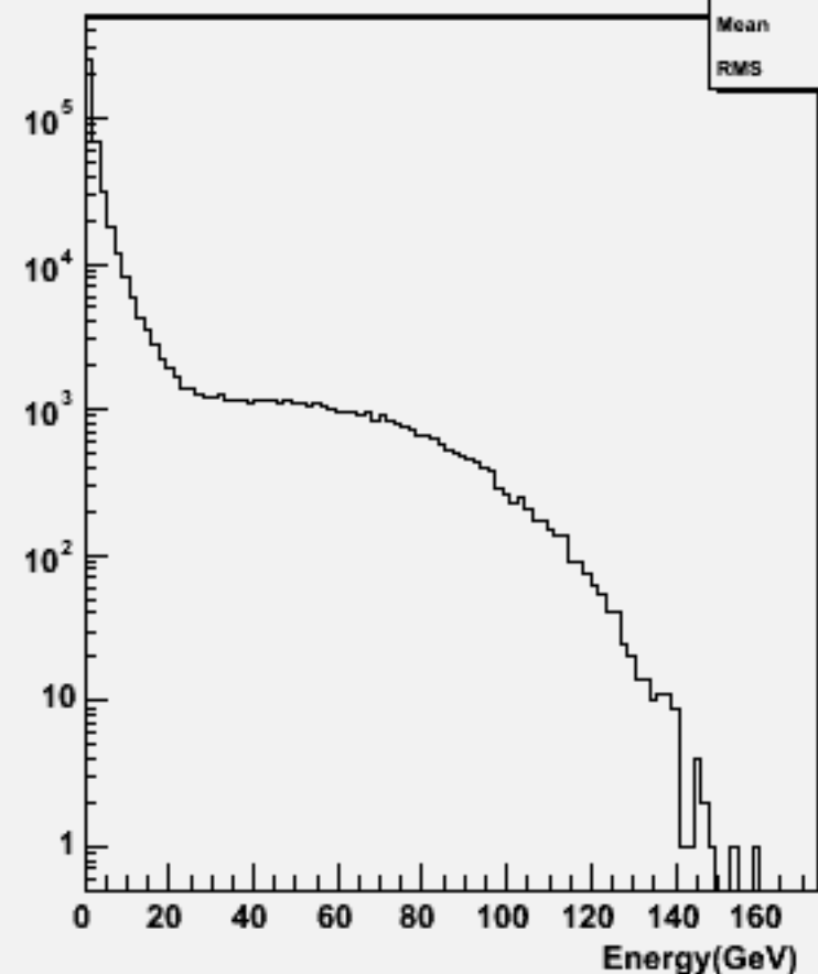
Start point R : w101458 n2n2ude1n1_o
