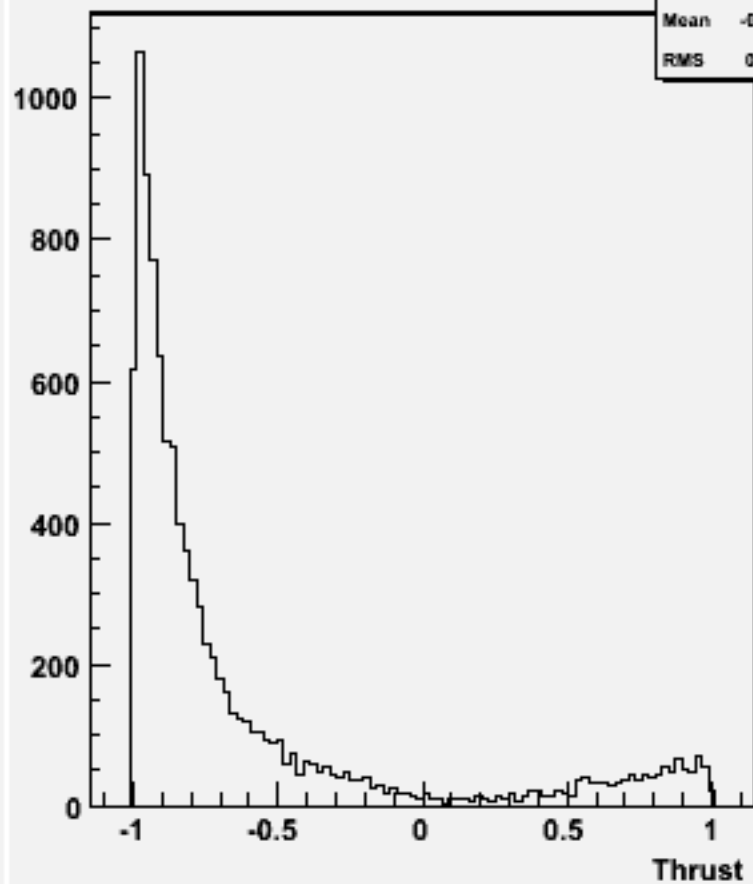
cos \Theta (thrust) w101458 n2n2ude1n1_o
