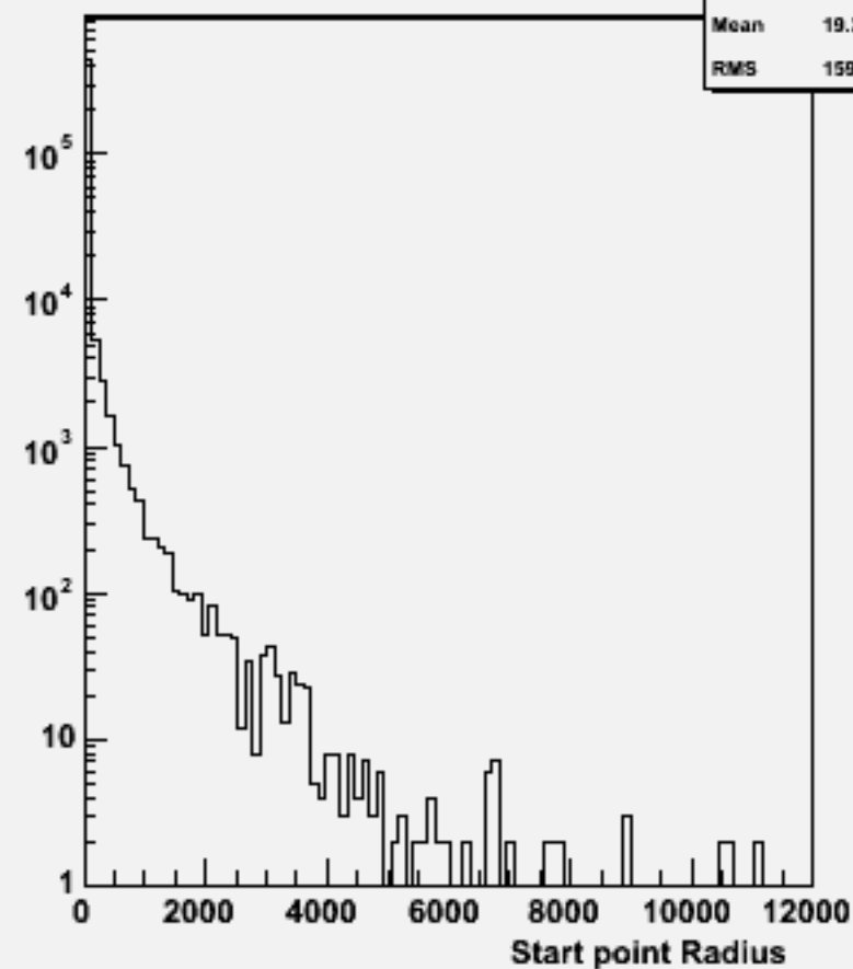
Start point R : w101458 n2n2ude1n1_o
