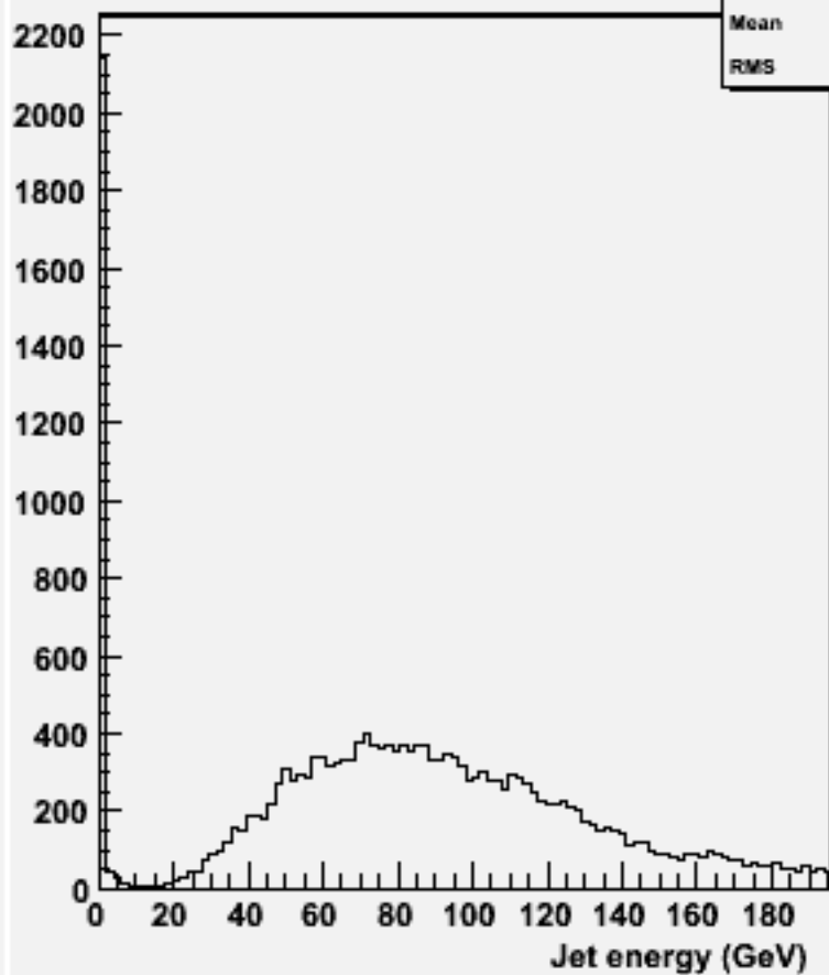
energy for 2-jets :w101458 n2n2ude1n1_o
