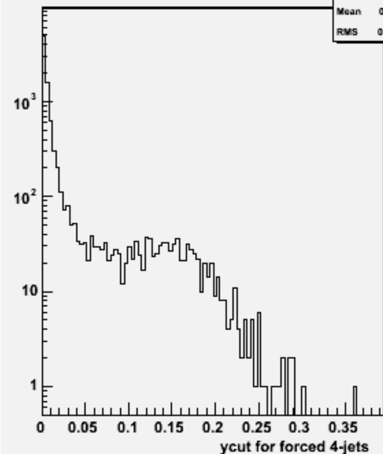
Ycut for 4-jets :w101458 n2n2ude1n1_o
