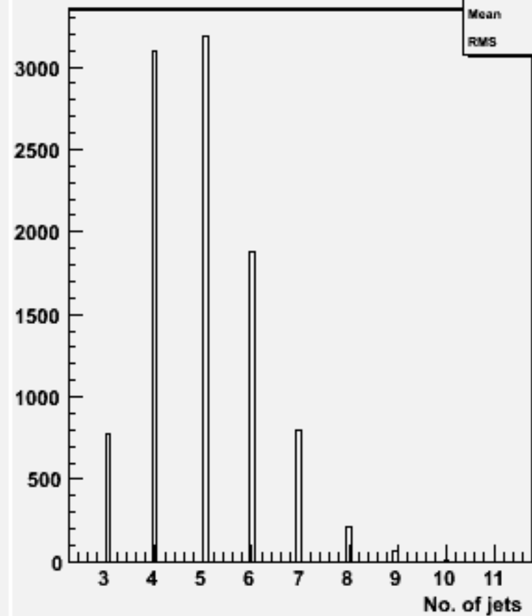
No. jets (ycut=0.001) : w101458 n2n2ude1n1_o
