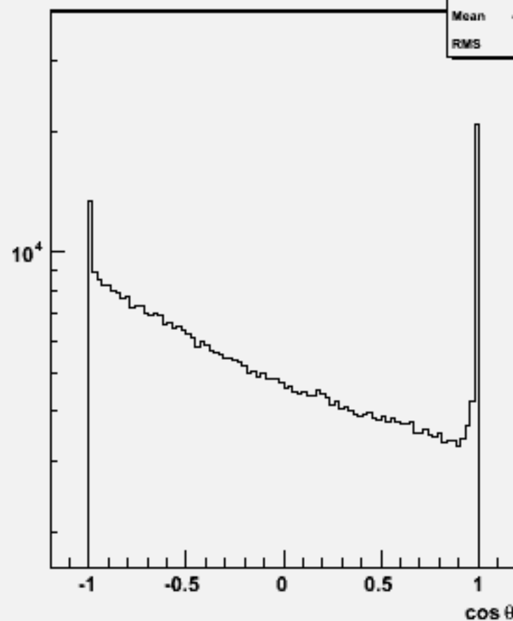
Particle cosθ : w101458 n2n2ude1n1_o
