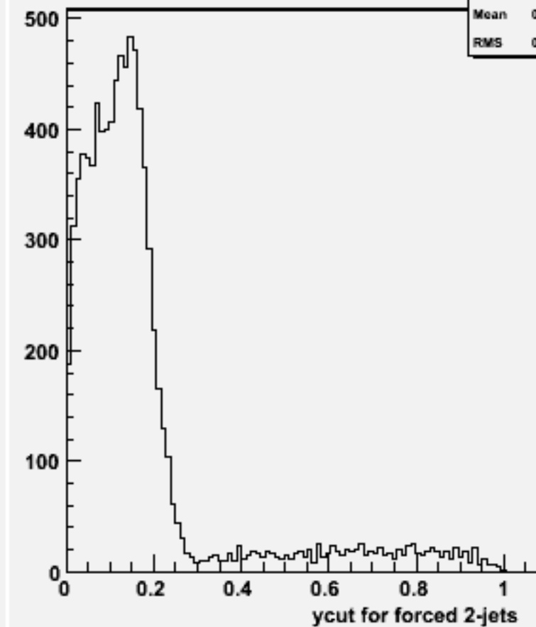
Ycut for 2-jets :w101458 n2n2ude1n1_o
