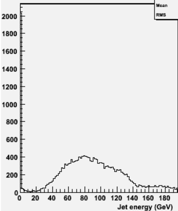
energy for 2-jets :w101457 n2n2ude1n1_o
