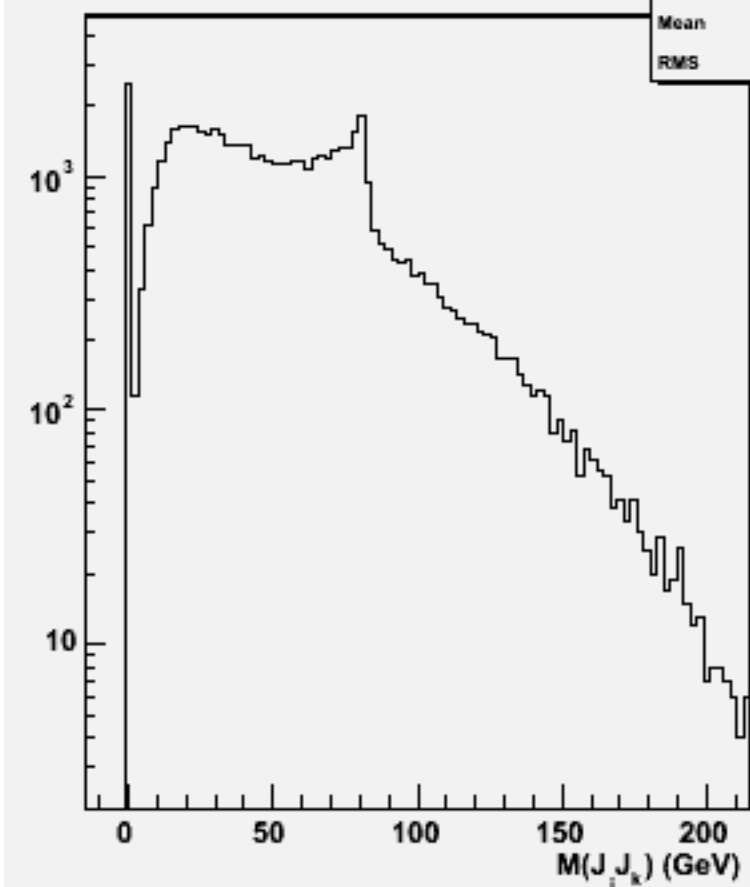
2jets mass(All comb)w101457 n2n2ude1n1_o
