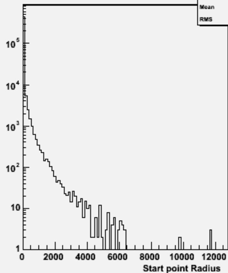
Start point R : w101457 n2n2ude1n1_o
