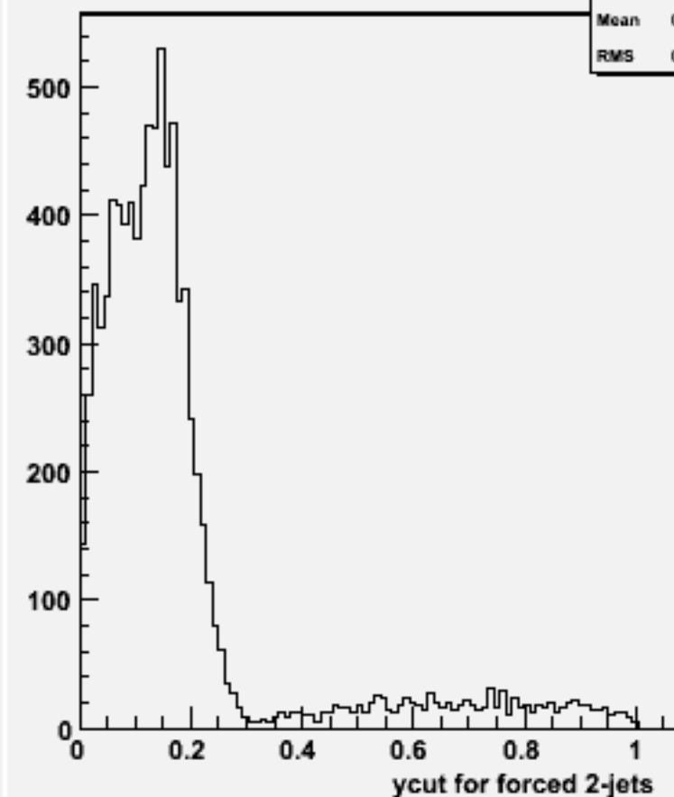
Ycut for 2-jets :w101457 n2n2ude1n1_o
