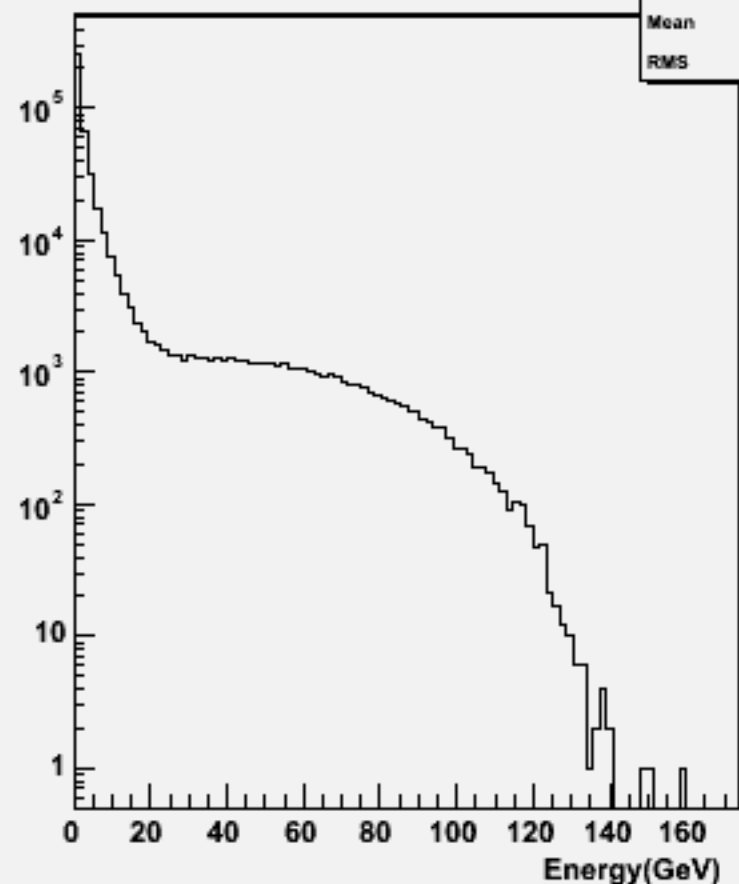
Start point R : w101457 n2n2ude1n1_o
