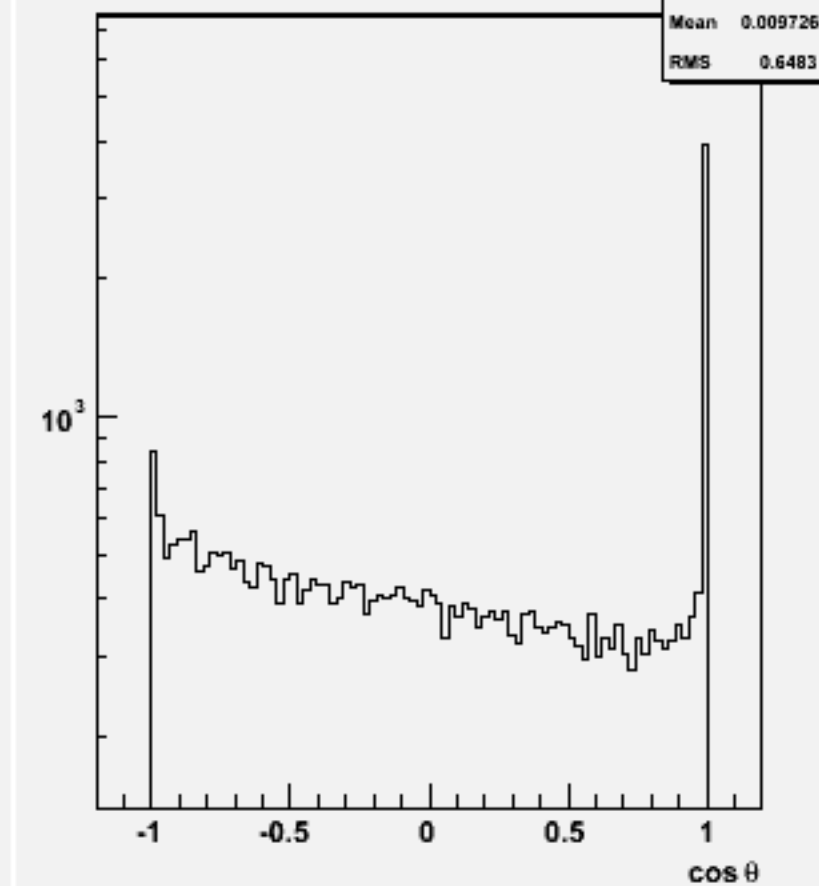
Jet cos \theta (All jets)w101457 n2n2ude1n1_o
