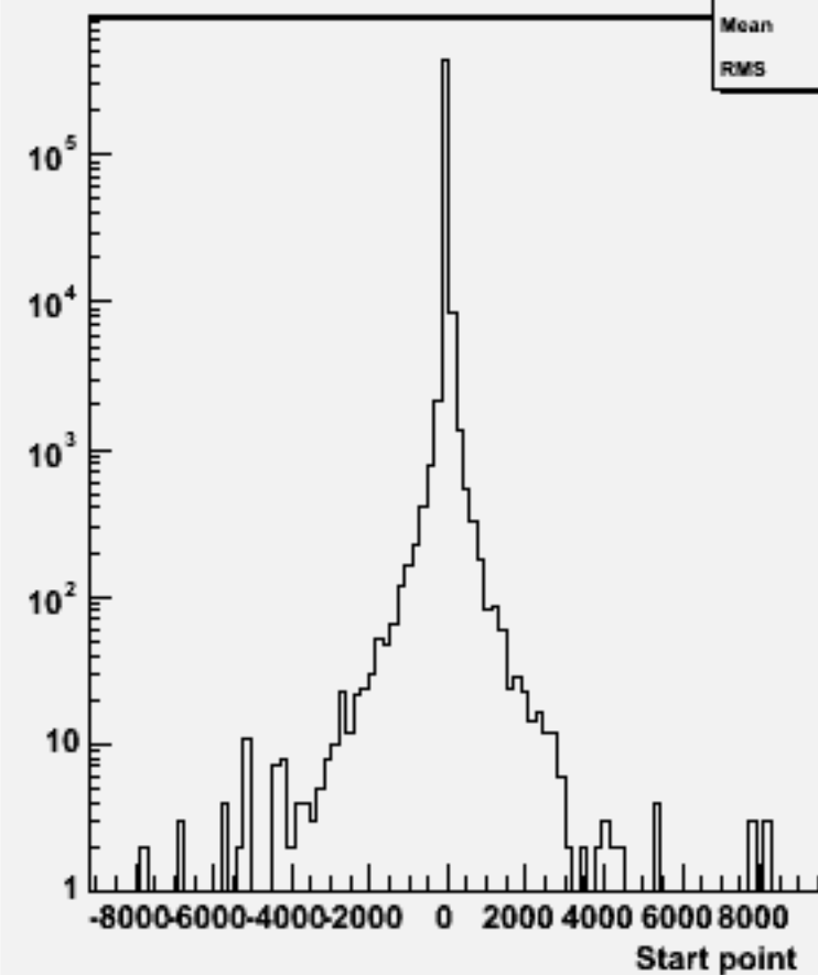
Start point Z : w101457 n2n2ude1n1_o
