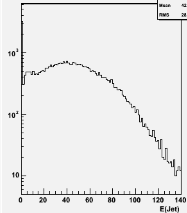
Jet energies(All jets)w101457 n2n2ude1n1_o
