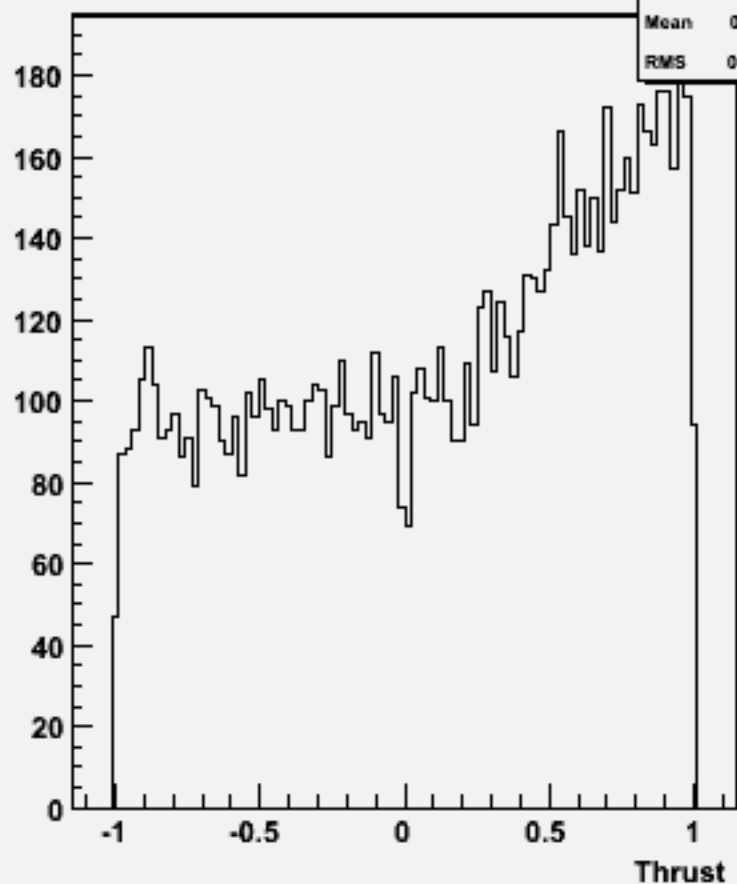
cos \Theta (thrust) w101457 n2n2ude1n1_o
