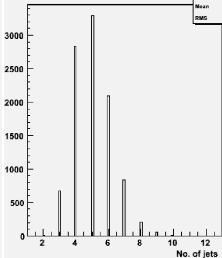
No. jets (ycut=0.001) : w101457 n2n2ude1n1_o
