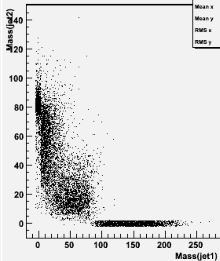
Jet mass for forced 2-jets : w101457 n2n2ude1n1_o
