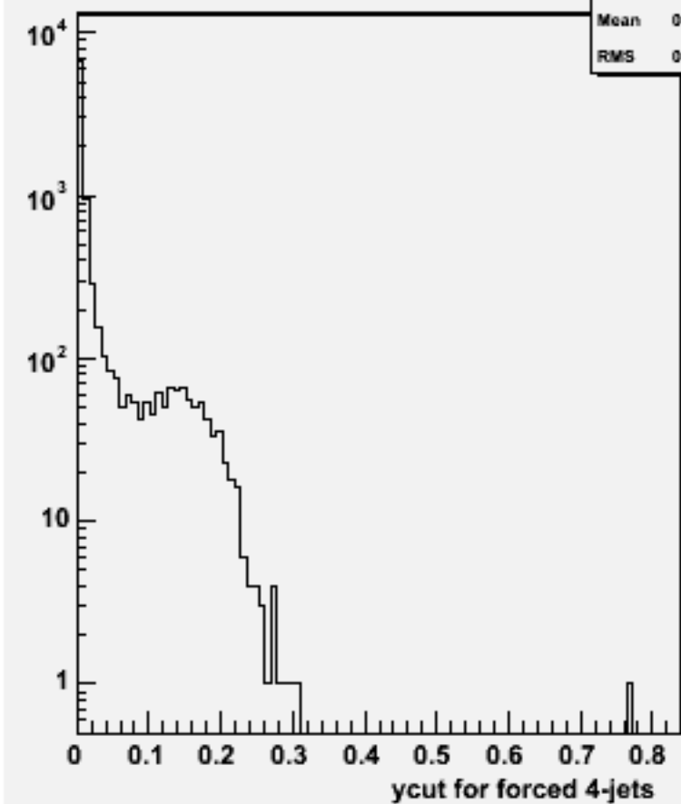
Ycut for 4-jets :w101457 n2n2ude1n1_o
