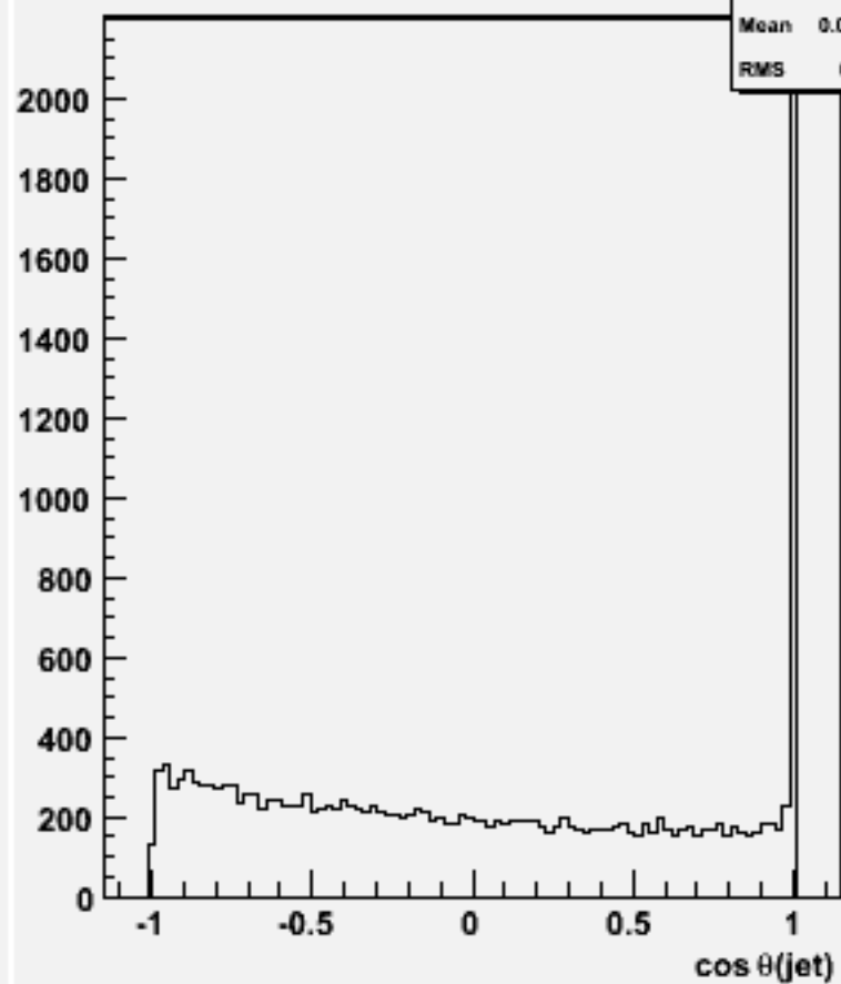
cos \theta for 2-jets :w101457 n2n2ude1n1_o
