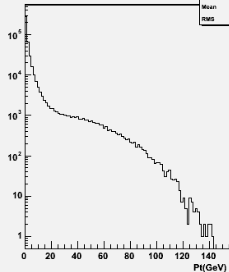
Start point Z : w101456 n2n2ude1n1_o
