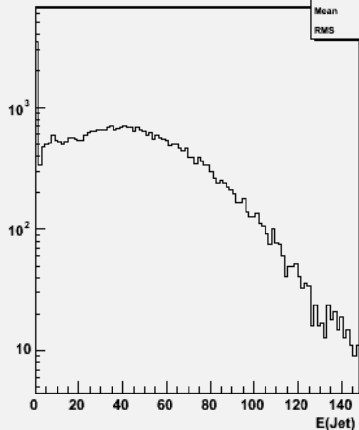
Jet energies(All jets)w101456 n2n2ude1n1_o
