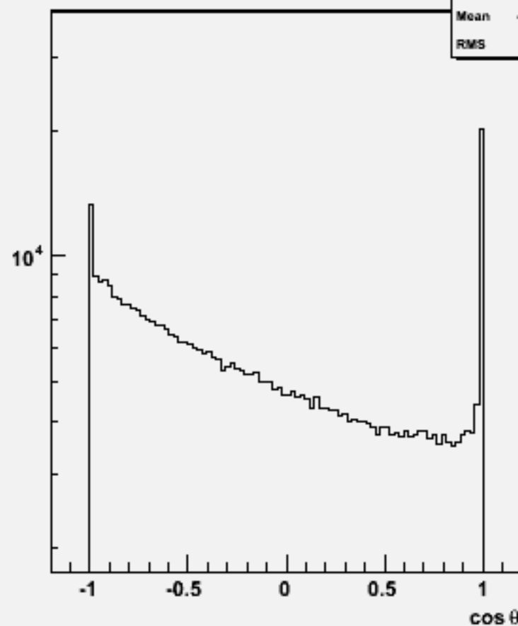
Particle cosθ : w101456 n2n2ude1n1_o
