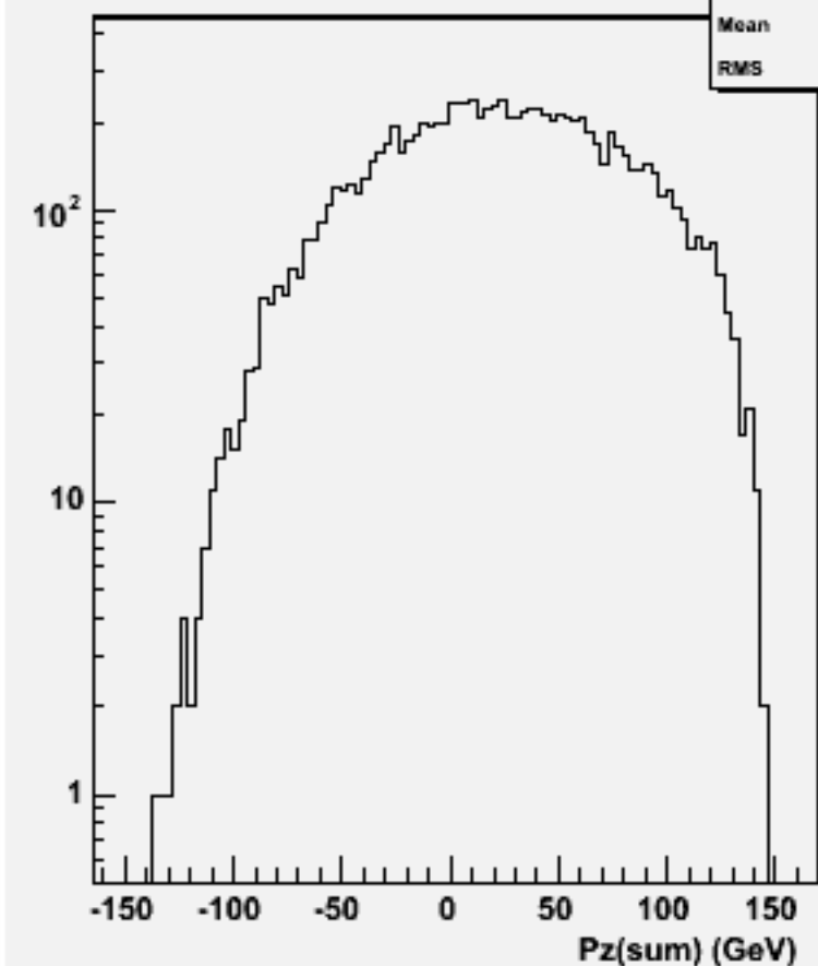
Pz Sum: w101456 n2n2ude1n1_o
