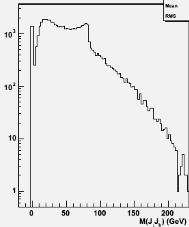
2jets mass(All comb)w101456 n2n2ude1n1_o
