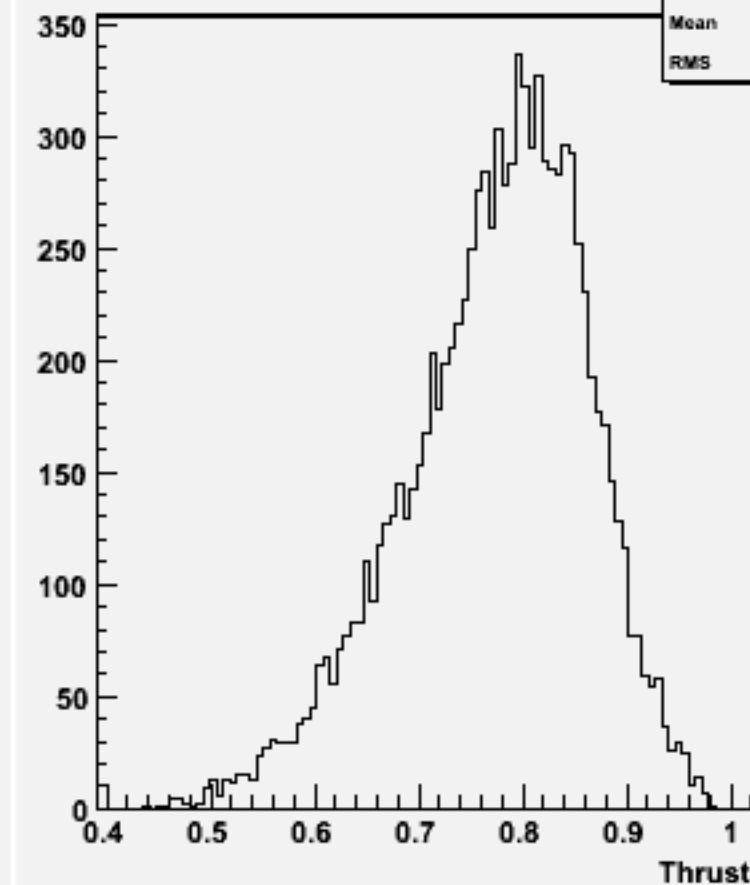
Thrust w101456 n2n2ude1n1_o
