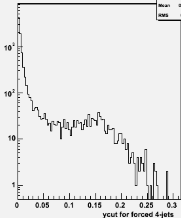
Ycut for 4-jets :w101456 n2n2ude1n1_o
