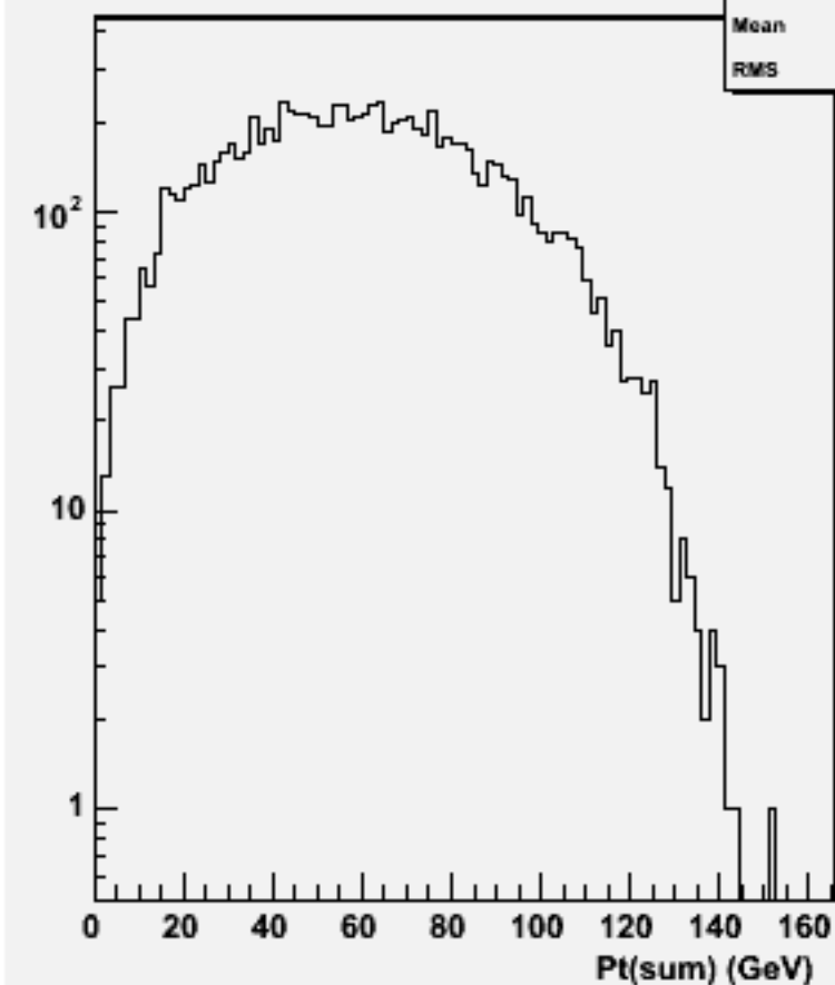
Pt Sum: w101456 n2n2ude1n1_o
