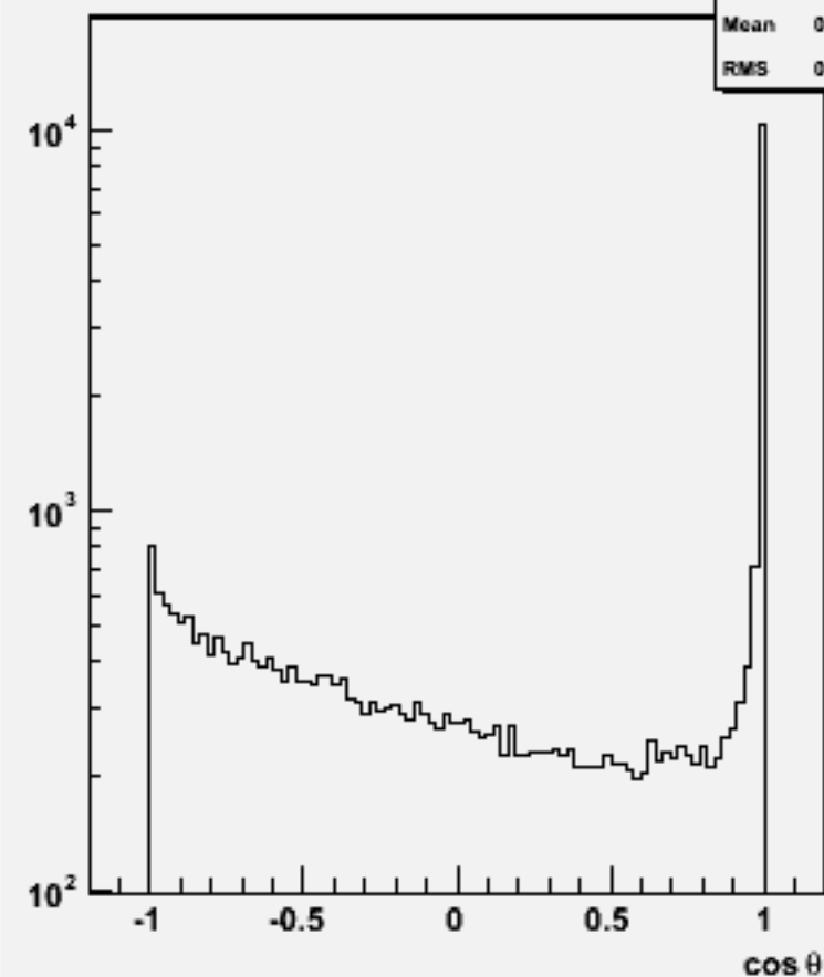
Jet cos \theta (All jets)w101456 n2n2ude1n1_o
