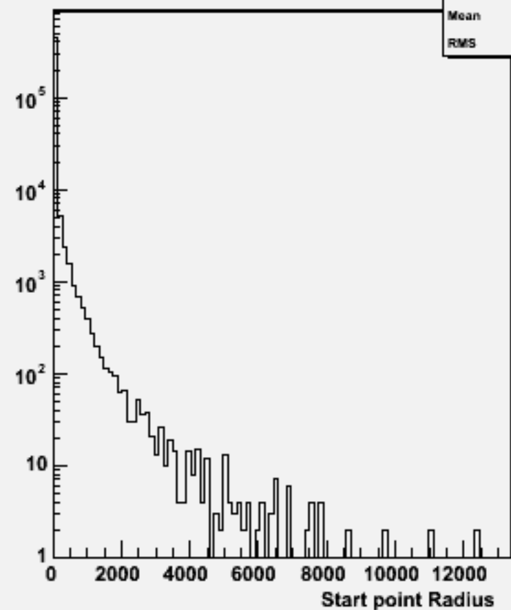
Start point R : w101456 n2n2ude1n1_o
