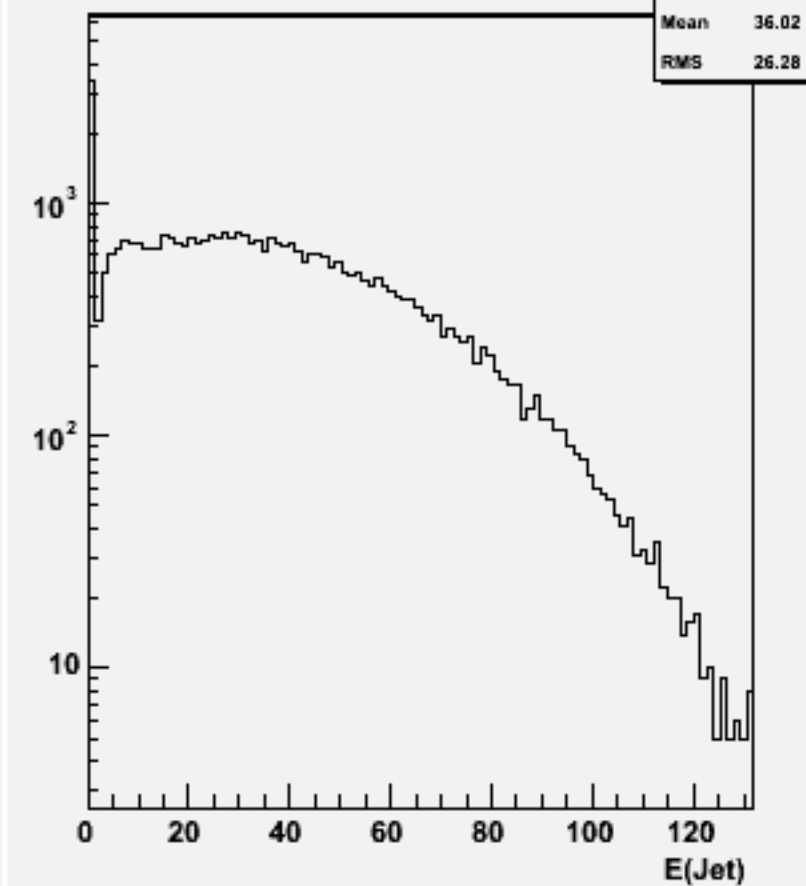
Jet energies(All jets)w101453 n2n2n3e3sc_o
