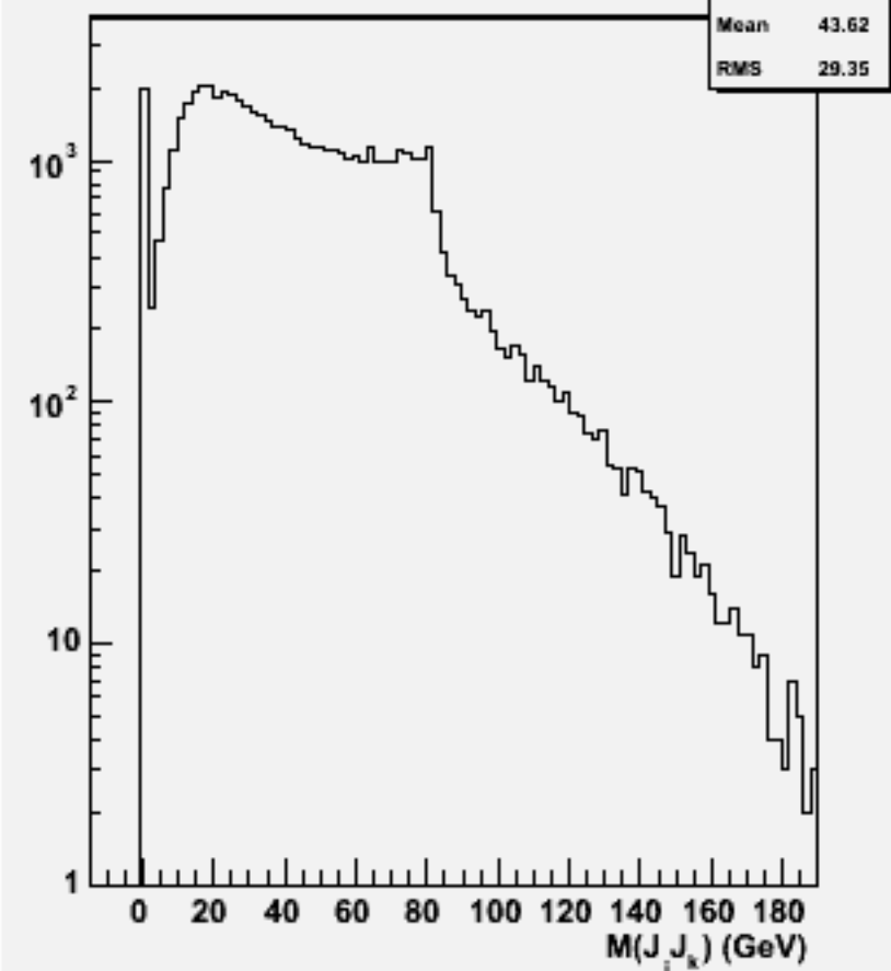
2jets mass(All comb)w101453 n2n2n3e3sc_o
