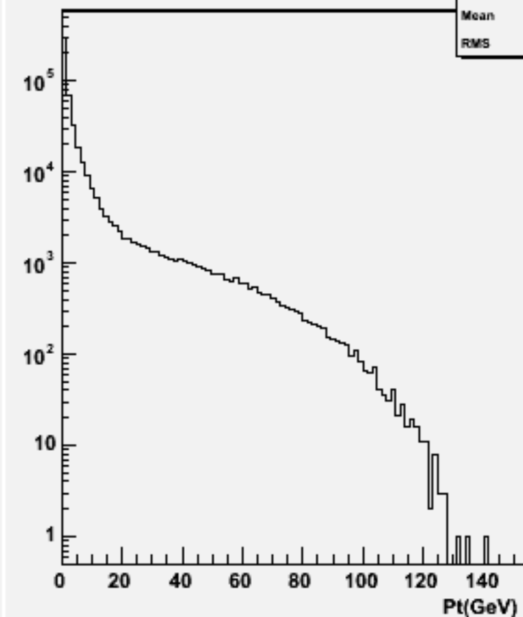
Particle Pt : w101453 n2n2n3e3sc_o
