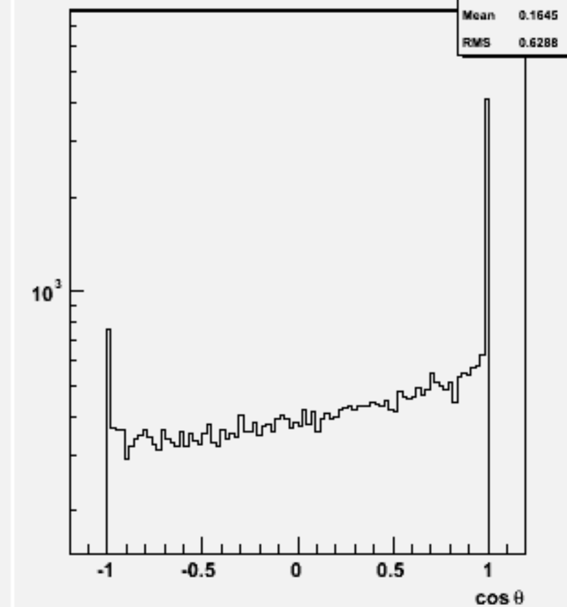
Jet cos \theta (All jets)w101453 n2n2n3e3sc_o
