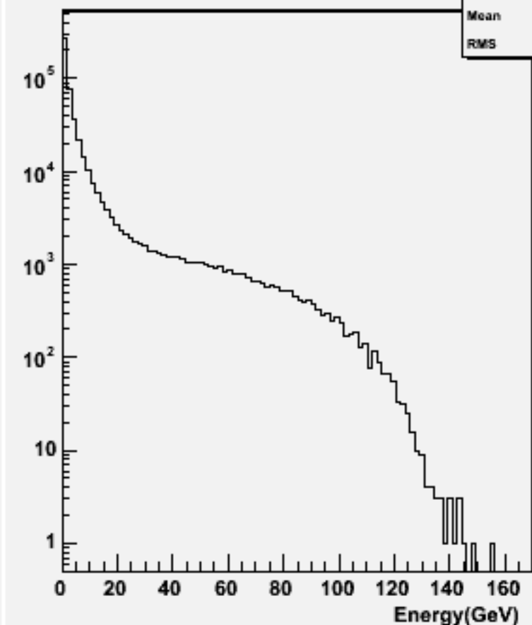
Particle Energy : w101453 n2n2n3e3sc_o
