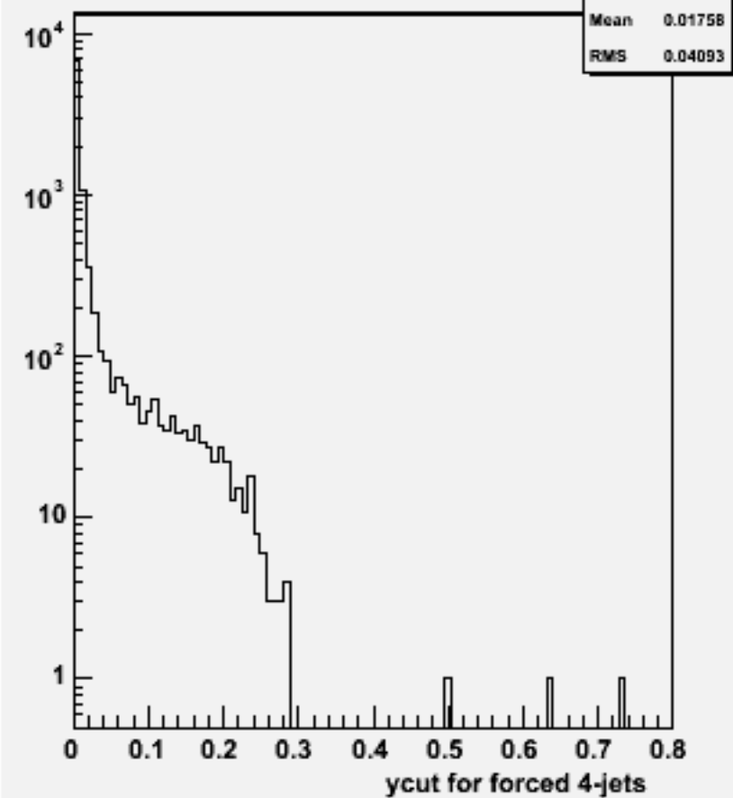
Ycut for 4-jets :w101453 n2n2n3e3sc_o
