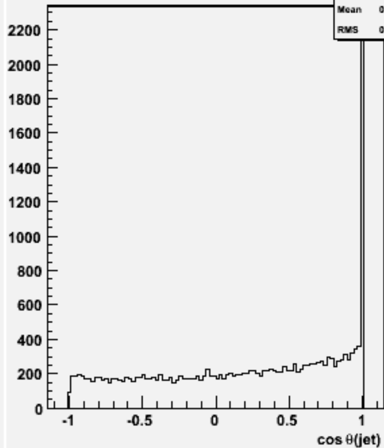
cos \theta for 2-jets :w101453 n2n2n3e3sc_o
