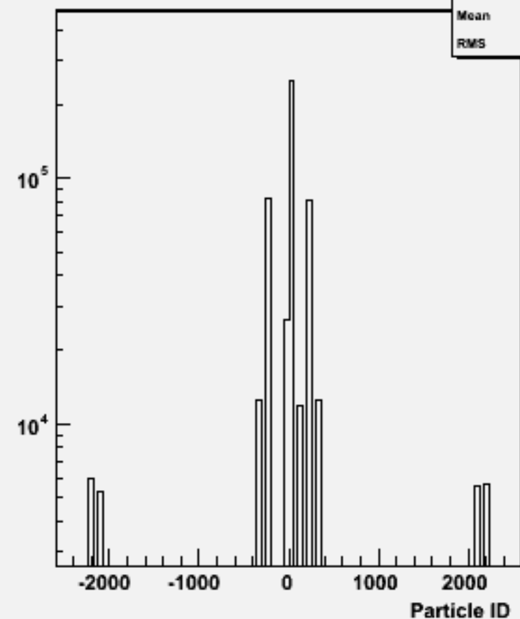
Particle ID : w101453 n2n2n3e3sc_o
