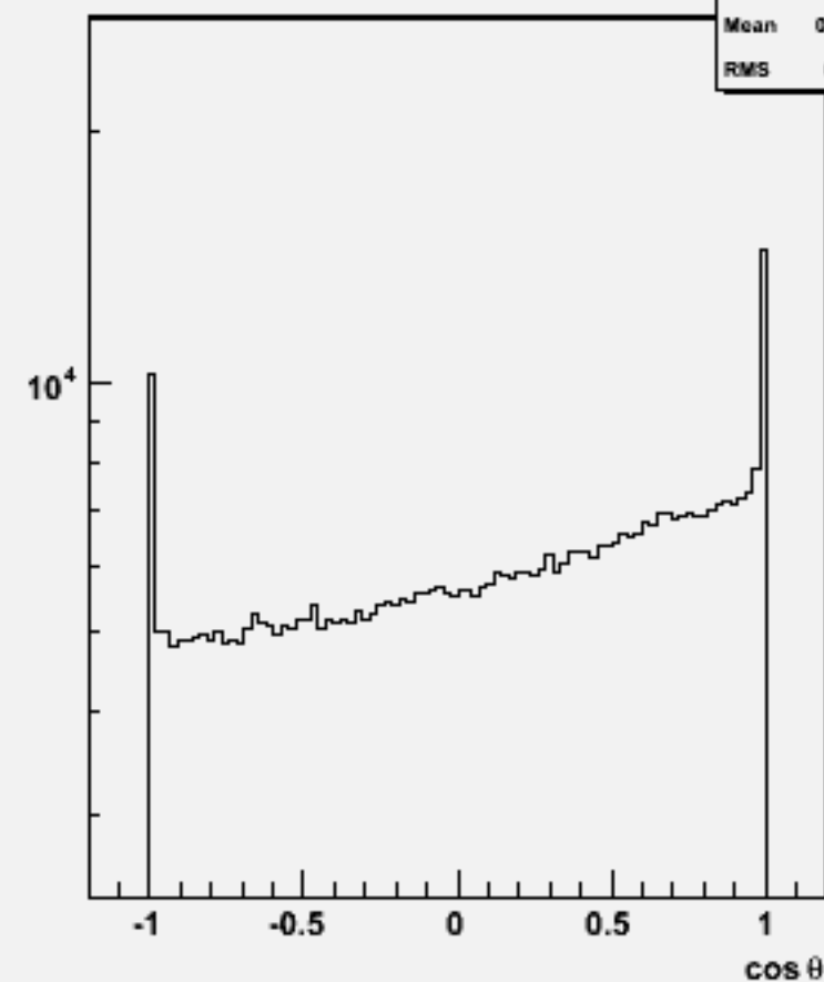
Particle cosθ : w101453 n2n2n3e3sc_o
