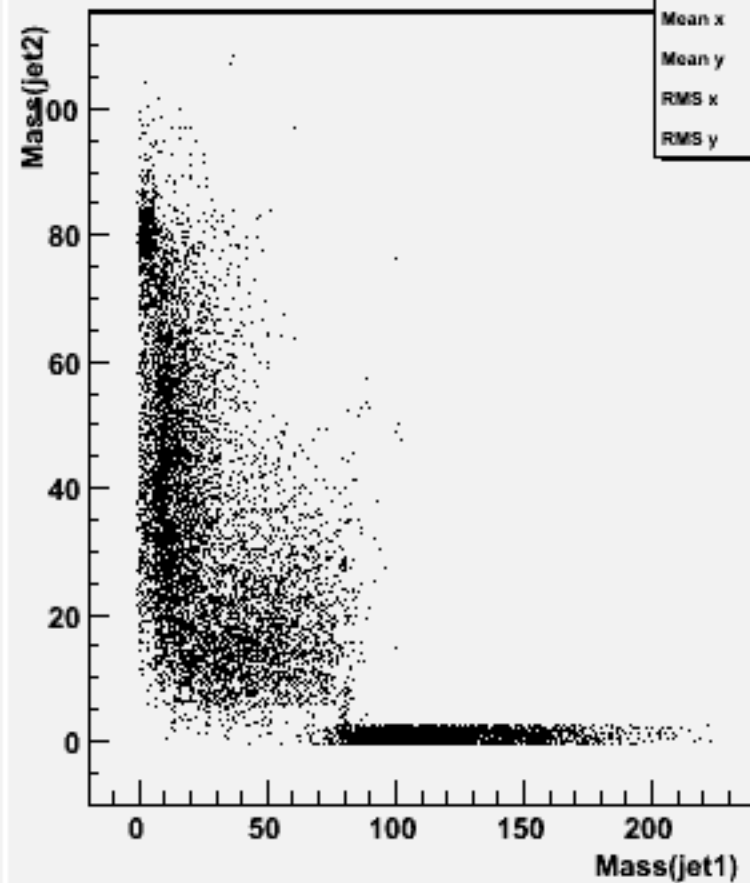
Jet mass for forced 2-jets : w101453 n2n2n3e3sc_o
