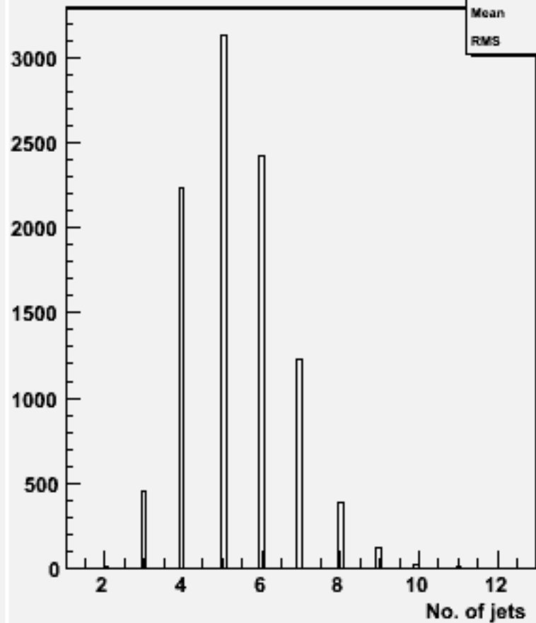
No. jets (ycut=0.001) : w101453 n2n2n3e3sc_o
