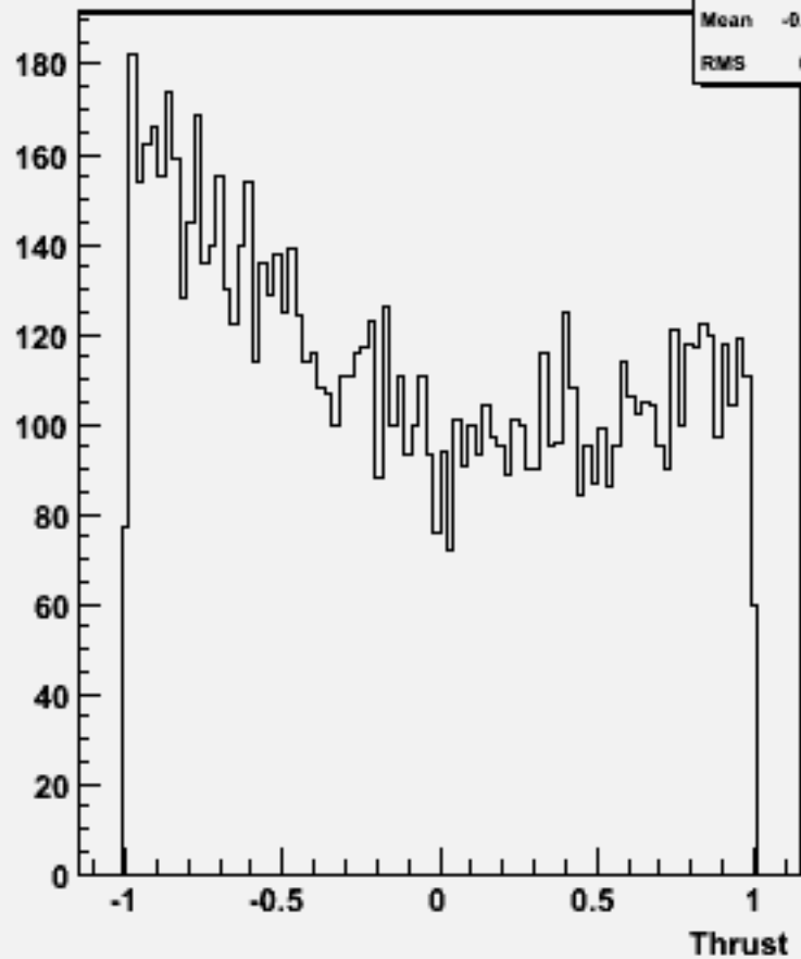
cos \Theta (thrust) w101453 n2n2n3e3sc_o
