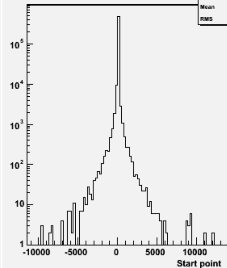
Start point Z : w101453 n2n2n3e3sc_o
