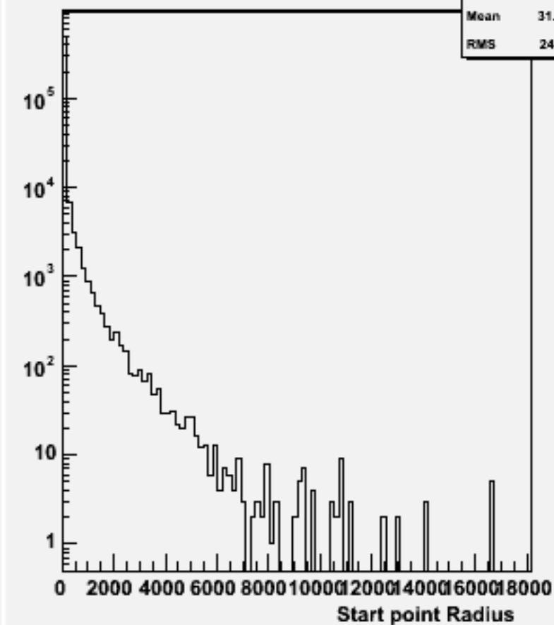
Start point R : w101453 n2n2n3e3sc_o
