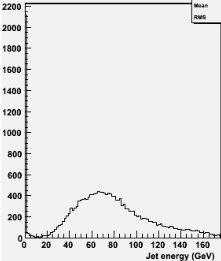
energy for 2-jets :w101453 n2n2n3e3sc_o
