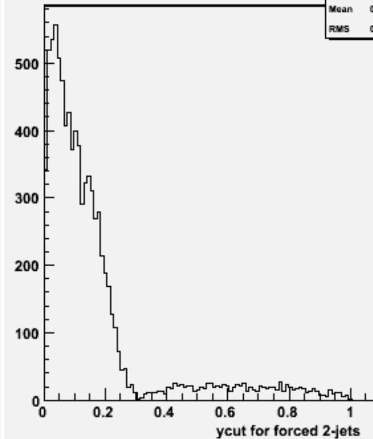
Ycut for 2-jets :w101453 n2n2n3e3sc_o
