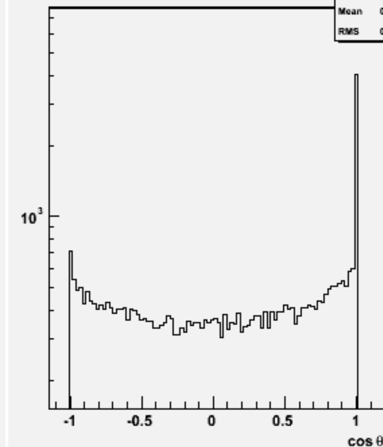
Jet cos \theta (All jets)w101452 n2n2n3e3sc_o
