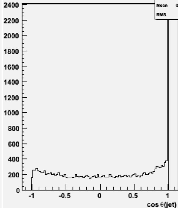
cos \theta for 2-jets :w101452 n2n2n3e3sc_o
