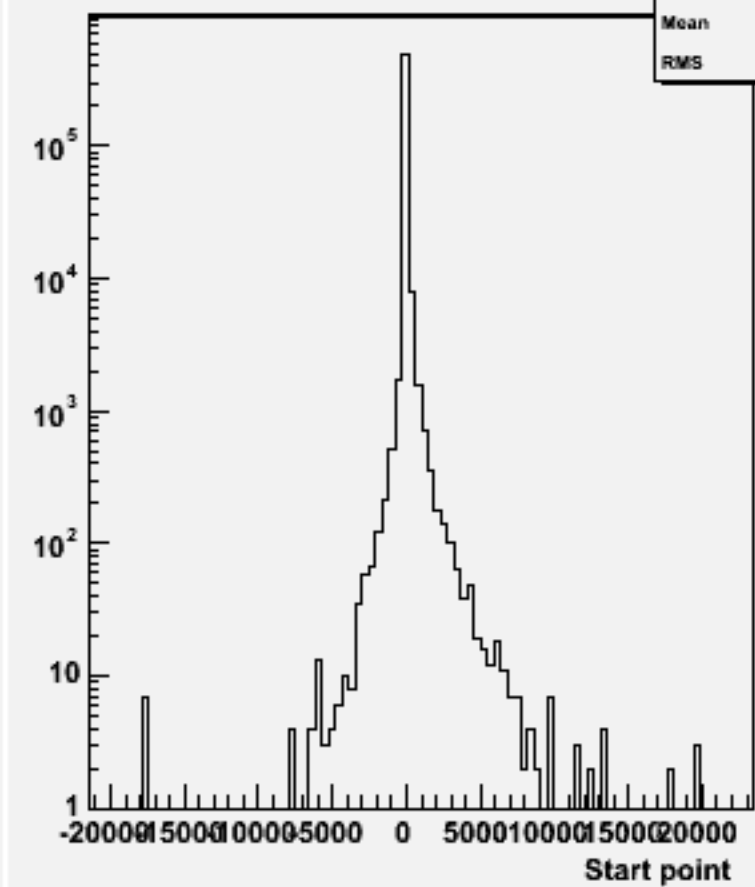
Start point Z : w101452 n2n2n3e3sc_o
