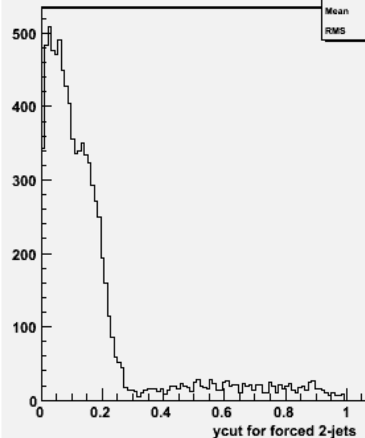
Ycut for 2-jets :w101452 n2n2n3e3sc_o
