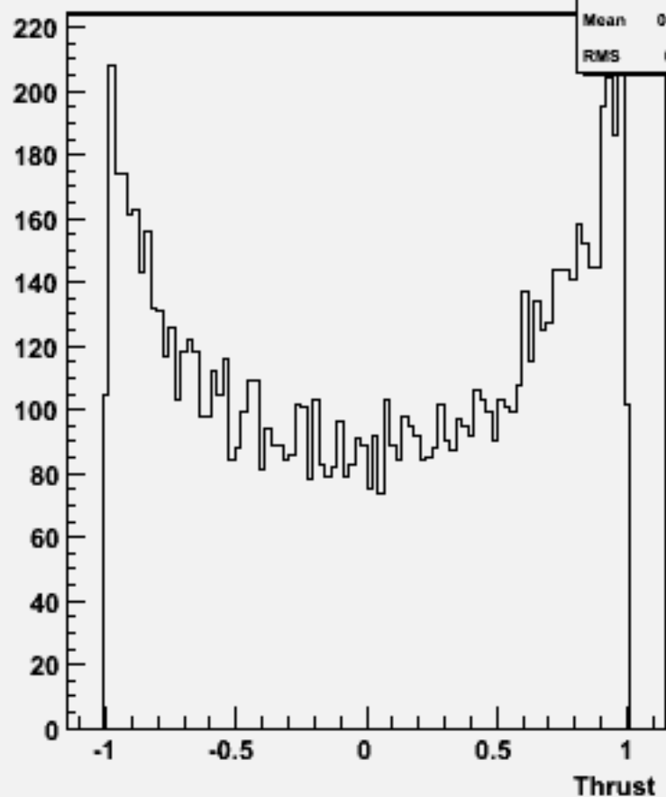
cos \Theta (thrust) w101452 n2n2n3e3sc_o
