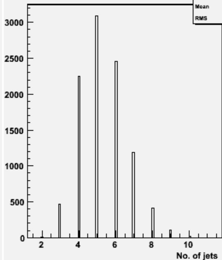
No. jets (ycut=0.001) : w101452 n2n2n3e3sc_o
