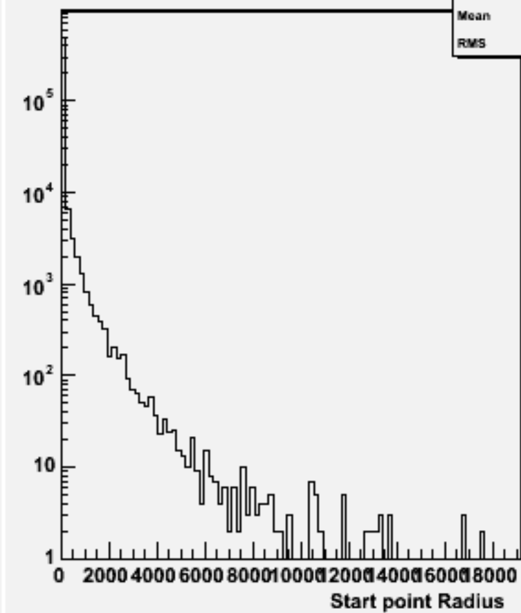
Start point R : w101452 n2n2n3e3sc_o
