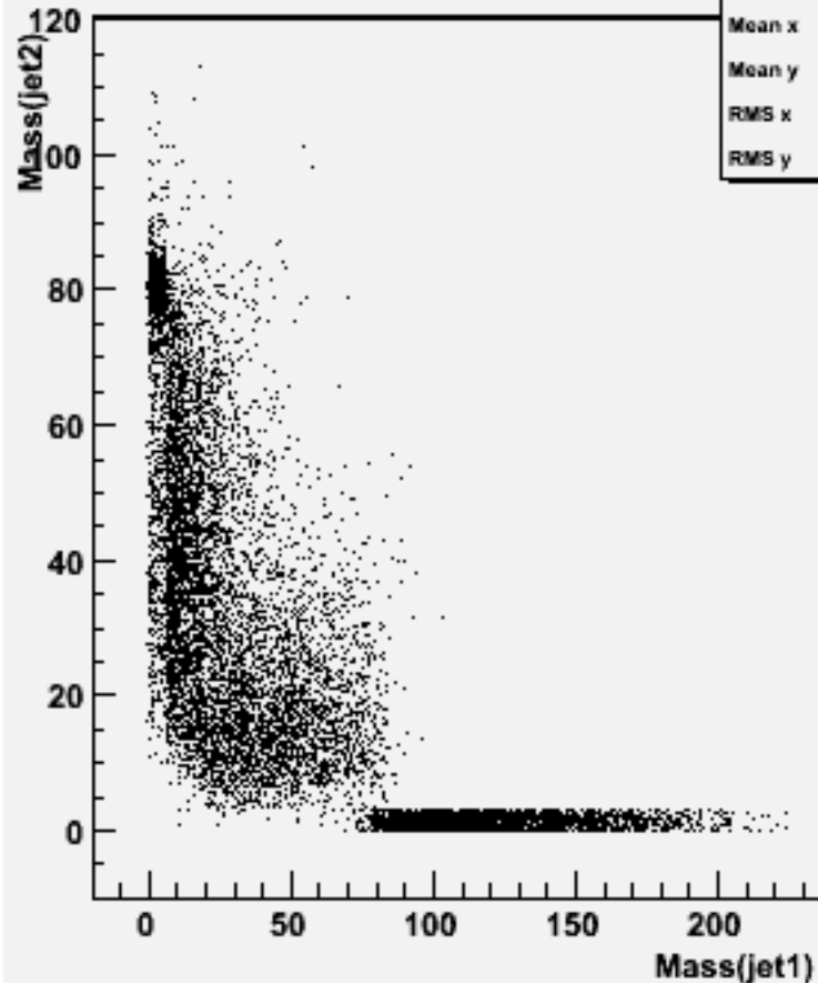
Jet mass for forced 2-jets : w101452 n2n2n3e3sc_o
