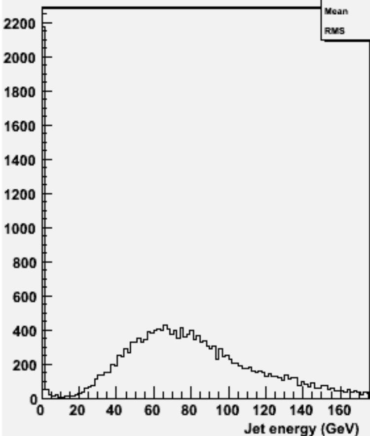
energy for 2-jets :w101452 n2n2n3e3sc_o
