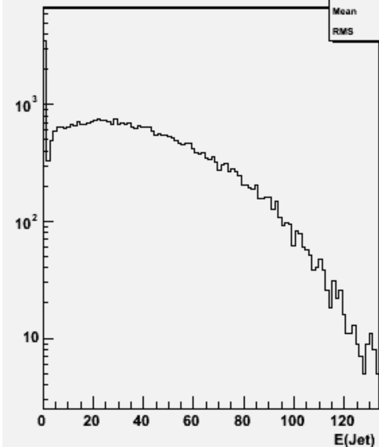
Jet energies(All jets)w101452 n2n2n3e3sc_o
