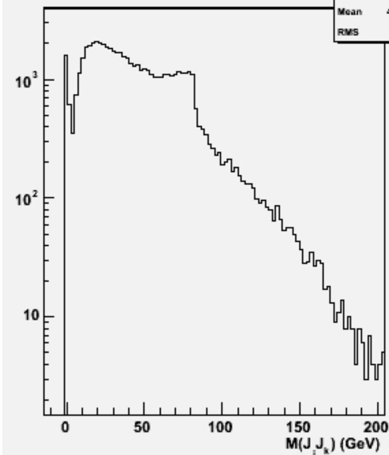
2jets mass(All comb)w101452 n2n2n3e3sc_o
