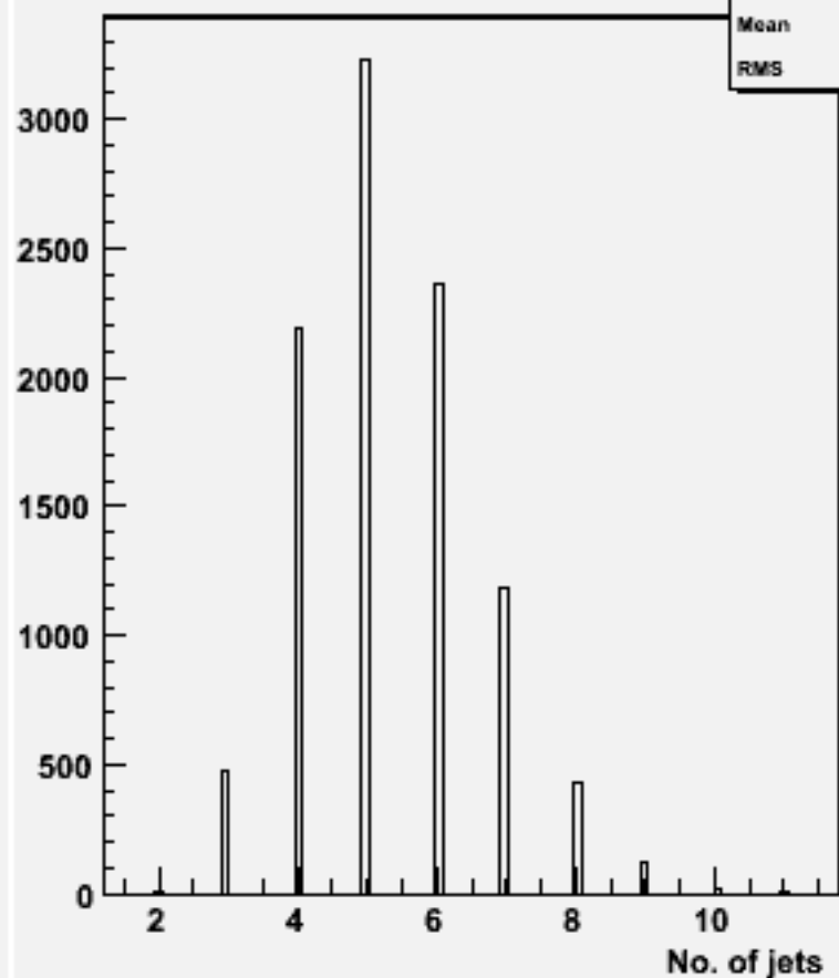
No. jets (ycut=0.001) : w101449 n2n2n3e3du_o
