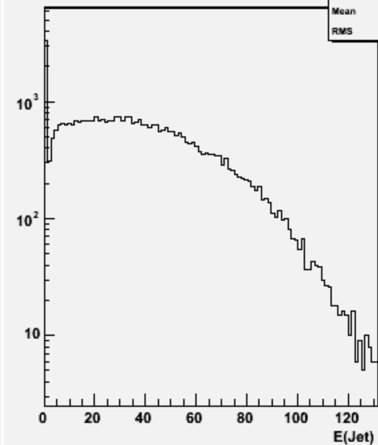
Jet energies(All jets)w101449 n2n2n3e3du_o
