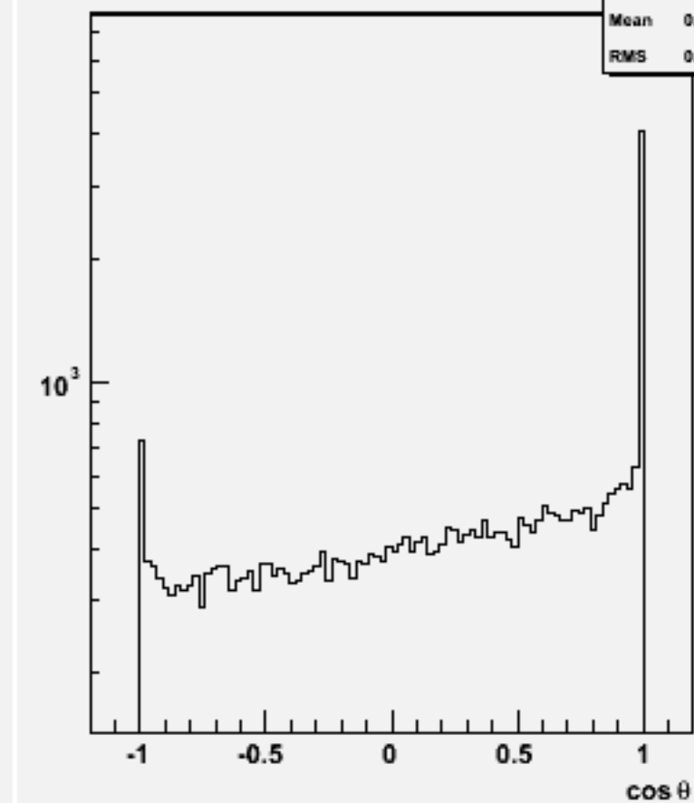
Jet cos \theta (All jets)w101449 n2n2n3e3du_o
