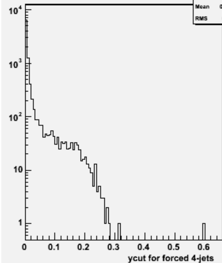
Ycut for 4-jets :w101449 n2n2n3e3du_o
