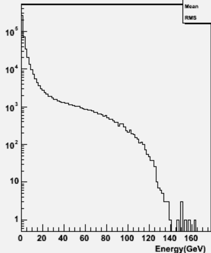
Start point R : w101449 n2n2n3e3du_o
