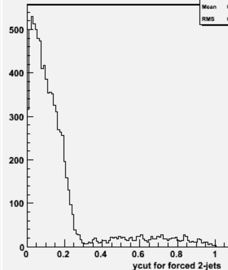
Ycut for 2-jets :w101449 n2n2n3e3du_o
