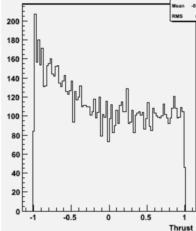
cos \Theta (thrust) w101449 n2n2n3e3du_o
