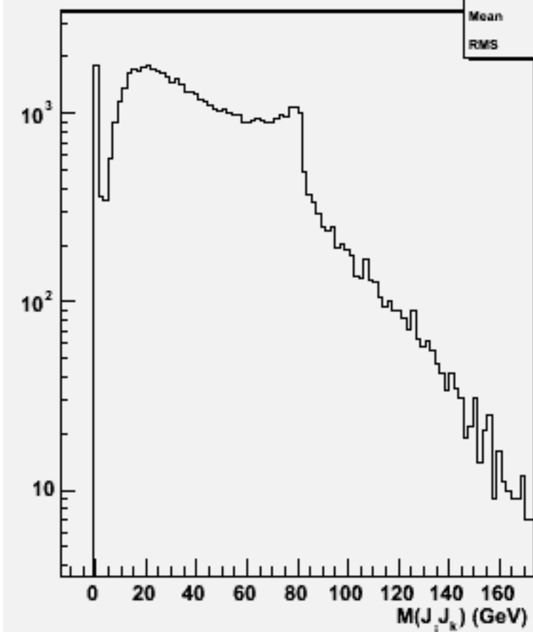
2jets mass(All comb)w101449 n2n2n3e3du_o
