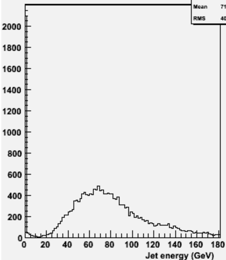
energy for 2-jets :w101449 n2n2n3e3du_o
