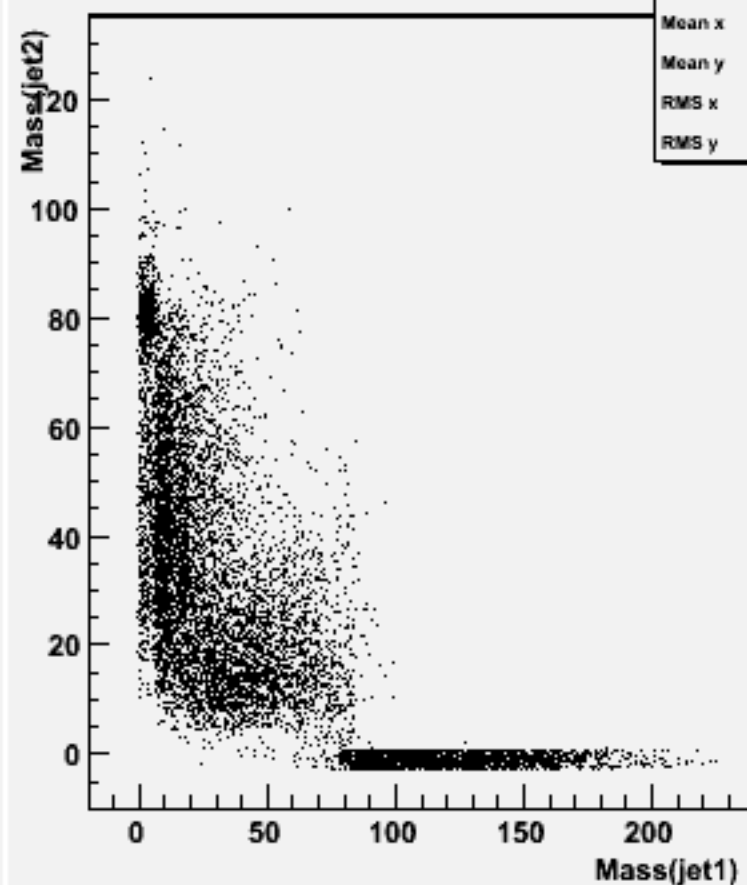
Jet mass for forced 2-jets : w101449 n2n2n3e3du_o
