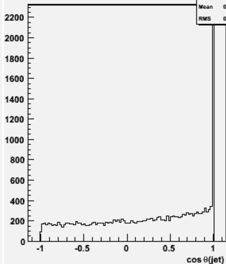
cos \theta for 2-jets :w101449 n2n2n3e3du_o
