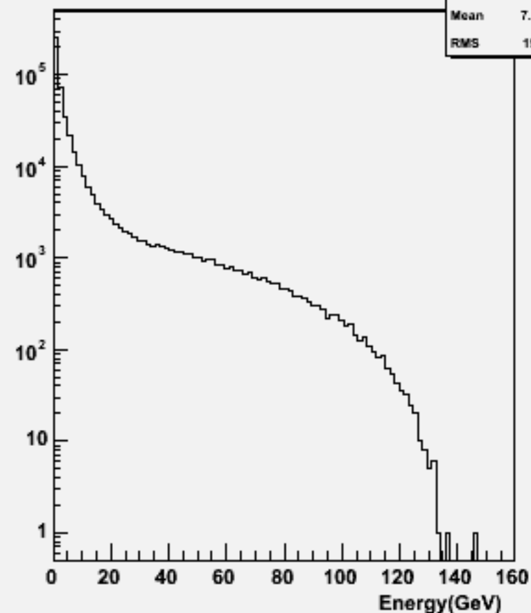
Start point R : w101448 n2n2n3e3du_o
