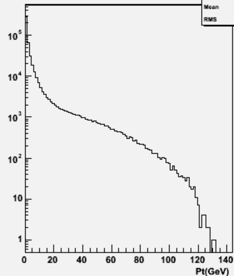
Start point Z : w101448 n2n2n3e3du_o
