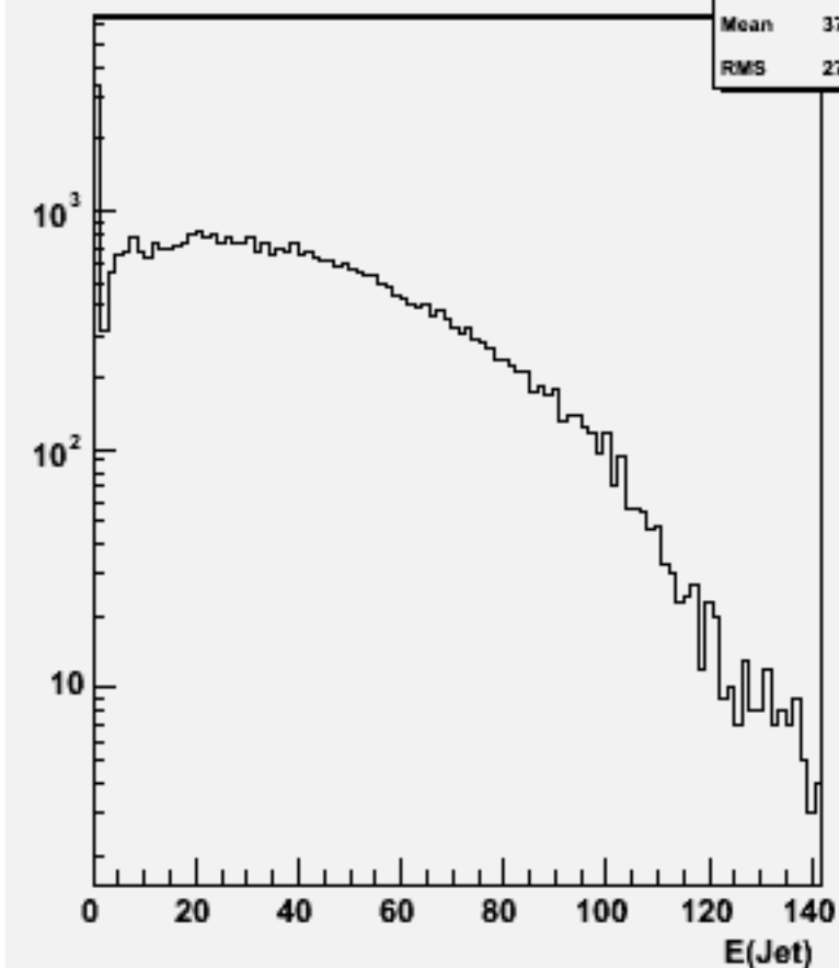
Jet energies(All jets)w101448 n2n2n3e3du_o
