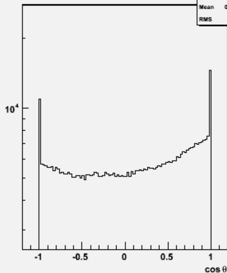
Particle cos \theta : w101448 n2n2n3e3du_o
