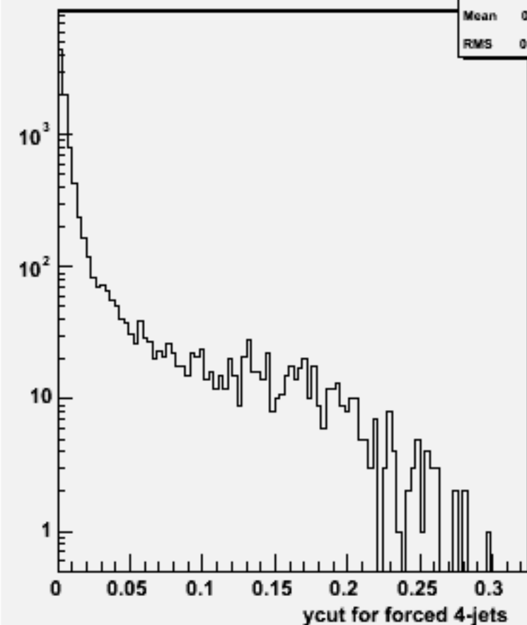
Ycut for 4-jets :w101448 n2n2n3e3du_o
