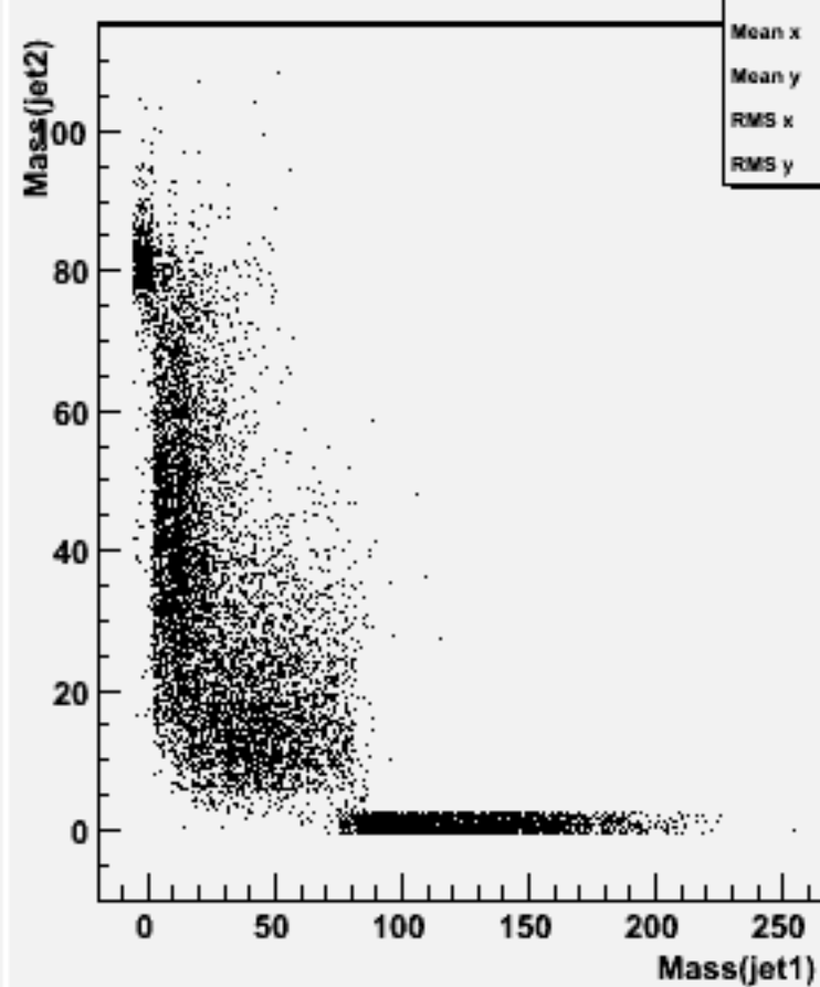
Jet mass for forced 2-jets : w101448 n2n2n3e3du_o
