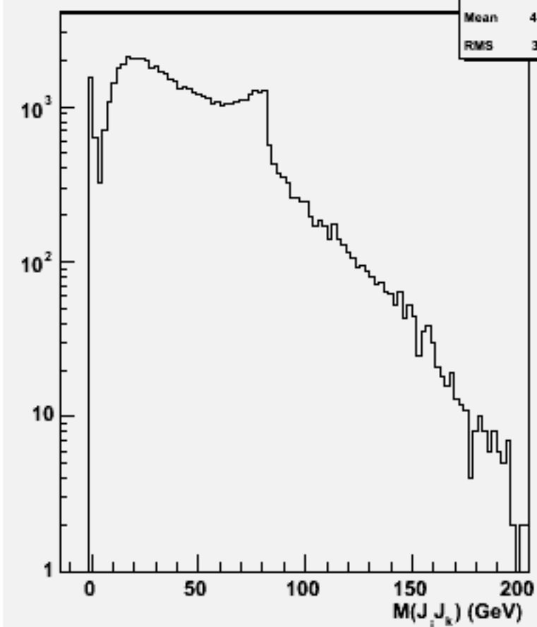
2jets mass(All comb)w101448 n2n2n3e3du_o
