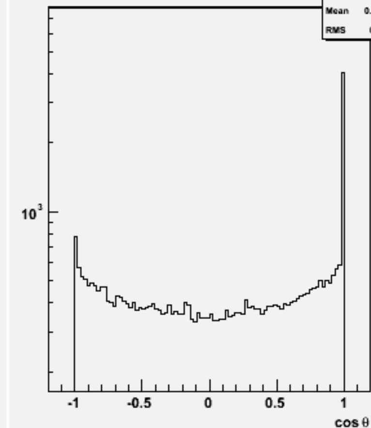
Jet cos \theta (All jets)w101448 n2n2n3e3du_o
