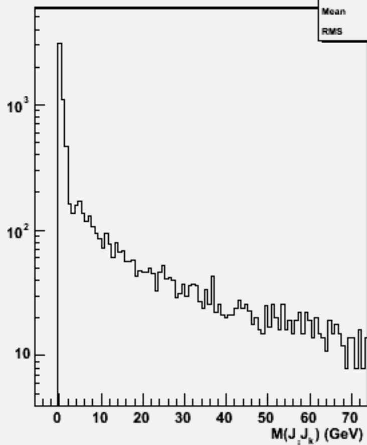
2jets mass(All comb)w101440 n2n2n3e3e2n2_o
