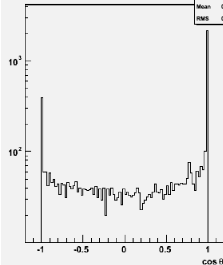
Jet cos \theta (All jets)w101440 n2n2n3e3e2n2_o
