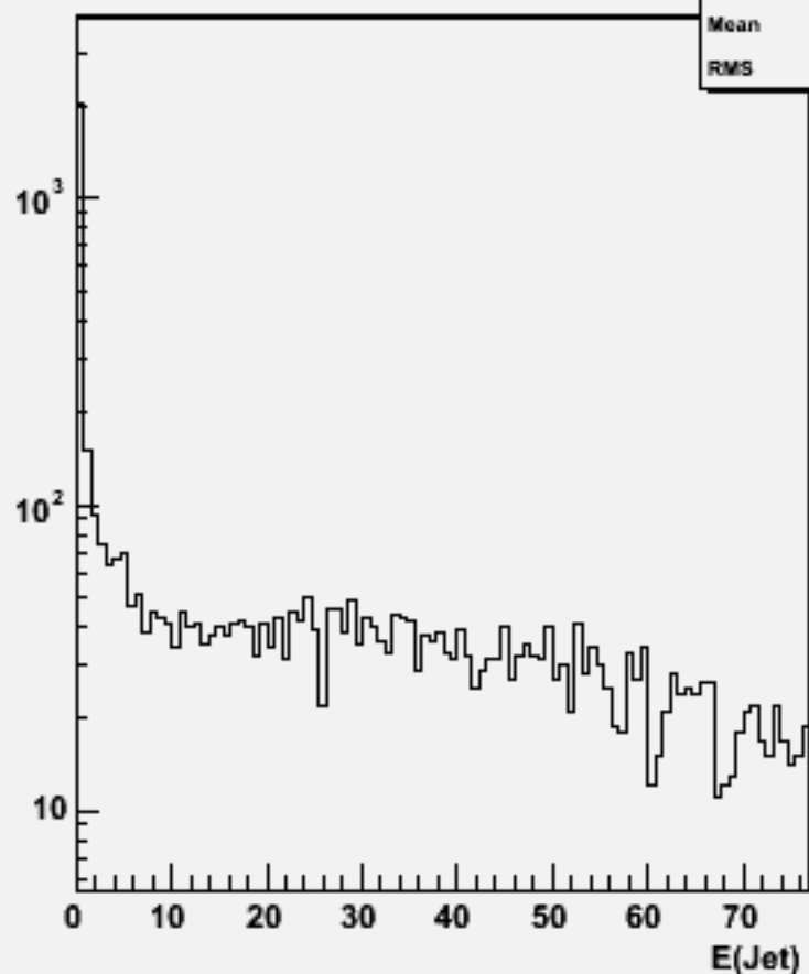
Jet energies(All jets)w101440 n2n2n3e3e2n2_o
