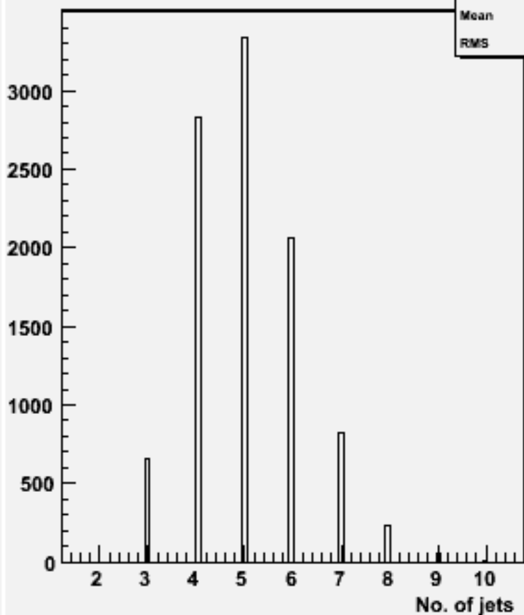
No. jets (ycut=0.001) : w101433 n2n2n2e2sc_o
