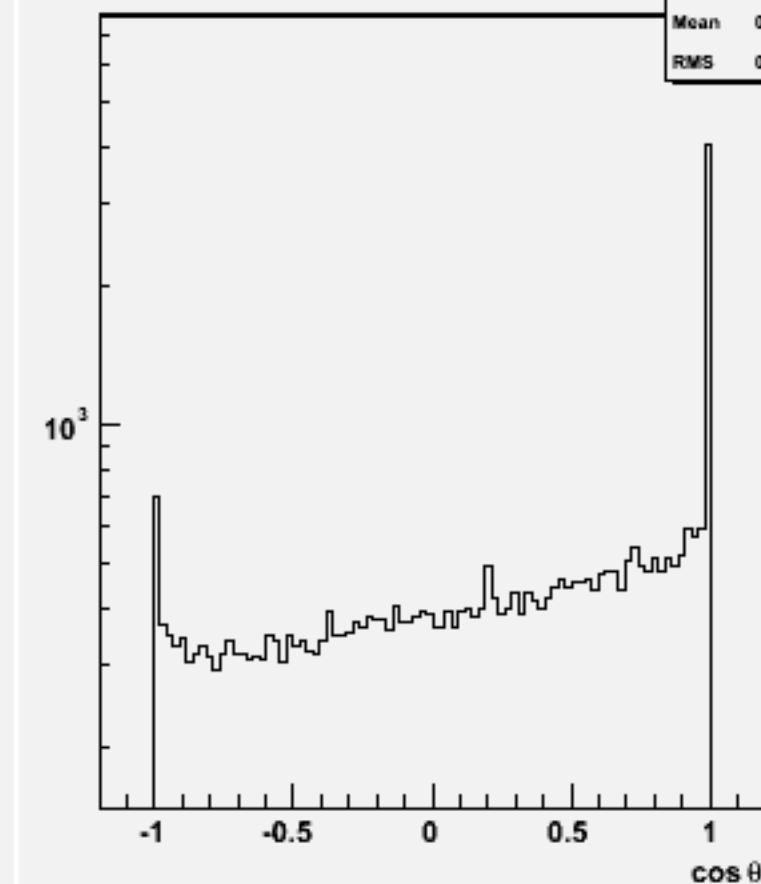
Jet cos \theta (All jets)w101433 n2n2n2e2sc_o
