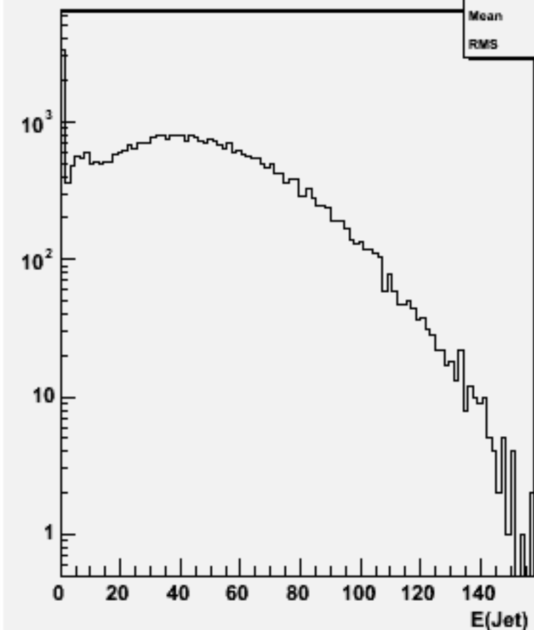
Jet energies(All jets)w101433 n2n2n2e2sc_o
