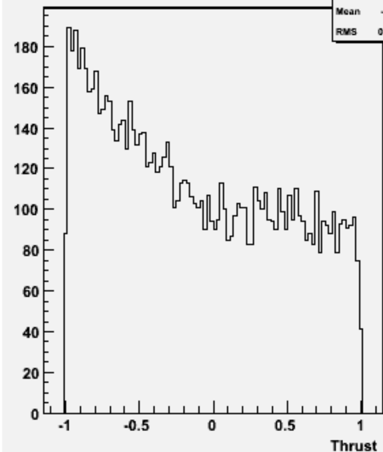
cos \Theta (thrust) w101433 n2n2n2e2sc_o
