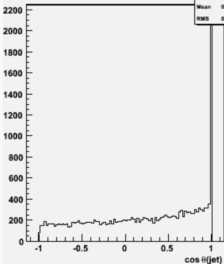
cos \theta for 2-jets :w101433 n2n2n2e2sc_o
