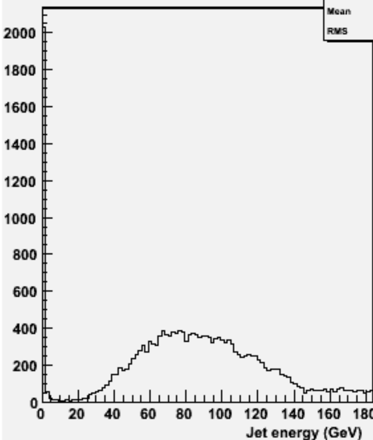
energy for 2-jets :w101433 n2n2n2e2sc_o
