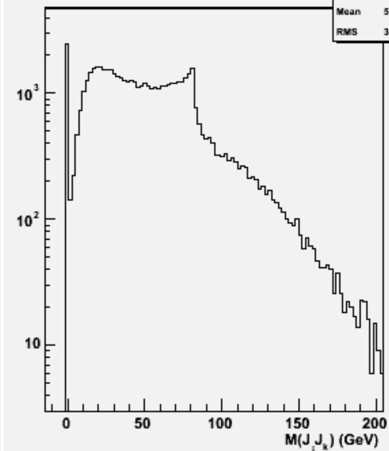
2jets mass(All comb)w101433 n2n2n2e2sc_o
