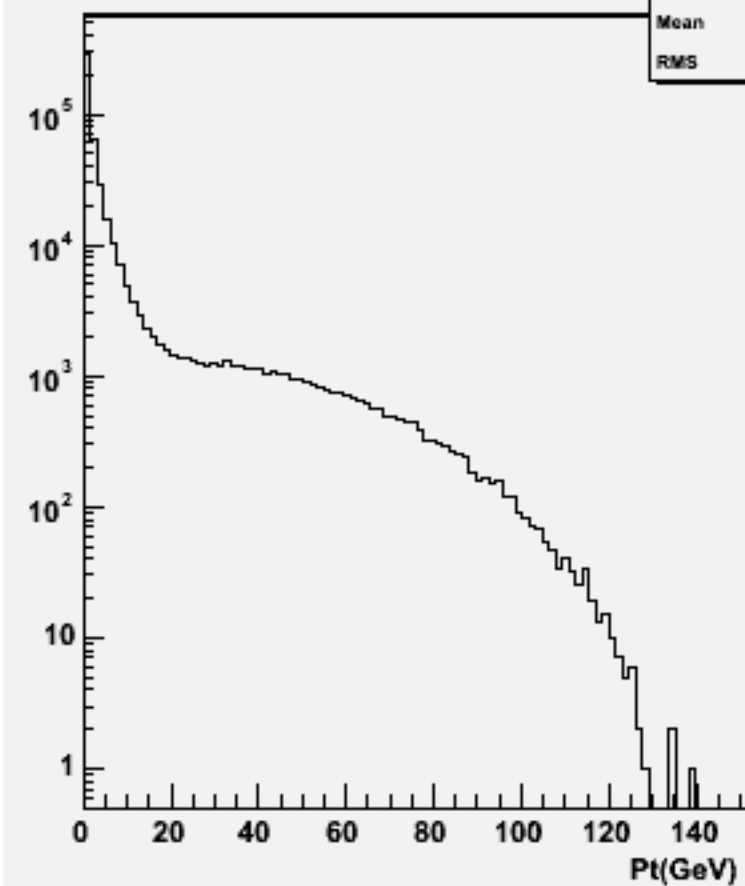
Start point Z : w101433 n2n2n2e2sc_o
