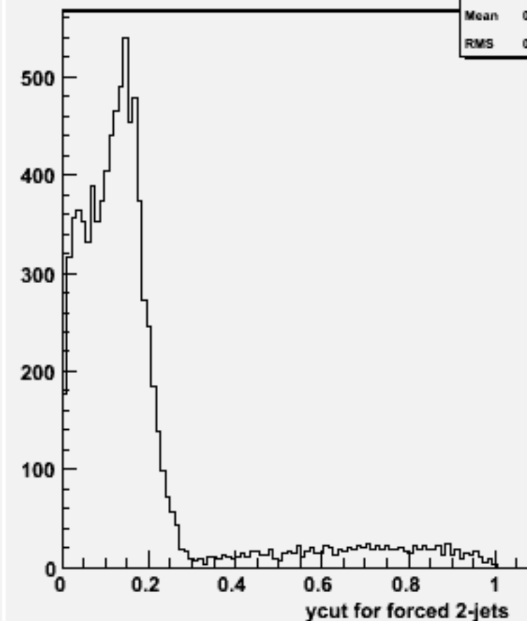
Ycut for 2-jets :w101433 n2n2n2e2sc_o
