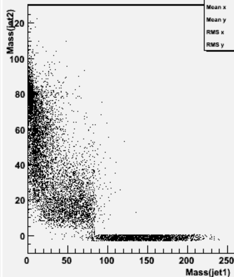
Jet mass for forced 2-jets : w101433 n2n2n2e2sc_o
