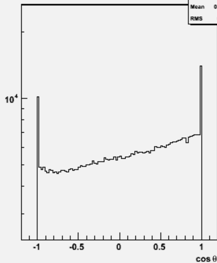
Particle cosθ : w101433 n2n2n2e2sc_o
