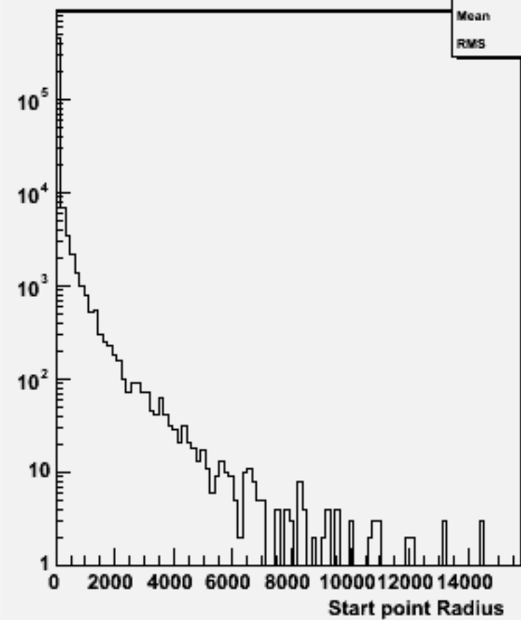
Start point R : w101433 n2n2n2e2sc_o
