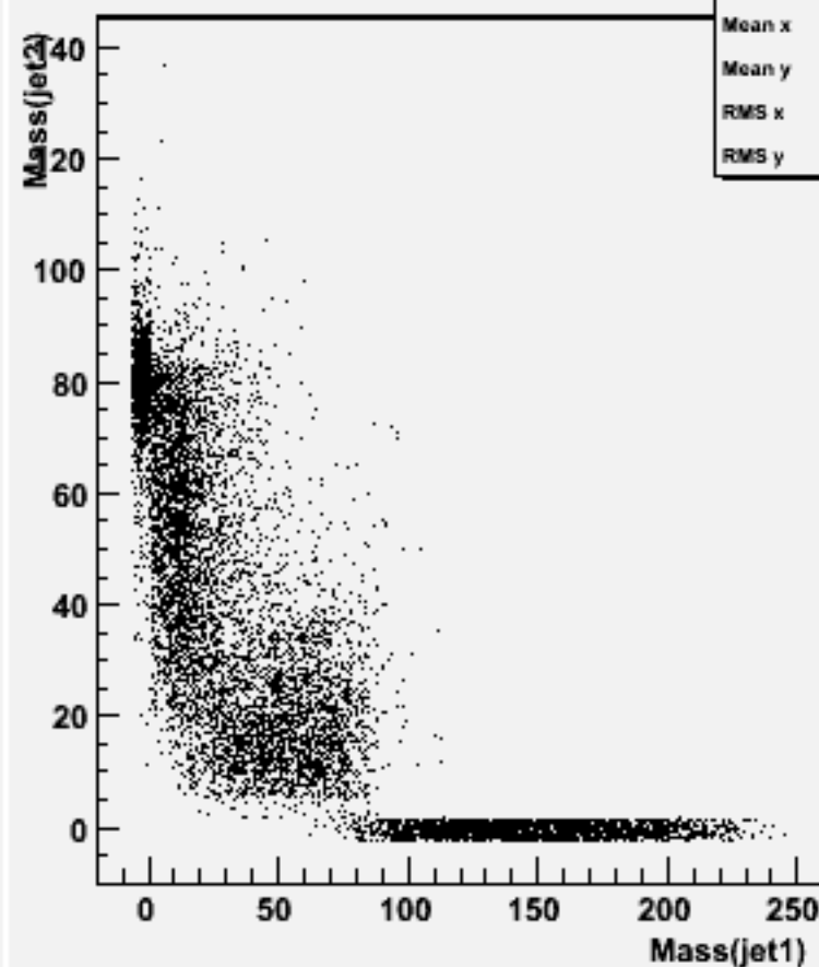
Jet mass for forced 2-jets : w101432 n2n2n2e2sc_o
