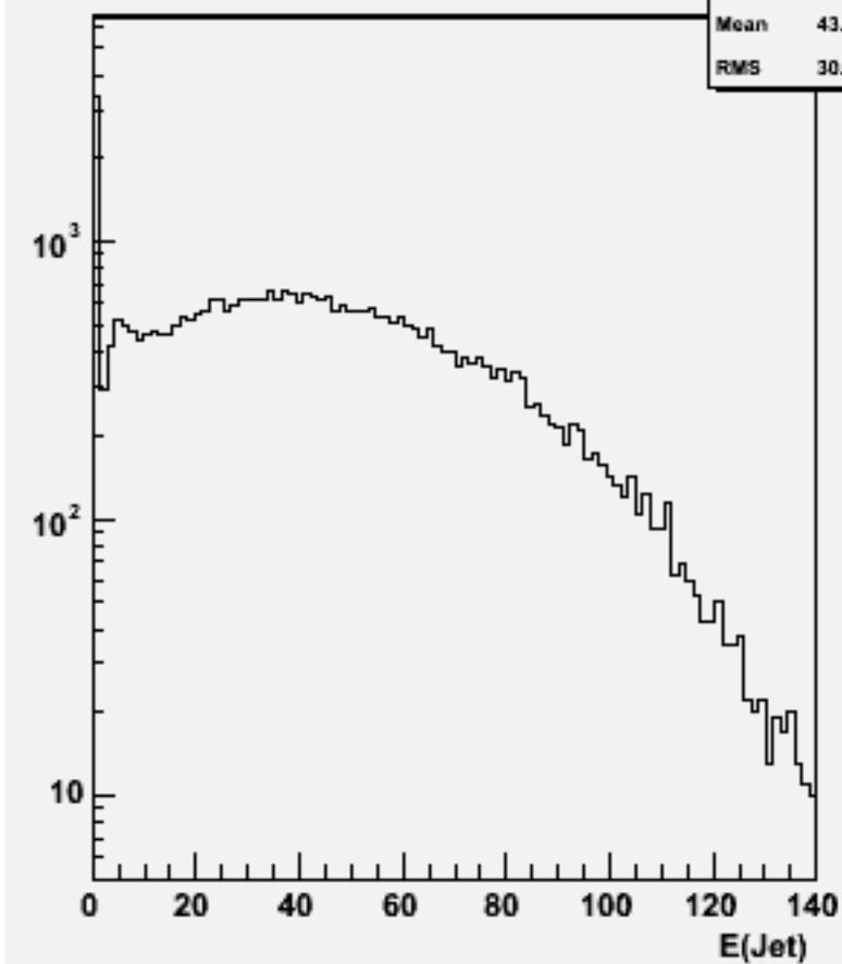
Jet energies(All jets)w101432 n2n2n2e2sc_o
