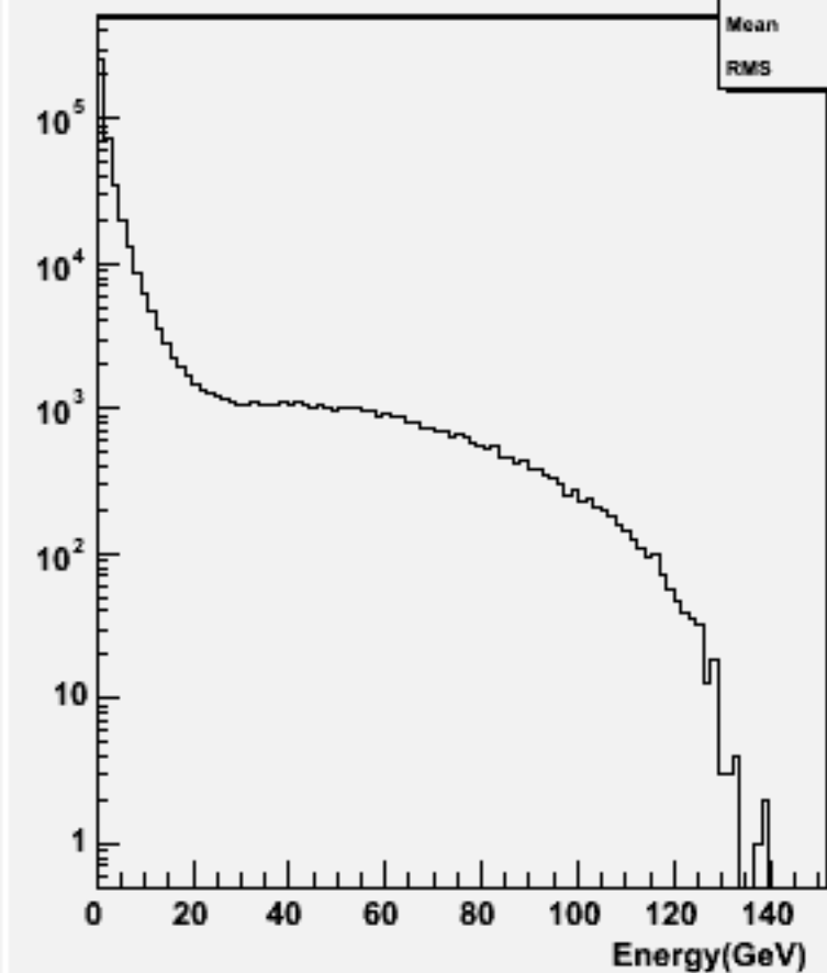
Start point R : w101432 n2n2n2e2sc_o
