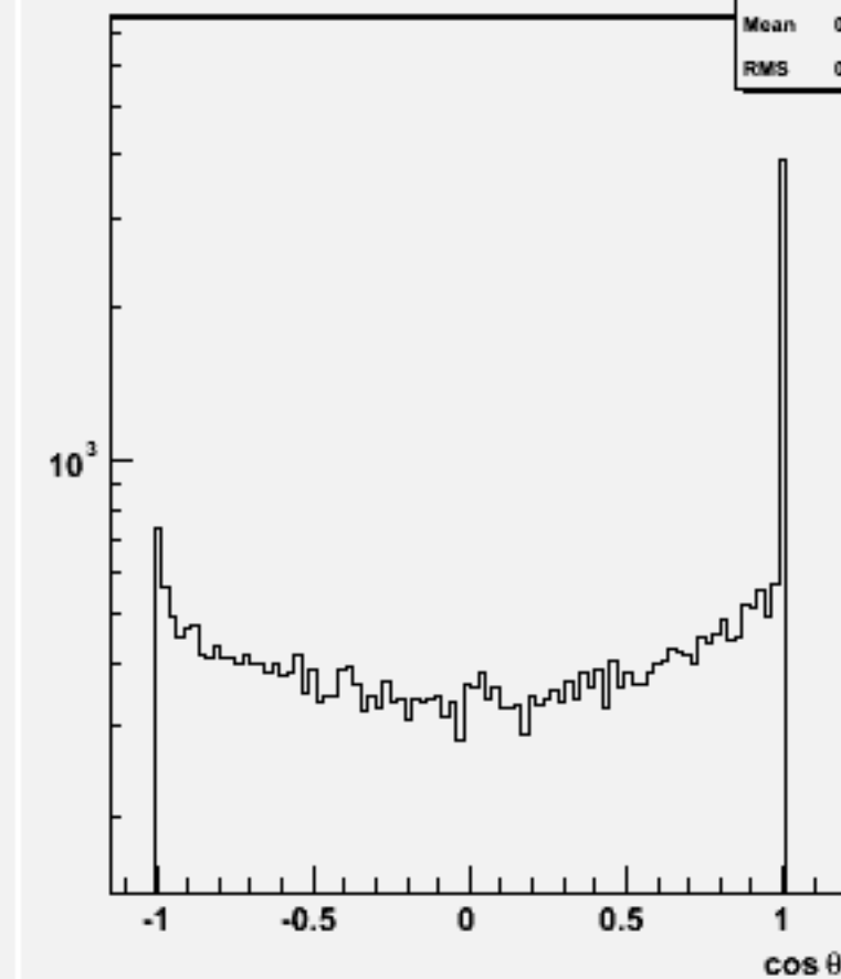
Jet cos \theta (All jets)w101432 n2n2n2e2sc_o
