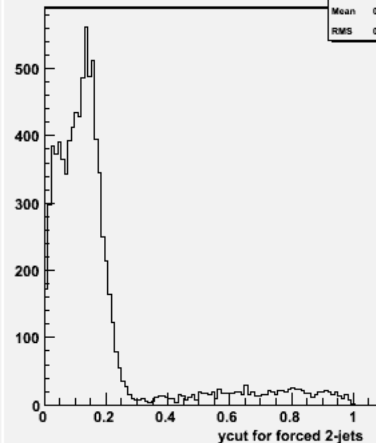
Ycut for 2-jets :w101432 n2n2n2e2sc_o
