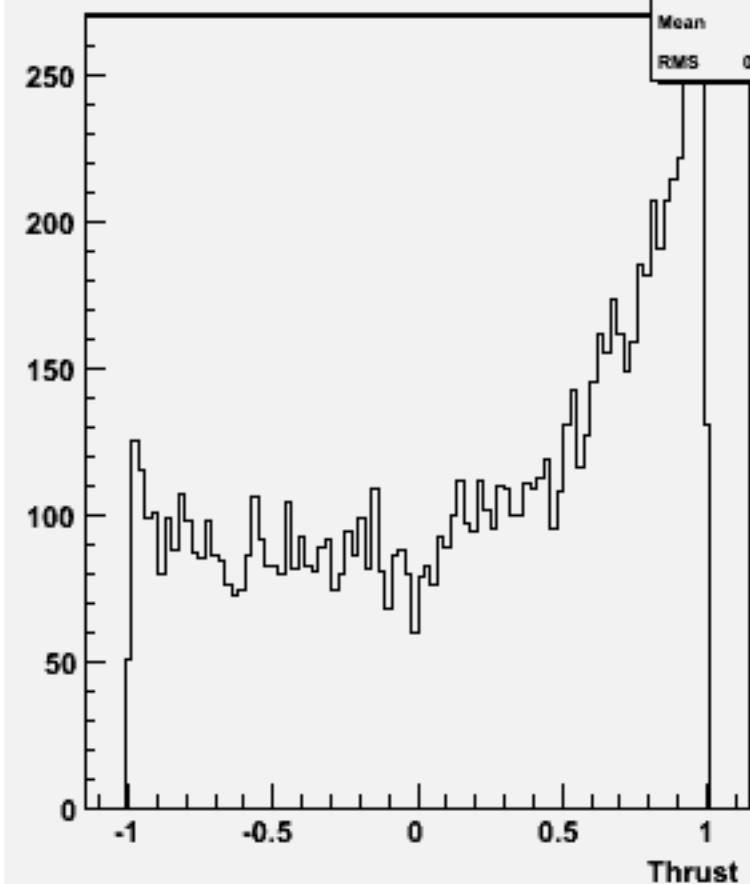
cos \Theta (thrust) w101432 n2n2n2e2sc_o
