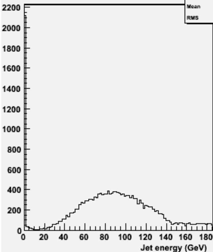
energy for 2-jets :w101432 n2n2n2e2sc_o
