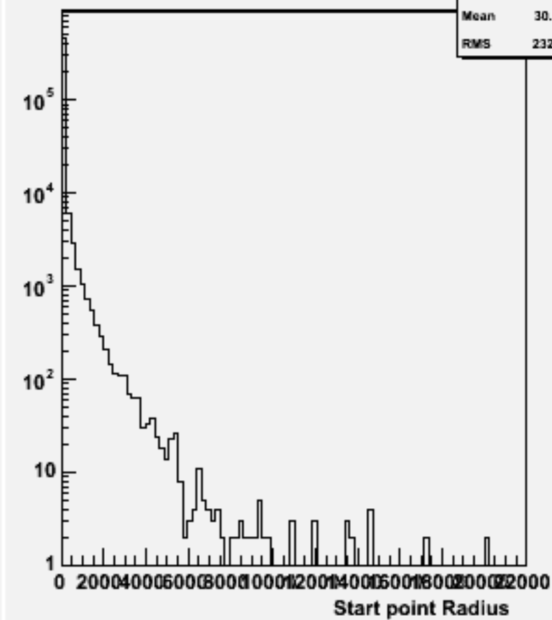
Start point R : w101432 n2n2n2e2sc_o
