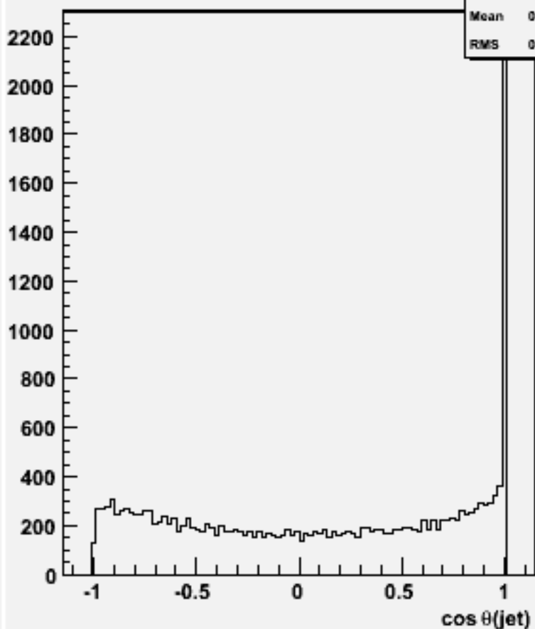
cos \theta for 2-jets :w101432 n2n2n2e2sc_o
