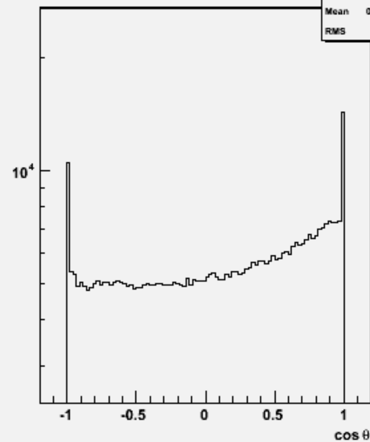
Particle cos \theta : w101432 n2n2n2e2sc_o
