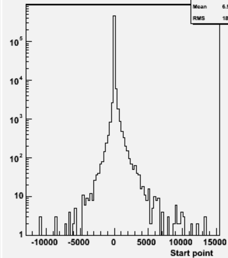
Start point Z : w101432 n2n2n2e2sc_o
