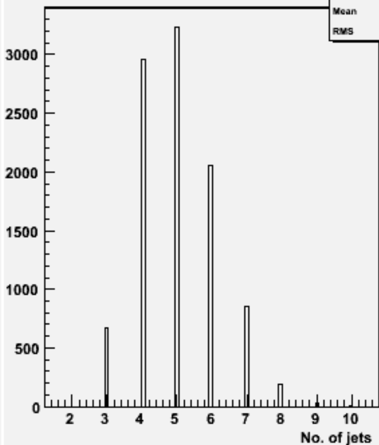
No. jets (ycut=0.001) : w101432 n2n2n2e2sc_o
