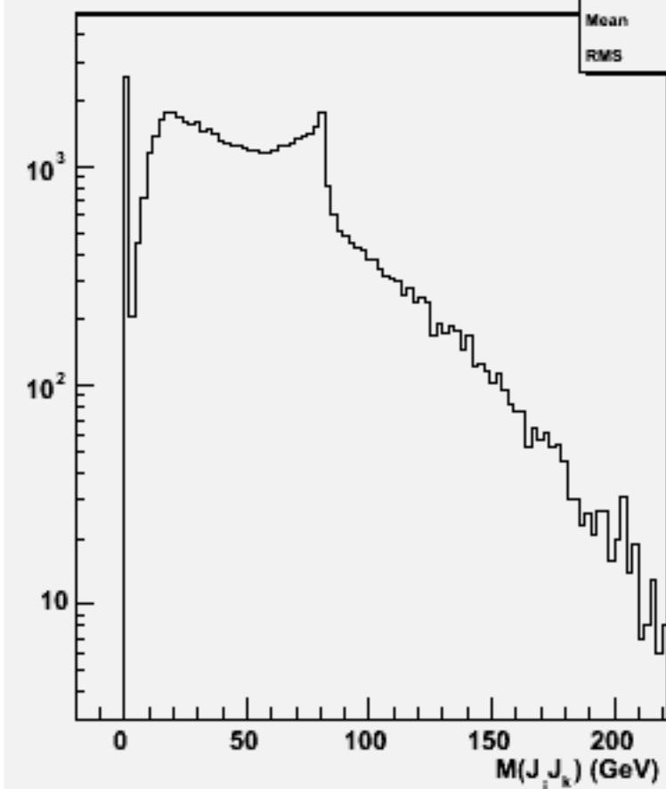
2jets mass(All comb)w101432 n2n2n2e2sc_o
