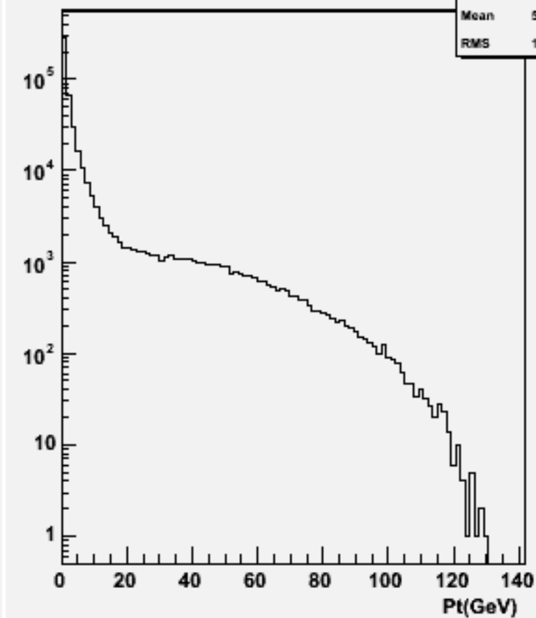
Start point Z : w101432 n2n2n2e2sc_o
