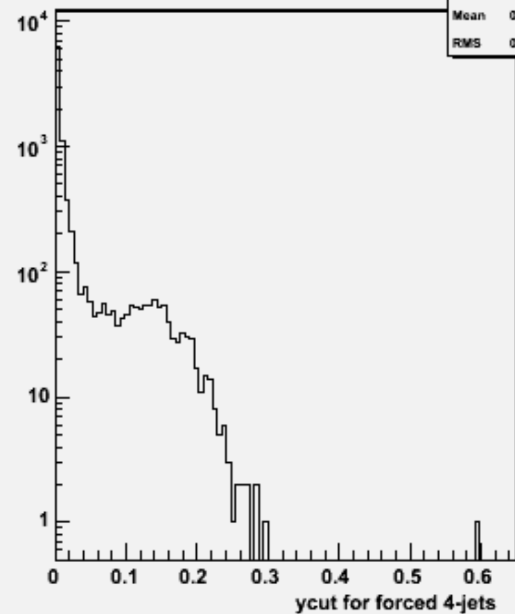
Ycut for 4-jets :w101432 n2n2n2e2sc_o
