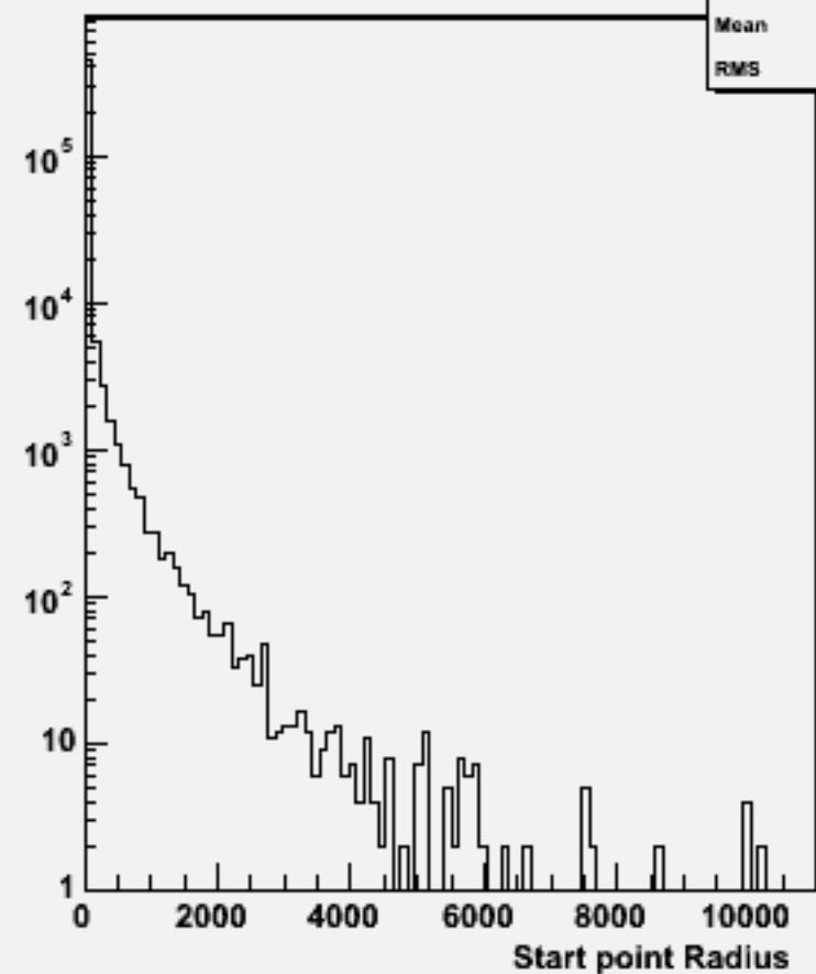
Start point R : w101429 n2n2n2e2du_o
