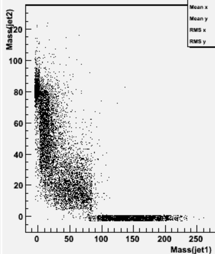
Jet mass for forced 2-jets : w101429 n2n2n2e2du_o
