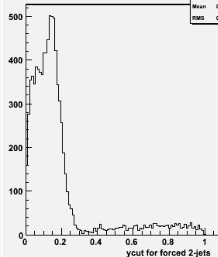
Ycut for 2-jets :w101429 n2n2n2e2du_o
