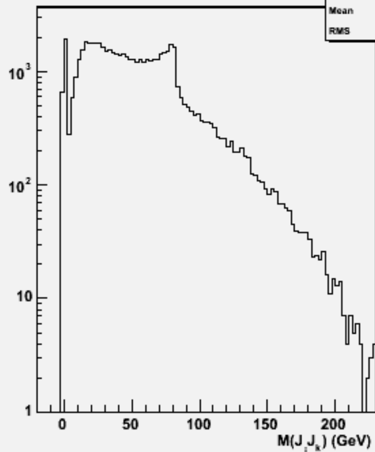
2jets mass(All comb)w101429 n2n2n2e2du_o
