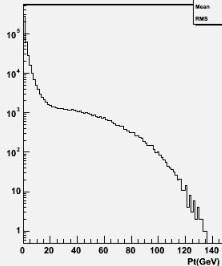
Start point Z : w101429 n2n2n2e2du_o
