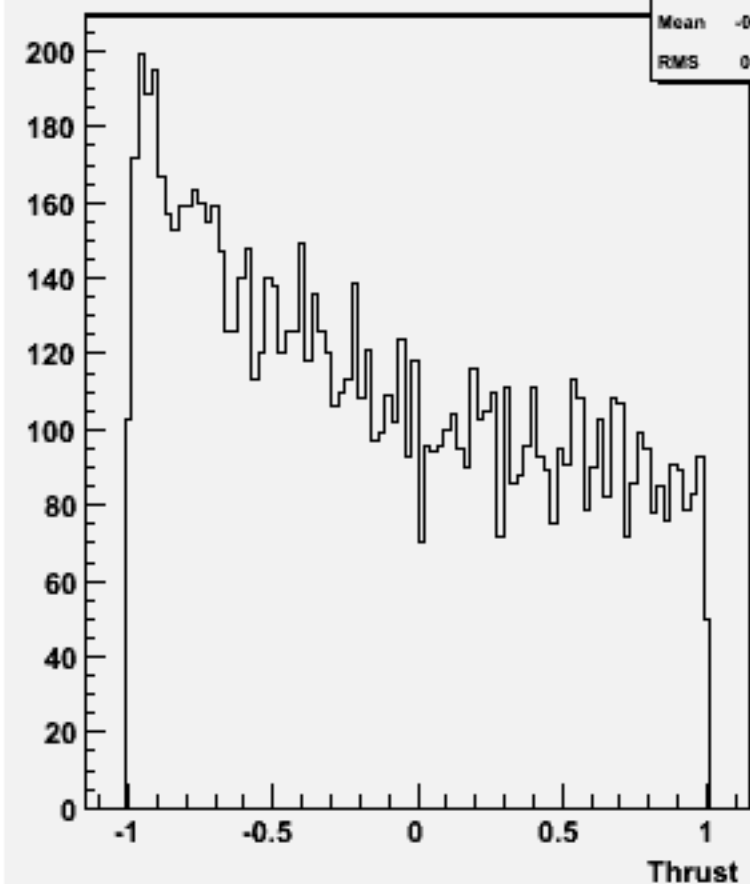
cos \Theta (thrust) w101429 n2n2n2e2du_o
