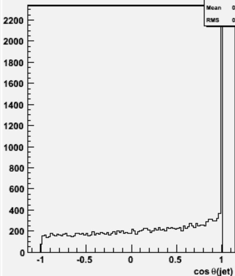
cos \theta for 2-jets :w101429 n2n2n2e2du_o
