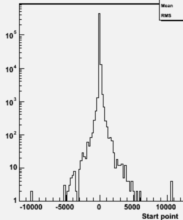
Start point Z : w101429 n2n2n2e2du_o
