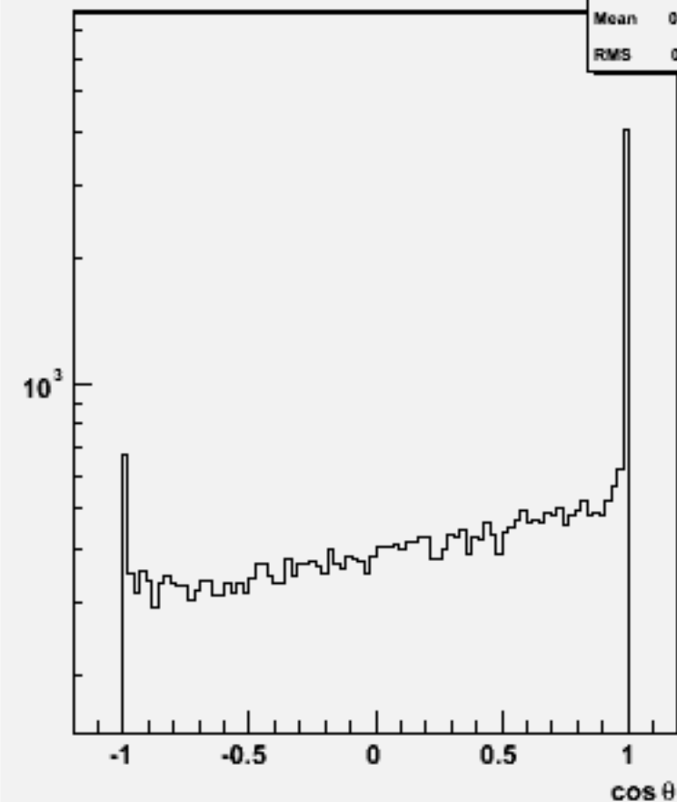
Jet cos \theta (All jets)w101429 n2n2n2e2du_o
