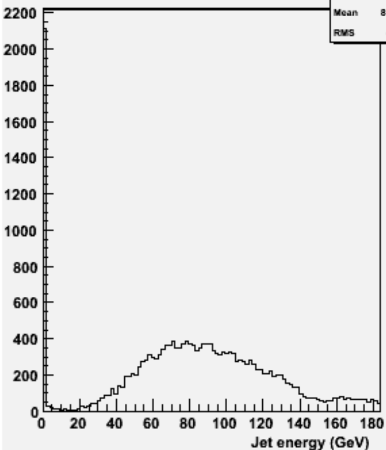
energy for 2-jets :w101429 n2n2n2e2du_o
