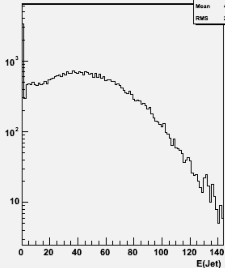
Jet energies(All jets)w101429 n2n2n2e2du_o
