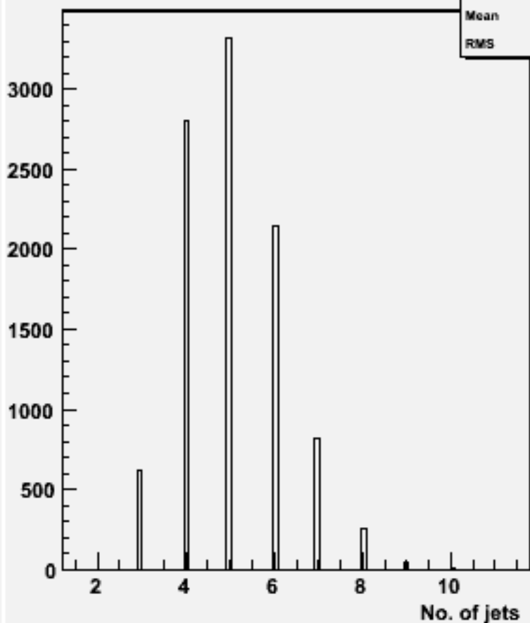
No. jets (ycut=0.001) : w101429 n2n2n2e2du_o
