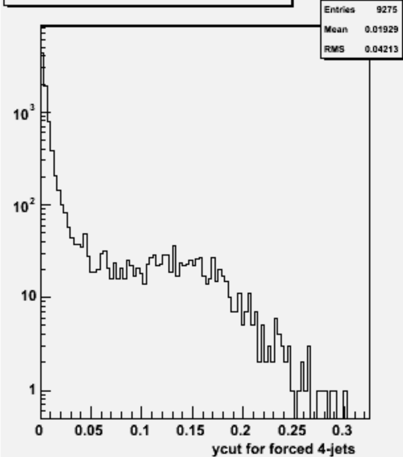
Ycut for 4-jets :w101428 n2n2n2e2du_o
