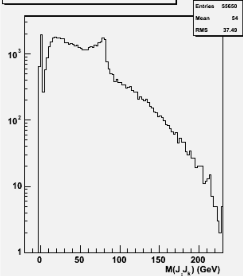
2jets mass(All comb)w101428 n2n2n2e2du_o
