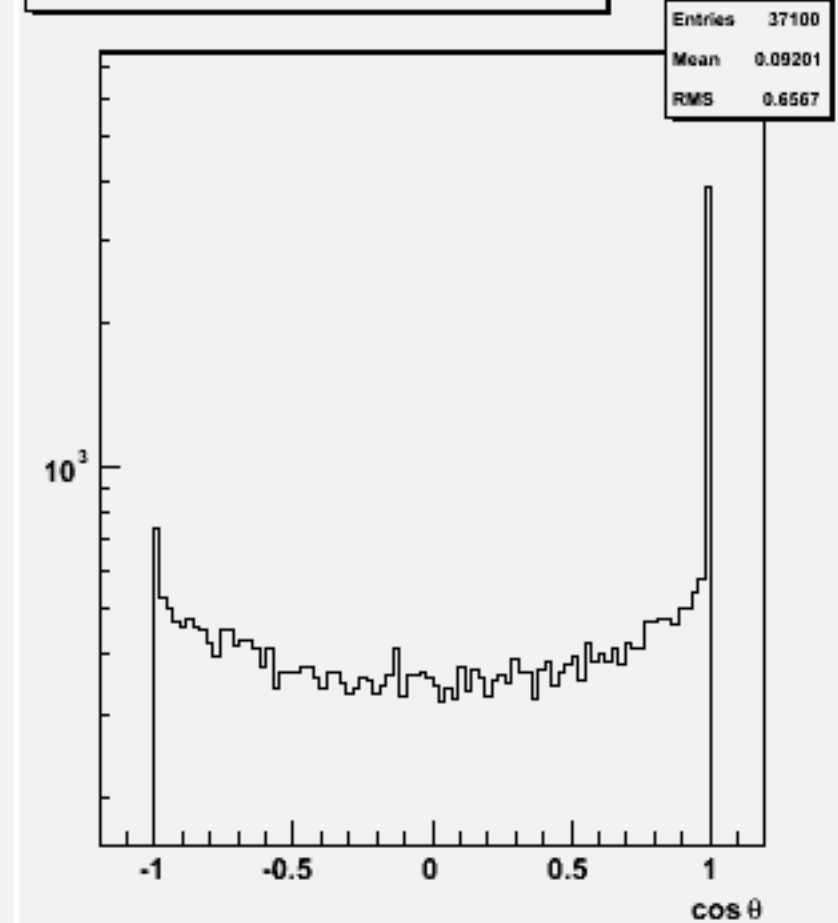
Jet cos \theta (All jets)w101428 n2n2n2e2du_o
