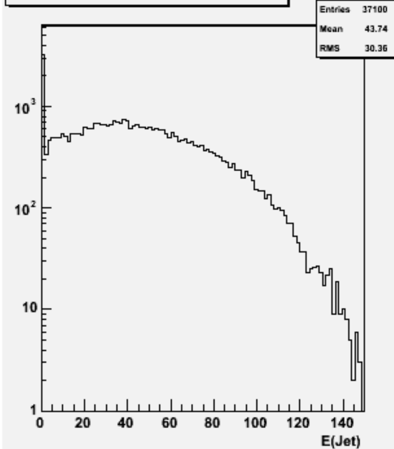
Jet energies(All jets)w101428 n2n2n2e2du_o
