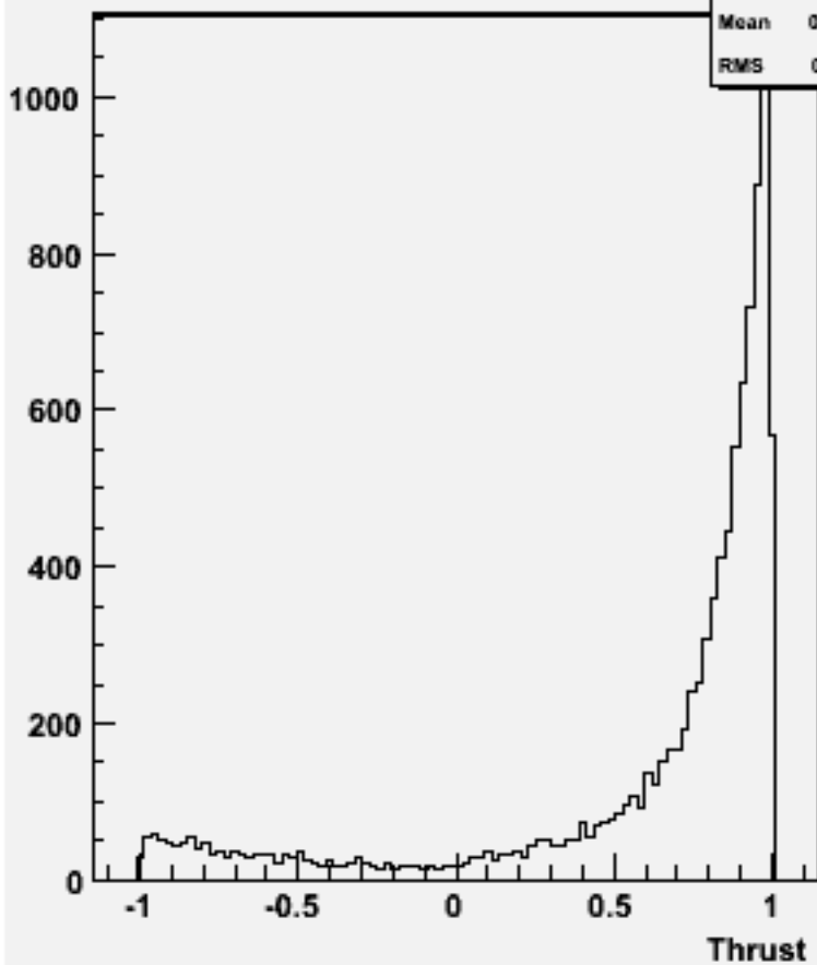
cos \Theta (thrust) w101412 n2n2n1e1sc_o
