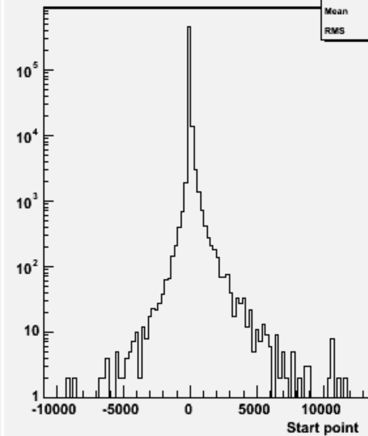
Start point Z : w101412 n2n2n1e1sc_o
