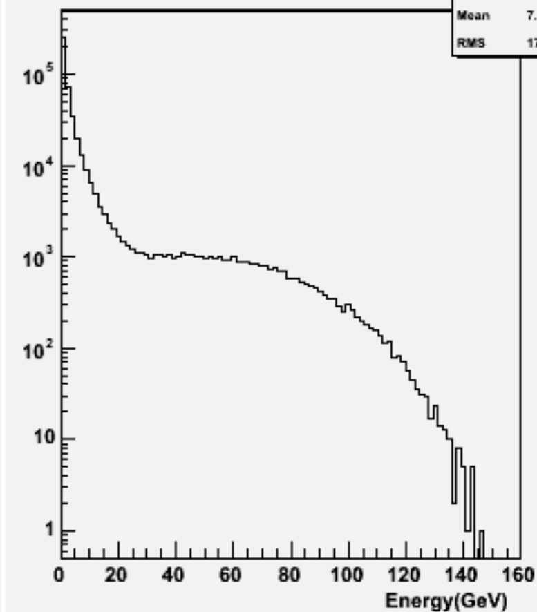
Start point R : w101412 n2n2n1e1sc_o
