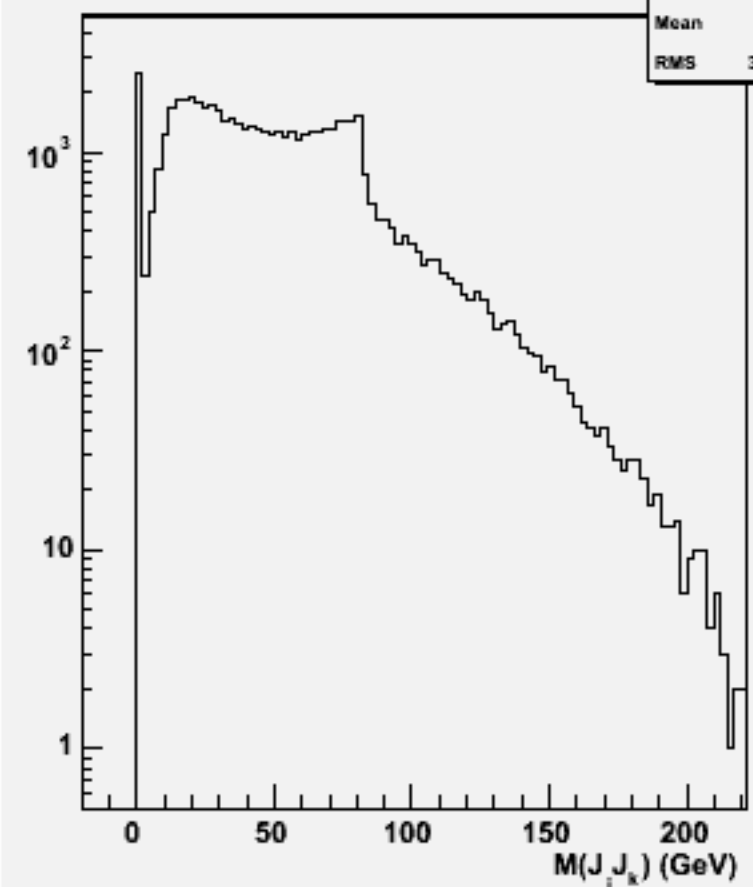
2jets mass(All comb)w101412 n2n2n1e1sc_o
