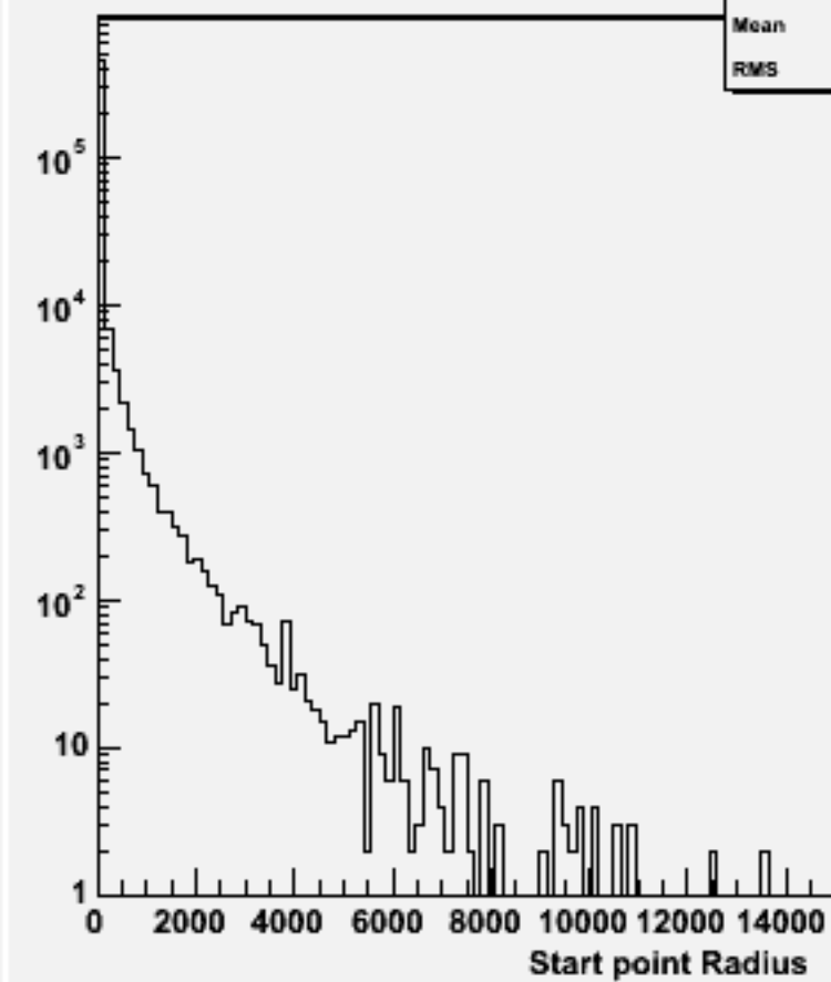
Start point R : w101412 n2n2n1e1sc_o
