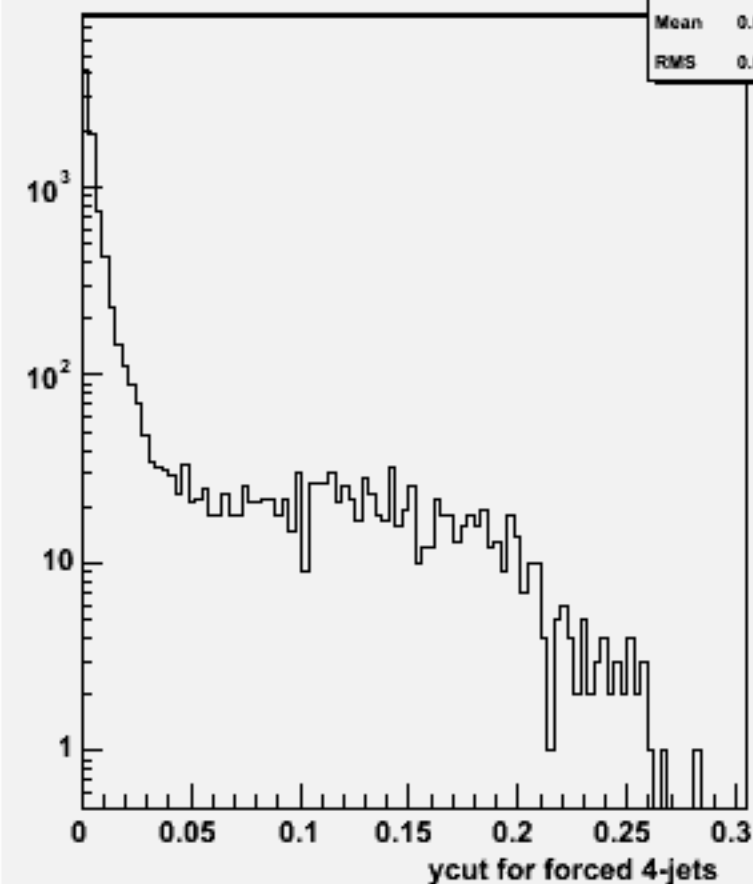
Ycut for 4-jets :w101412 n2n2n1e1sc_o
