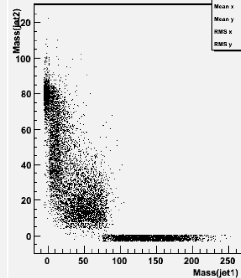
Jet mass for forced 2-jets : w101412 n2n2n1e1sc_o
