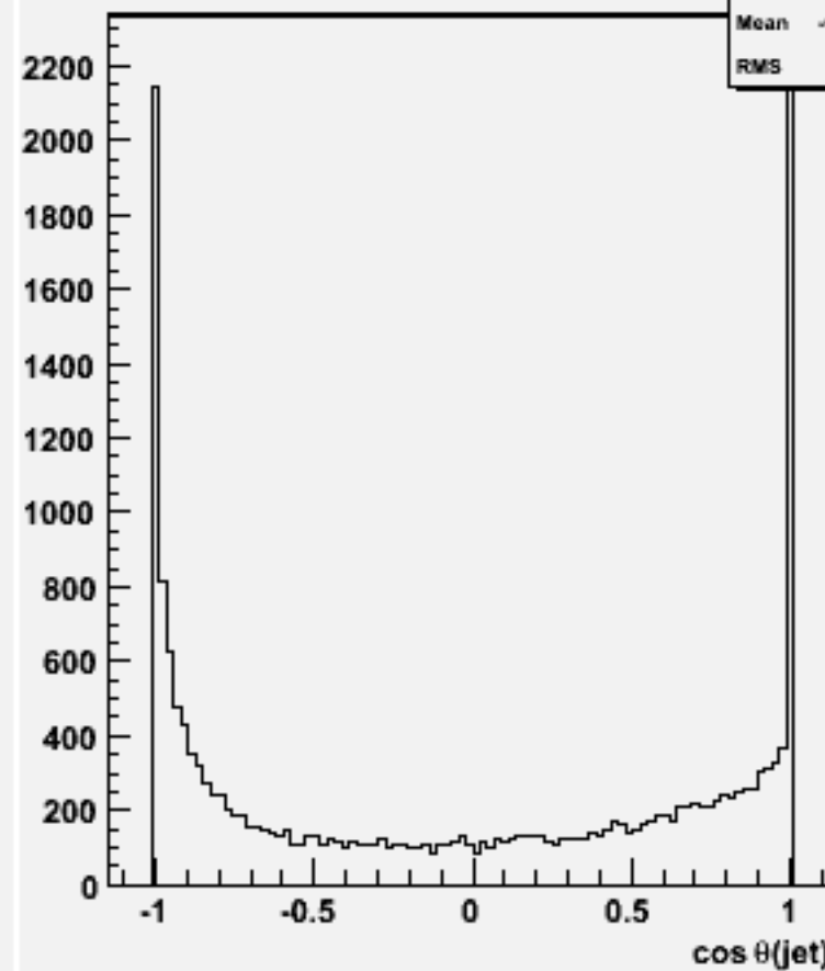
cos \theta for 2-jets :w101412 n2n2n1e1sc_o
