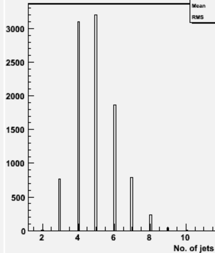
No. jets (ycut=0.001) : w101412 n2n2n1e1sc_o
