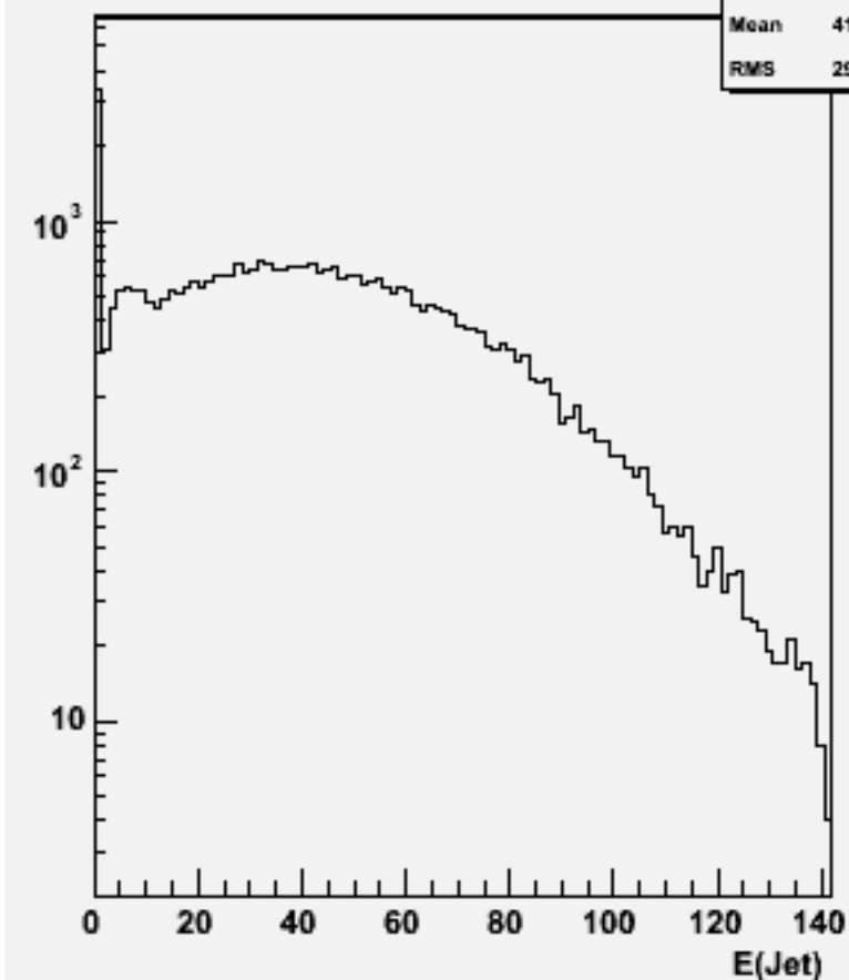
Jet energies(All jets)w101412 n2n2n1e1sc_o
