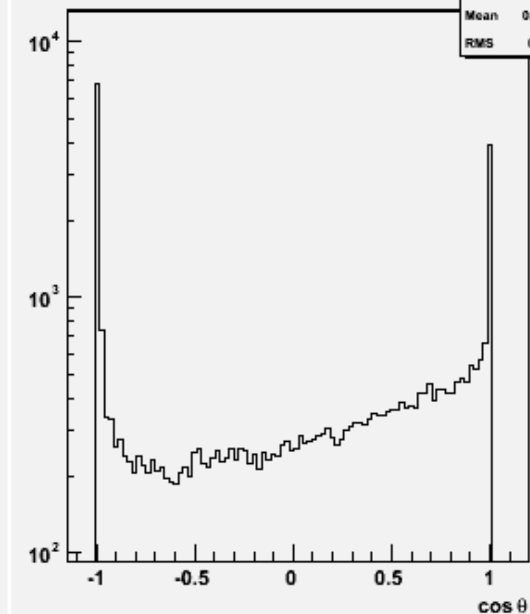
Jet cos \theta (All jets)w101412 n2n2n1e1sc_o
