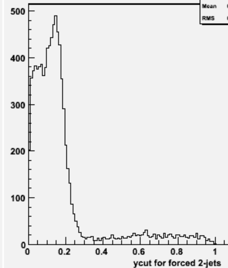
Ycut for 2-jets :w101412 n2n2n1e1sc_o
