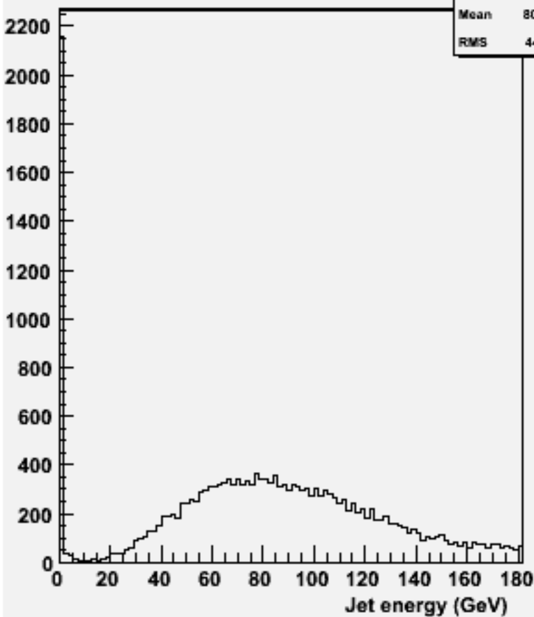
energy for 2-jets :w101412 n2n2n1e1sc_o
