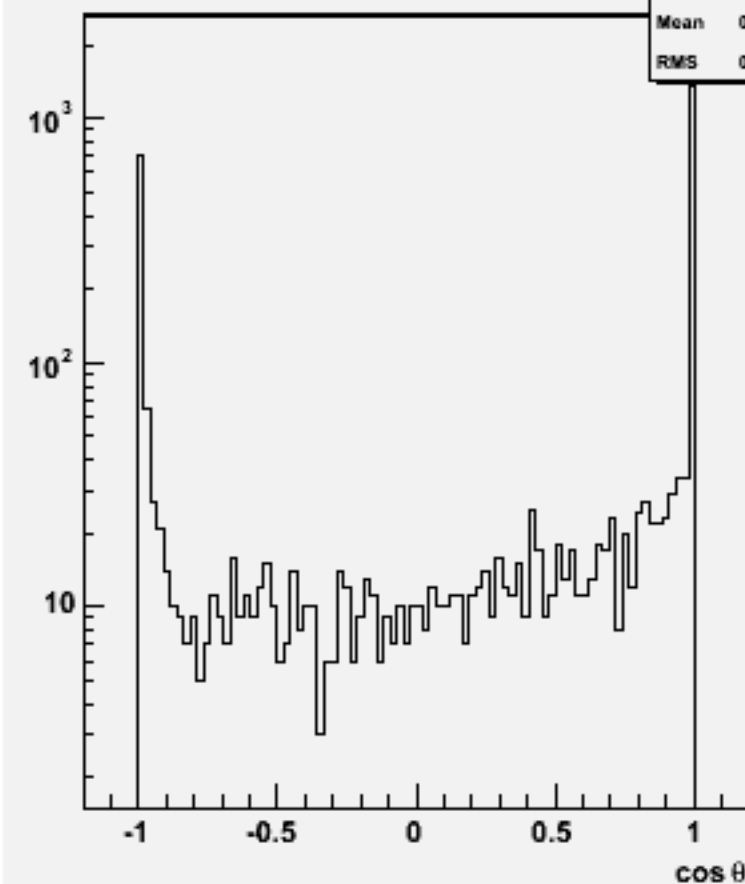
Jet cos \theta (All jets)w101404 n2n2n1e1e3n3_o
