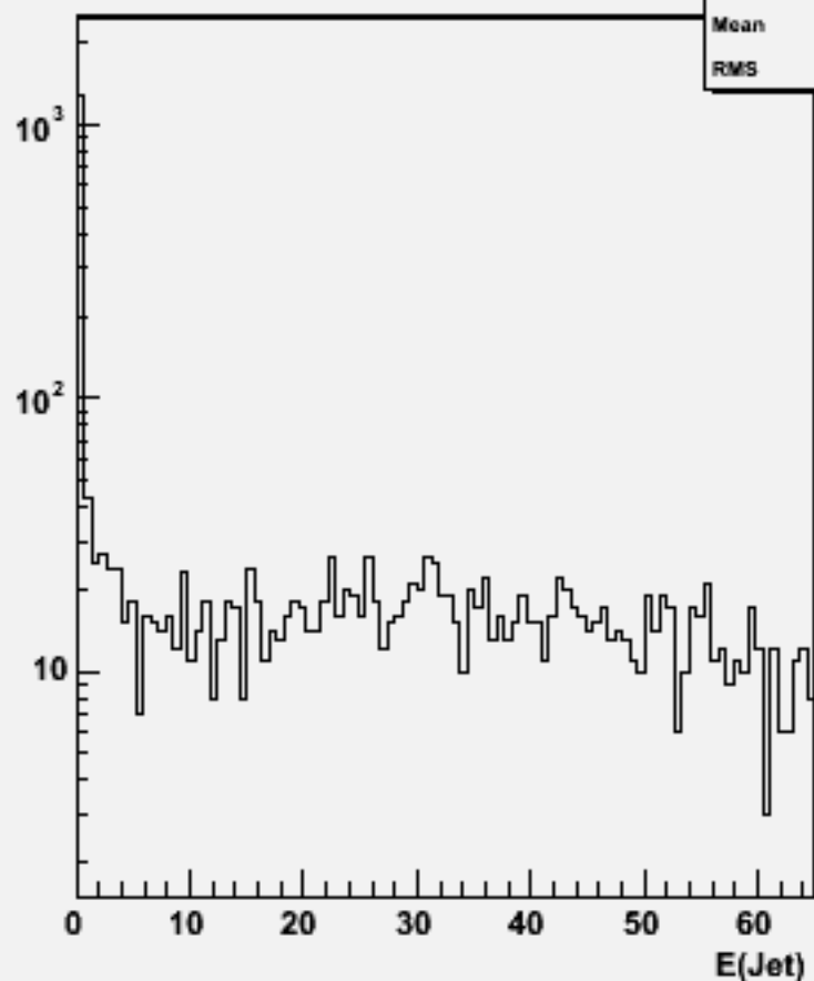
Jet energies(All jets)w101404 n2n2n1e1e3n3_o
