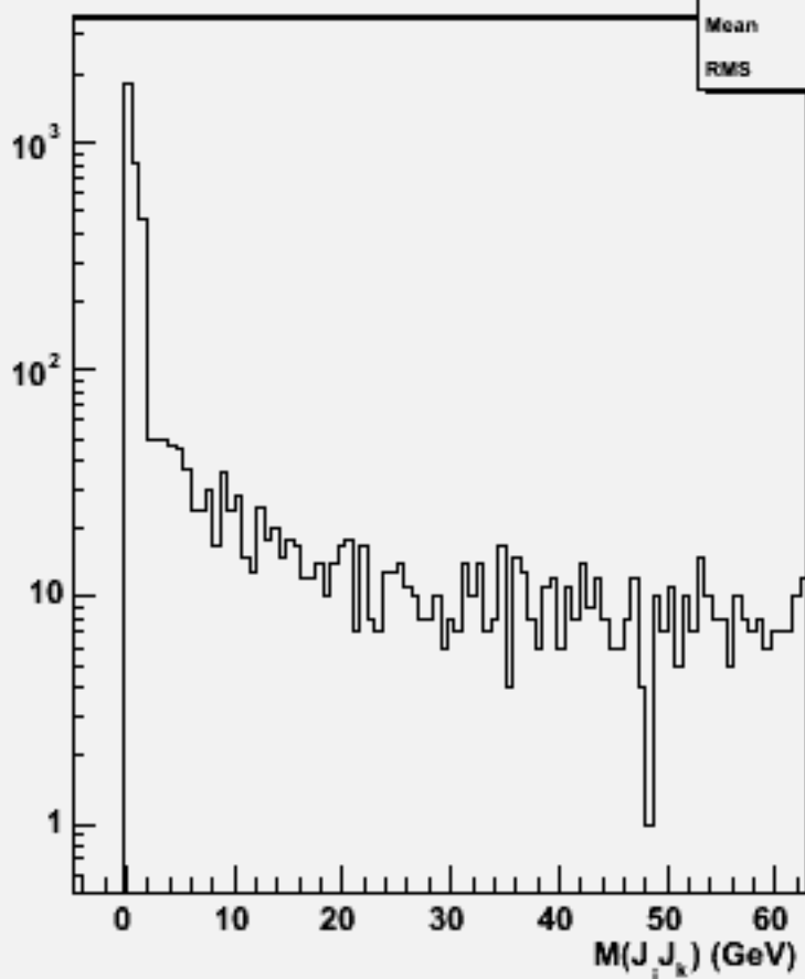
2jets mass(All comb)w101404 n2n2n1e1e3n3_o
