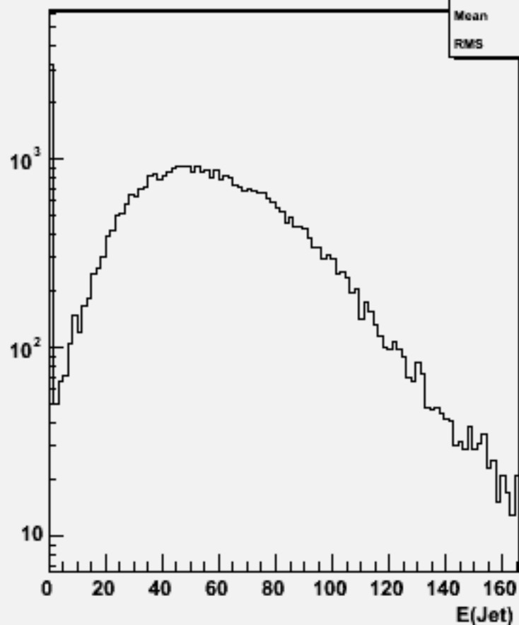
Jet energies(All jets)w101393 n1n1cssc_o
