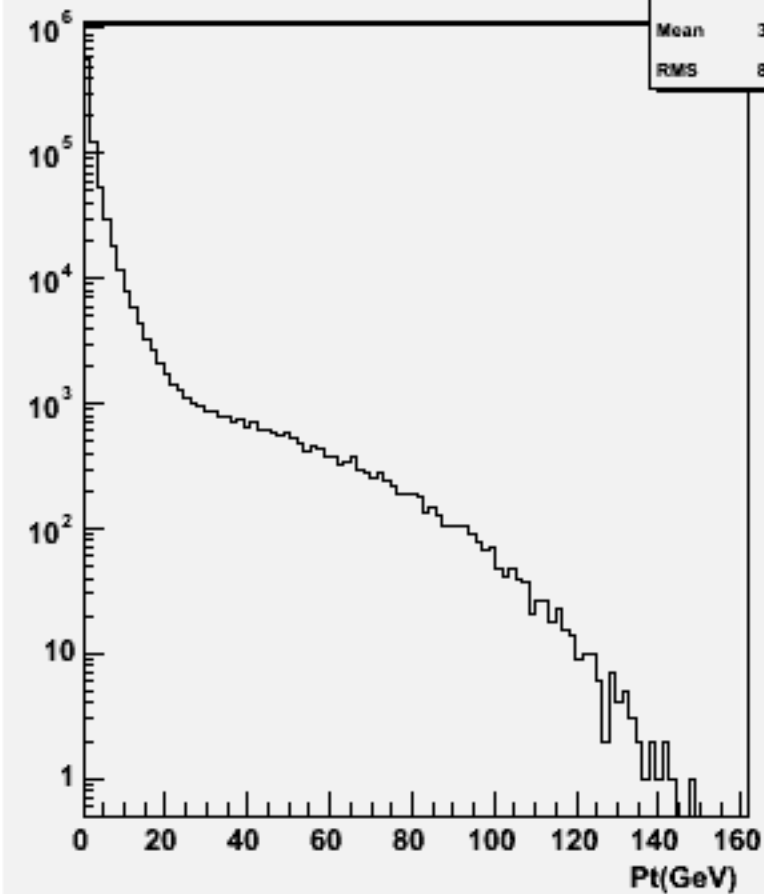
Particle Pt : w101393 n1n1cssc_o
