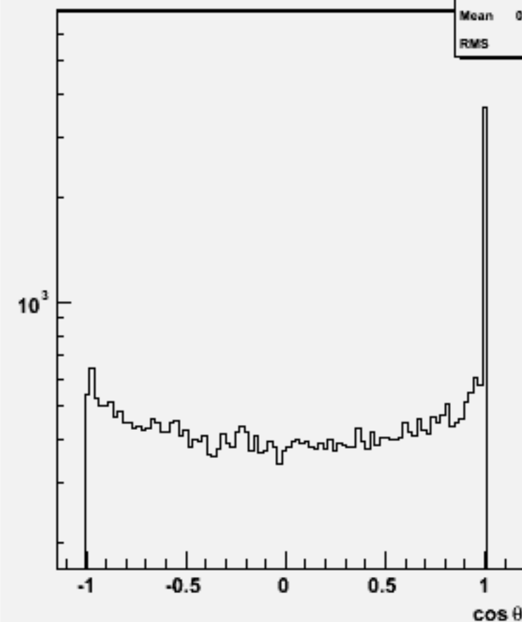
Jet cosθ (All jets)w101393 n1n1cssc_o
