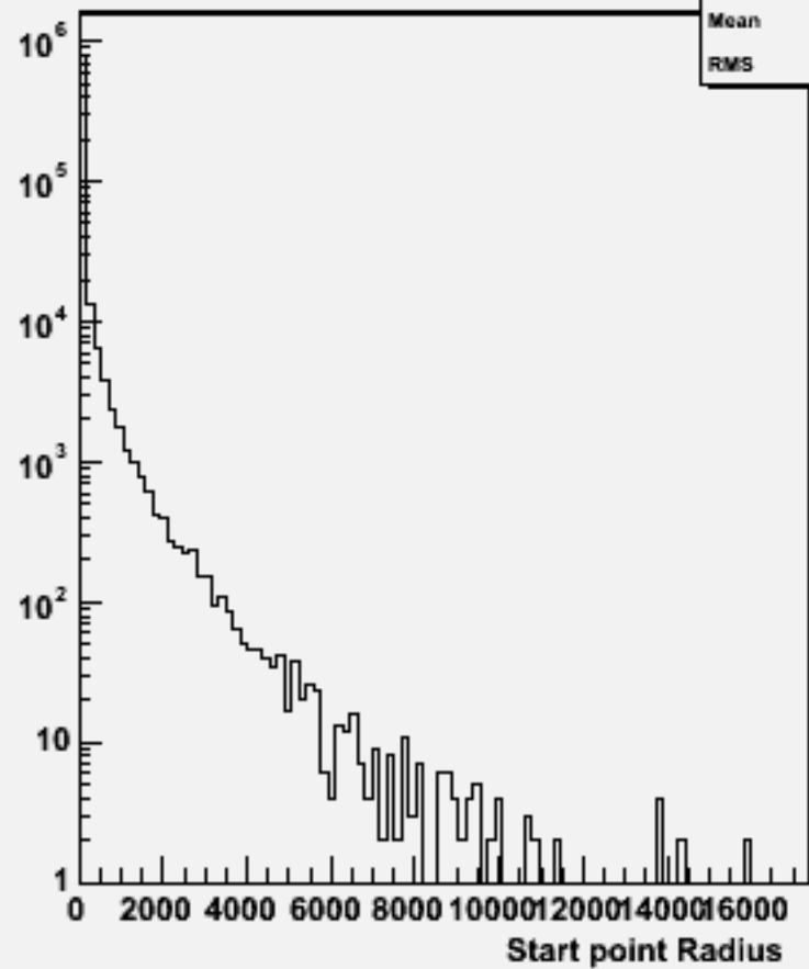
Start point R : w101393 n1n1cssc_o
