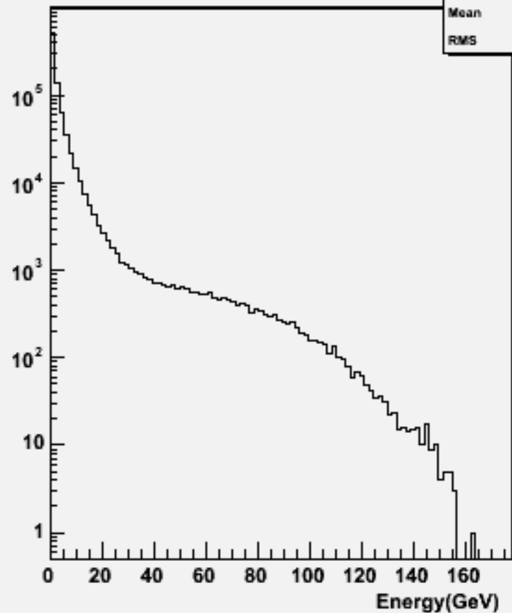
Start point R : w101393 n1n1cssc_o
