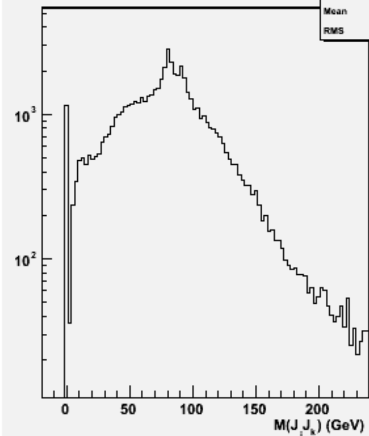
2jets mass(All comb)w101393 n1n1cssc_o
