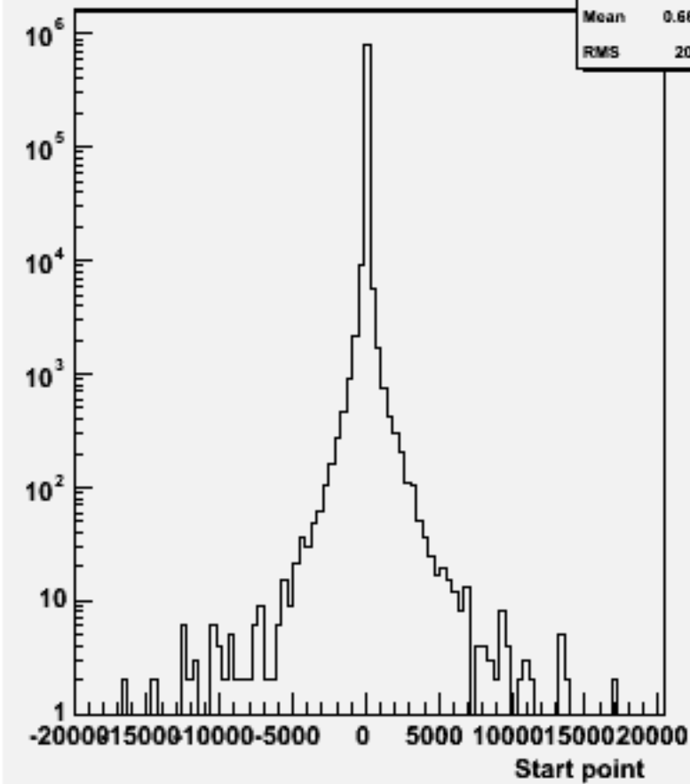
Start point Z : w101393 n1n1cssc_o
