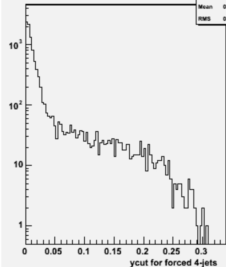
Ycut for 4-jets :w101393 n1n1cssc_o
