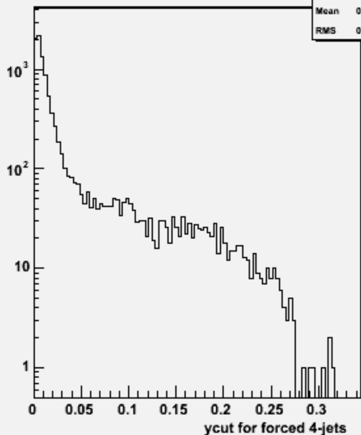
Ycut for 4-jets :w101389 n1n1csdu_o
