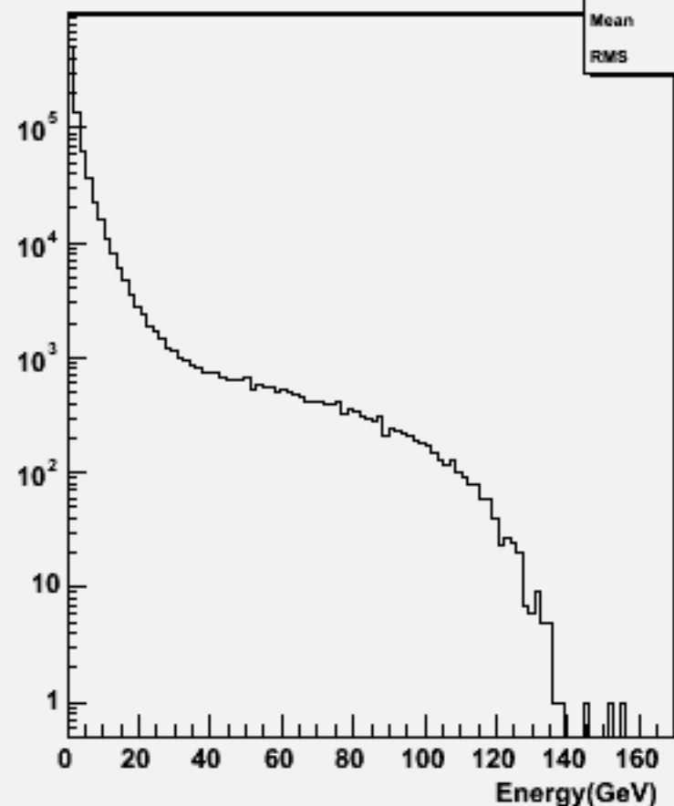
Particle Energy : w101389 n1n1csdu_o
