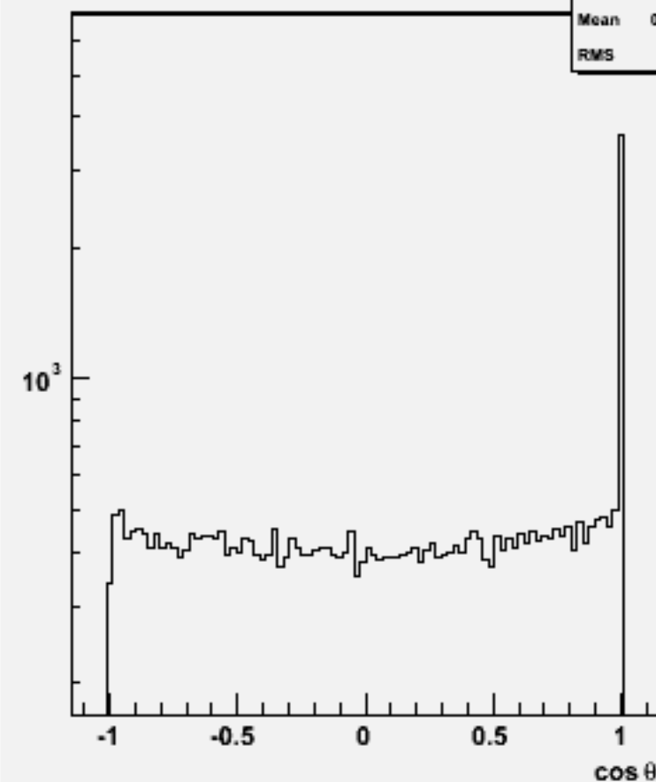
Jet cosθ (All jets)w101389 n1n1csdu_o
