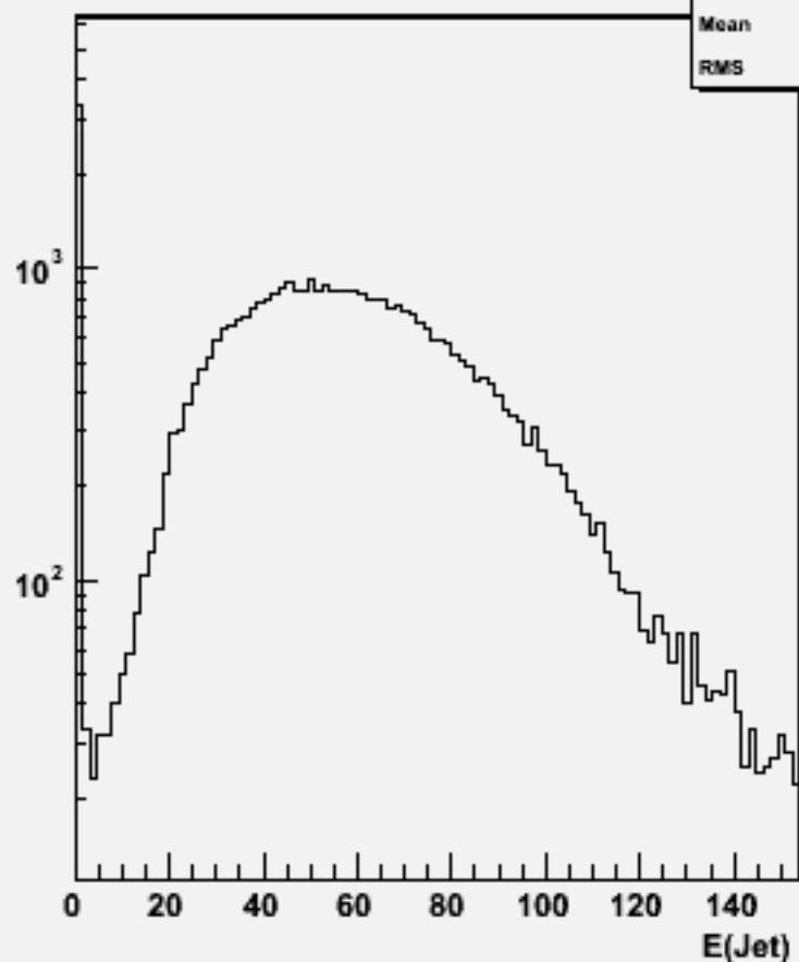
Jet energies(All jets)w101389 n1n1csdu_o
