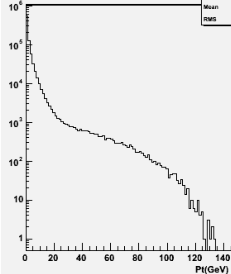
Particle Pt : w101389 n1n1csdu_o
