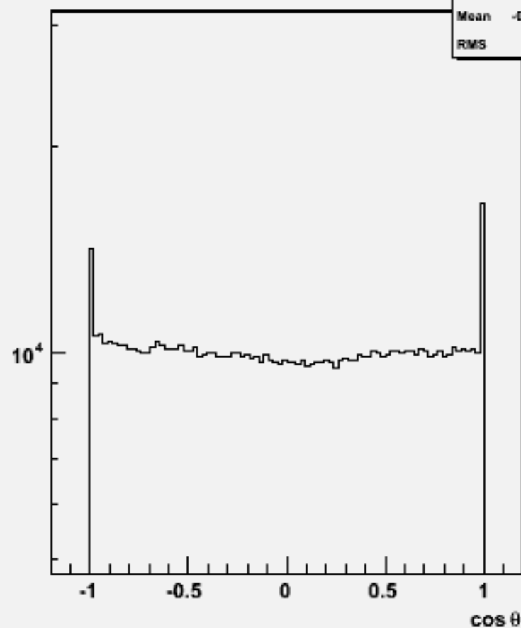
Particle cos \theta : w101389 n1n1csdu_o
