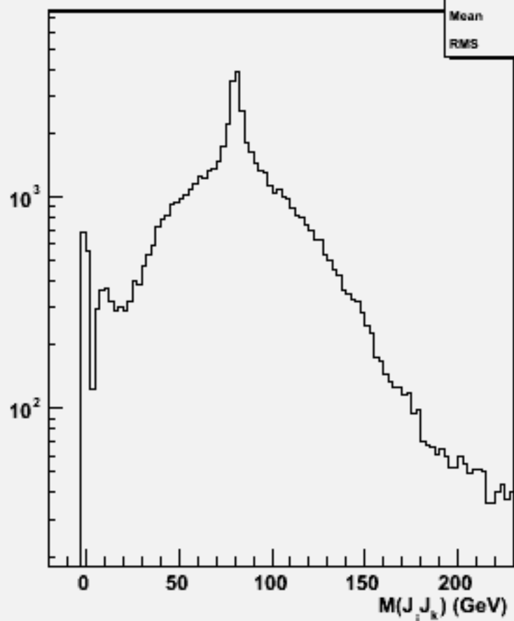
2jets mass(All comb)w101389 n1n1csdu_o
