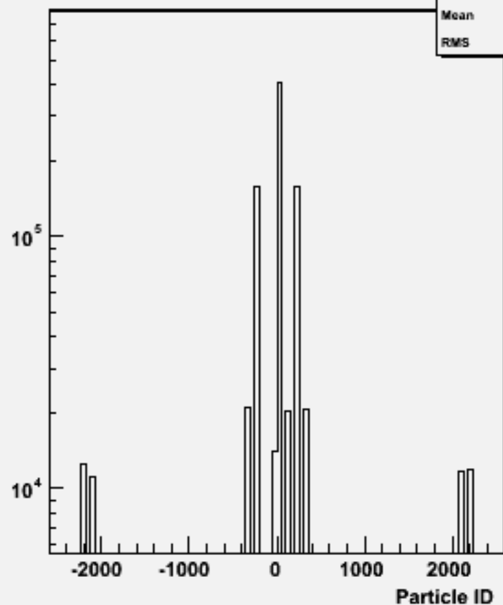
Particle ID : w101389 n1n1csdu_o
