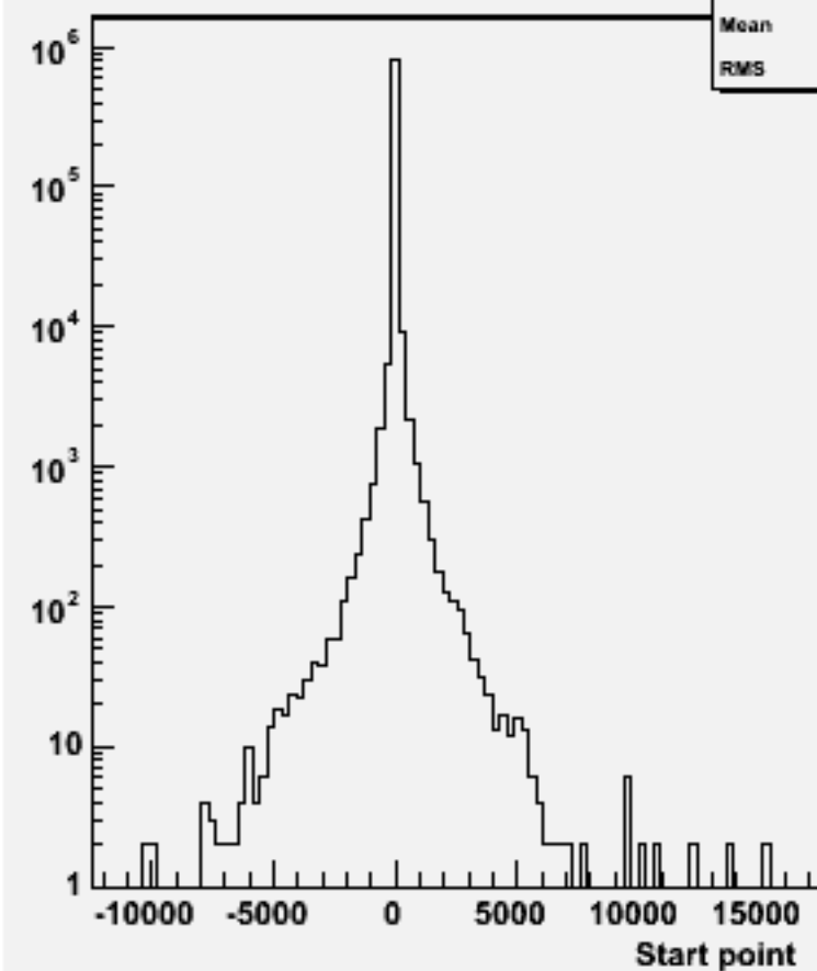
Start point Z : w101389 n1n1csdu_o
