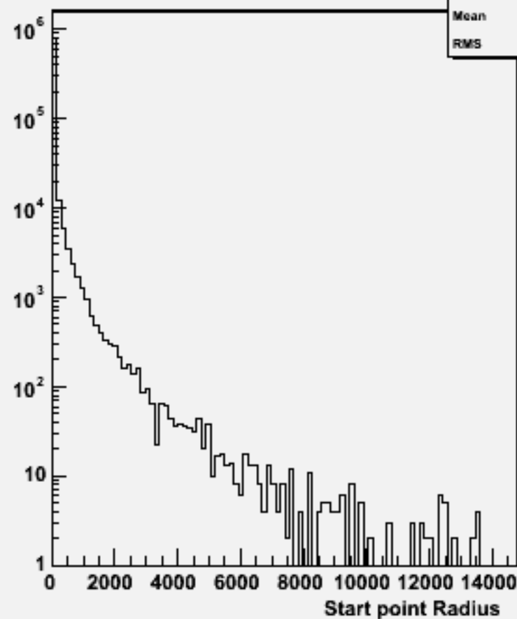
Start point R : w101389 n1n1csdu_o
