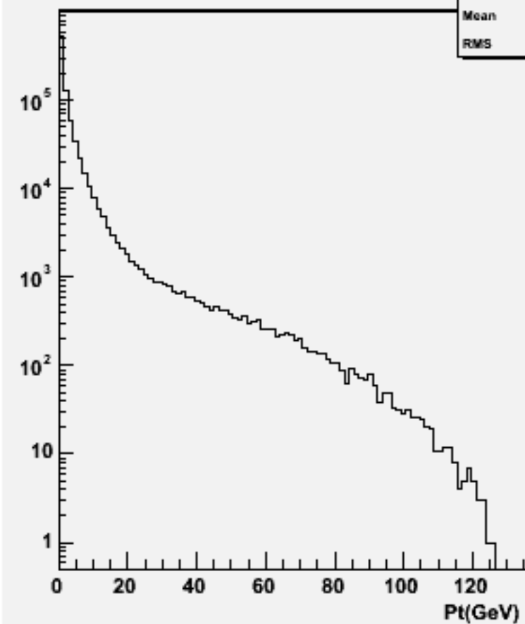
Particle Pt : w101388 n1n1csdu_o
