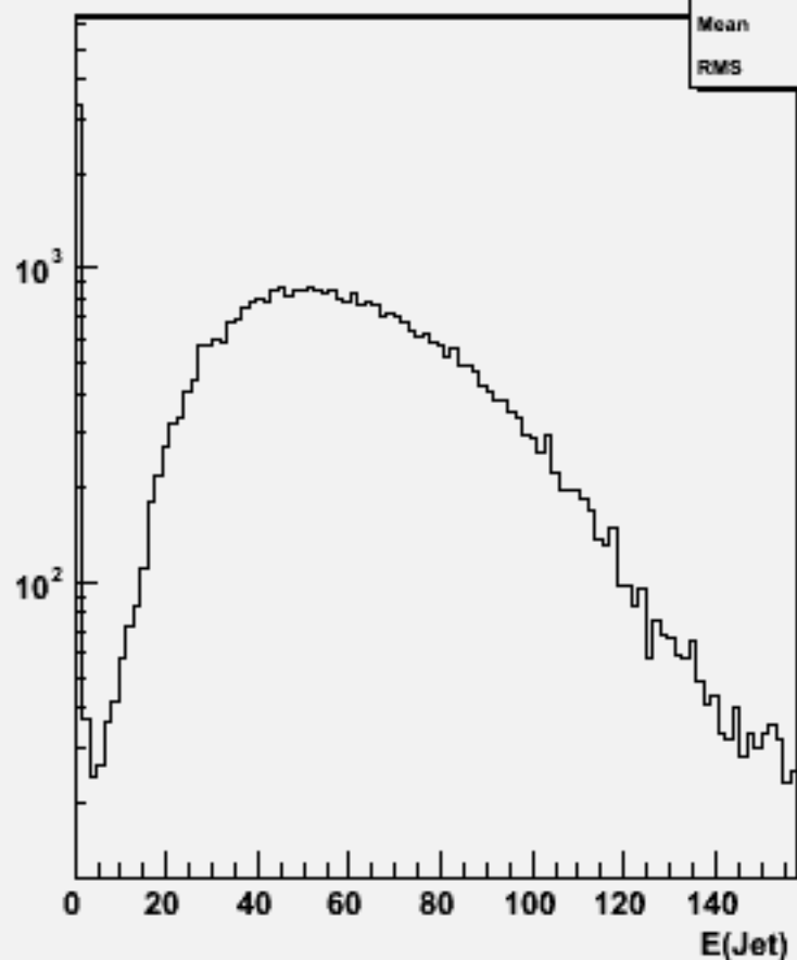
Jet energies(All jets)w101388 n1n1csdu_o
