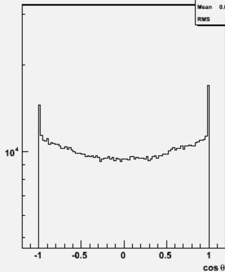
Particle cos \theta : w101388 n1n1csdu_o
