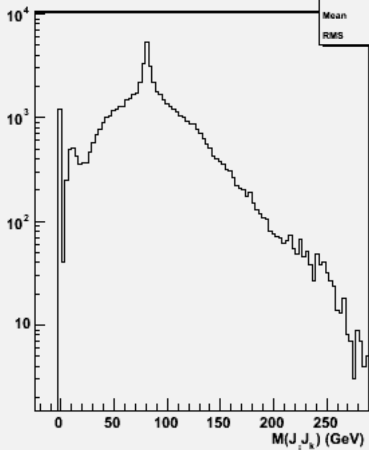
2jets mass(All comb)w101388 n1n1csdu_o
