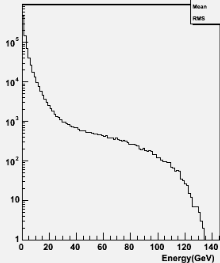
Particle Energy : w101388 n1n1csdu_o
