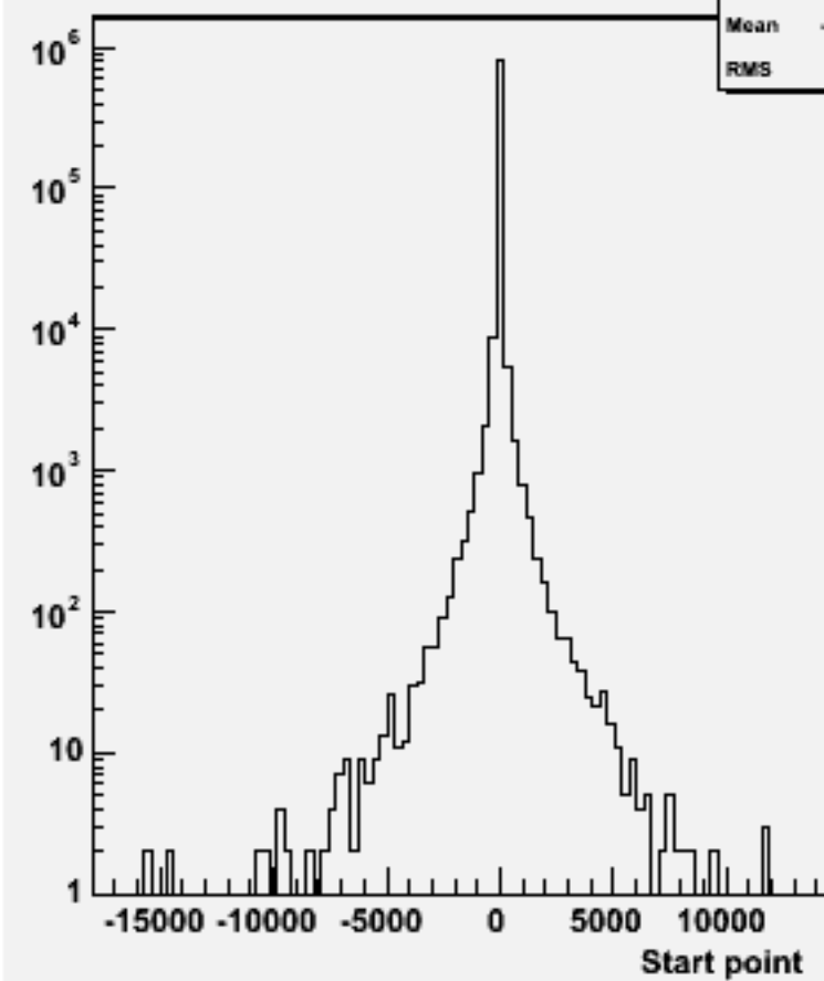
Start point Z : w101388 n1n1csdu_o
