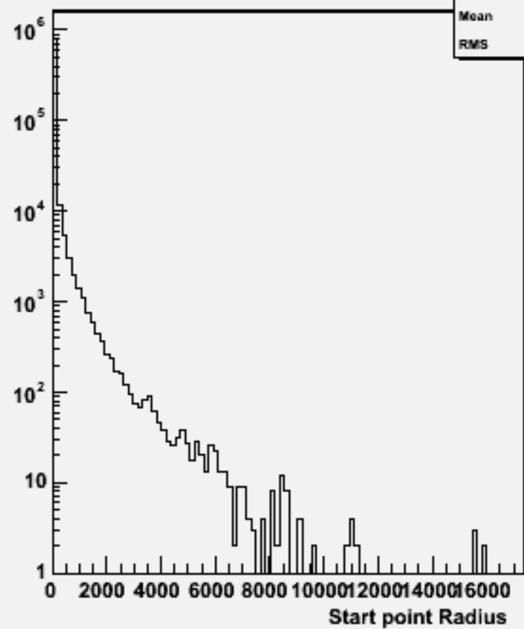
Start point R : w101388 n1n1csdu_o
