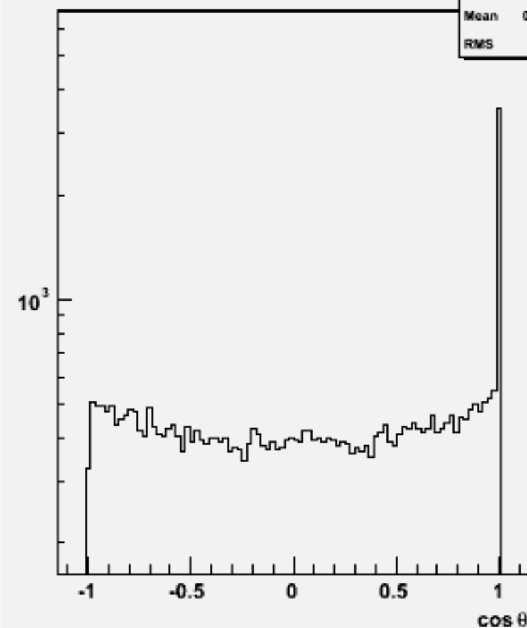
Jet cosθ (All jets)w101388 n1n1csdu_o
