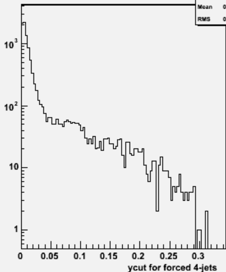
Ycut for 4-jets :w101388 n1n1csdu_o
