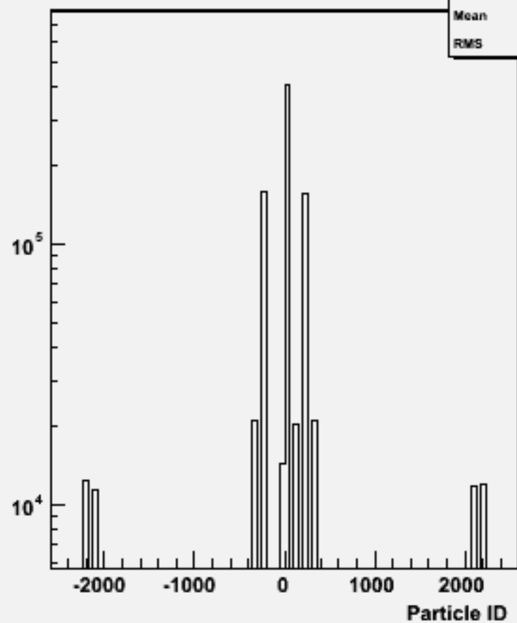
Particle ID : w101388 n1n1csdu_o
