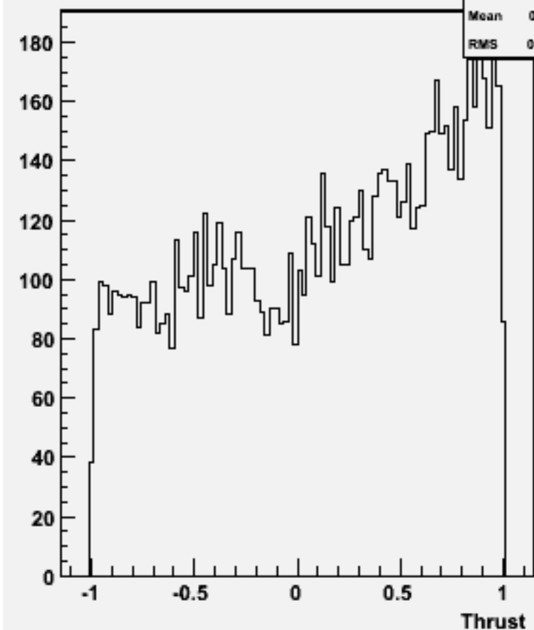
cos \Theta (thrust) w101381 n1n1cse2n2_o
