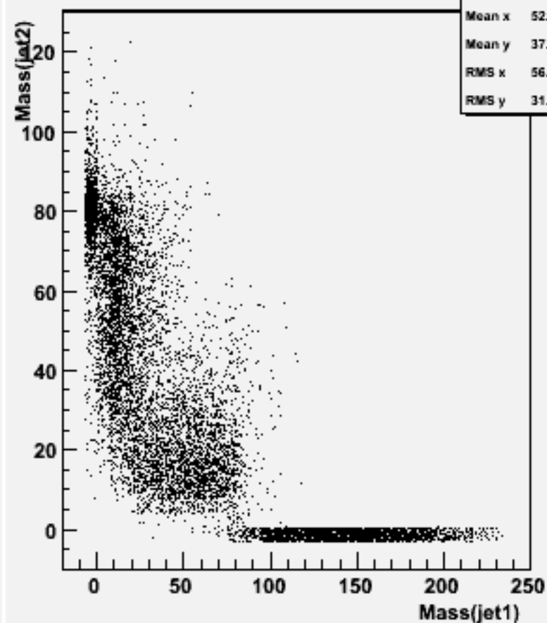
Jet mass for forced 2-jets : w101381 n1n1cse2n2_o
