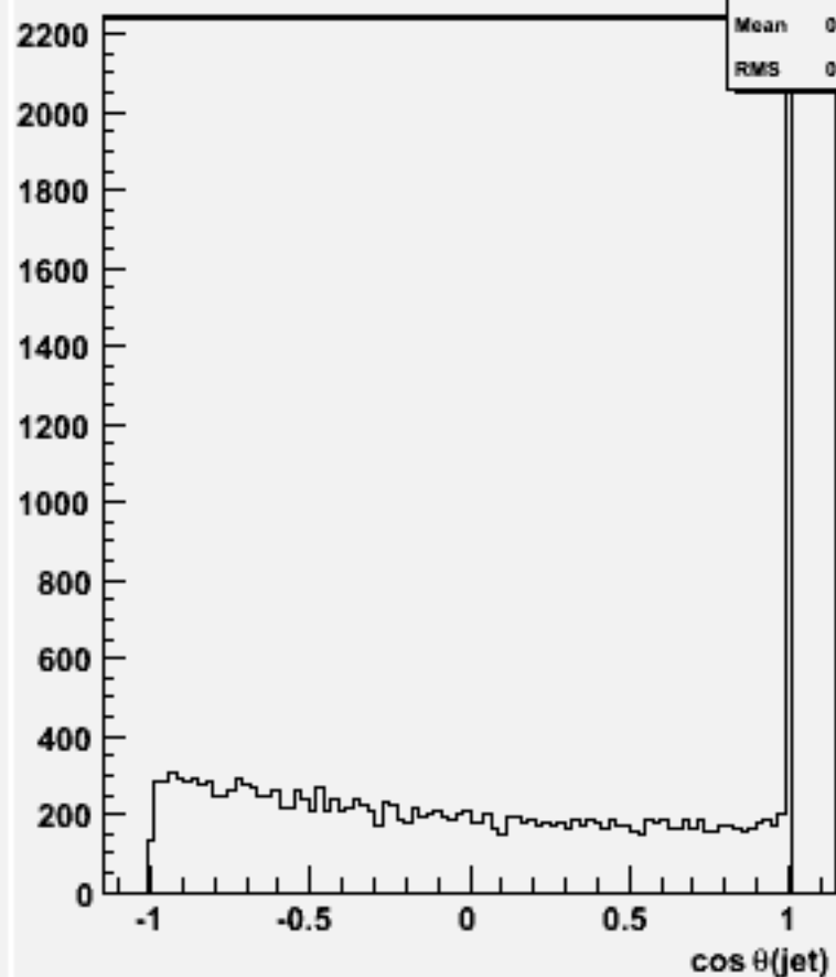
cos \theta for 2-jets :w101381 n1n1cse2n2_o
