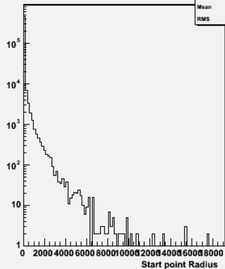
Start point R : w101381 n1n1cse2n2_o
