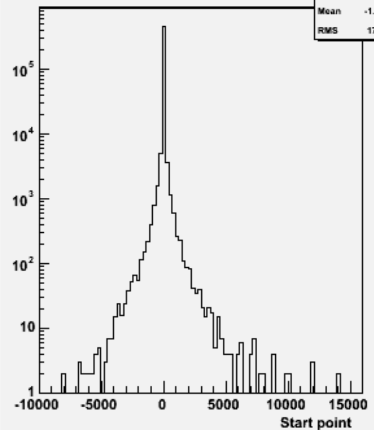
Start point Z : w101381 n1n1cse2n2_o
