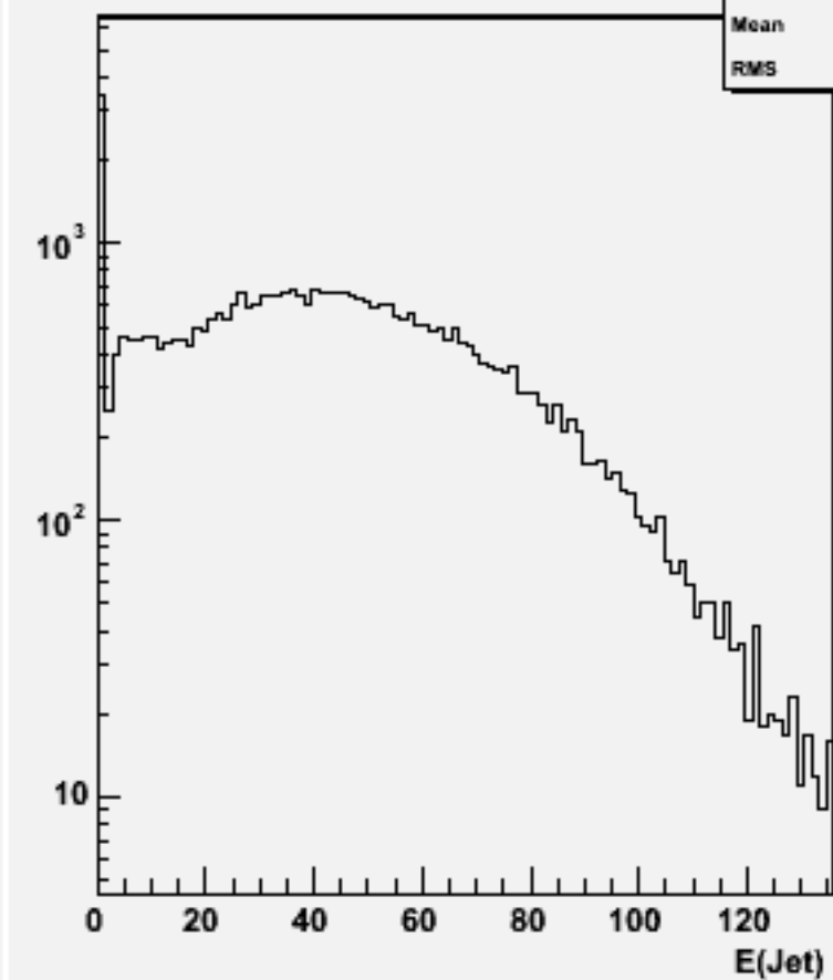
Jet energies(All jets)w101381 n1n1cse2n2_o
