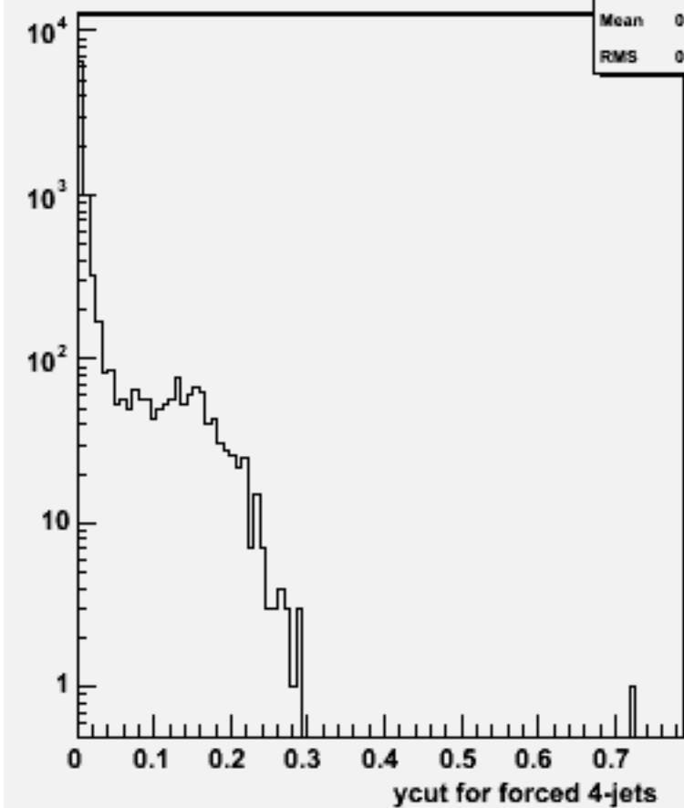
Ycut for 4-jets :w101381 n1n1cse2n2_o
