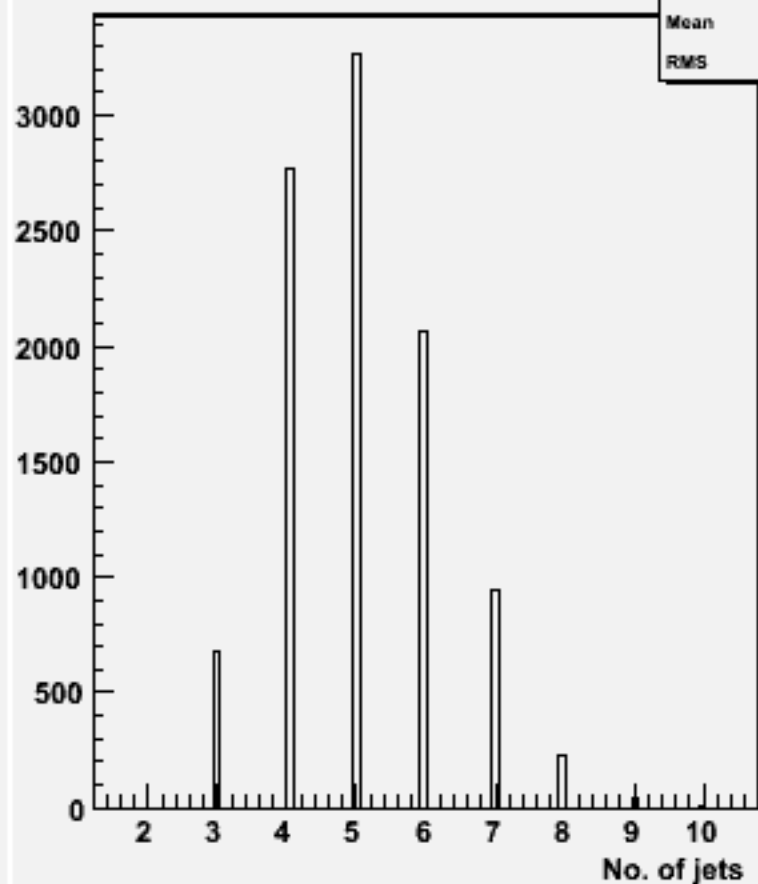
No. jets (ycut=0.001) : w101381 n1n1cse2n2_o
