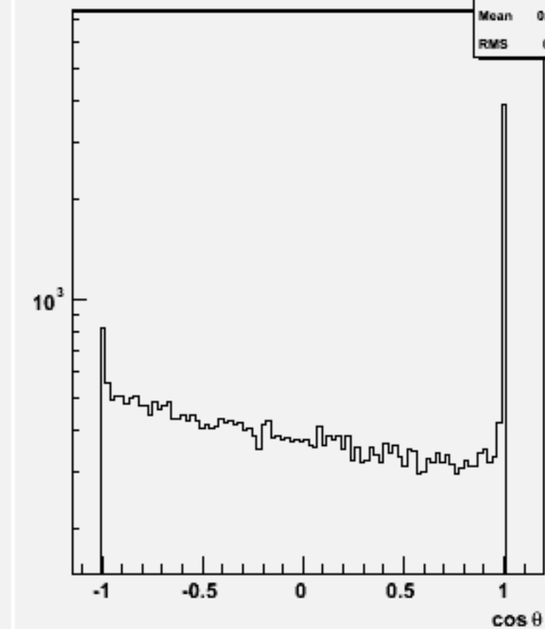
Jet cos \theta (All jets)w101381 n1n1cse2n2_o
