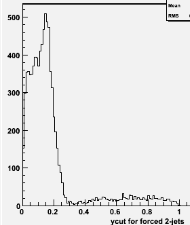
Ycut for 2-jets :w101381 n1n1cse2n2_o
