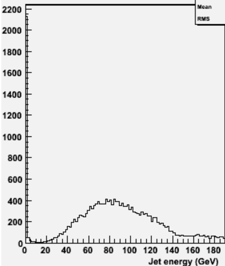
energy for 2-jets :w101381 n1n1cse2n2_o
