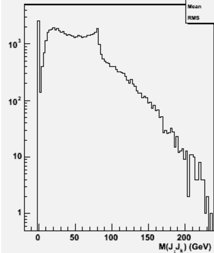
2jets mass(All comb)w101381 n1n1cse2n2_o
