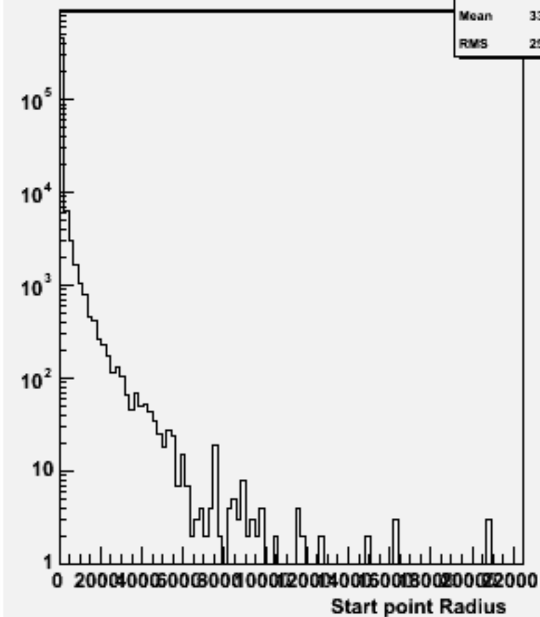
Start point R : w101380 n1n1cse2n2_o
