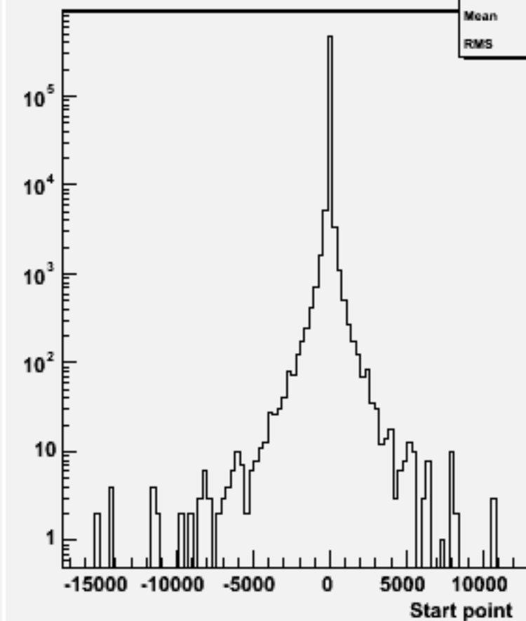
Start point Z : w101380 n1n1cse2n2_o
