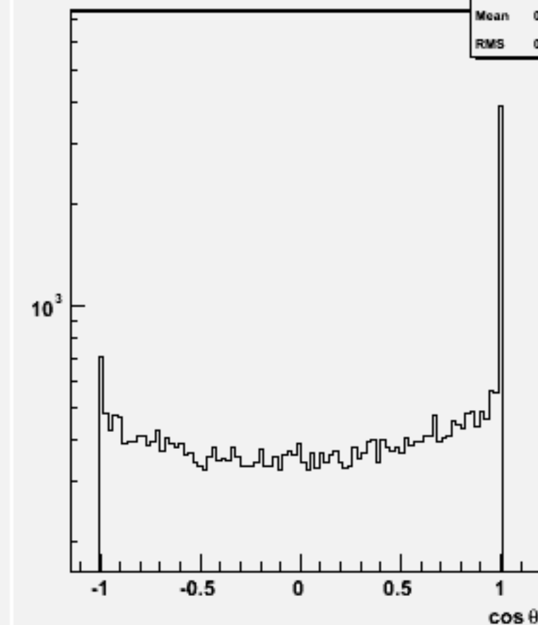
Jet cos \theta (All jets)w101380 n1n1cse2n2_o
