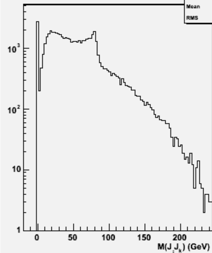
2jets mass(All comb)w101380 n1n1cse2n2_o
