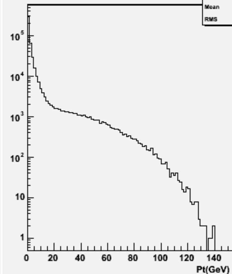
Particle Pt : w101380 n1n1cse2n2_o
