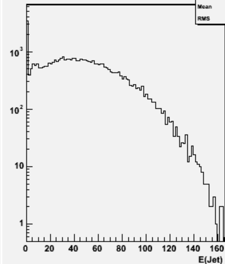
Jet energies(All jets)w101380 n1n1cse2n2_o
