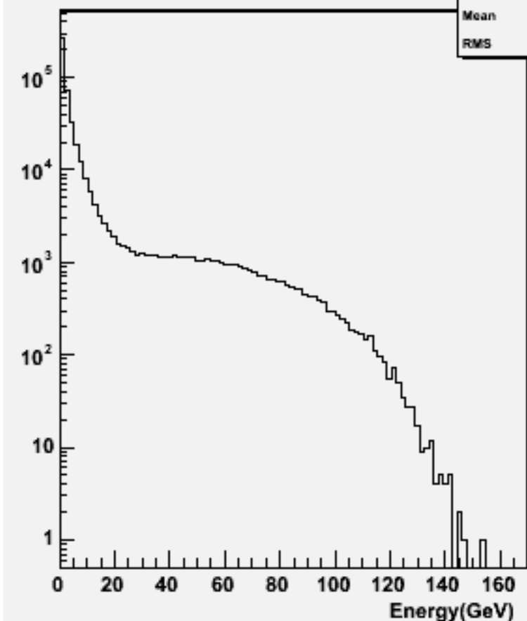
Particle Energy : w101380 n1n1cse2n2_o
