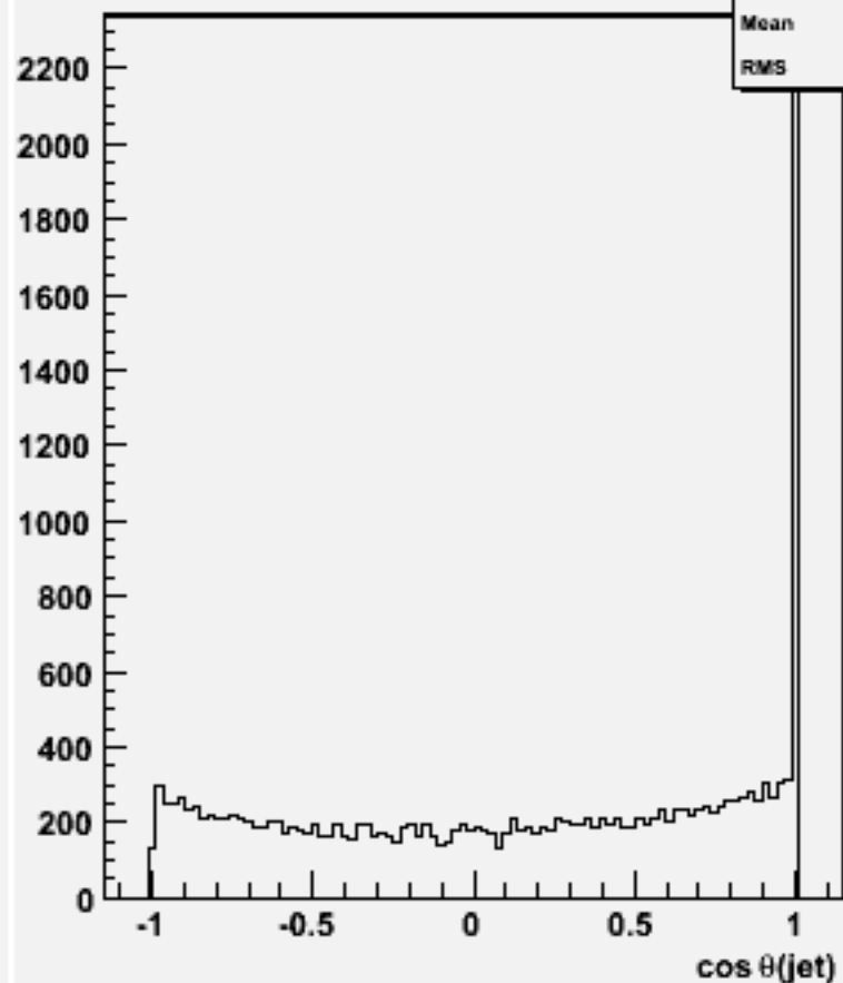
cos \theta for 2-jets :w101380 n1n1cse2n2_o
