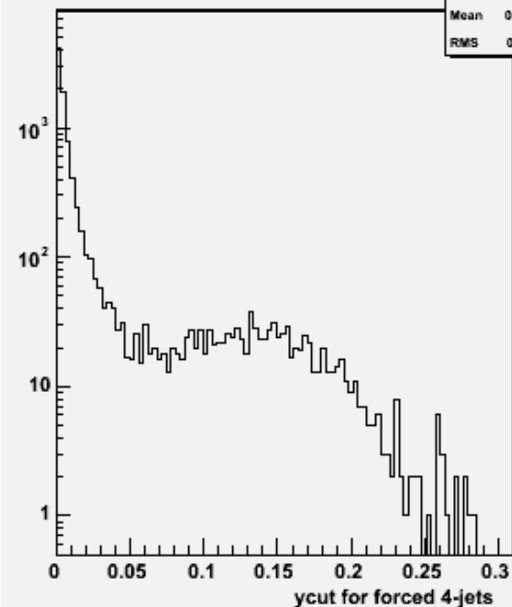
Ycut for 4-jets :w101380 n1n1cse2n2_o
