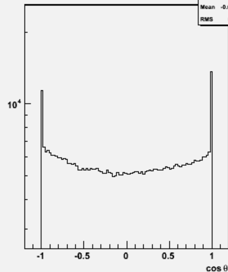
Particle cos \theta : w101380 n1n1cse2n2_o
