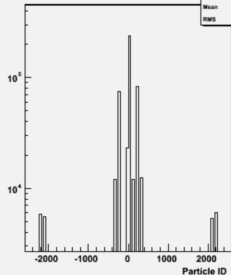
Particle ID : w101380 n1n1cse2n2_o
