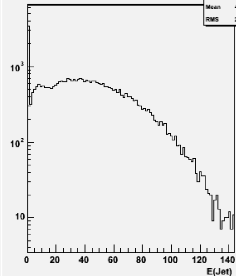
Jet energies(All jets)w101378 n1n1cse1n1_o
