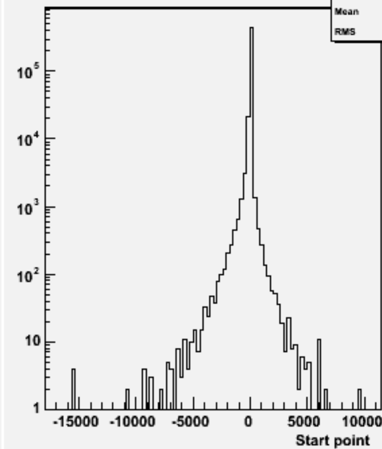
Start point Z : w101378 n1n1cse1n1_o
