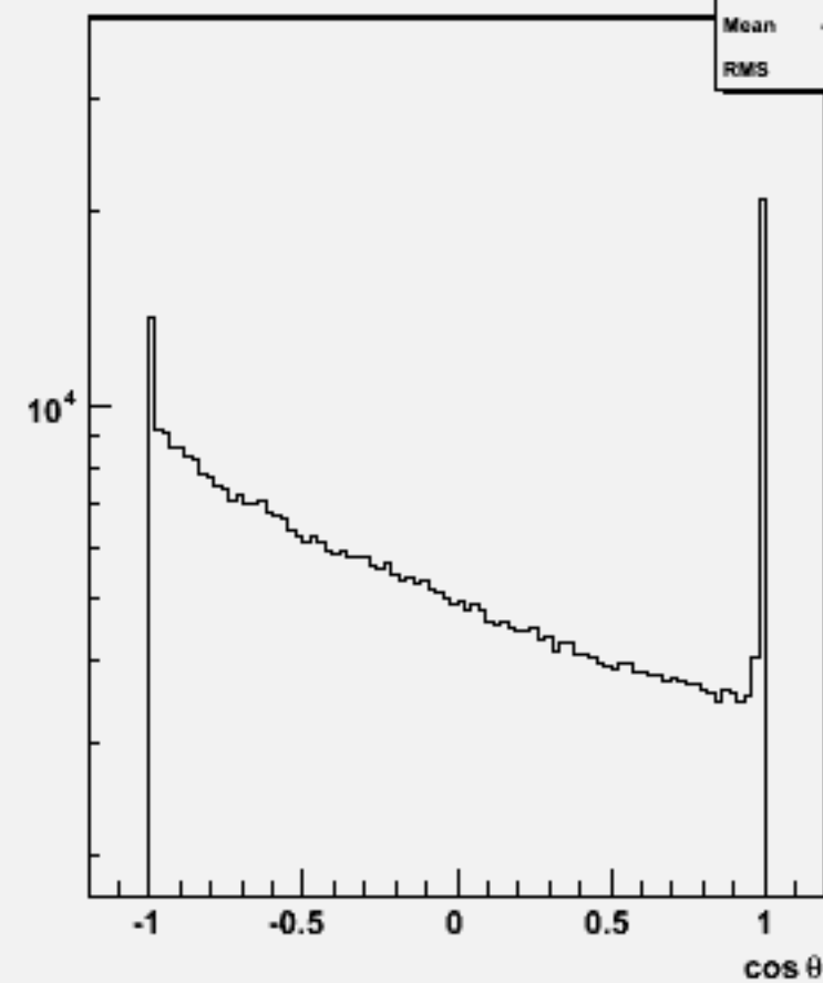
Particle \cos\theta : w101378 n1n1cse1n1_o
