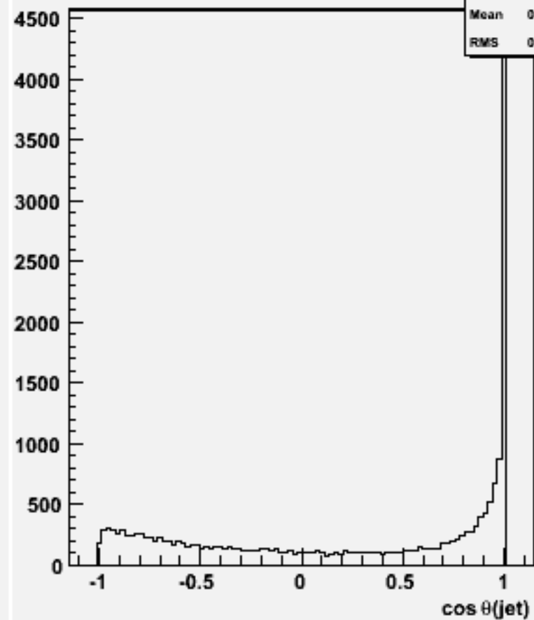
cos \Theta for 2-jets :w101378 n1n1cse1n1_o
