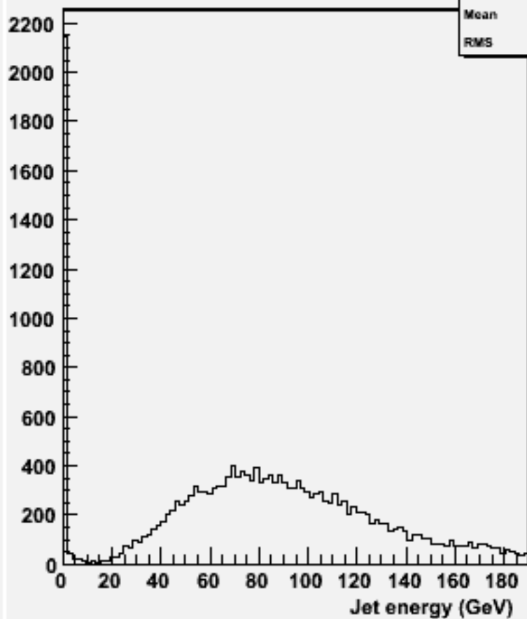
energy for 2-jets :w101378 n1n1cse1n1_o
