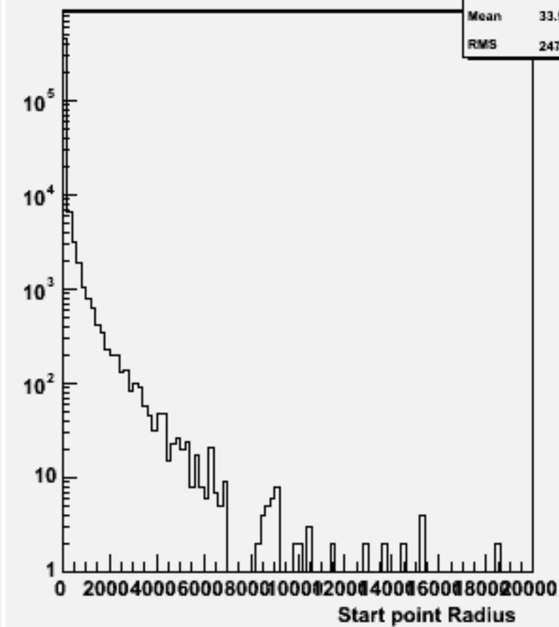
Start point R : w101378 n1n1cse1n1_o
