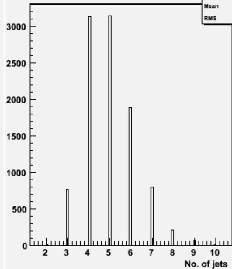
No. jets (ycut=0.001) : w101378 n1n1cse1n1_o
