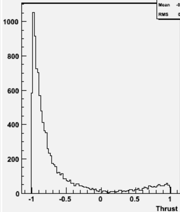
cos \Theta (thrust) w101378 n1n1cse1n1_o
