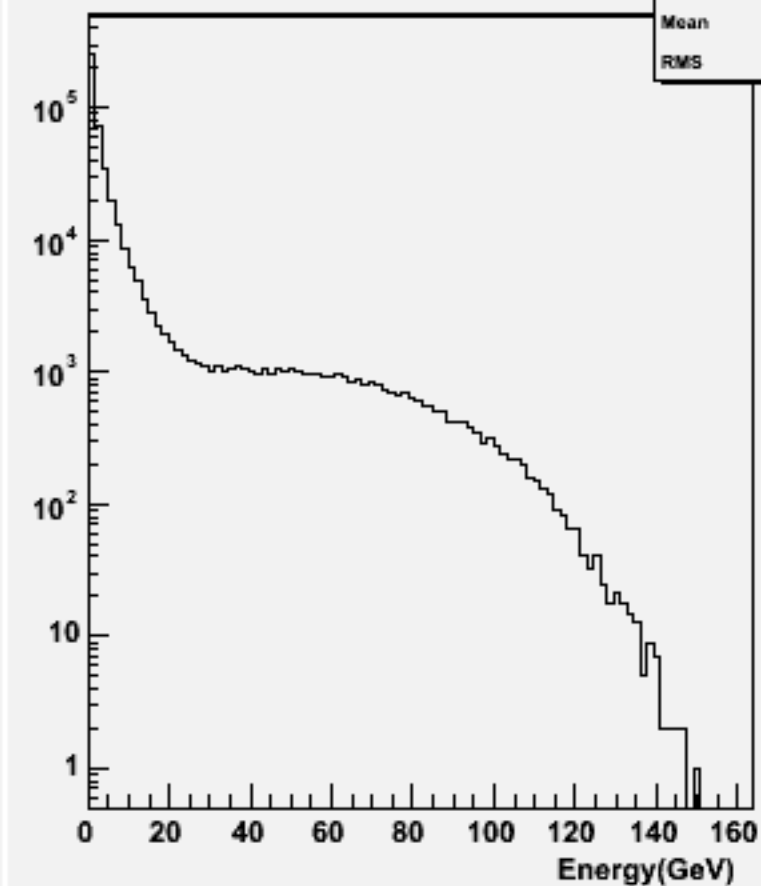
Start point R : w101378 n1n1cse1n1_o
