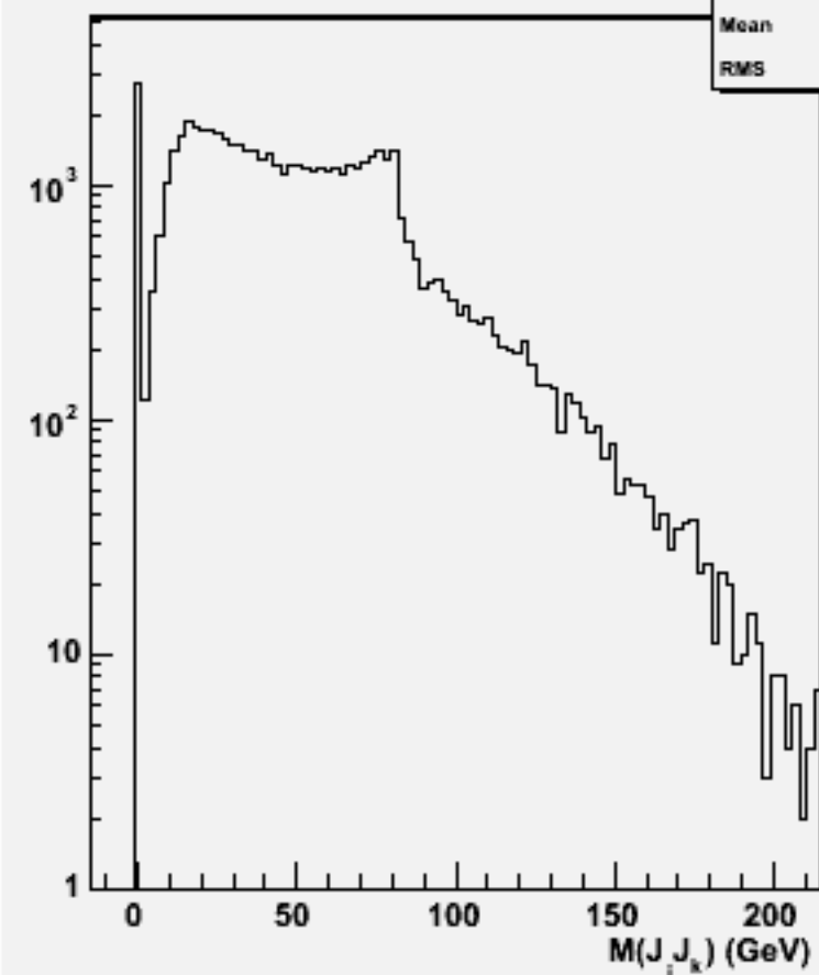
2jets mass(All comb)w101378 n1n1cse1n1_o
