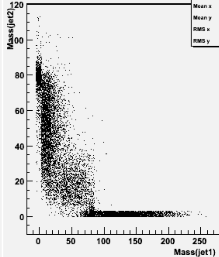
Jet mass for forced 2-jets : w101378 n1n1cse1n1_o
