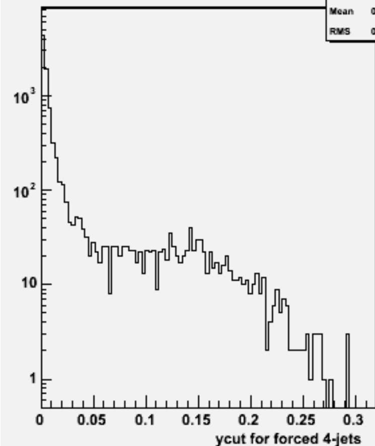
Ycut for 4-jets :w101378 n1n1cse1n1_o
