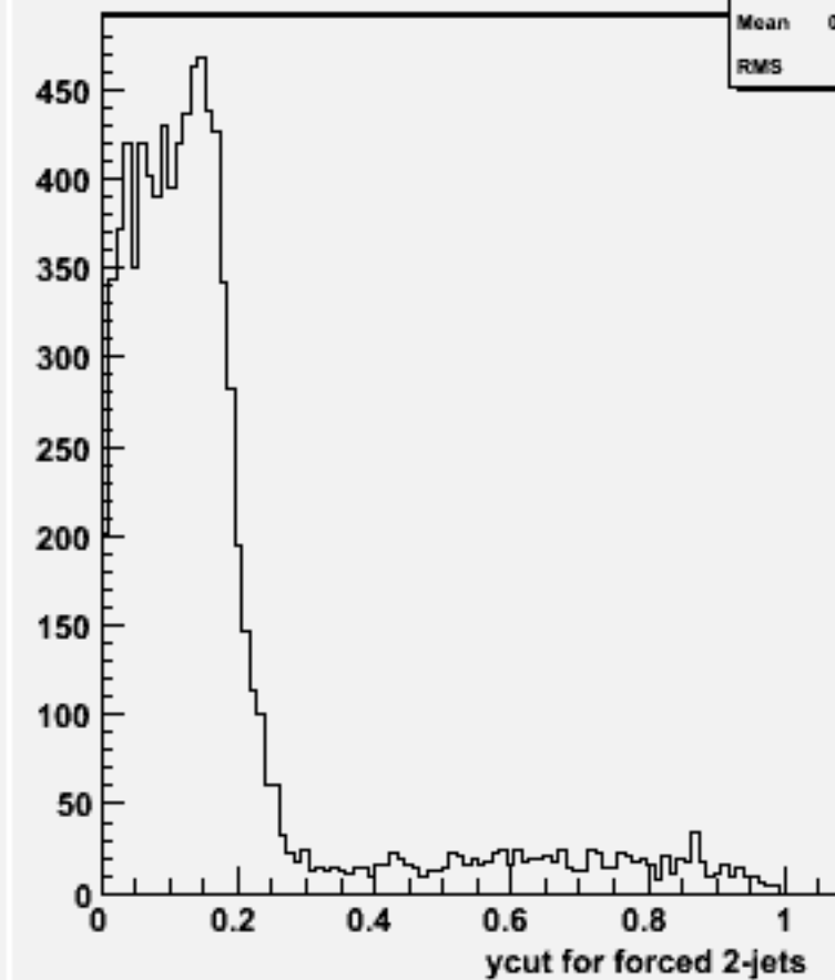
Ycut for 2-jets :w101378 n1n1cse1n1_o
