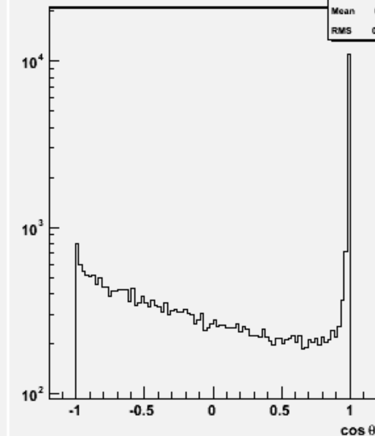
Jet cos \theta (All jets)w101378 n1n1cse1n1_o
