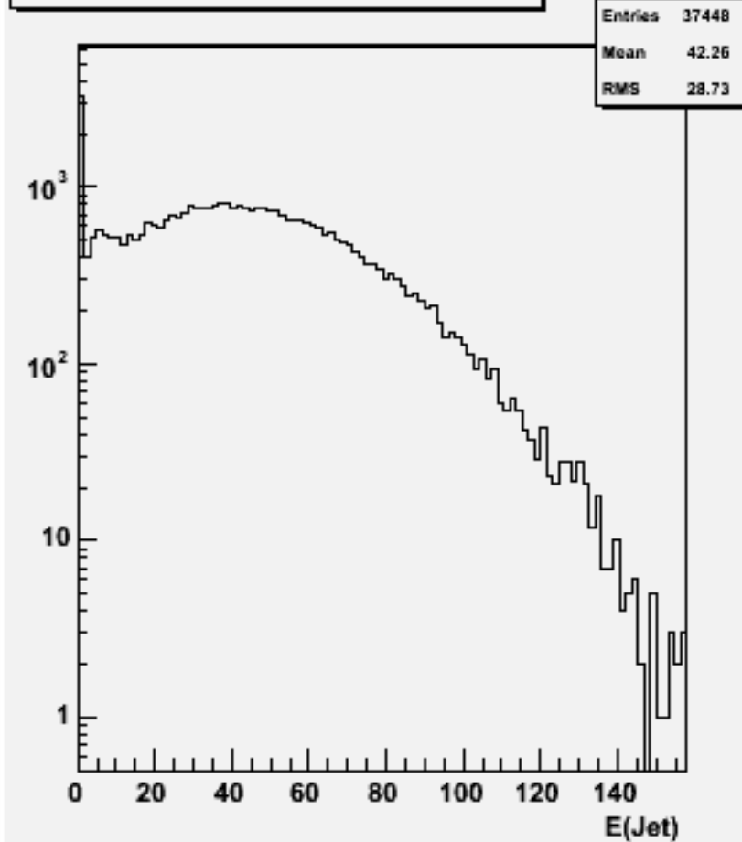
Jet energies(All jets)w101377 n1n1cse1n1_o
