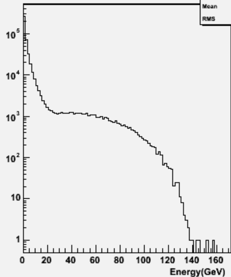
Particle Energy : w101377 n1n1cse1n1_o
