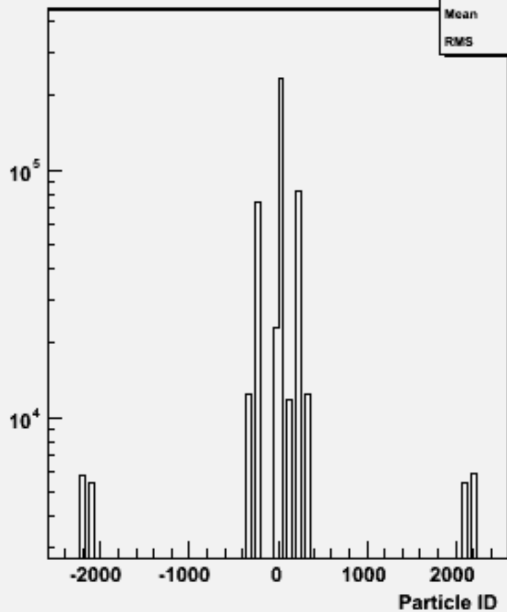
Particle ID : w101377 n1n1cse1n1_o
