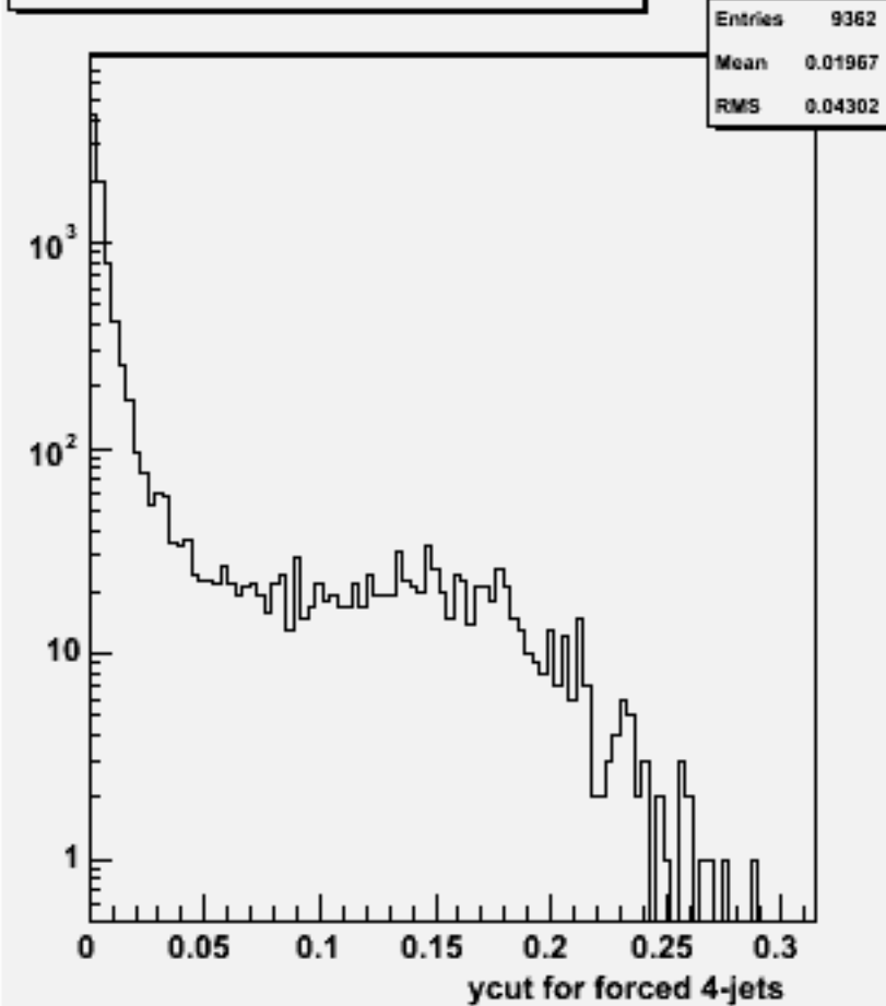
Ycut for 4-jets :w101377 n1n1cse1n1_o
