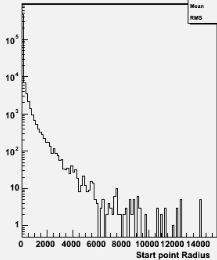
Start point R : w101377 n1n1cse1n1_o
