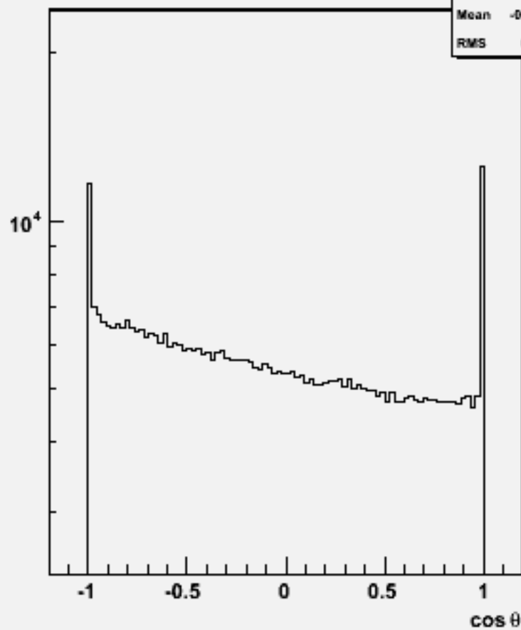
Particle \cos\theta : w101377 n1n1cse1n1_o
