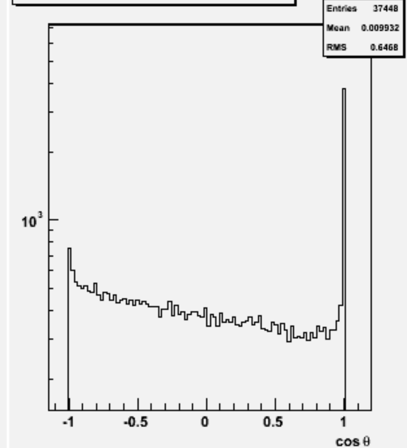
Jet cos \theta (All jets)w101377 n1n1cse1n1_o
