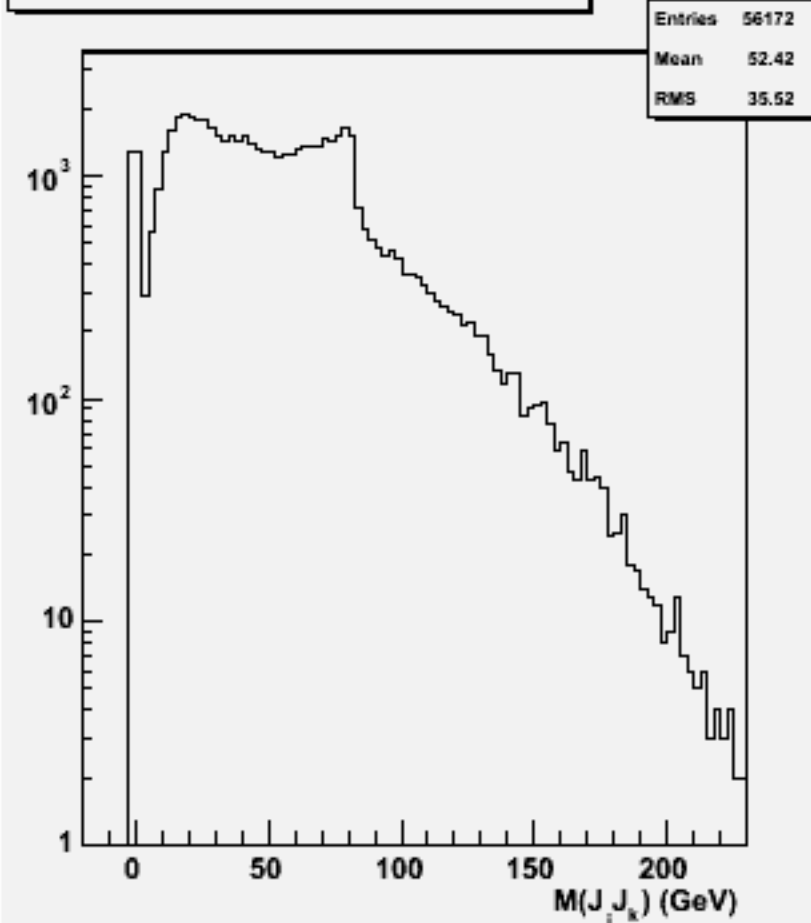
2jets mass(All comb)w101377 n1n1cse1n1_o
