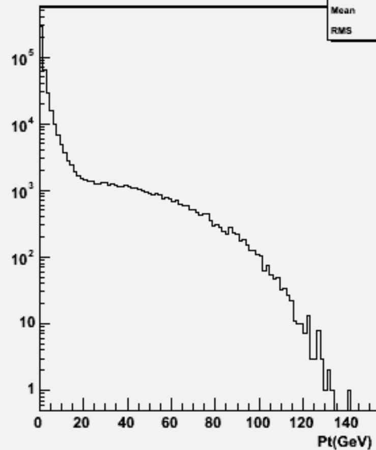
Particle Pt : w101377 n1n1cse1n1_o
