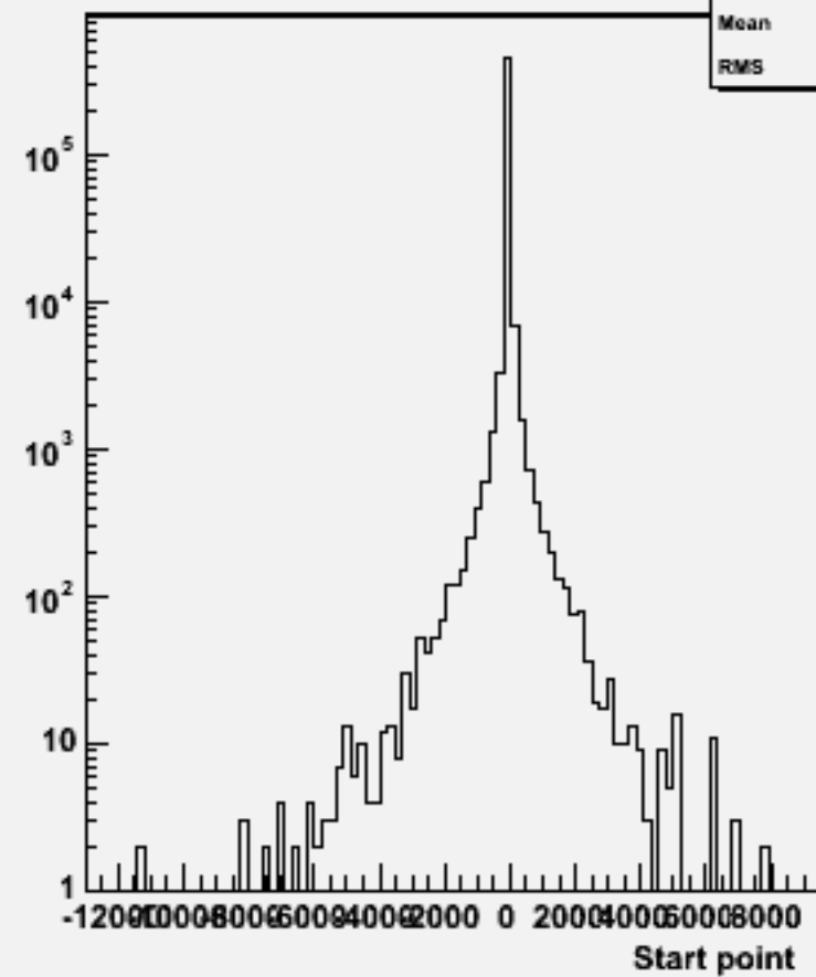
Start point Z : w101377 n1n1cse1n1_o
