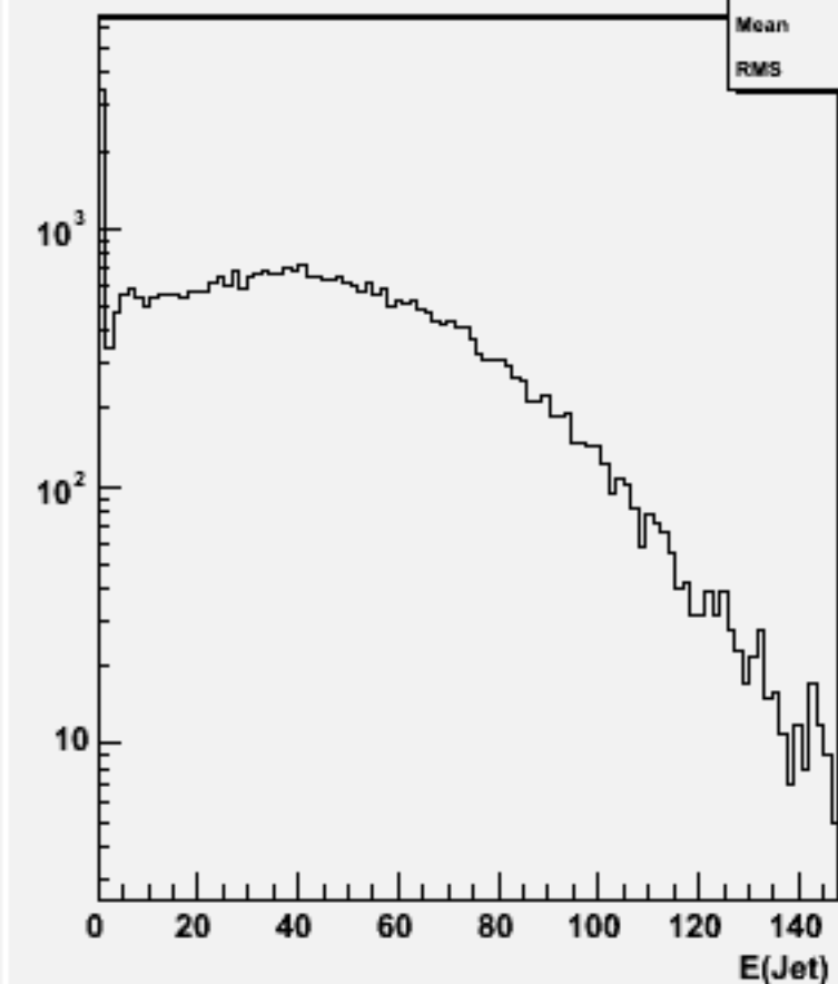
Jet energies(All jets)w101376 n1n1cse1n1_o
