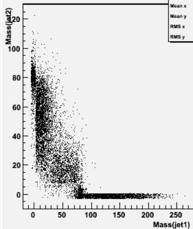
Jet mass for forced 2-jets : w101376 n1n1cse1n1_o
