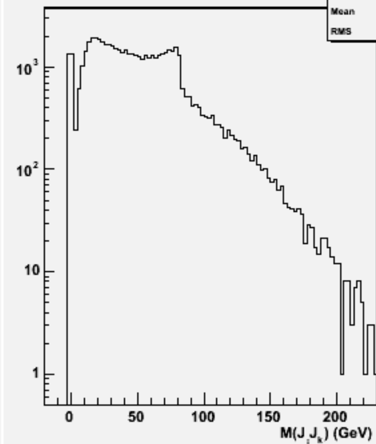
2jets mass(All comb)w101376 n1n1cse1n1_o
