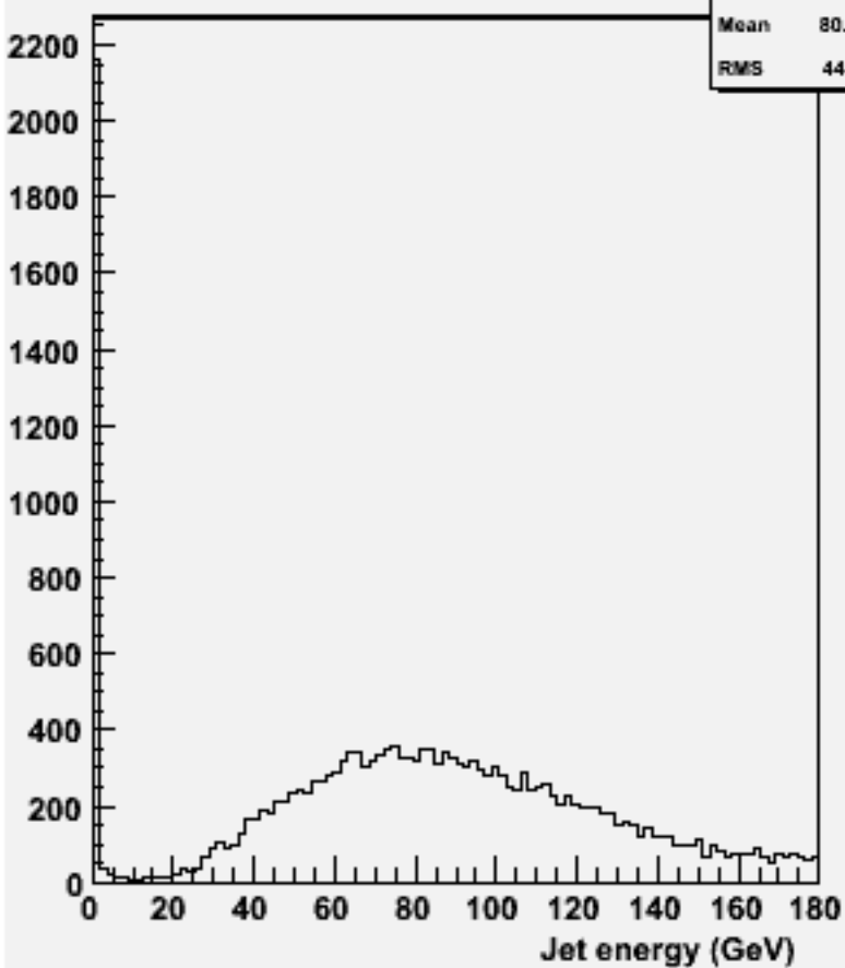
energy for 2-jets :w101376 n1n1cse1n1_o
