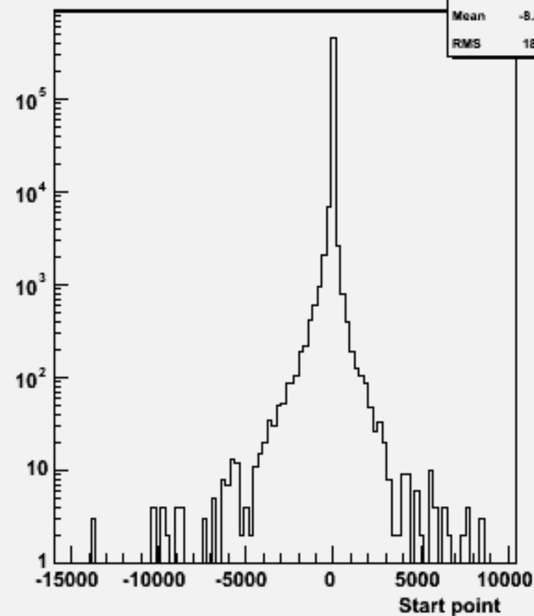
Start point Z : w101376 n1n1cse1n1_o
