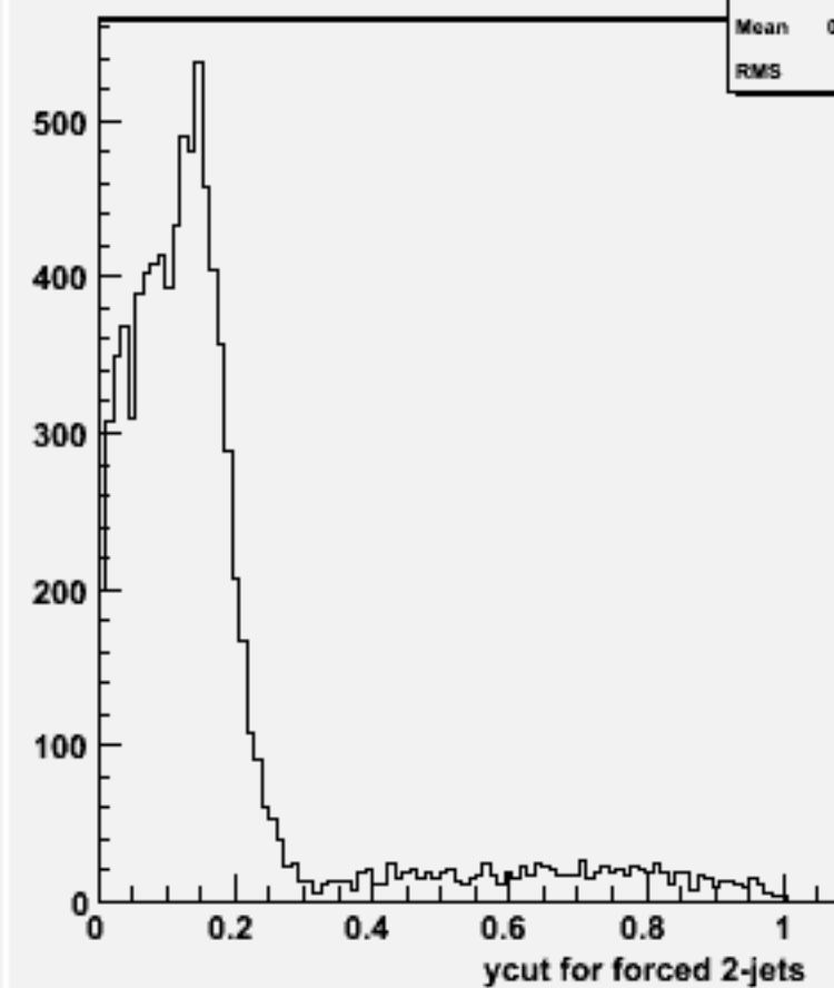
Ycut for 2-jets :w101376 n1n1cse1n1_o
