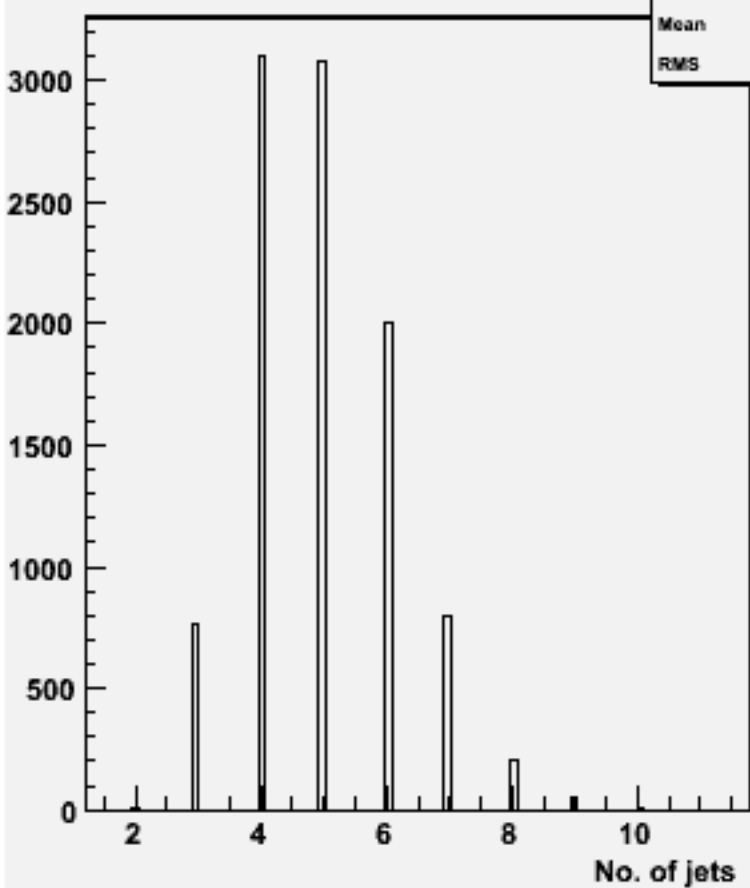
No. jets (ycut=0.001) : w101376 n1n1cse1n1_o
