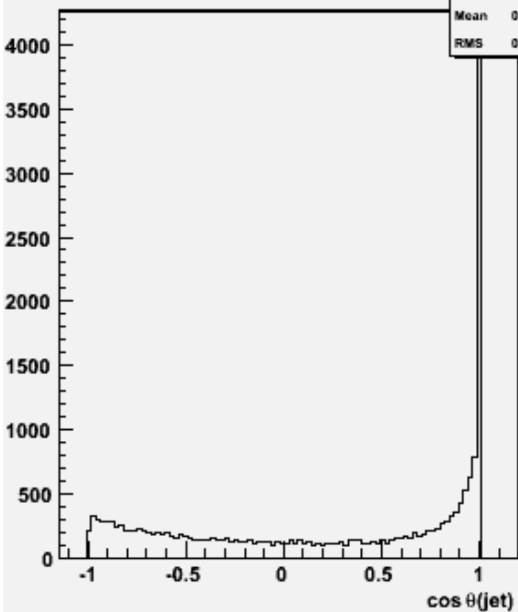
cos \theta for 2-jets :w101376 n1n1cse1n1_o
