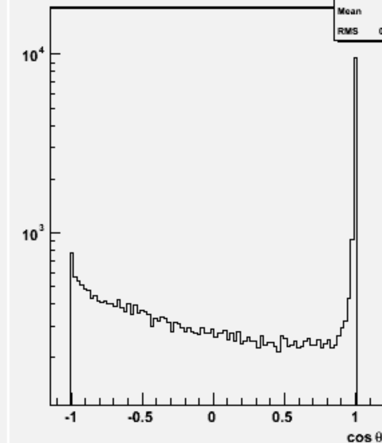
Jet cos \theta (All jets)w101376 n1n1cse1n1_o
