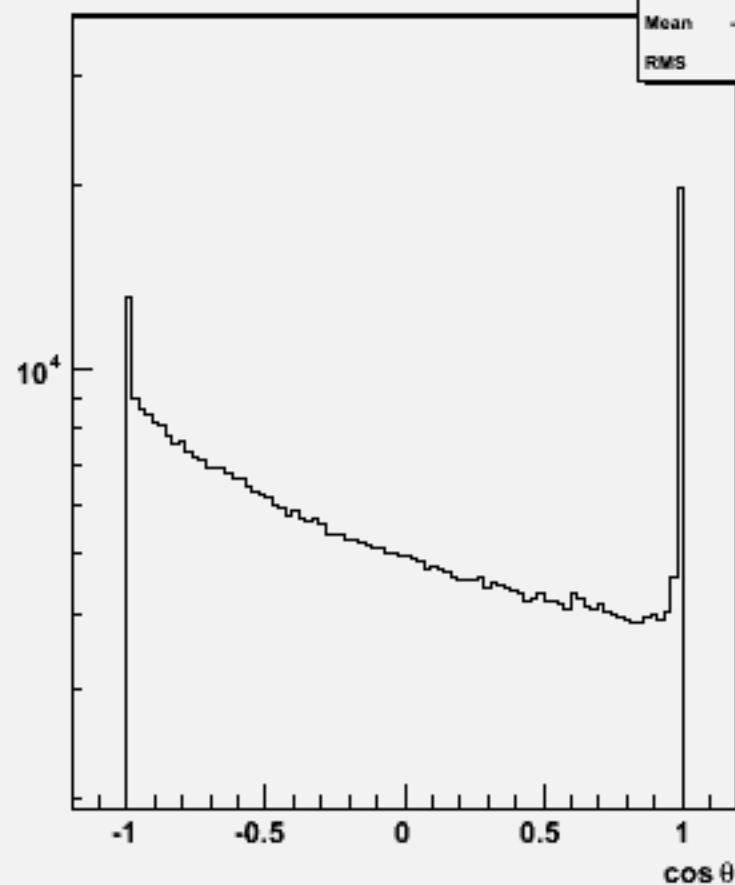
Particle cos \theta : w101376 n1n1cse1n1_o
