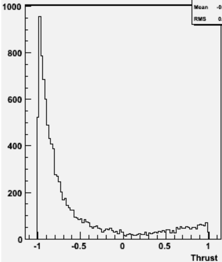
cos \Theta (thrust) w101376 n1n1cse1n1_o
