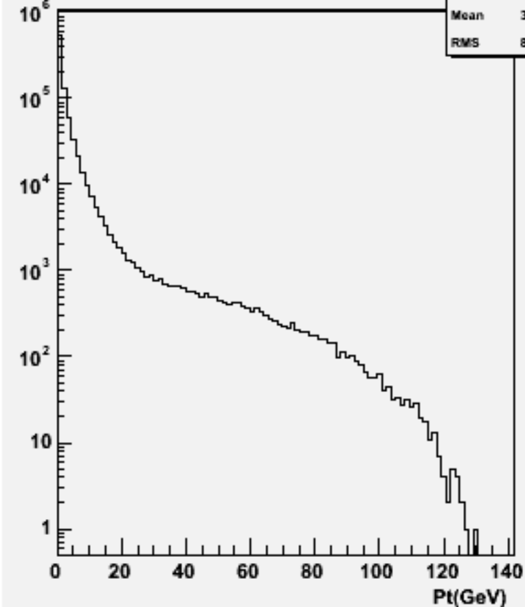
Particle Pt : w101373 n1n1udsc_o
