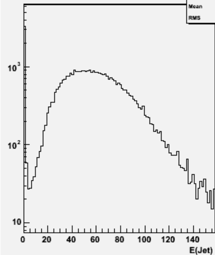
Jet energies(All jets)w101373 n1n1udsc_o
