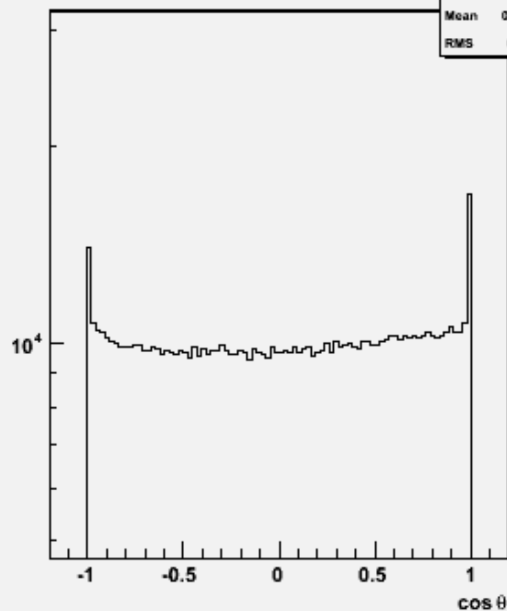
Particle cos \theta : w101373 n1n1udsc_o
