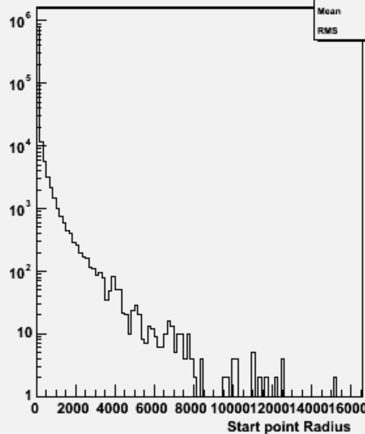
Start point R : w101373 n1n1udsc_o
