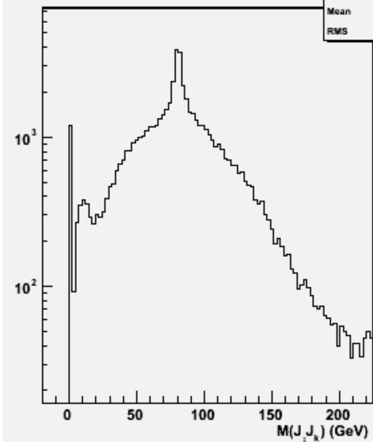
2jets mass(All comb)w101373 n1n1udsc_o
