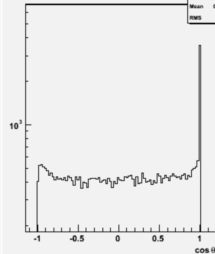
Jet cos \theta (All jets)w101373 n1n1udsc_o
