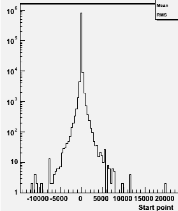
Start point Z : w101373 n1n1udsc_o
