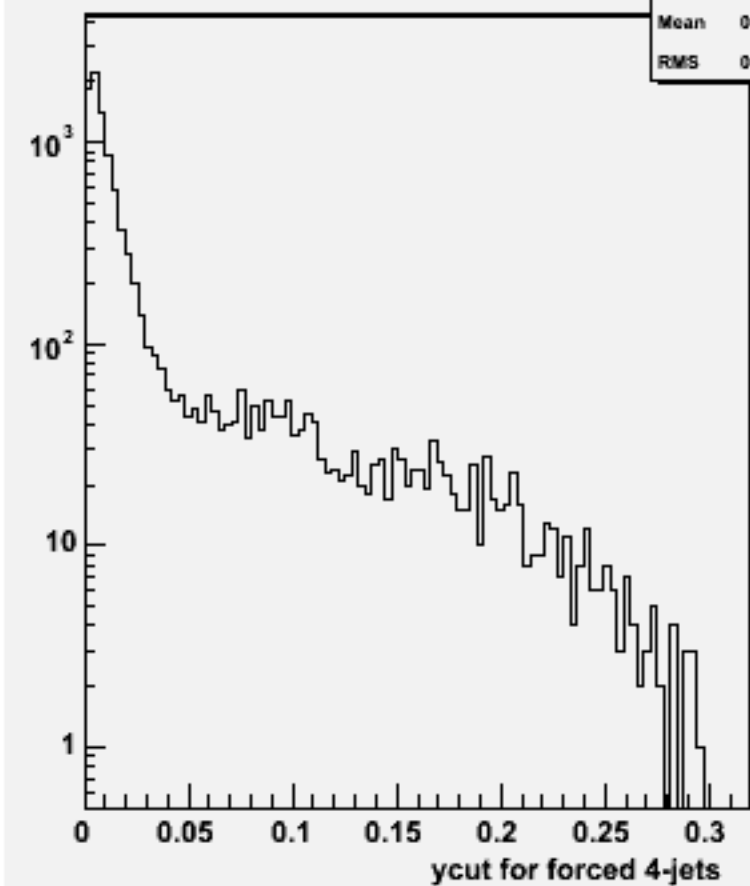
Ycut for 4-jets :w101373 n1n1udsc_o
