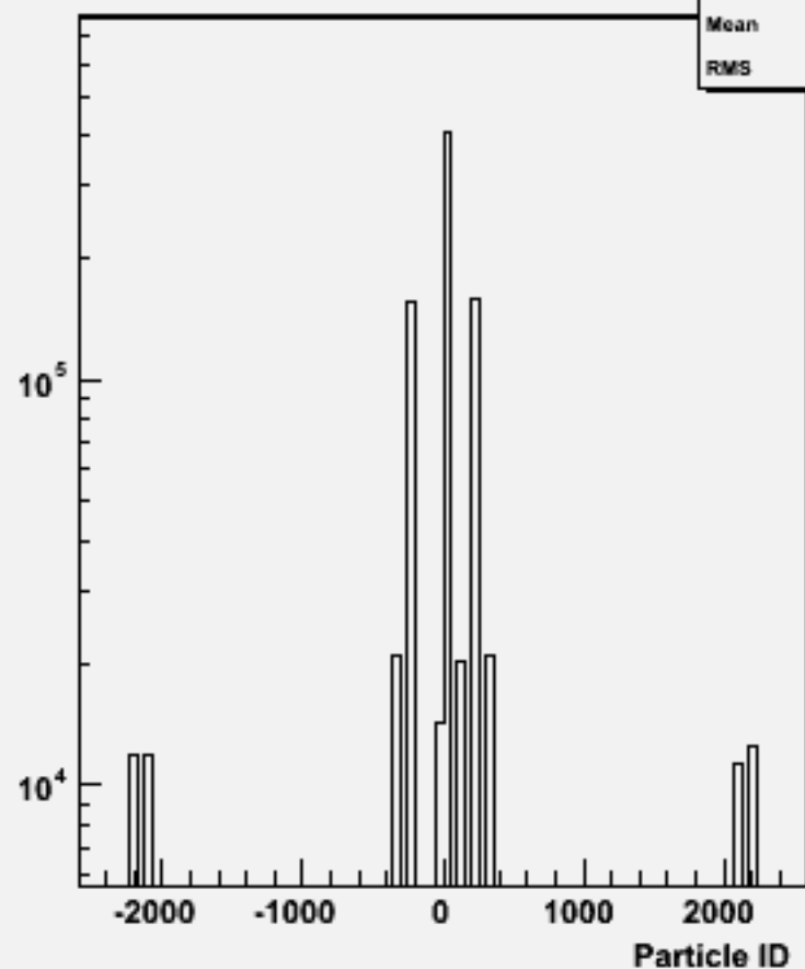
Particle ID : w101373 n1n1udsc_o
