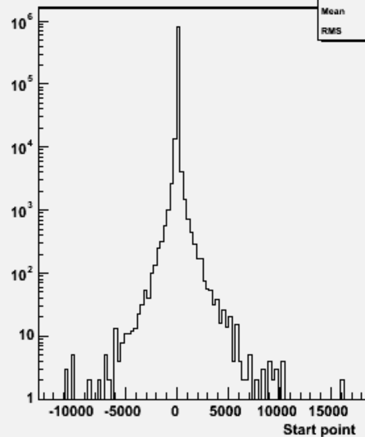
Start point Z : w101372 n1n1udsc_o
