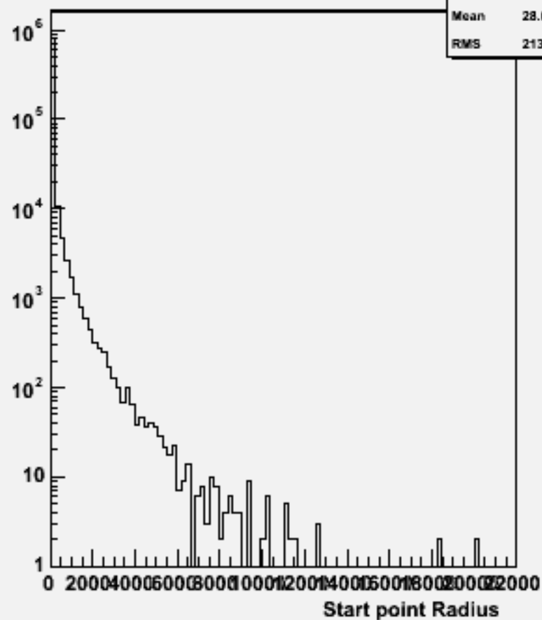
Start point R : w101372 n1n1udsc_o
