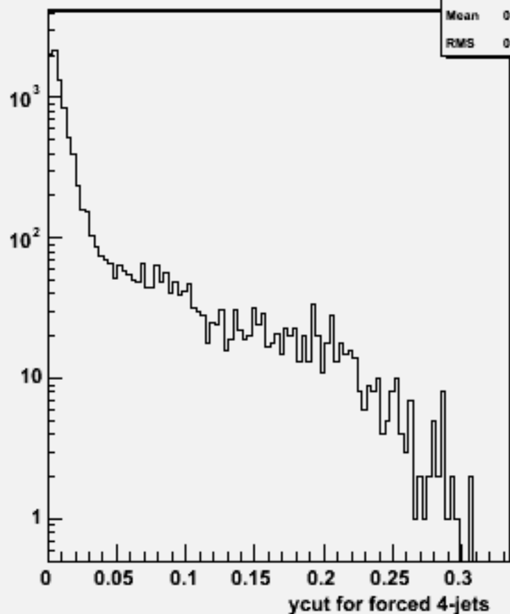
Ycut for 4-jets :w101372 n1n1udsc_o
