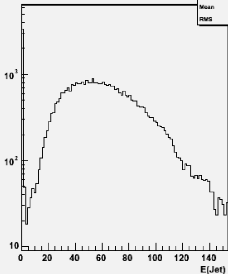
Jet energies(All jets)w101372 n1n1udsc_o
