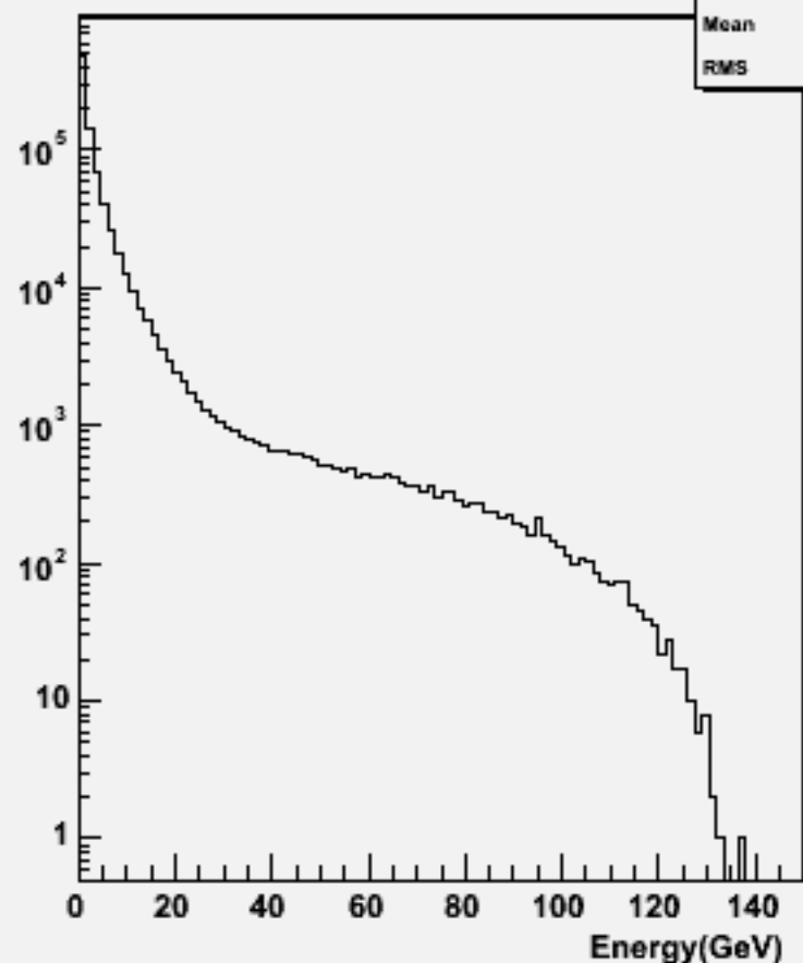
Particle Energy : w101372 n1n1udsc_o
