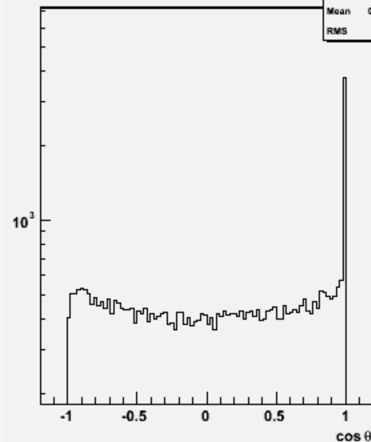
Jet cos \theta (All jets)w101372 n1n1udsc_o
