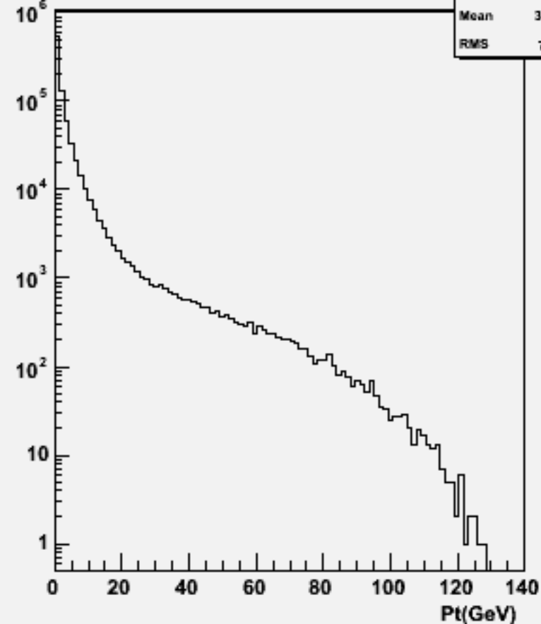
Particle Pt : w101372 n1n1udsc_o
