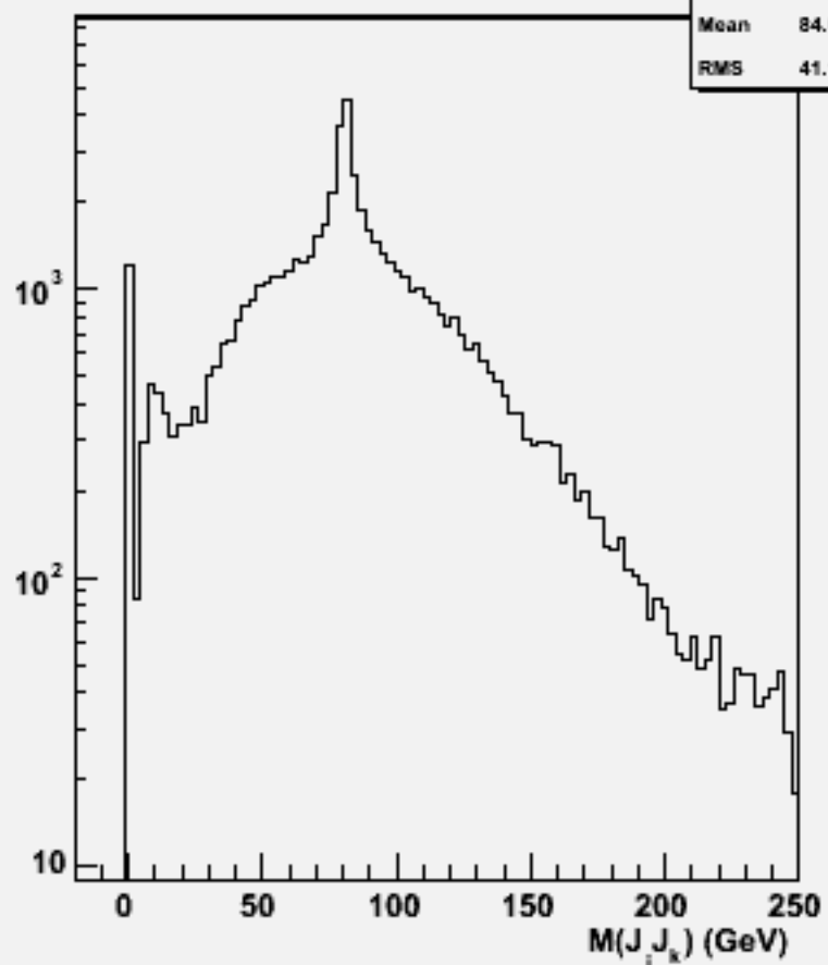
2jets mass(All comb)w101372 n1n1udsc_o
