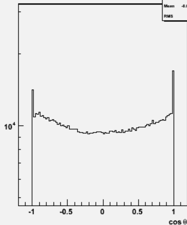
Particle cos \theta : w101372 n1n1udsc_o
