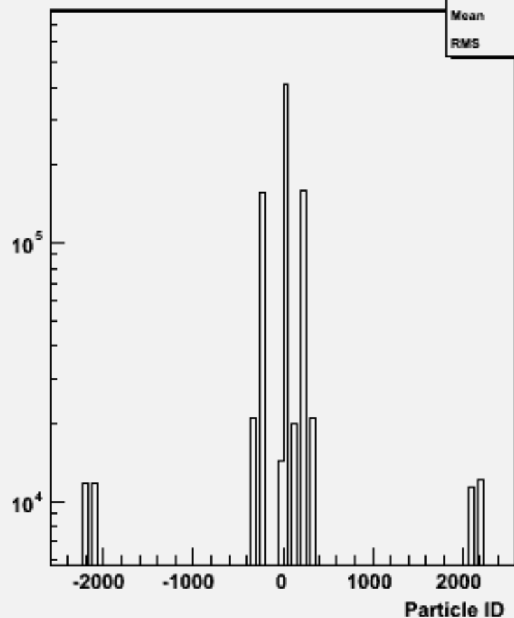
Particle ID : w101372 n1n1udsc_o
