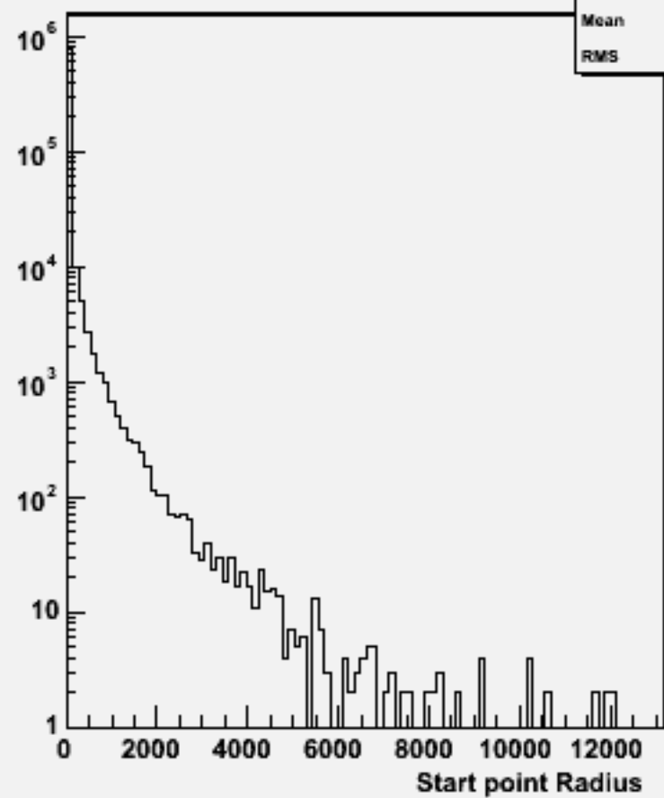
Start point R : w101369 n1n1uddu_o
