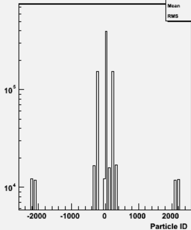
Particle ID : w101369 n1n1uddu_o
