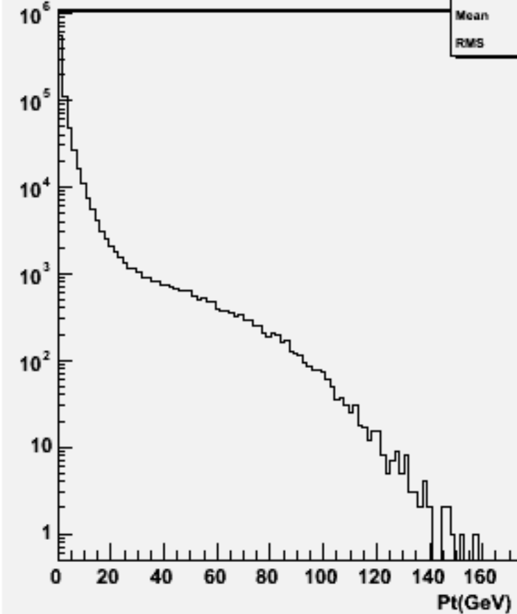
Particle Pt : w101369 n1n1uddu_o
