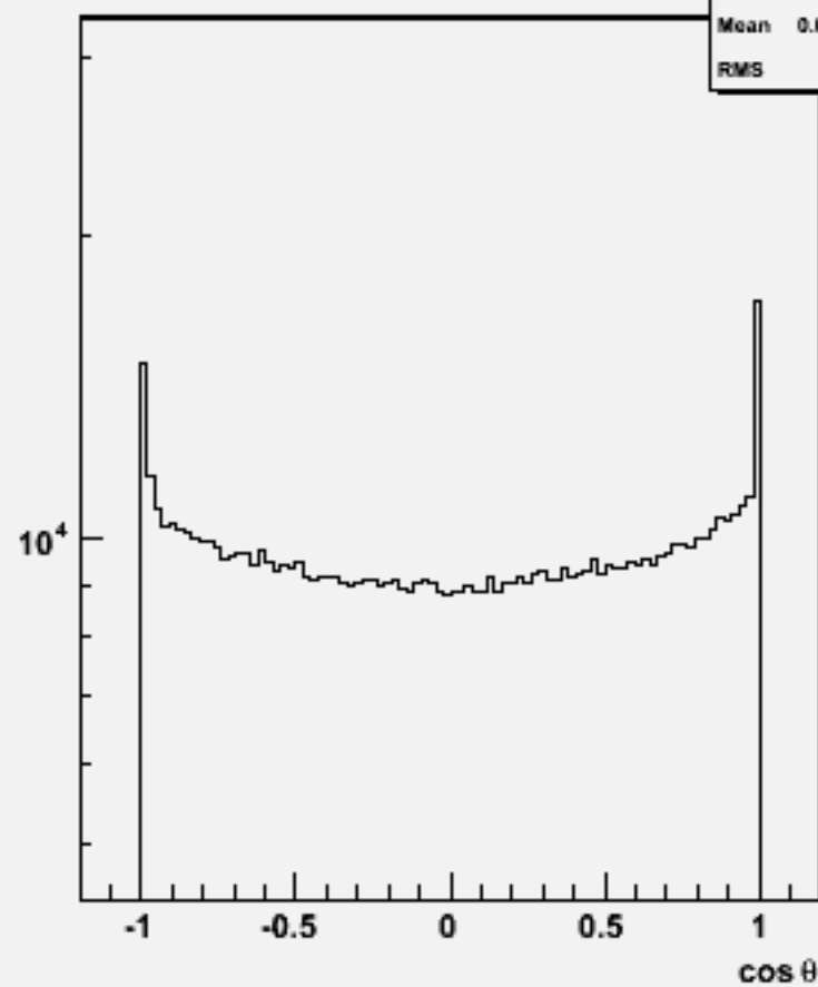
Particle cos \theta : w101369 n1n1uddu_o
