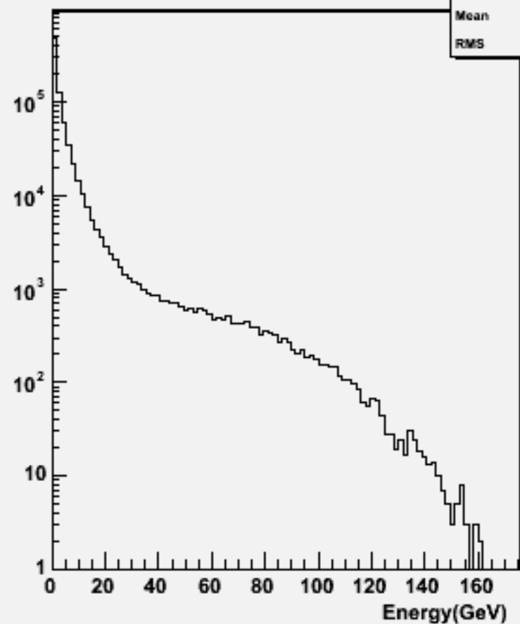
Particle Energy : w101369 n1n1uddu_o
