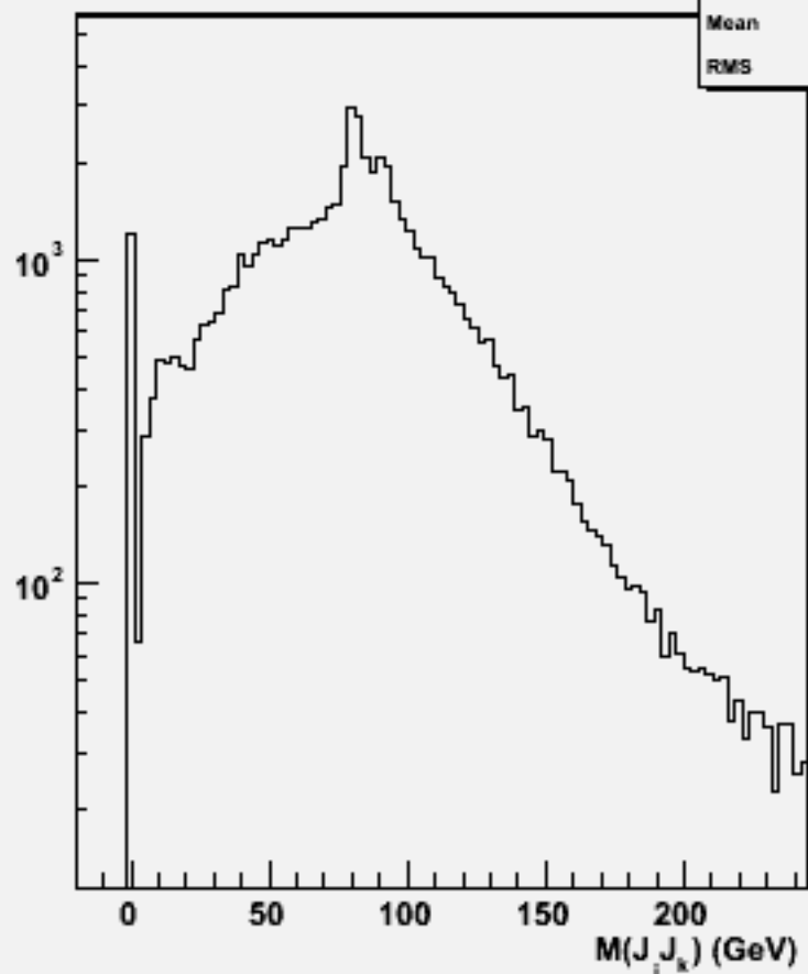
2jets mass(All comb)w101369 n1n1uddu_o
