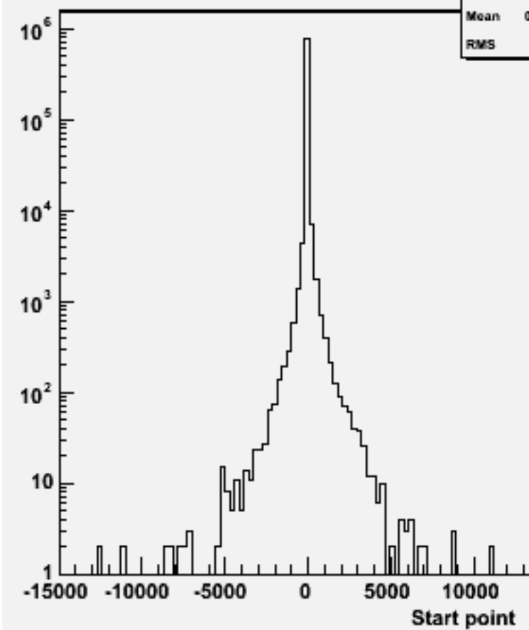
Start point Z : w101369 n1n1uddu_o
