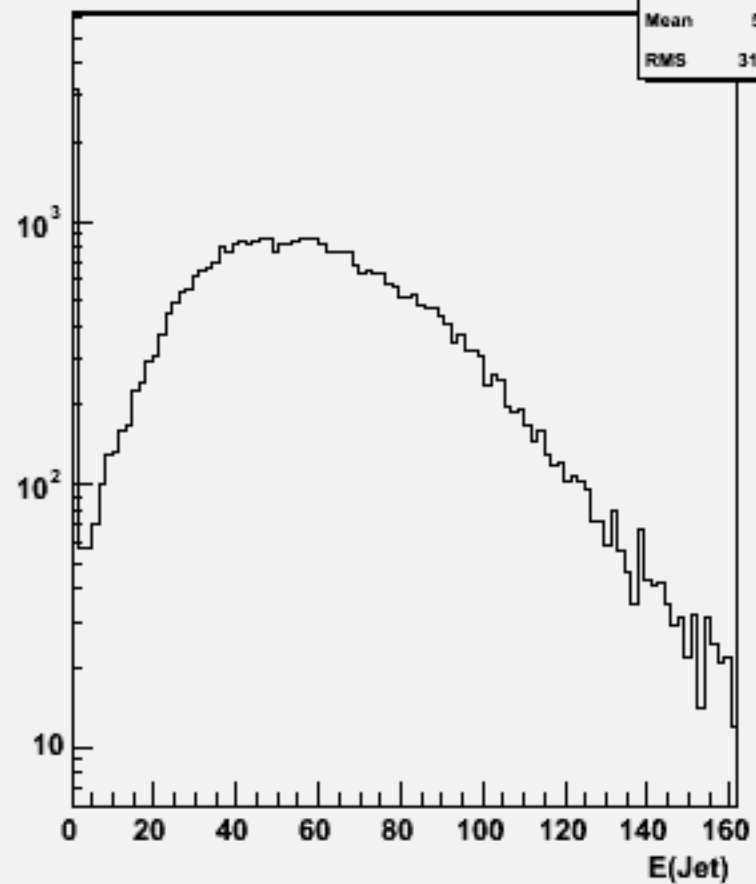
Jet energies(All jets)w101369 n1n1uddu_o
