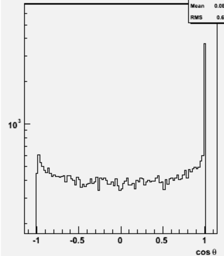
Jet cosθ (All jets)w101369 n1n1uddu_o
