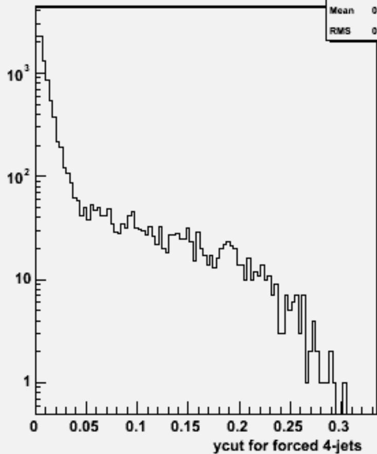
Ycut for 4-jets :w101369 n1n1uddu_o
