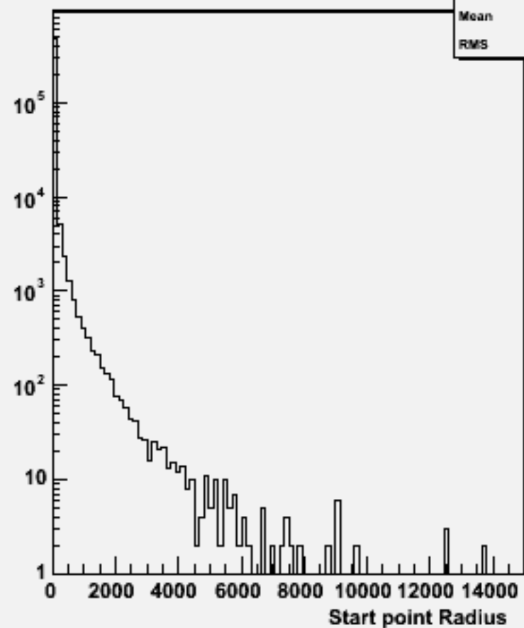
Start point R : w101364 n1n1ude3n3_o
