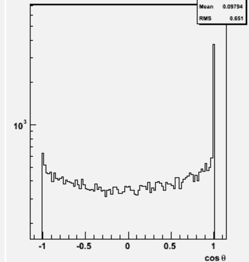
Jet cos \theta (All jets)w101364 n1n1ude3n3_o
