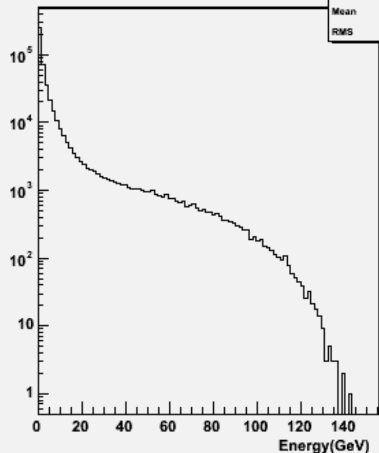
Start point R : w101364 n1n1ude3n3_o
