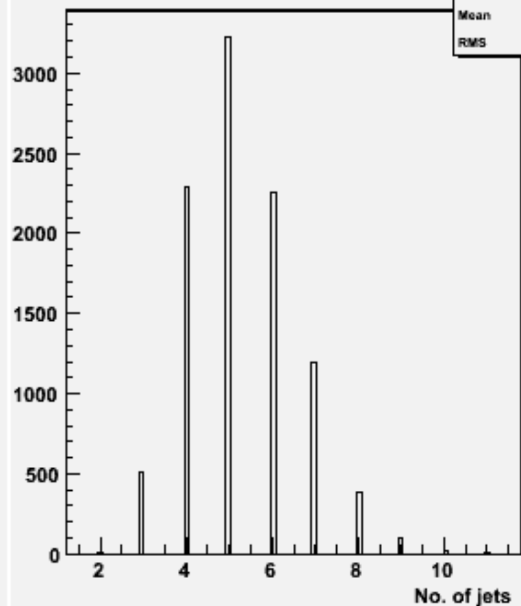
No. jets (ycut=0.001) : w101364 n1n1ude3n3_o
