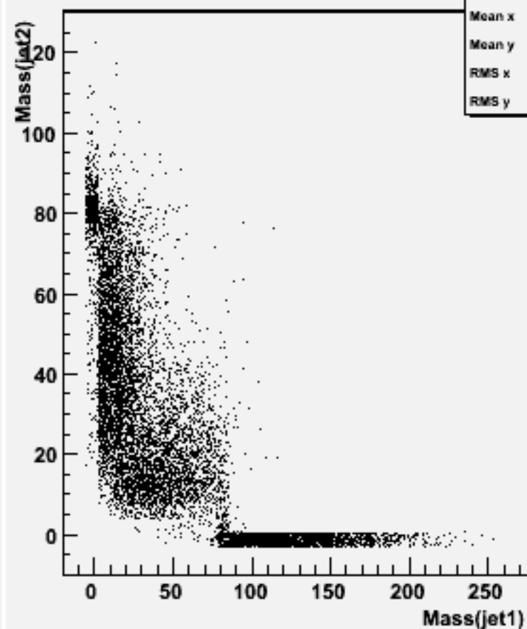
Jet mass for forced 2-jets : w101364 n1n1ude3n3_o
