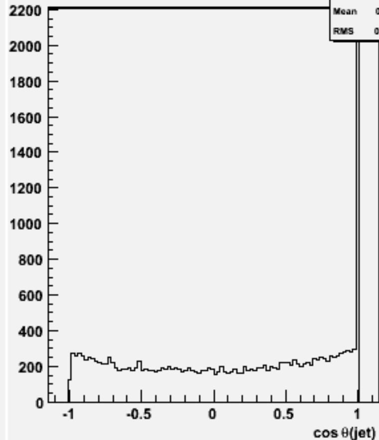
cos \theta for 2-jets :w101364 n1n1ude3n3_o
