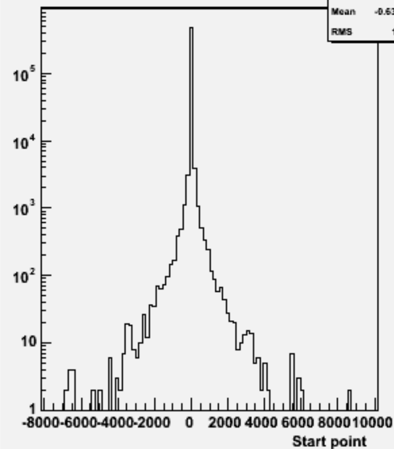
Start point Z : w101364 n1n1ude3n3_o
