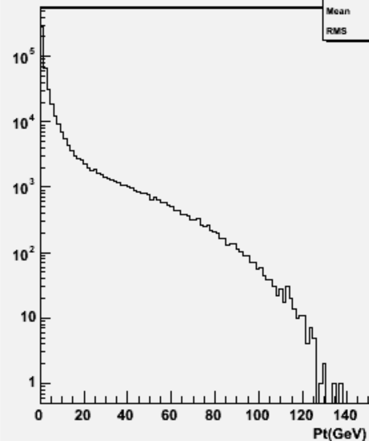
Start point Z : w101364 n1n1ude3n3_o
