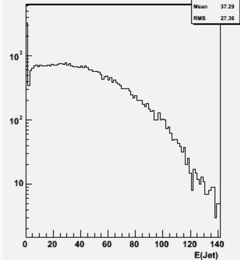
Jet energies(All jets)w101364 n1n1ude3n3_o
