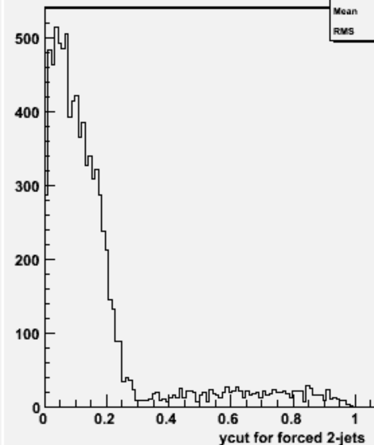
Ycut for 2-jets :w101364 n1n1ude3n3_o
