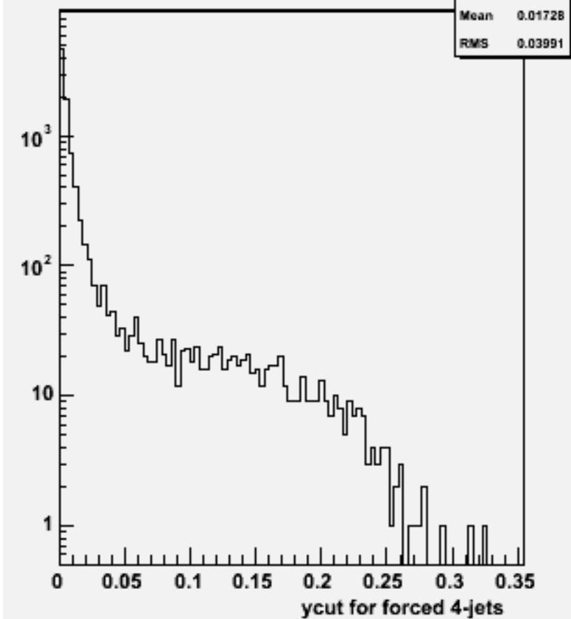
Ycut for 4-jets :w101364 n1n1ude3n3_o
