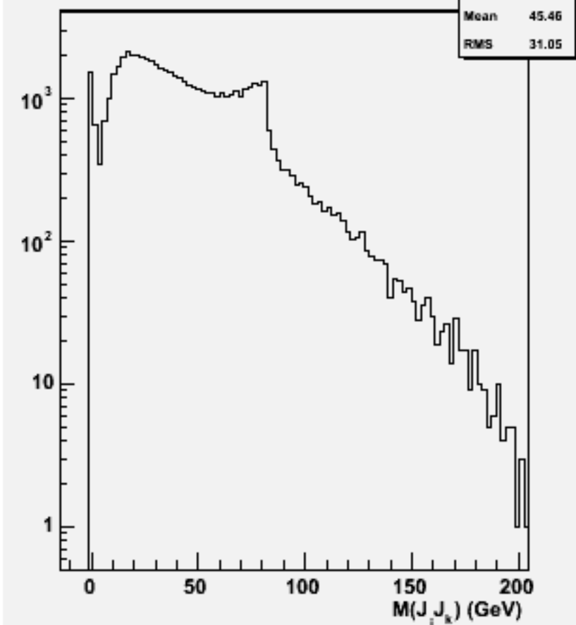
2jets mass(All comb)w101364 n1n1ude3n3_o
