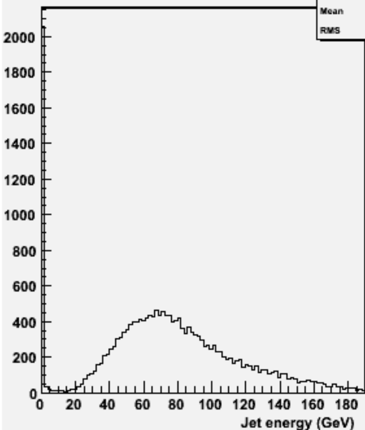
energy for 2-jets :w101364 n1n1ude3n3_o
