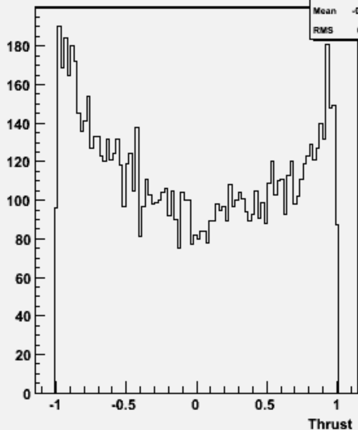
cos \Theta (thrust) w101364 n1n1ude3n3_o
