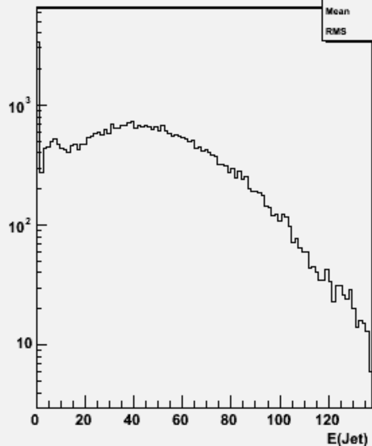
Jet energies(All jets)w101361 n1n1ude2n2_o
