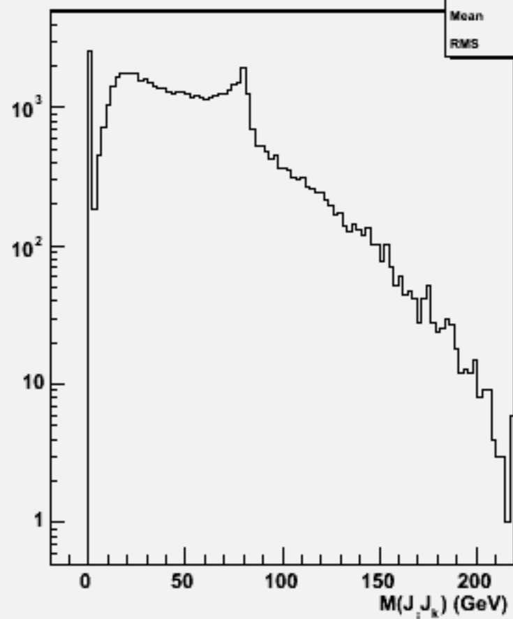
2jets mass(All comb)w101361 n1n1ude2n2_o
