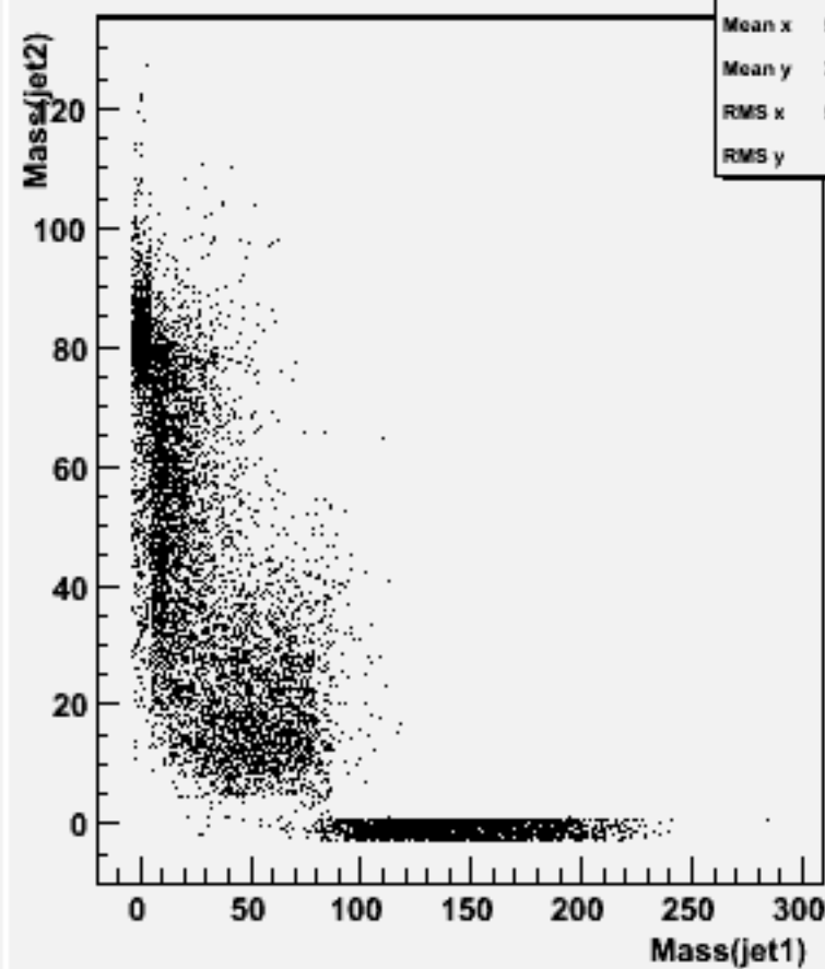
Jet mass for forced 2-jets : w101361 n1n1ude2n2_o
