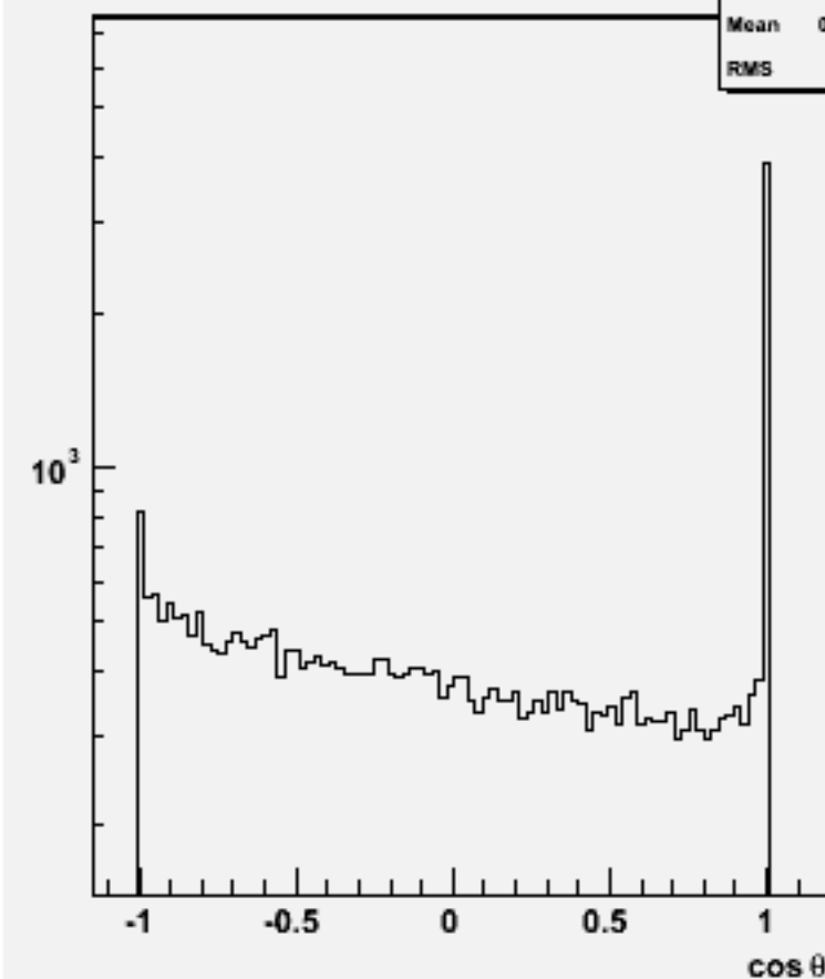
Jet cos \theta (All jets)w101361 n1n1ude2n2_o
