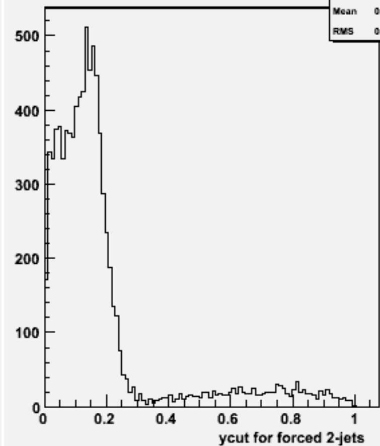
Ycut for 2-jets :w101361 n1n1ude2n2_o
