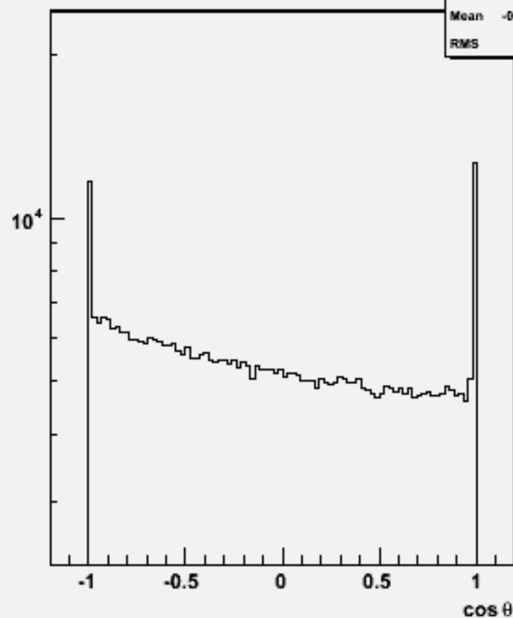
Particle cos \theta : w101361 n1n1ude2n2_o
