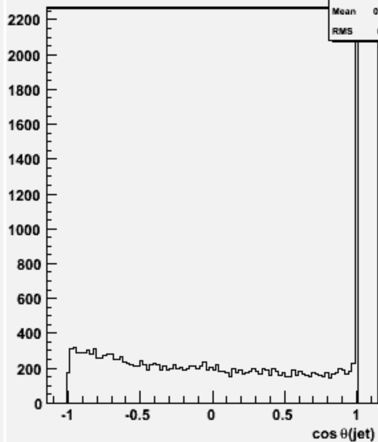
cos \theta for 2-jets :w101361 n1n1ude2n2_o
