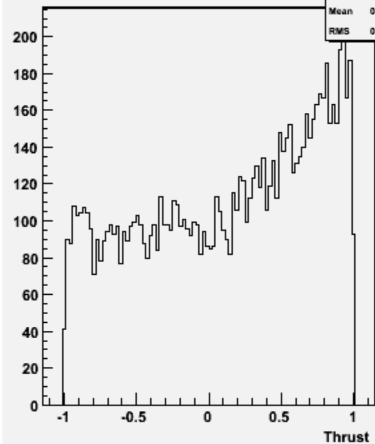
cos \Theta (thrust) w101361 n1n1ude2n2_o
