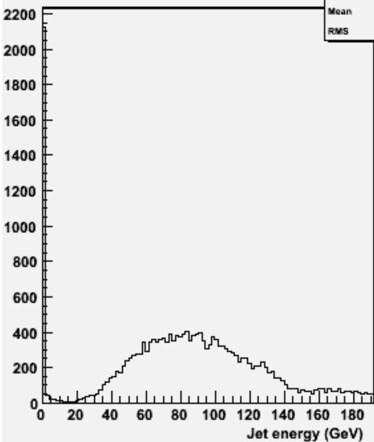
energy for 2-jets :w101361 n1n1ude2n2_o
