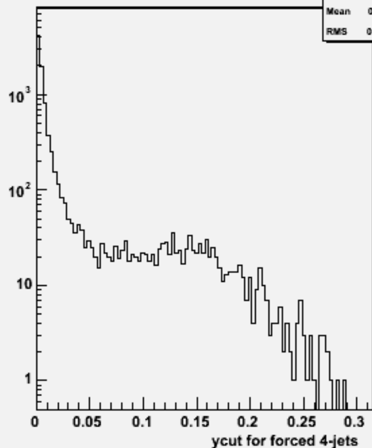
Ycut for 4-jets :w101361 n1n1ude2n2_o
