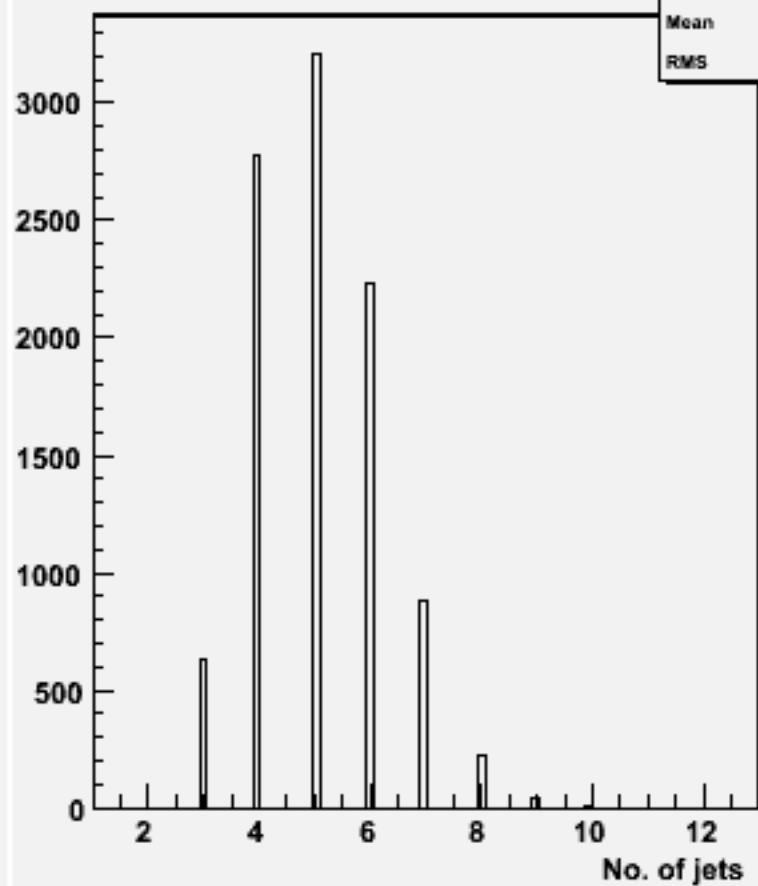
No. jets (ycut=0.001) : w101361 n1n1ude2n2_o
