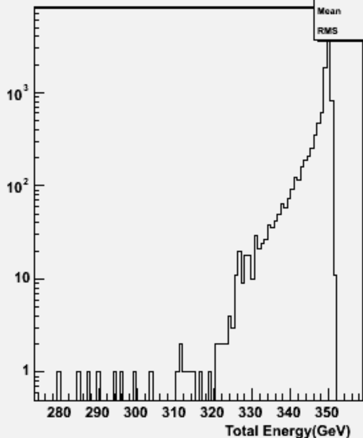
Total Energy (inc. \nu ): w101360 n1n1ude2n2_o
