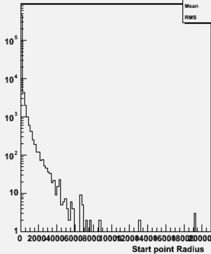
Start point R : w101360 n1n1ude2n2_o
