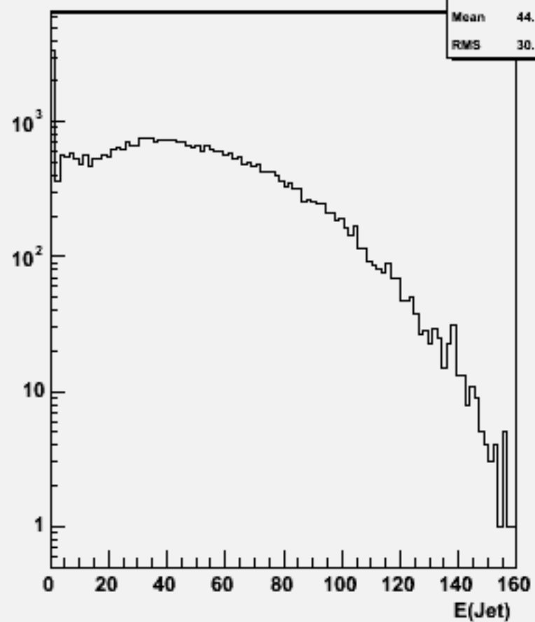
Jet energies(All jets)w101360 n1n1ude2n2_o
