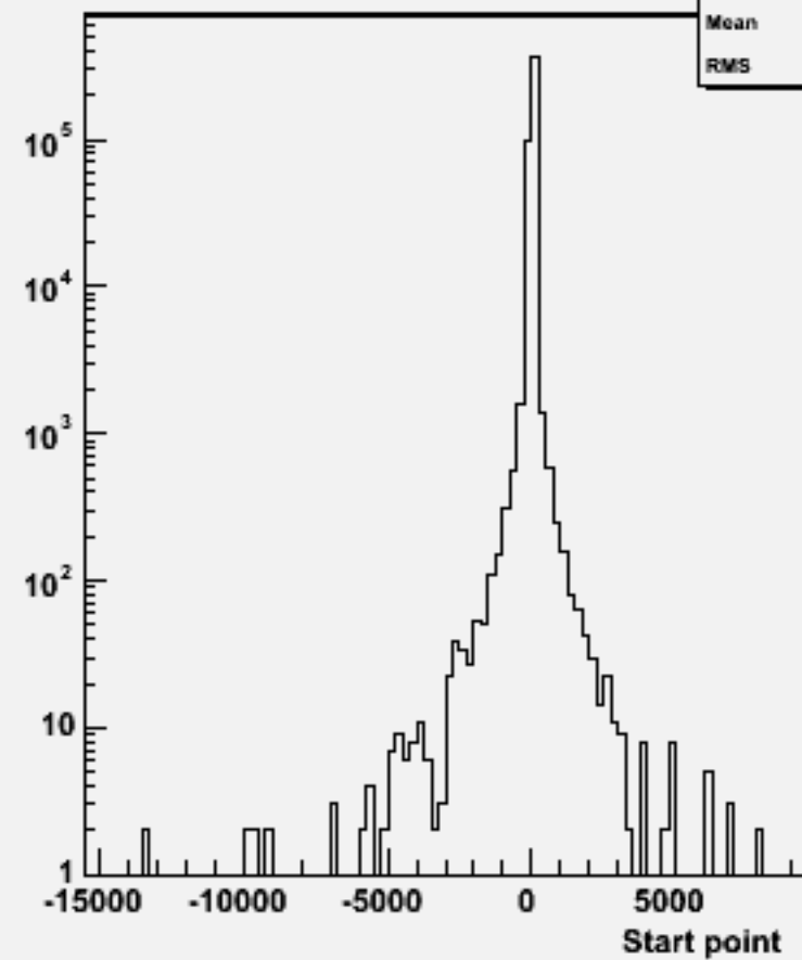
Start point Z : w101360 n1n1ude2n2_o
