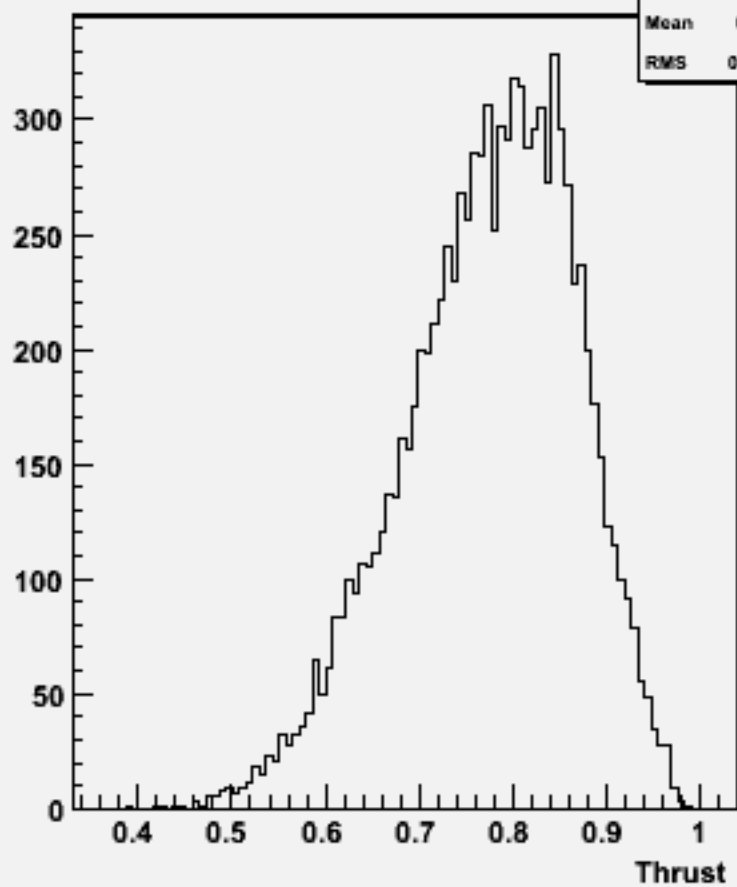
Thrust w101360 n1n1ude2n2_o
