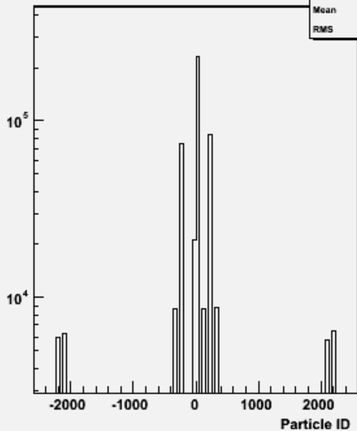
Particle ID : w101360 n1n1ude2n2_o
