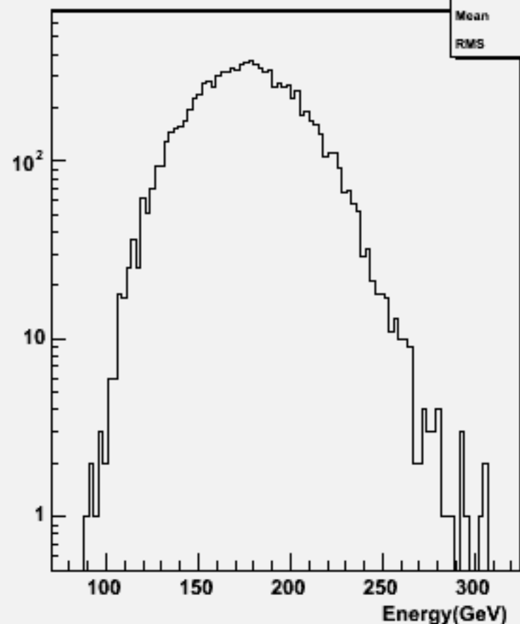
Total Energy (w/o \nu ): w101360 n1n1ude2n2_o
