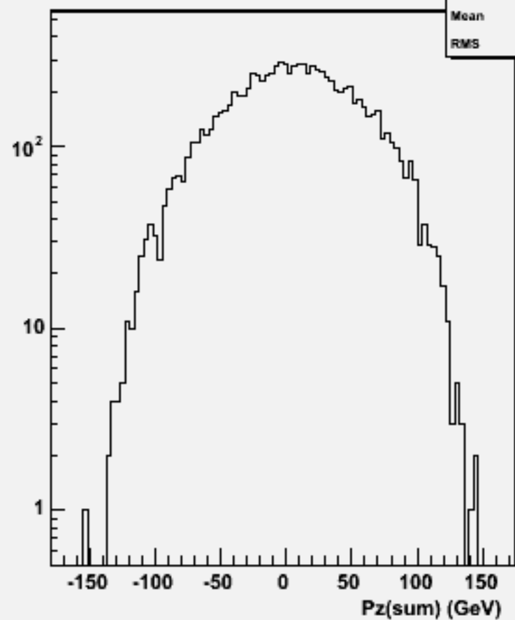
Pz Sum: w101360 n1n1ude2n2_o
