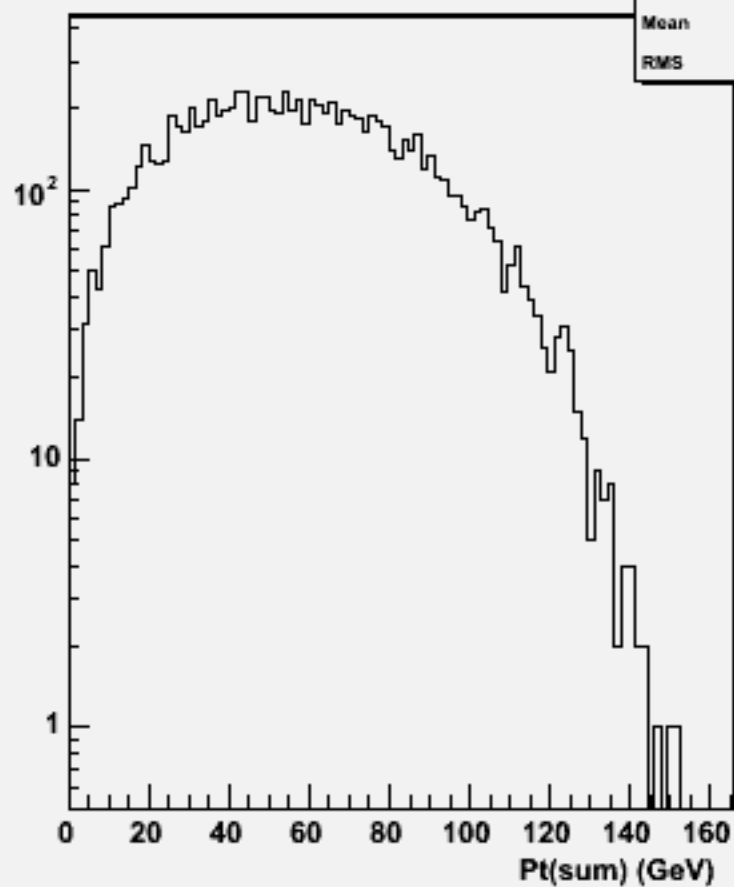
Pt Sum: w101360 n1n1ude2n2_o
