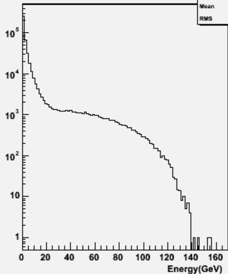
Particle Energy : w101360 n1n1ude2n2_o
