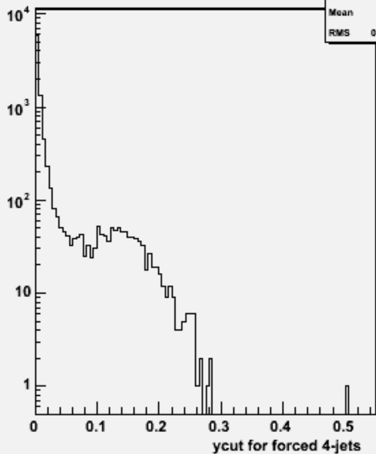
Ycut for 4-jets :w101360 n1n1ude2n2_o
