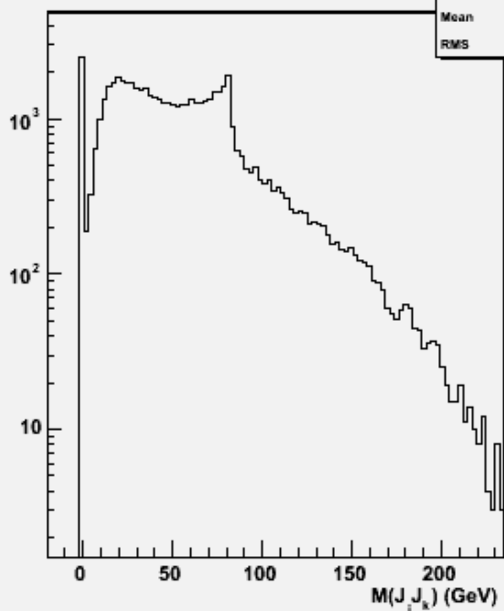
2jets mass(All comb)w101360 n1n1ude2n2_o
