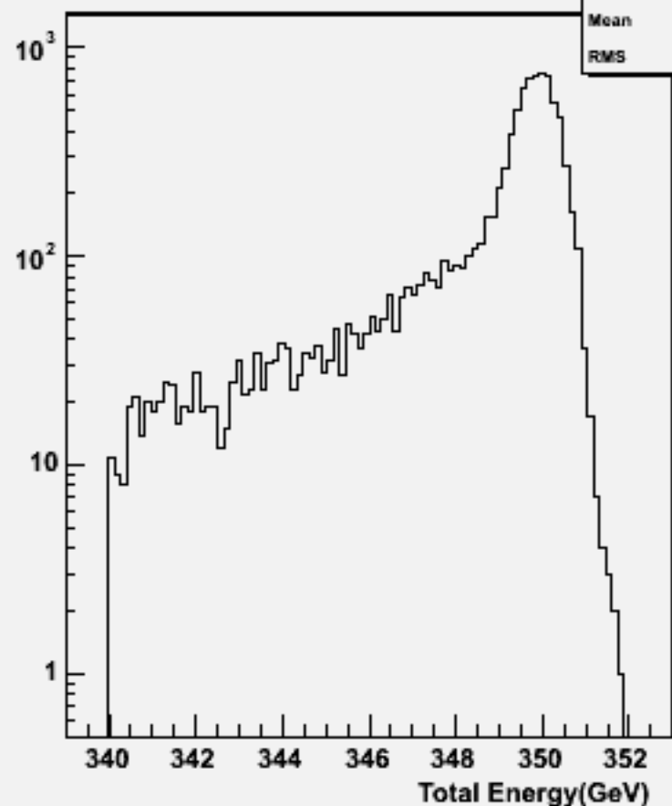
Total Energy (inc. \nu ): w101360 n1n1ude2n2_o
