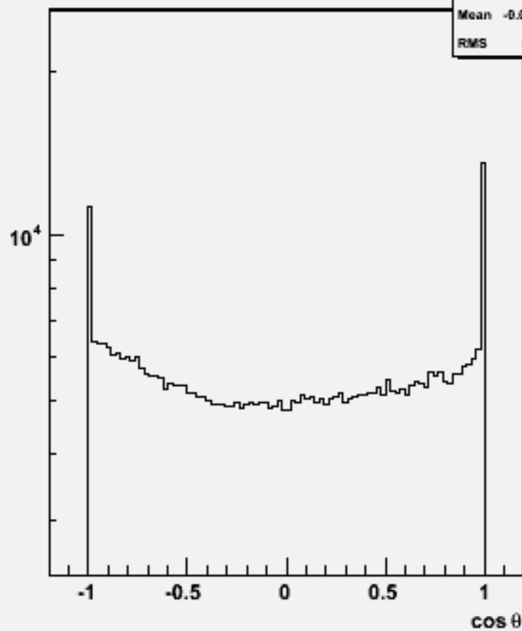
Particle \cos\theta : w101360 n1n1ude2n2_o
