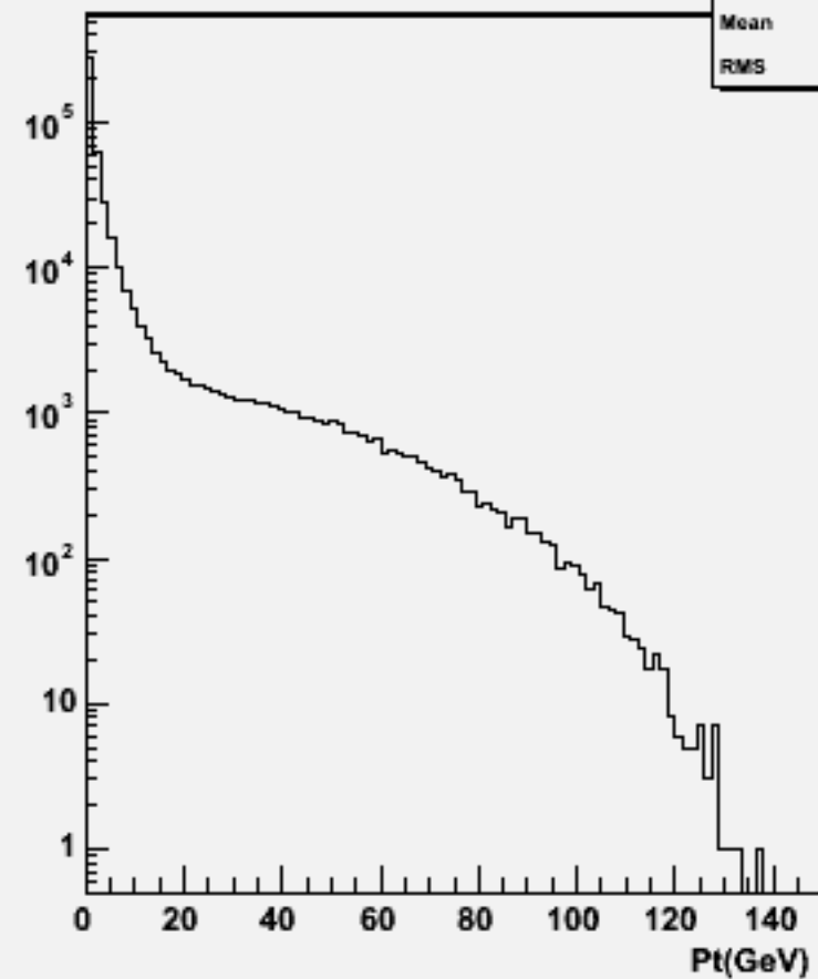
Particle Pt : w101360 n1n1ude2n2_o
