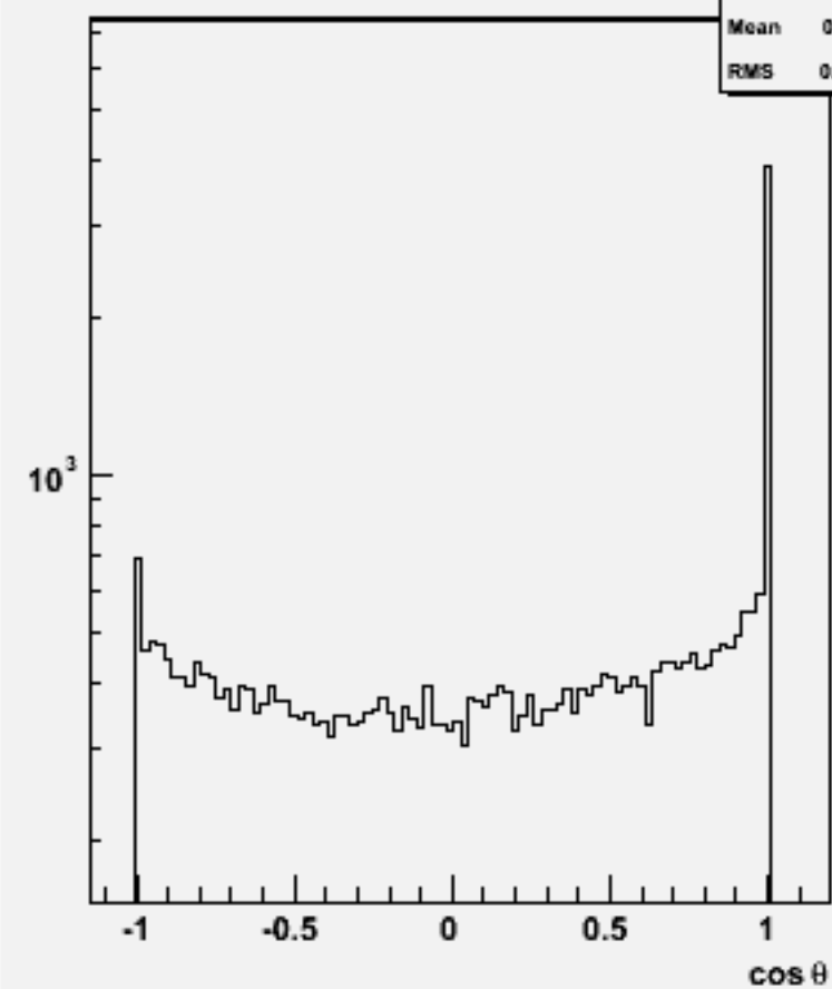
Jet cos \theta (All jets)w101360 n1n1ude2n2_o
