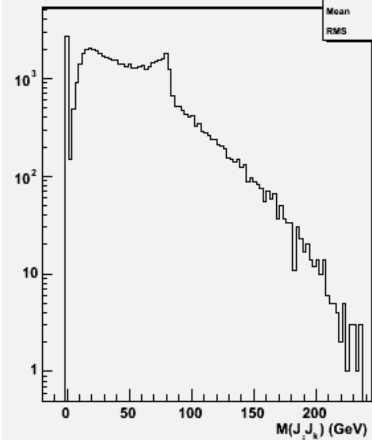
2jets mass(All comb)w101356 n1n1ude1n1_o
