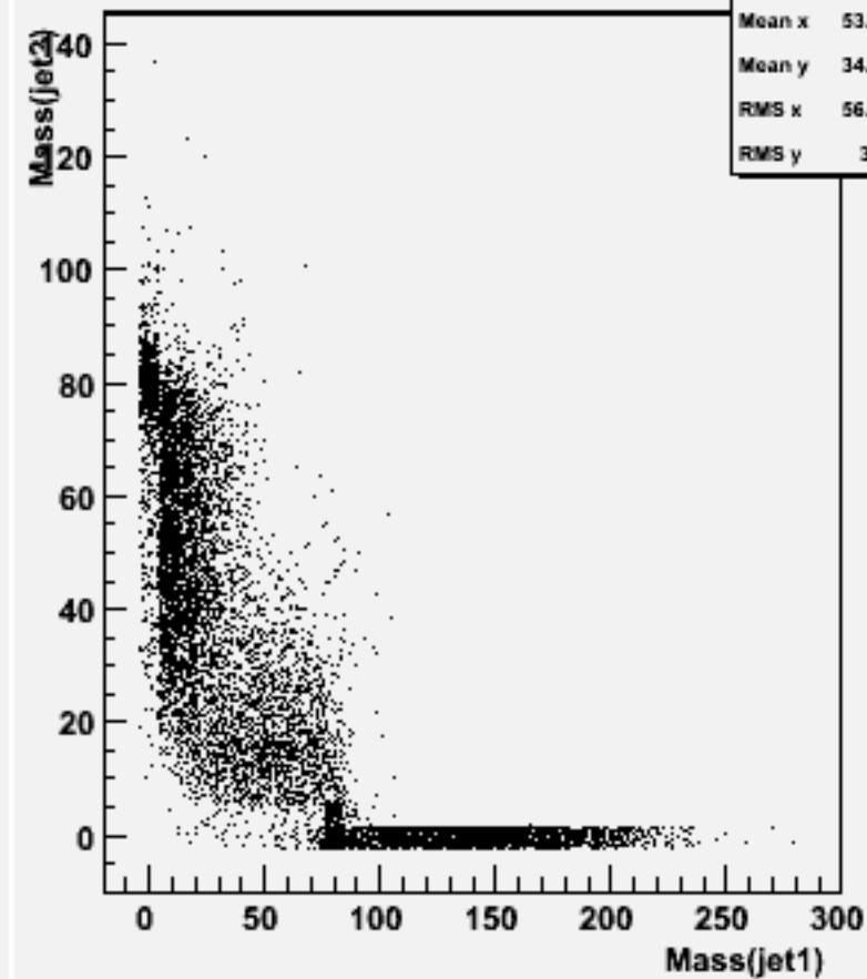
Jet mass for forced 2-jets : w101356 n1n1ude1n1_o
