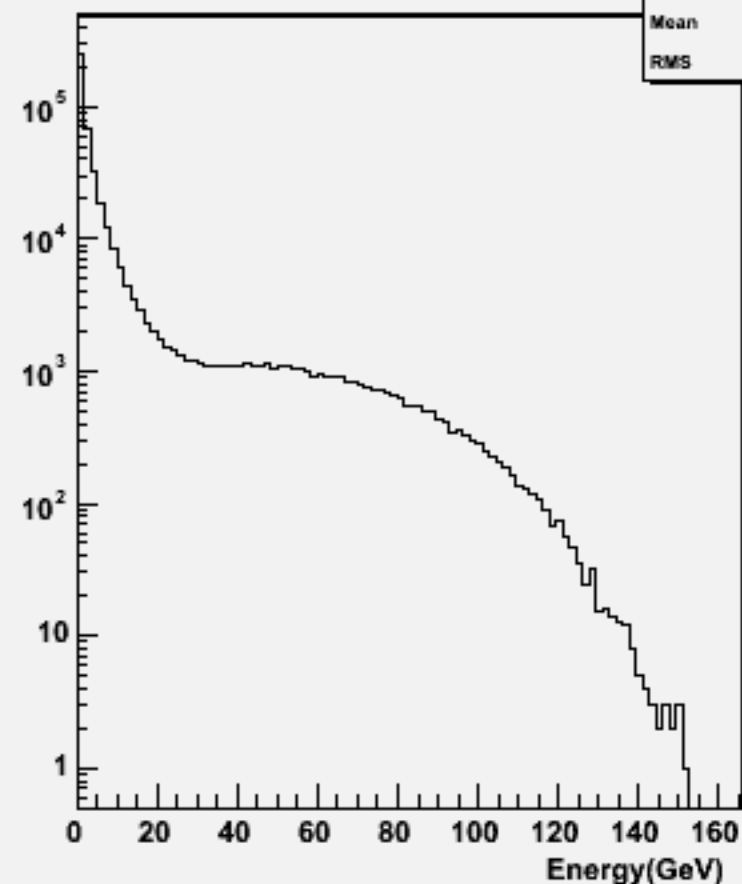
Start point R : w101356 n1n1ude1n1_o
