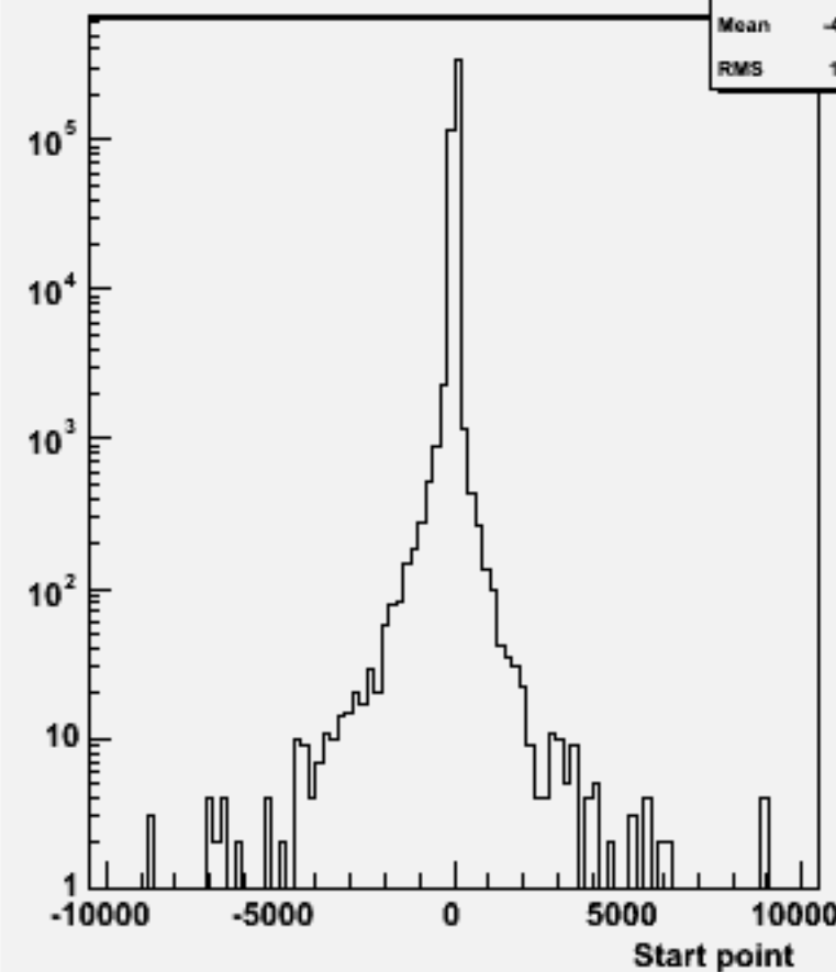
Start point Z : w101356 n1n1ude1n1_o
