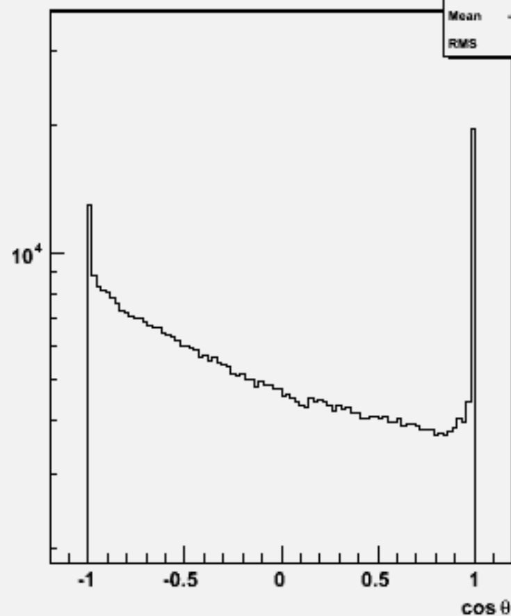
Particle cosθ : w101356 n1n1ude1n1_o
