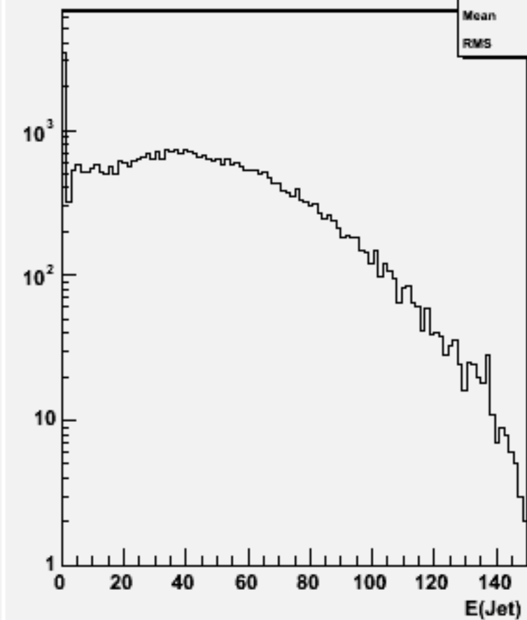
Jet energies(All jets)w101356 n1n1ude1n1_o
