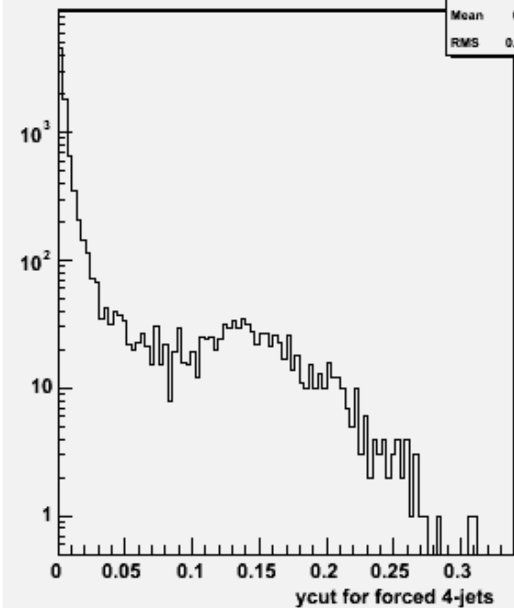
Ycut for 4-jets :w101356 n1n1ude1n1_o
