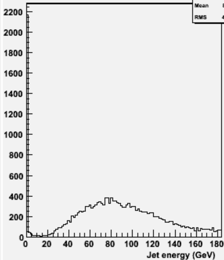
energy for 2-jets :w101356 n1n1ude1n1_o
