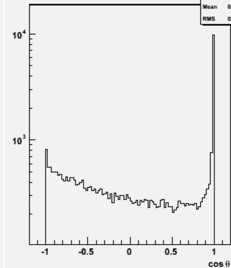
Jet cos \theta (All jets)w101356 n1n1ude1n1_o
