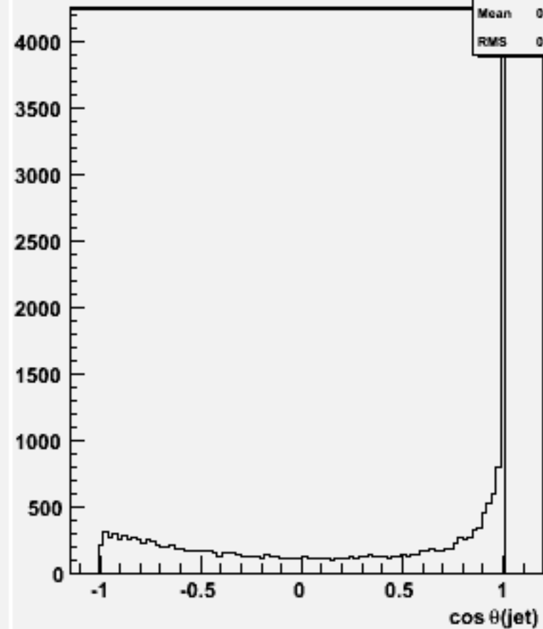
cos \theta for 2-jets :w101356 n1n1ude1n1_o
