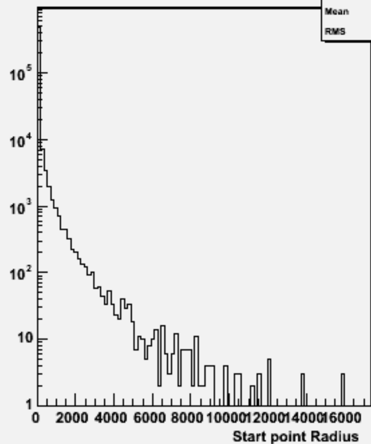
Start point R : w101353 n1n1n3e3sc_o
