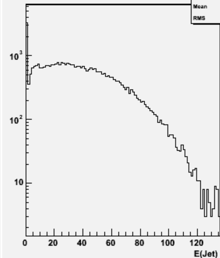
Jet energies(All jets)w101353 n1n1n3e3sc_o
