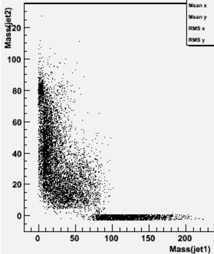
Jet mass for forced 2-jets : w101353 n1n1n3e3sc_o
