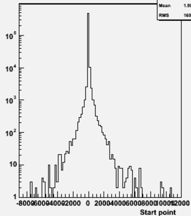
Start point Z : w101353 n1n1n3e3sc_o
