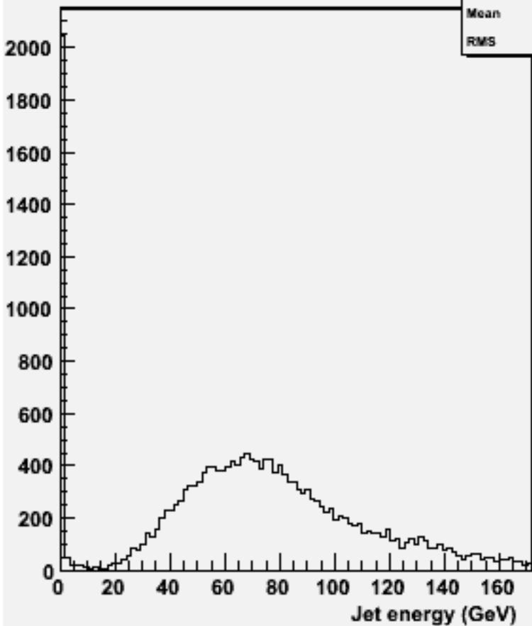
energy for 2-jets :w101353 n1n1n3e3sc_o
