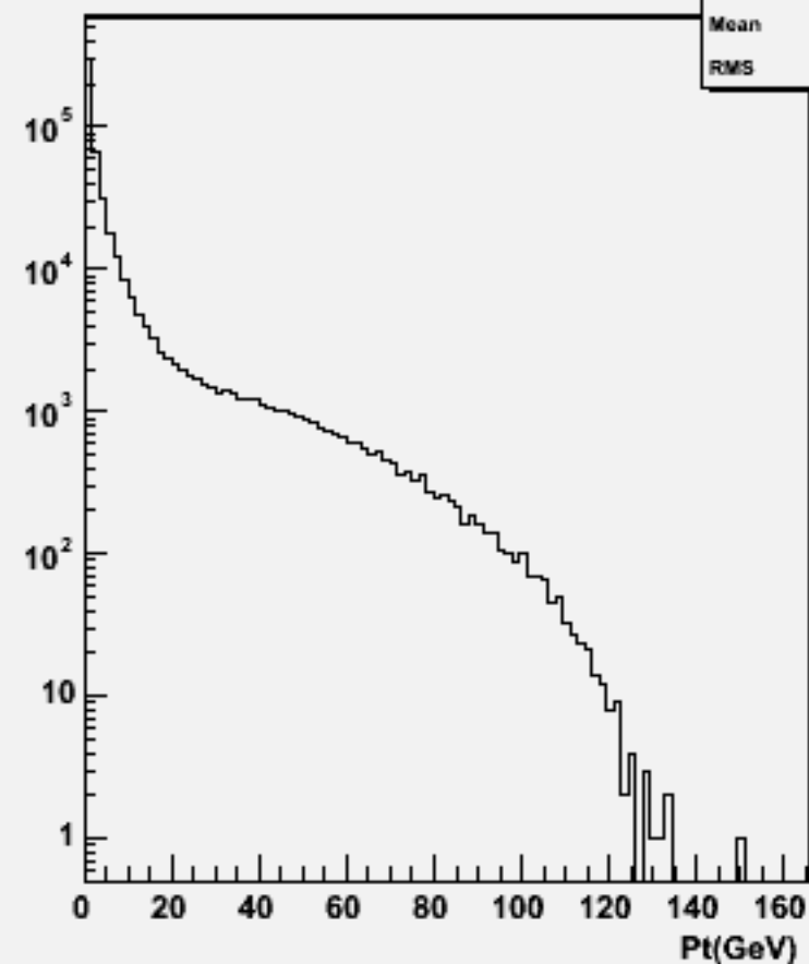
Particle Pt : w101353 n1n1n3e3sc_o
