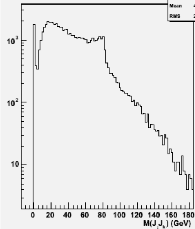
2jets mass(All comb)w101353 n1n1n3e3sc_o
