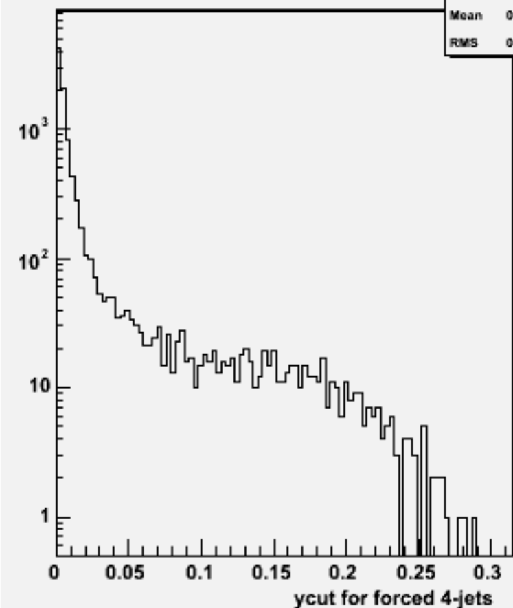
Ycut for 4-jets :w101353 n1n1n3e3sc_o
