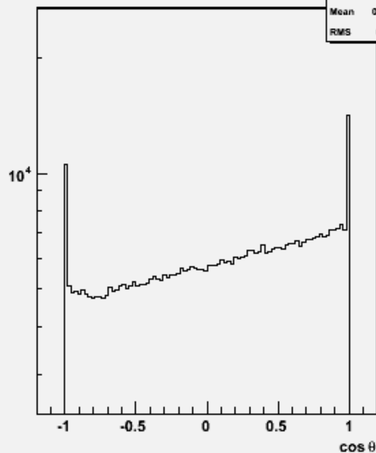
Particle cosθ : w101353 n1n1n3e3sc_o
