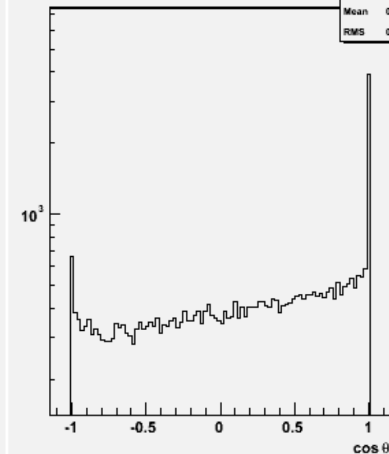
Jet cos \theta (All jets)w101353 n1n1n3e3sc_o
