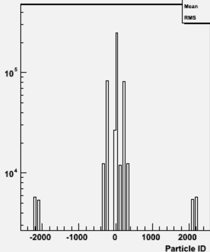
Particle ID : w101353 n1n1n3e3sc_o
