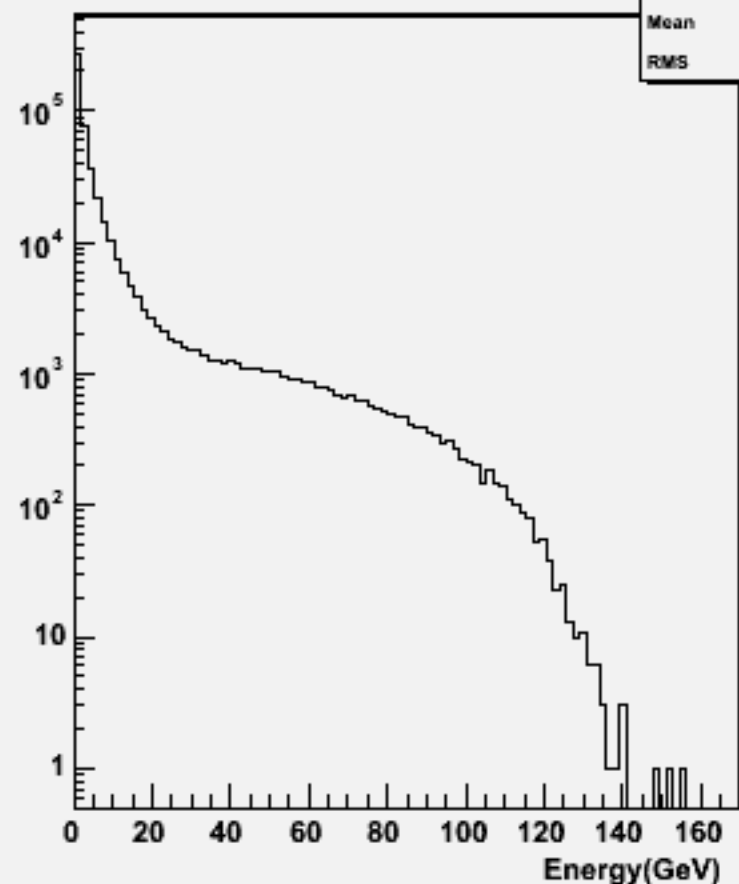
Particle Energy : w101353 n1n1n3e3sc_o
