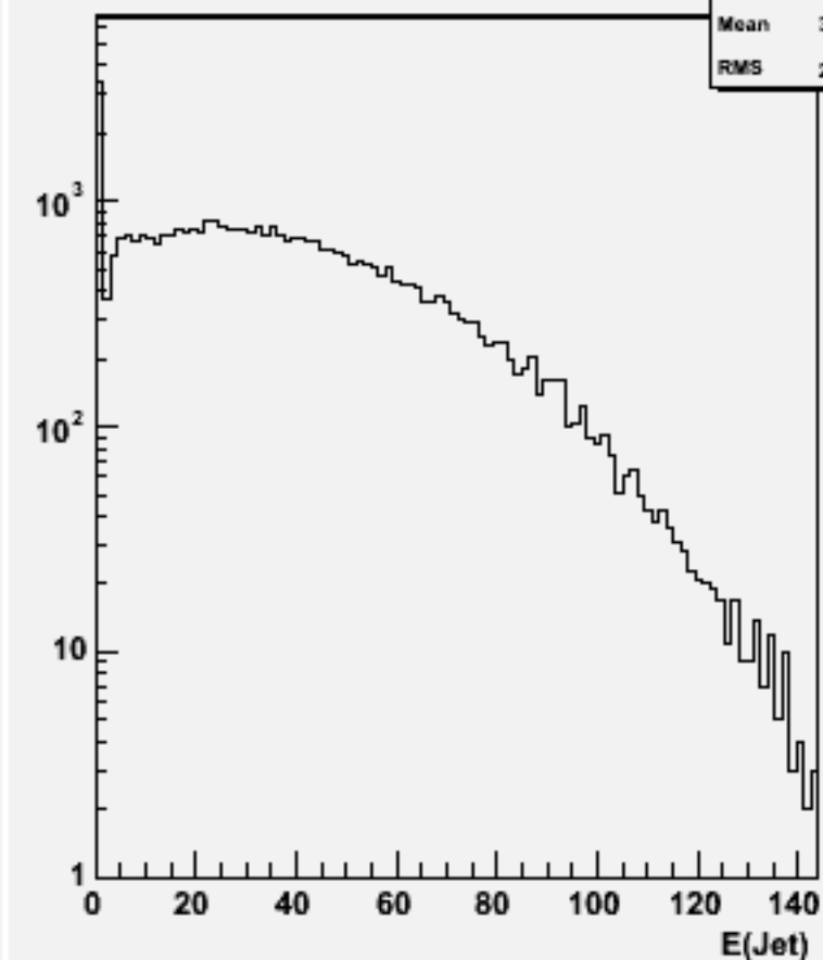
Jet energies(All jets)w101352 n1n1n3e3sc_o
