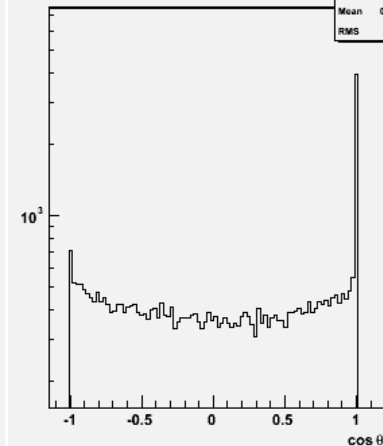
Jet cos \theta (All jets)w101352 n1n1n3e3sc_o
