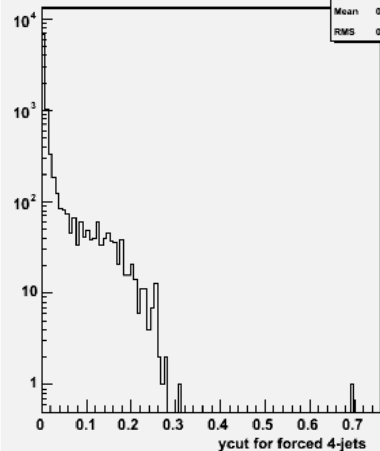
Ycut for 4-jets :w101352 n1n1n3e3sc_o
