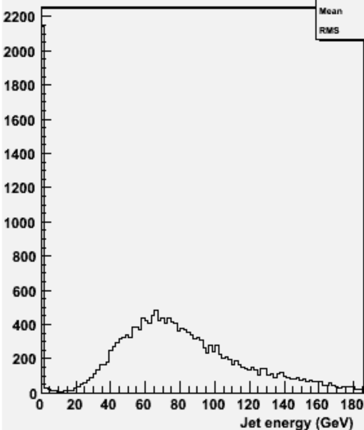
energy for 2-jets :w101352 n1n1n3e3sc_o
