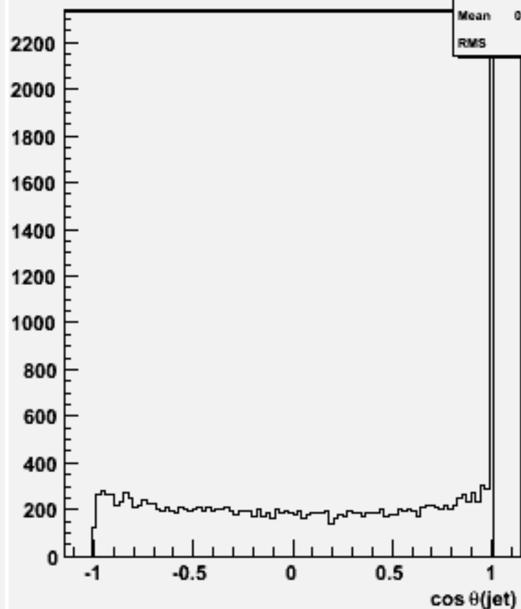
cos \theta for 2-jets :w101352 n1n1n3e3sc_o
