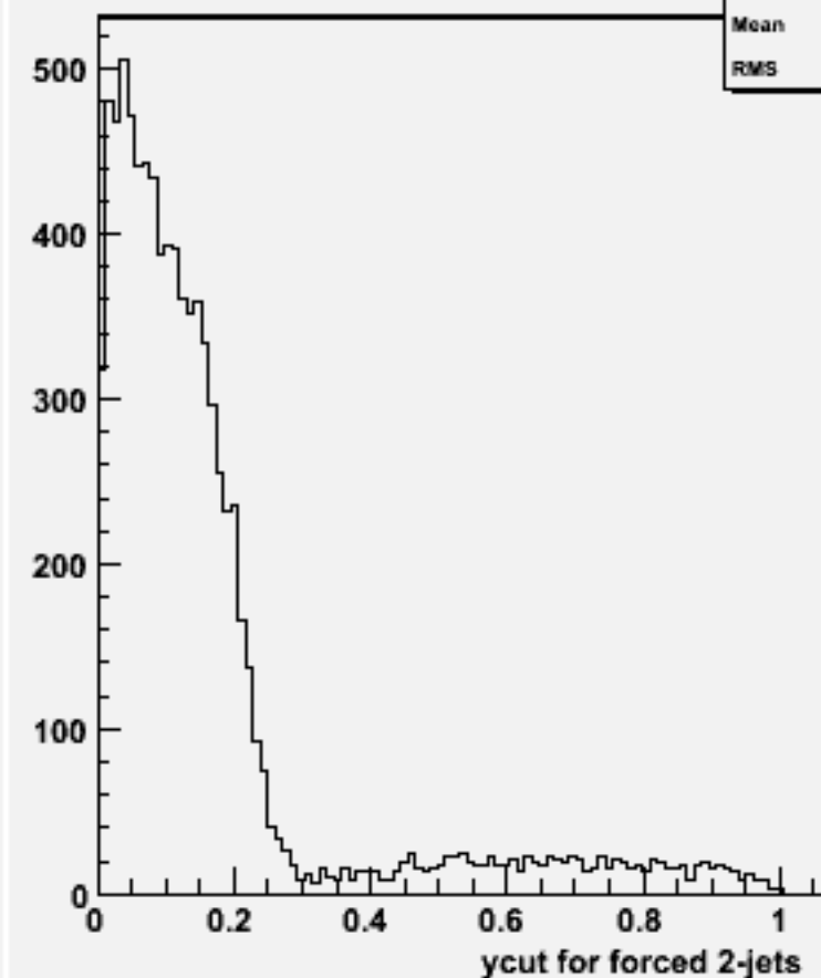
Ycut for 2-jets :w101352 n1n1n3e3sc_o
