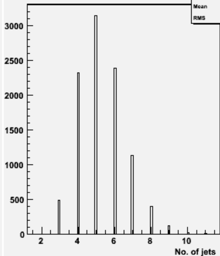
No. jets (ycut=0.001) : w101352 n1n1n3e3sc_o
