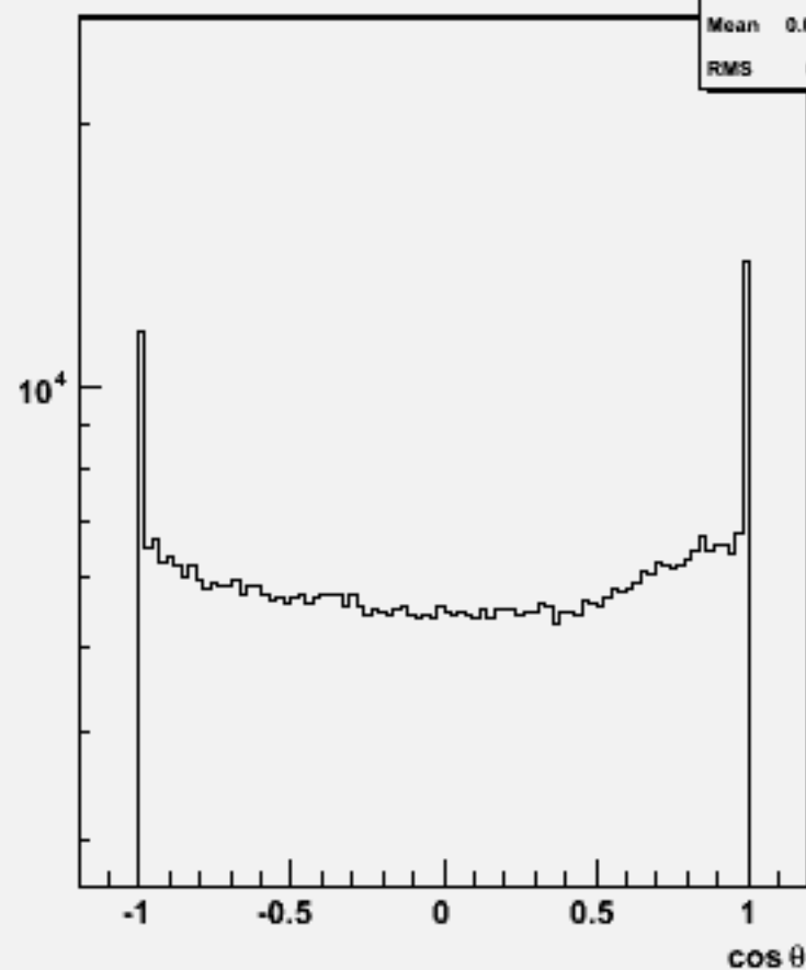
Particle cosθ : w101352 n1n1n3e3sc_o
