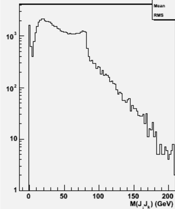
2jets mass(All comb)w101352 n1n1n3e3sc_o
