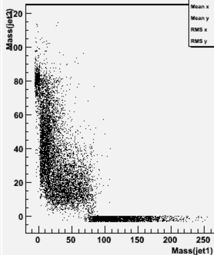
Jet mass for forced 2-jets : w101352 n1n1n3e3sc_o
