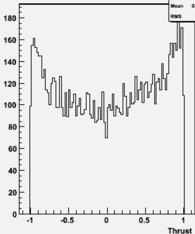
cos \Theta (thrust) w101352 n1n1n3e3sc_o
