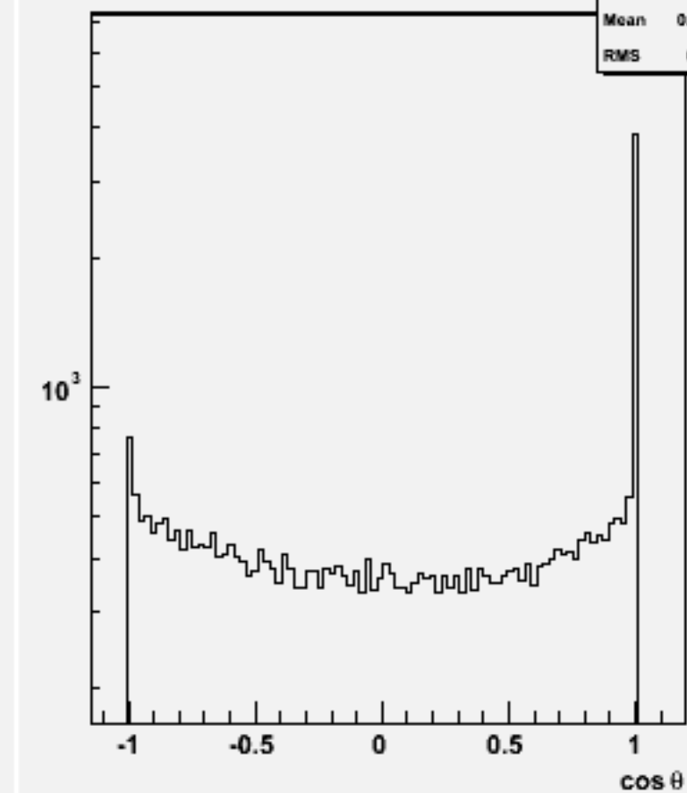
Jet cos \theta (All jets)w101348 n1n1n3e3du_o
