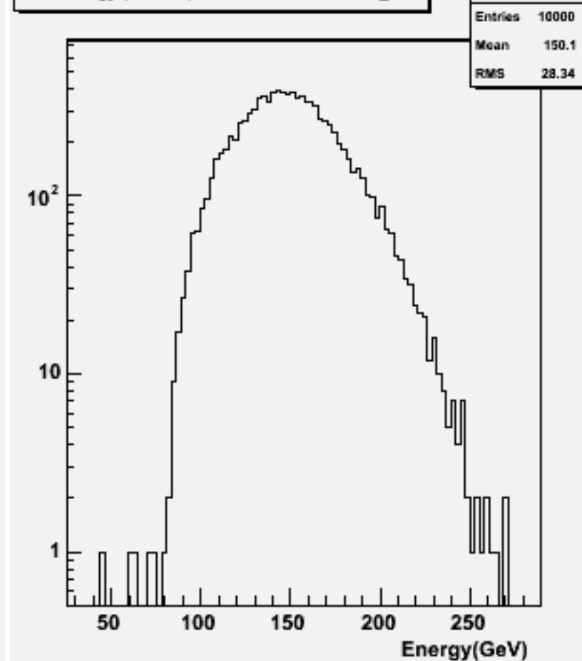
Total Energy (w/o \nu ): w101348 n1n1n3e3du_o
