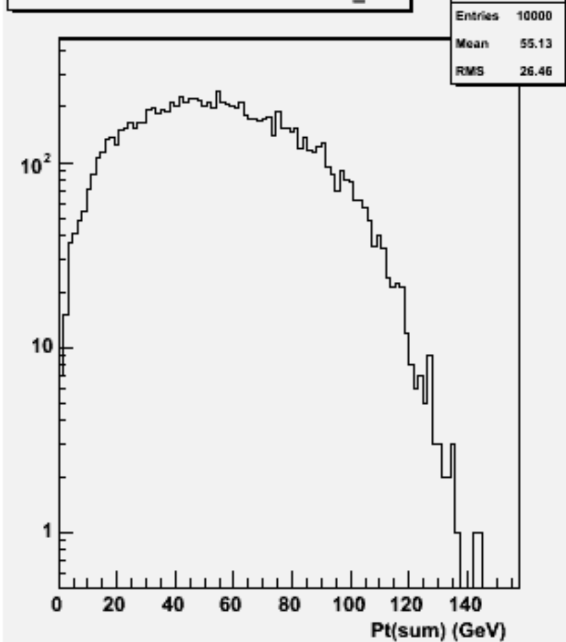
Pt Sum: w101348 n1n1n3e3du_o
