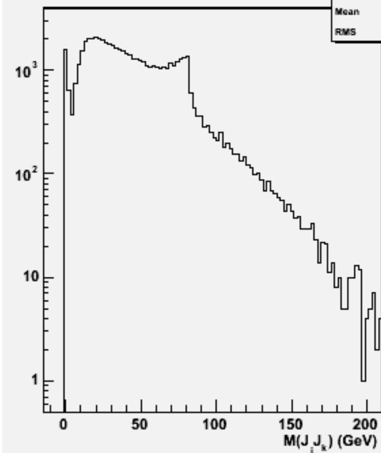
2jets mass(All comb)w101348 n1n1n3e3du_o
