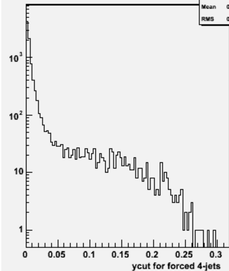
Ycut for 4-jets :w101348 n1n1n3e3du_o
