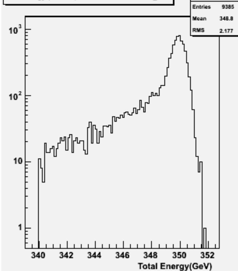
Total Energy (Inc. \nu ): w101348 n1n1n3e3du_o
