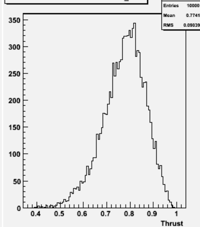
Thrust w101348 n1n1n3e3du_o
