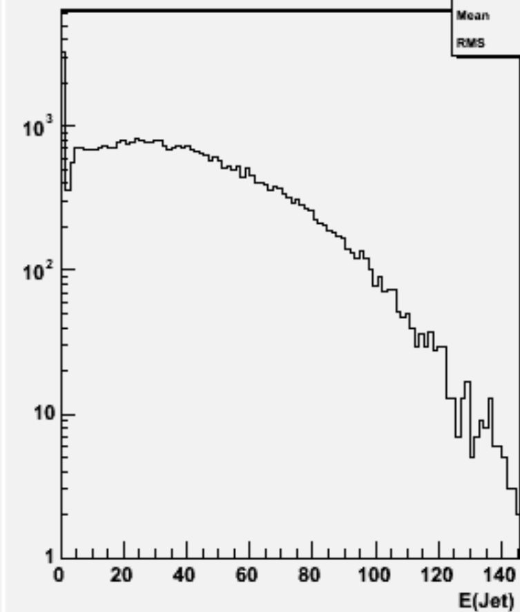
Jet energies(All jets)w101348 n1n1n3e3du_o
