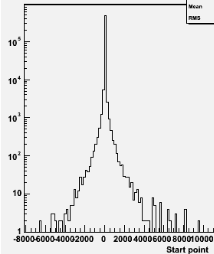
Start point Z : w101348 n1n1n3e3du_o
