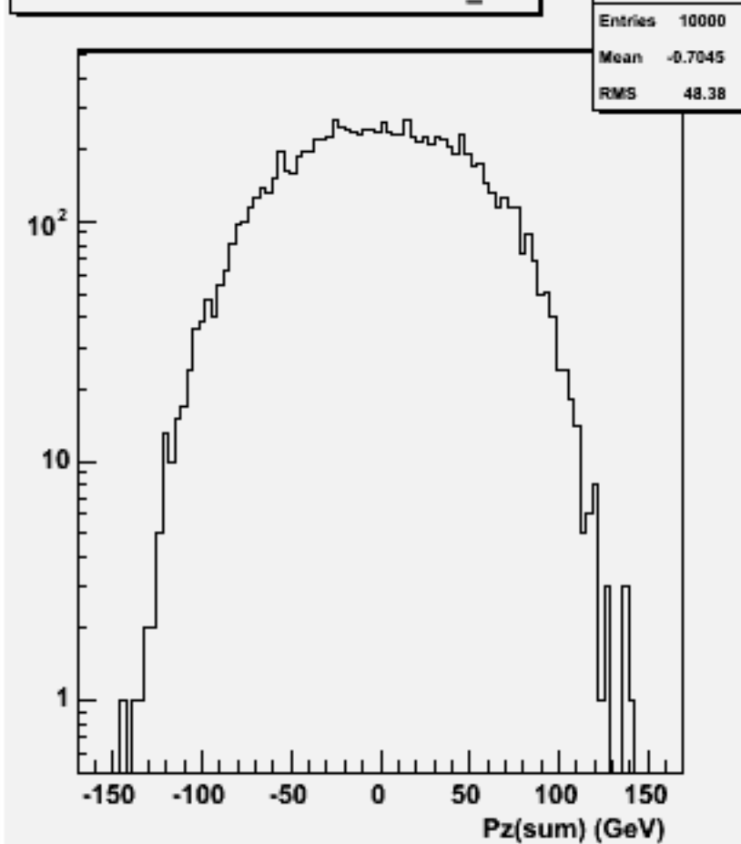
Pz Sum: w101348 n1n1n3e3du_o
