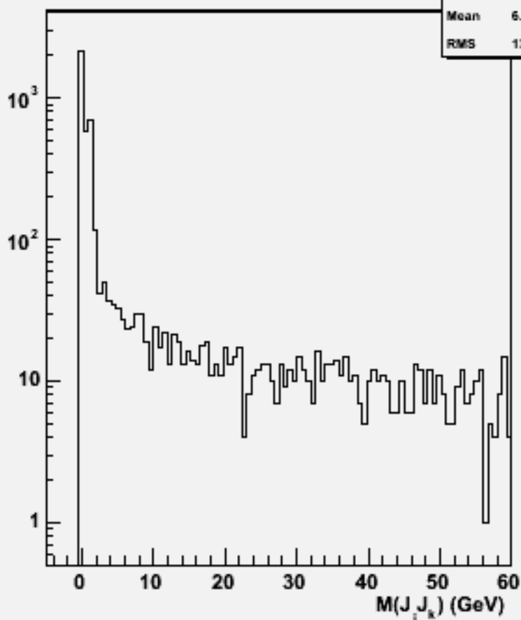
2jets mass(All comb)w101338 n1n1n3e3e1n1_o
