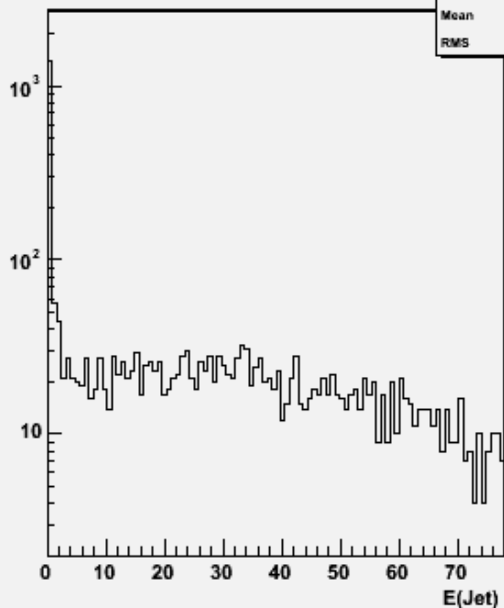
Jet energies(All jets)w101338 n1n1n3e3e1n1_o
