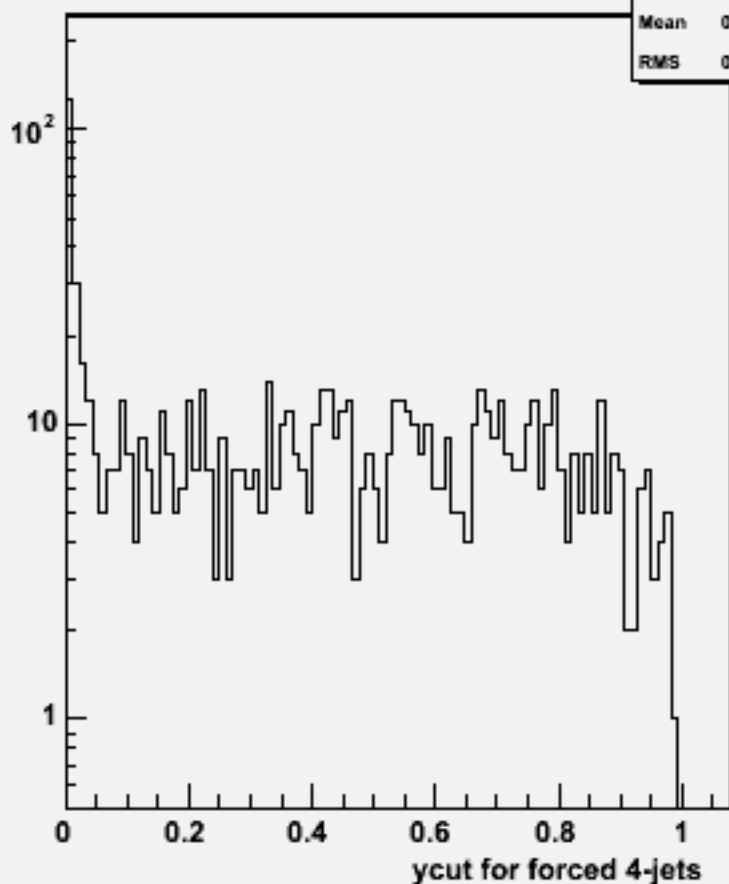
Ycut for 4-jets :w101338 n1n1n3e3e1n1_o
