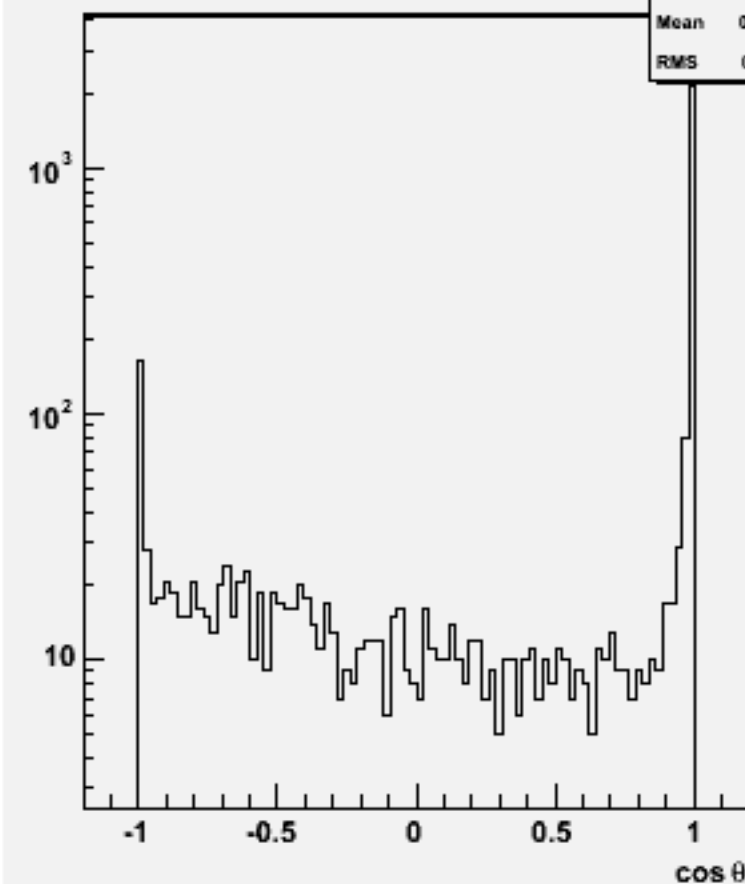
Jet cos \theta (All jets)w101338 n1n1n3e3e1n1_o
