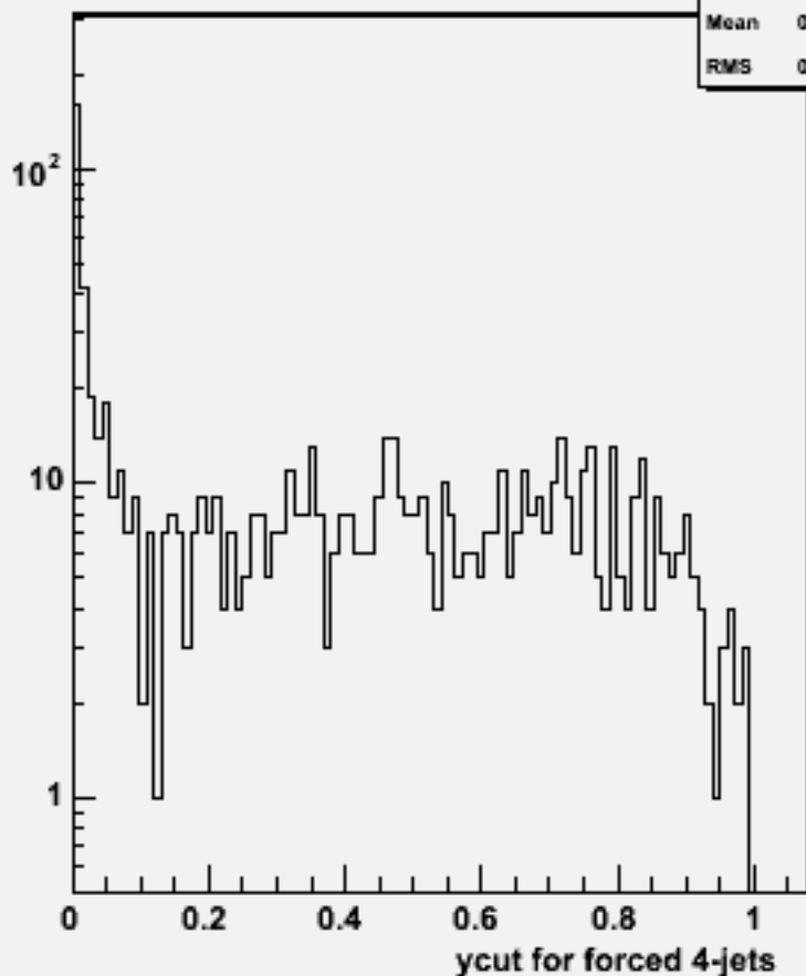
Ycut for 4-jets :w101336 n1n1n3e3e1n1_o
