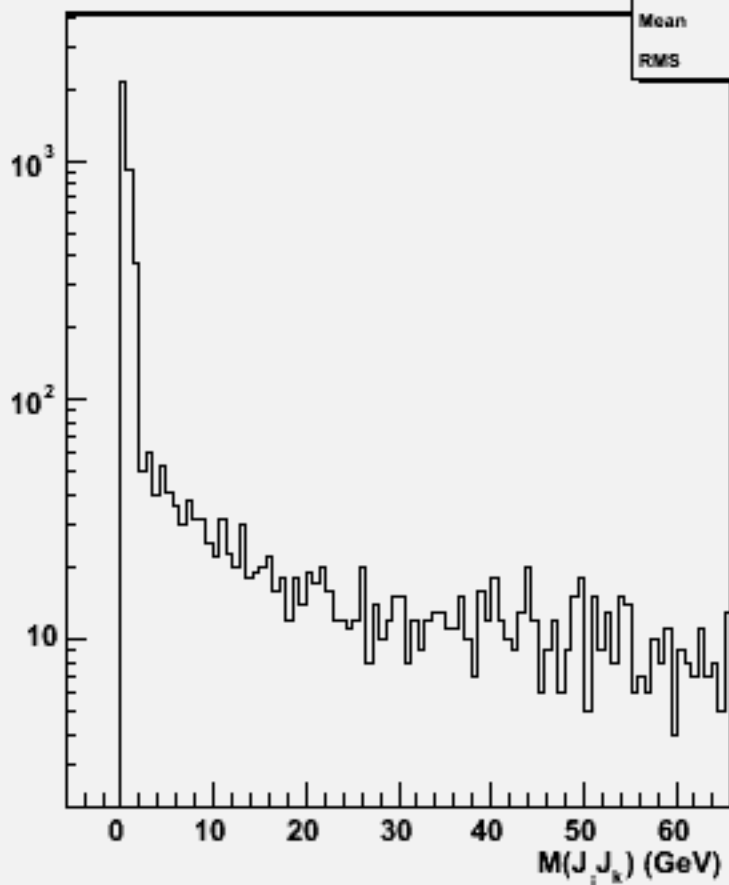
2jets mass(All comb)w101336 n1n1n3e3e1n1_o
