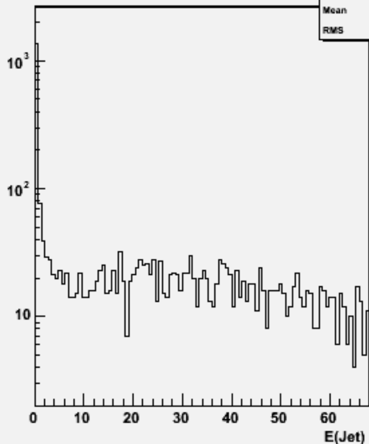
Jet energies(All jets)w101336 n1n1n3e3e1n1_o
