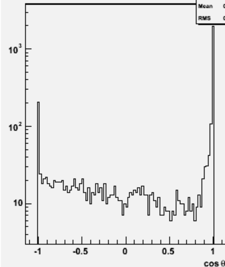
Jet cos \theta (All jets)w101336 n1n1n3e3e1n1_o
