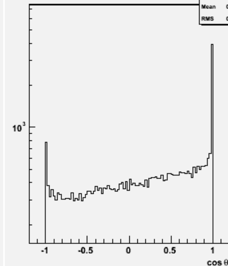
Jet cos \theta (All jets)w101333 n1n1n2e2sc_o
