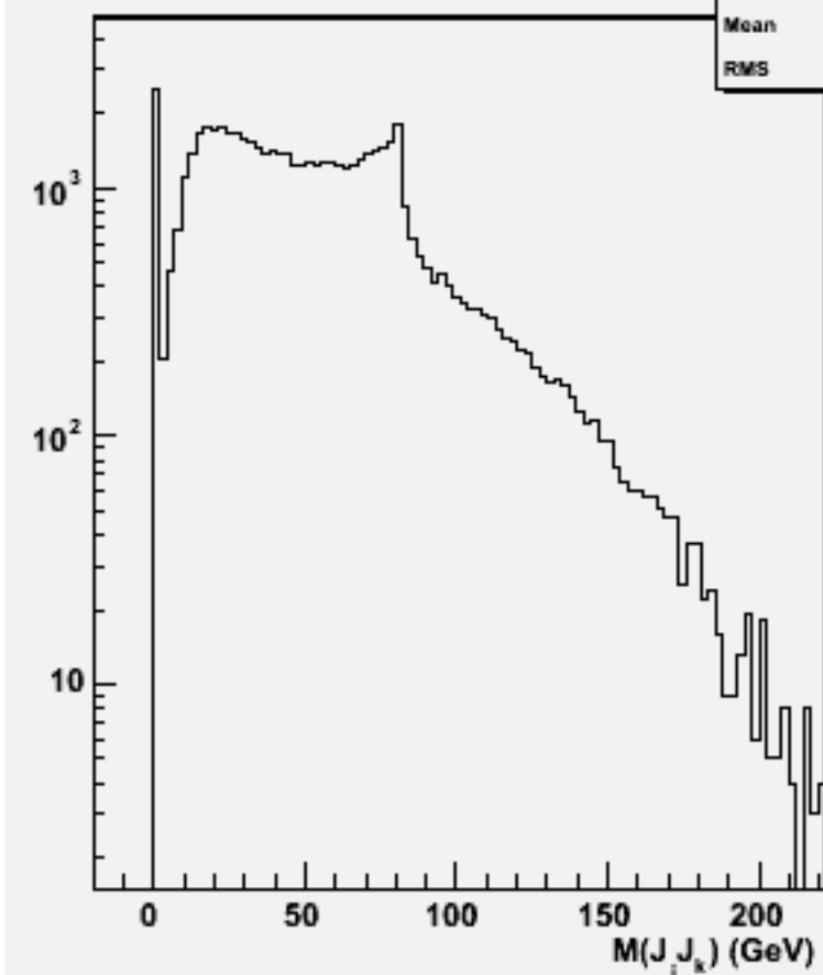
2jets mass(All comb)w101333 n1n1n2e2sc_o
