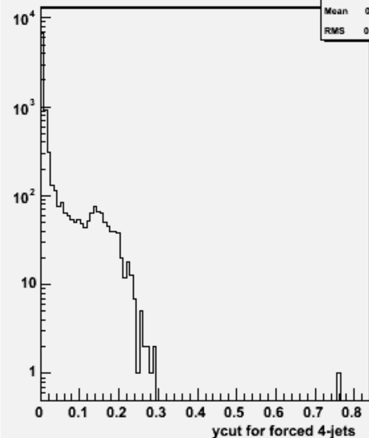
Ycut for 4-jets :w101333 n1n1n2e2sc_o
