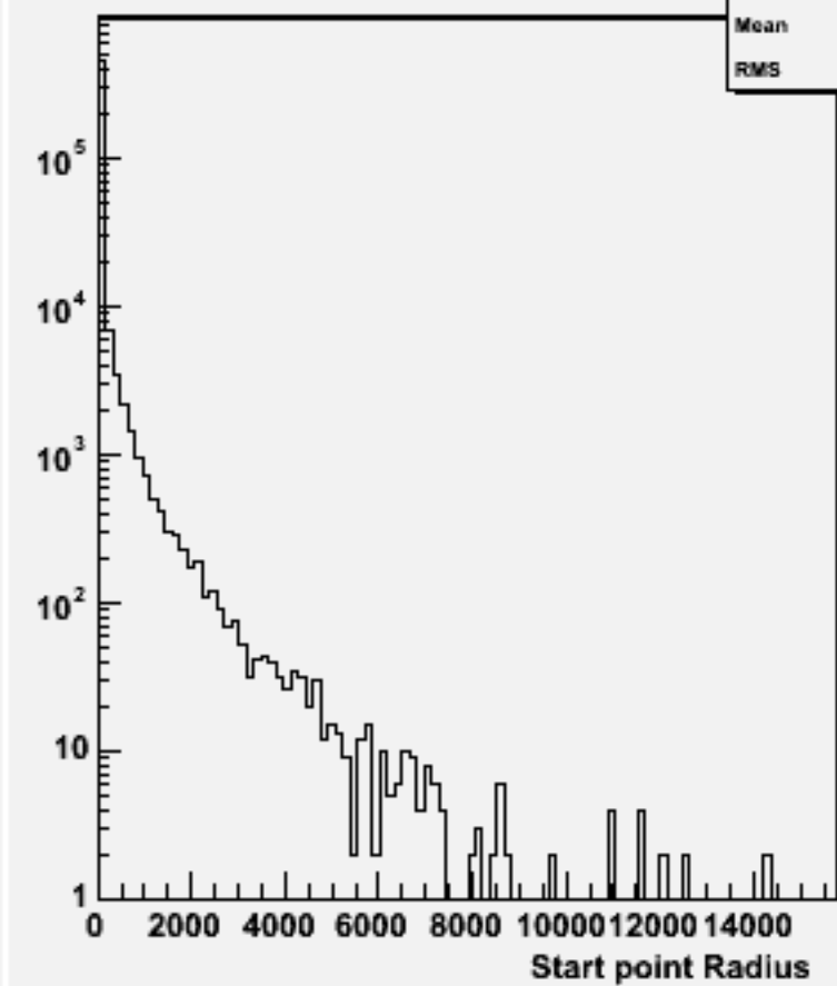
Start point R : w101333 n1n1n2e2sc_o
