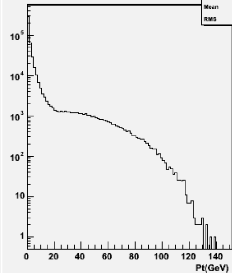
Start point Z : w101333 n1n1n2e2sc_o
