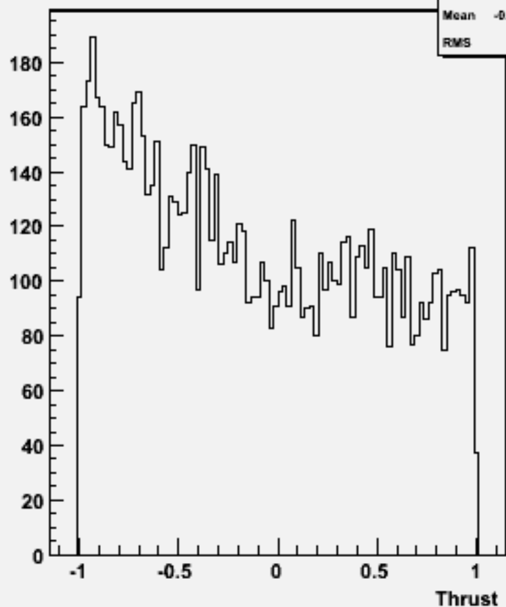
cos \Theta (thrust) w101333 n1n1n2e2sc_o
