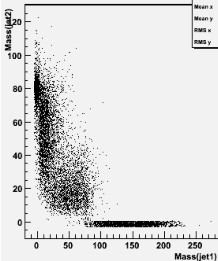
Jet mass for forced 2-jets : w101333 n1n1n2e2sc_o
