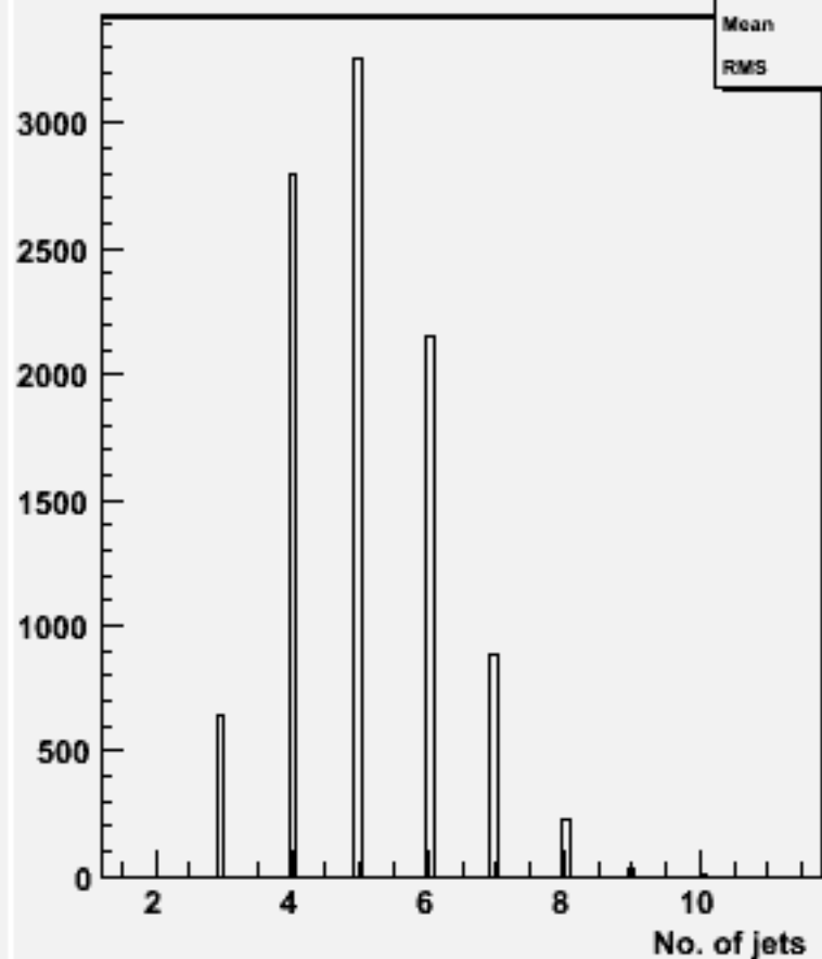
No. jets (ycut=0.001) : w101333 n1n1n2e2sc_o
