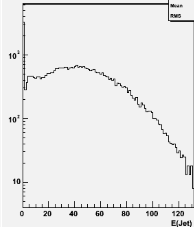
Jet energies(All jets)w101333 n1n1n2e2sc_o
