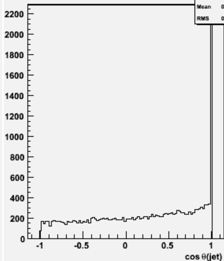
cos \theta for 2-jets :w101333 n1n1n2e2sc_o
