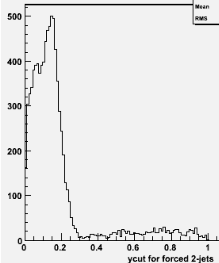
Ycut for 2-jets :w101333 n1n1n2e2sc_o
