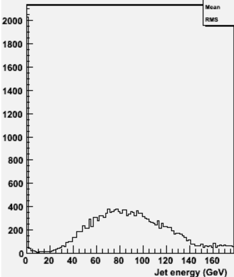
energy for 2-jets :w101333 n1n1n2e2sc_o
