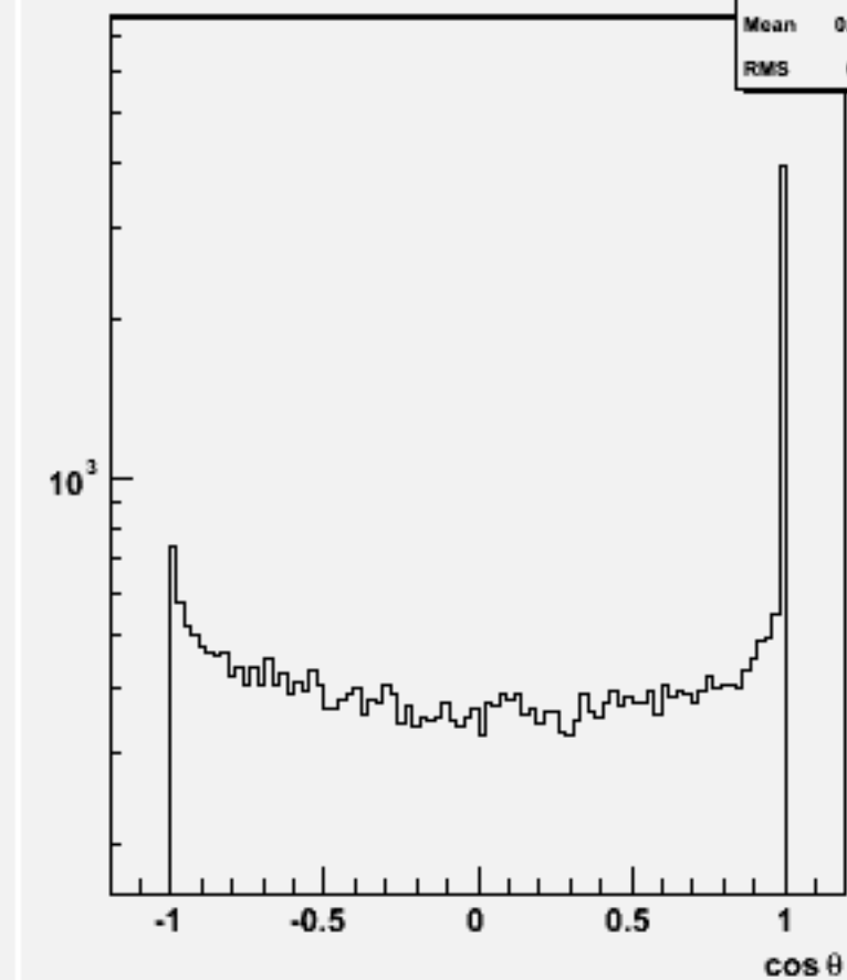
Jet cos \theta (All jets)w101328 n1n1n2e2du_o
