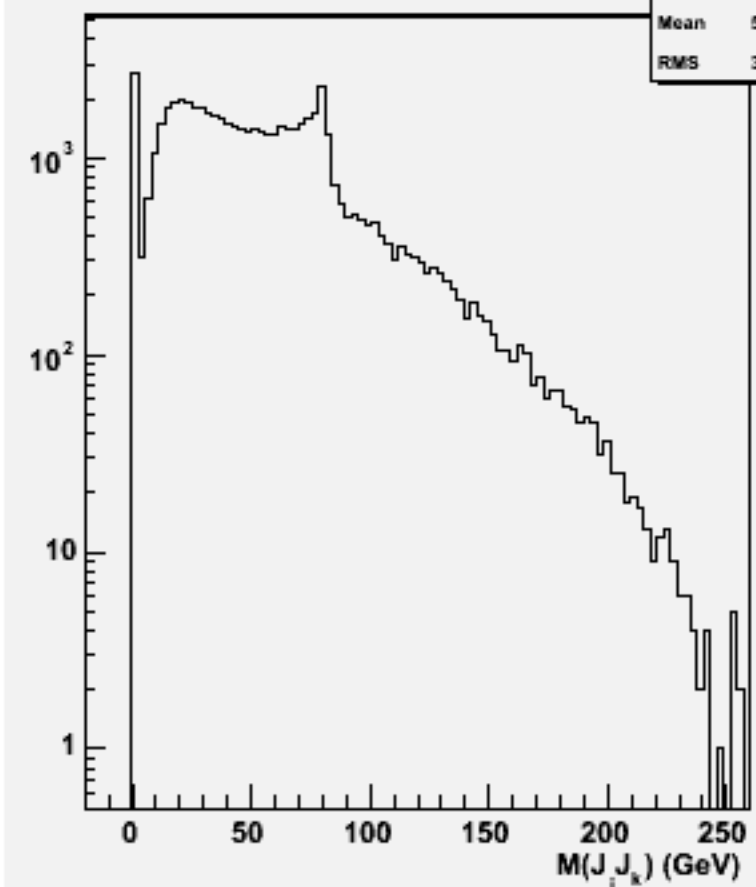
2jets mass(All comb)w101328 n1n1n2e2du_o
