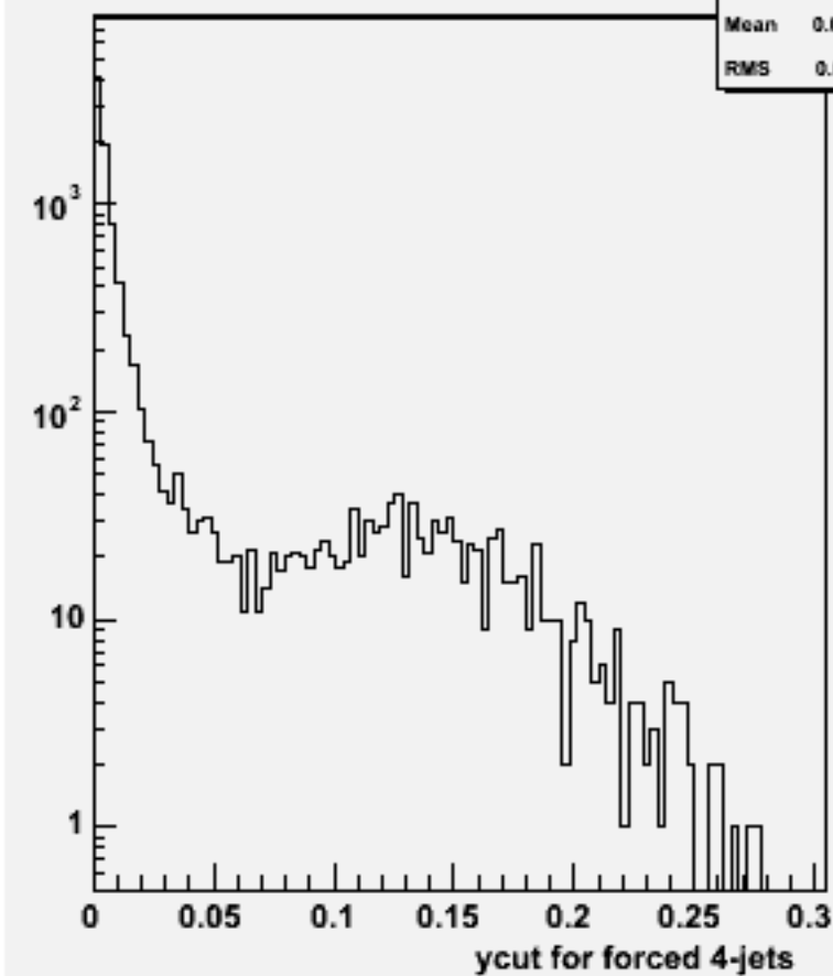
Ycut for 4-jets :w101328 n1n1n2e2du_o
