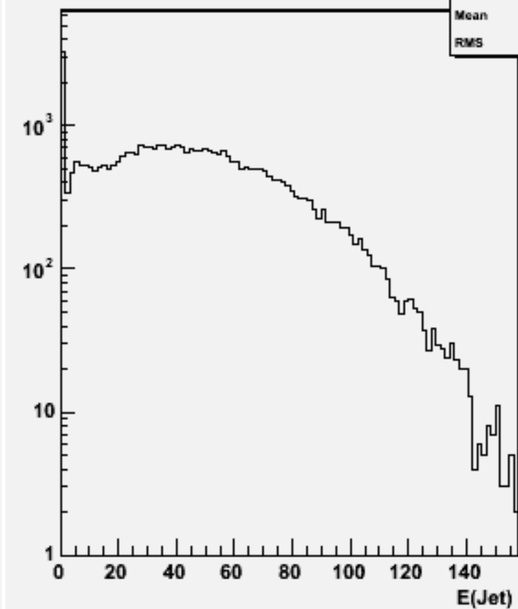
Jet energies(All jets)w101328 n1n1n2e2du_o
