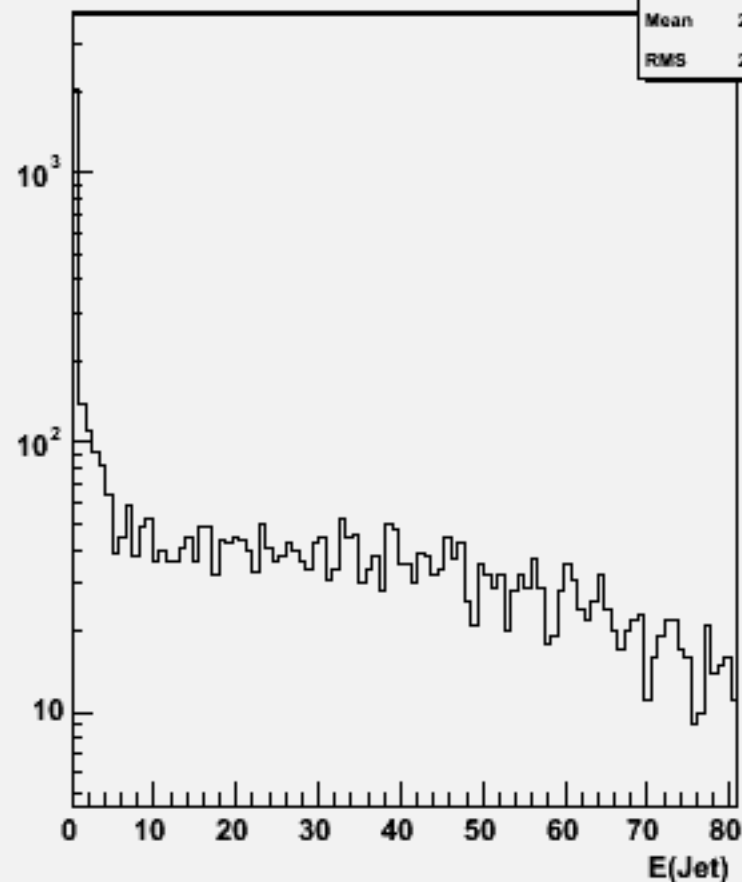
Jet energies(All jets)w101324 n1n1n2e2e3n3_o
