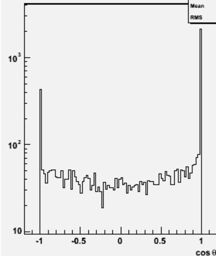
Jet cos \theta (All jets)w101324 n1n1n2e2e3n3_o
