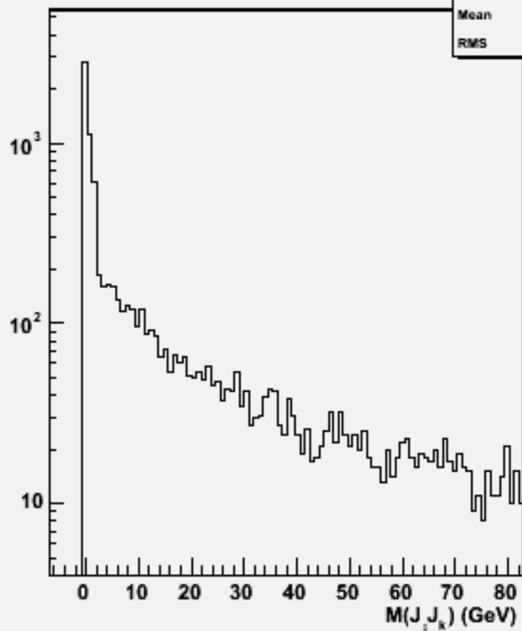
2jets mass(All comb)w101324 n1n1n2e2e3n3_o
