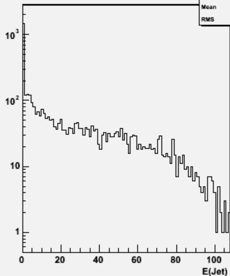
Jet energies(All jets)w101321 n1n1n2e2e2n2_o
