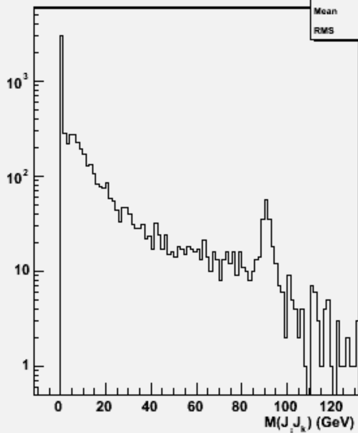
2jets mass(All comb)w101321 n1n1n2e2e2n2_o
