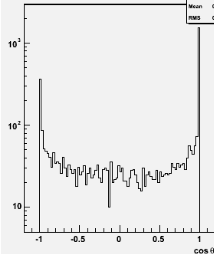
Jet cos \theta (All jets)w101321 n1n1n2e2e2n2_o
