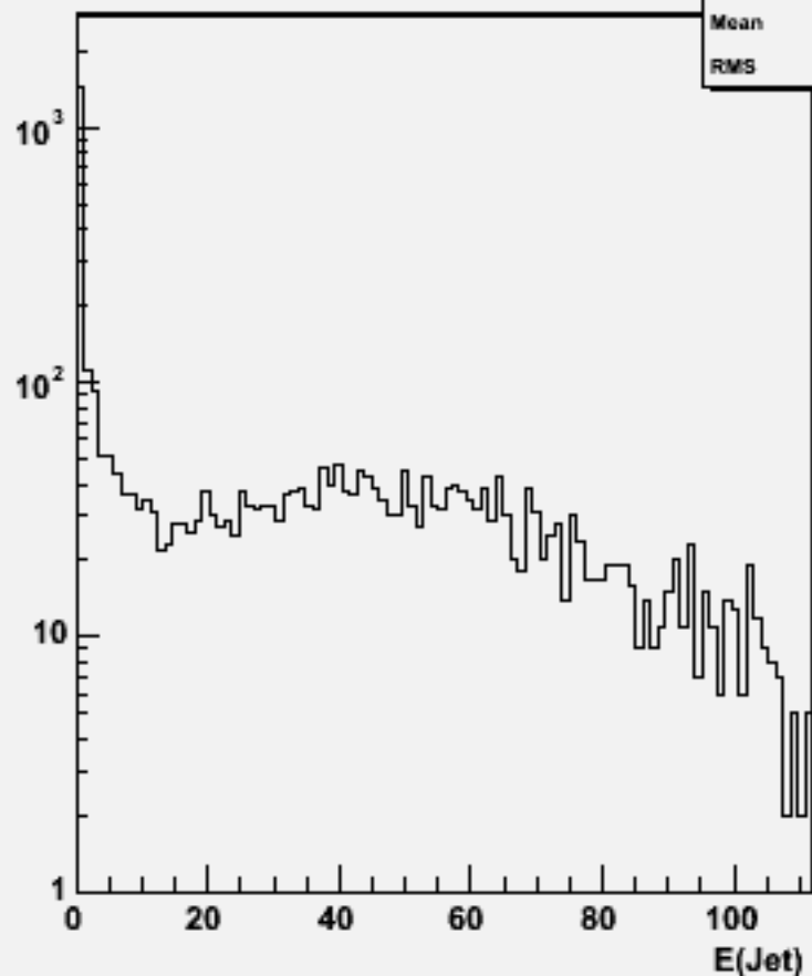
Jet energies(All jets)w101320 n1n1n2e2e2n2_o
