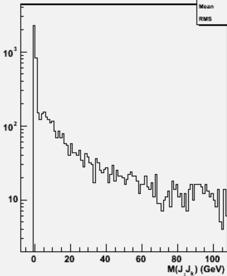
2jets mass(All comb)w101320 n1n1n2e2e2n2_o
