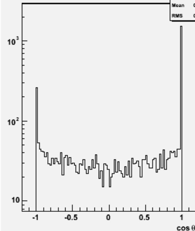
Jet cos \theta (All jets)w101320 n1n1n2e2e2n2_o
