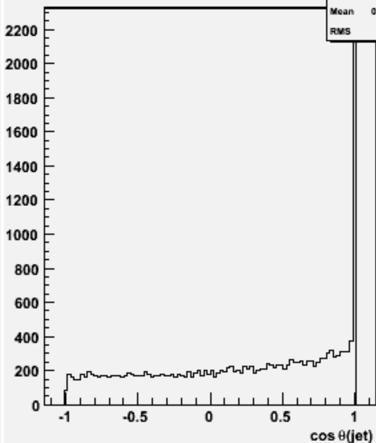
cos \theta for 2-jets :w101313 n1n1n1e1sc_o
