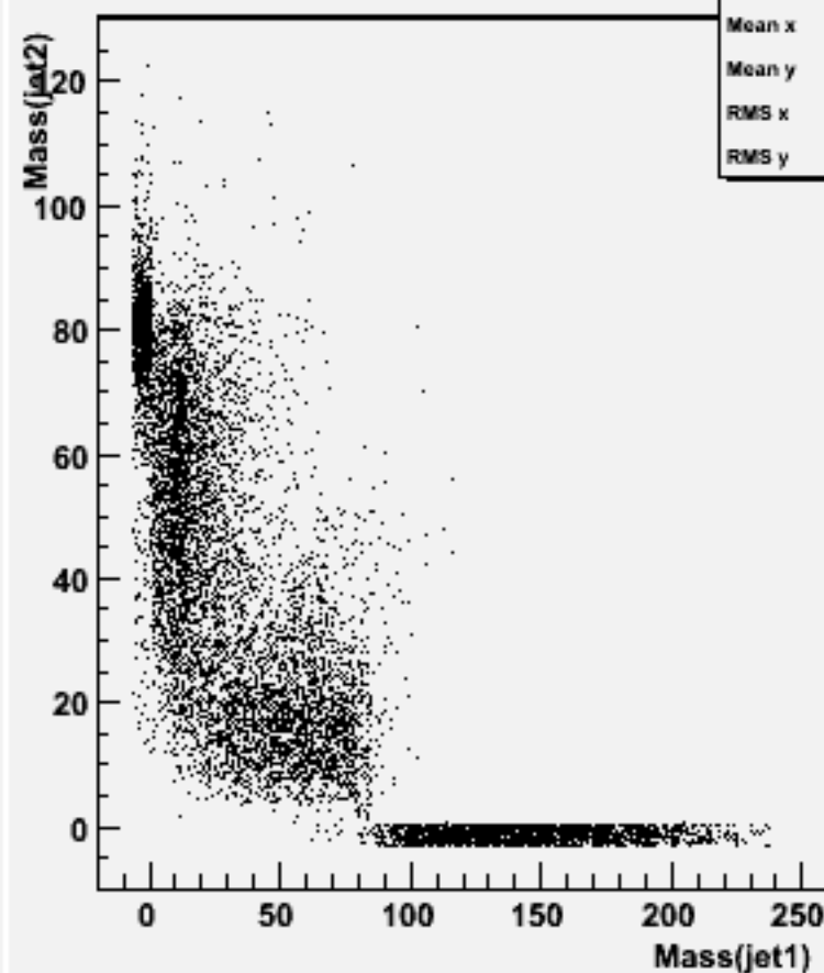
Jet mass for forced 2-jets : w101313 n1n1n1e1sc_o
