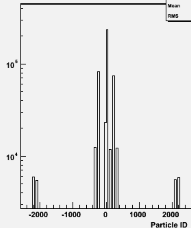
Particle ID : w101313 n1n1n1e1sc_o
