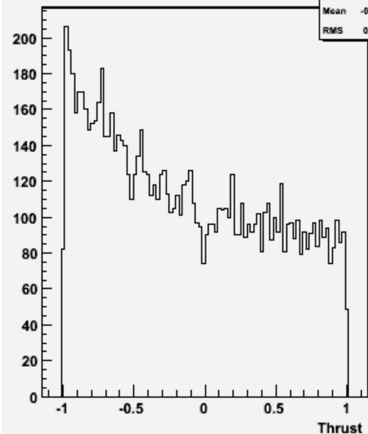
cos \Theta (thrust) w101313 n1n1n1e1sc_o
