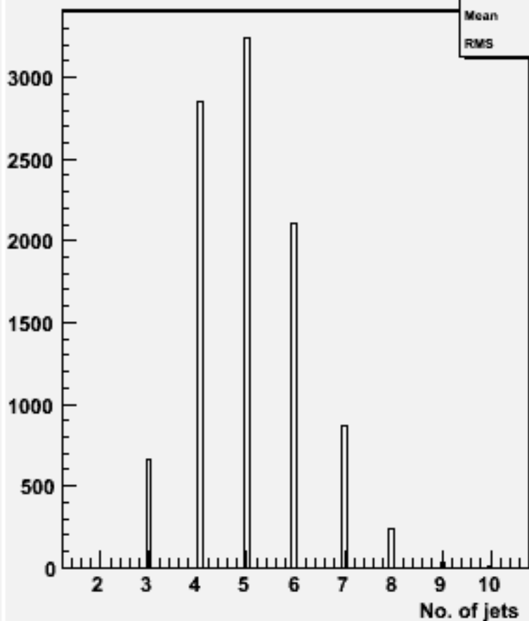
No. jets (ycut=0.001) : w101313 n1n1n1e1sc_o
