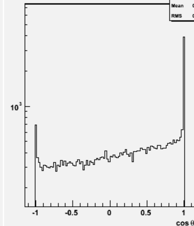
Jet cos \theta (All jets)w101313 n1n1n1e1sc_o
