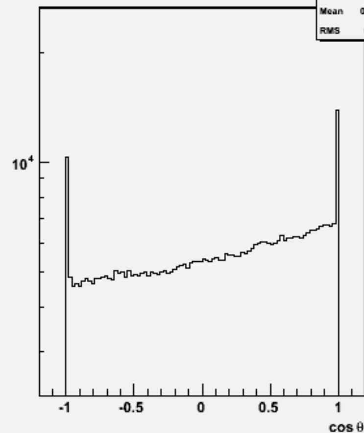
Particle cos \theta : w101313 n1n1n1e1sc_o
