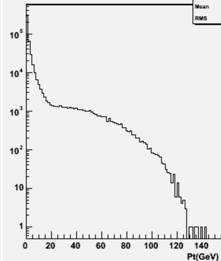
Particle Pt : w101313 n1n1n1e1sc_o
