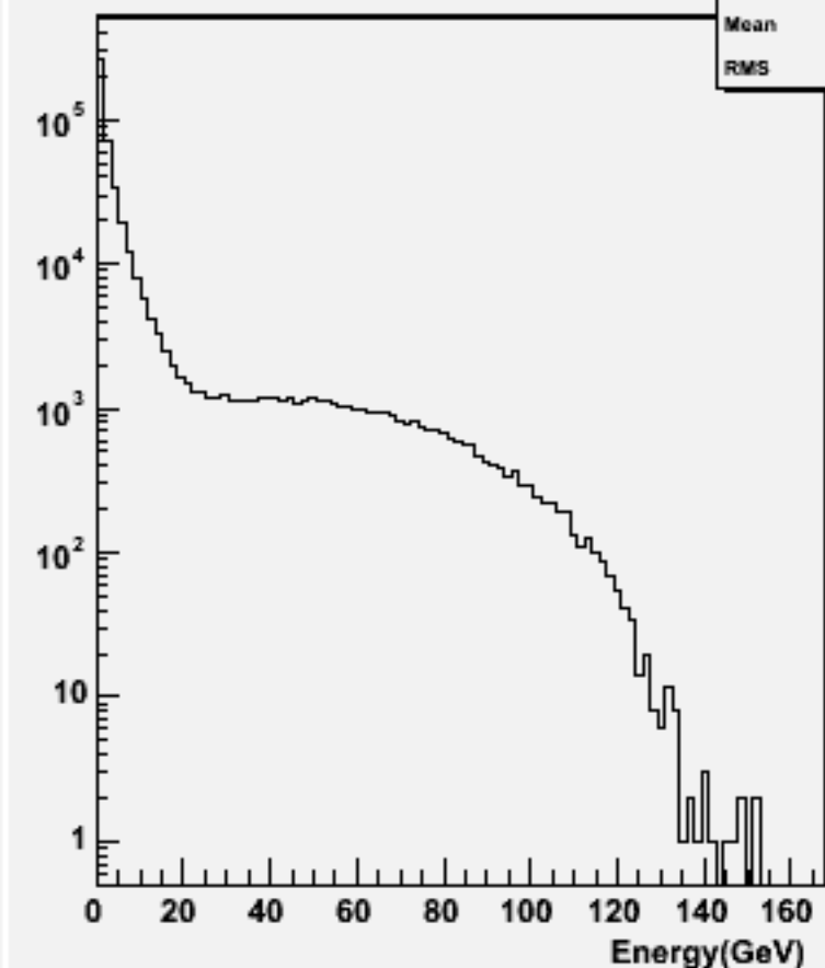
Particle Energy : w101313 n1n1n1e1sc_o
