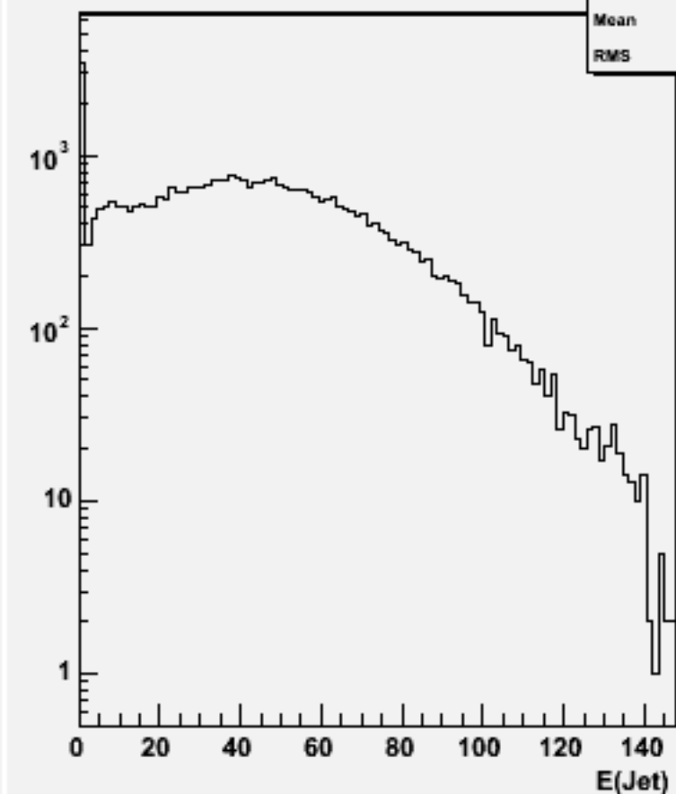
Jet energies(All jets)w101313 n1n1n1e1sc_o
