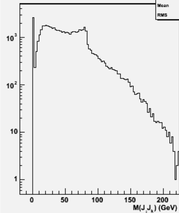
2jets mass(All comb)w101313 n1n1n1e1sc_o
