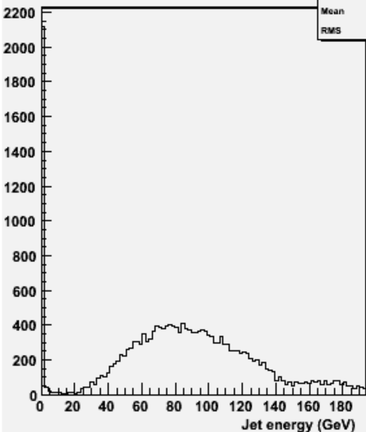
energy for 2-jets :w101313 n1n1n1e1sc_o
