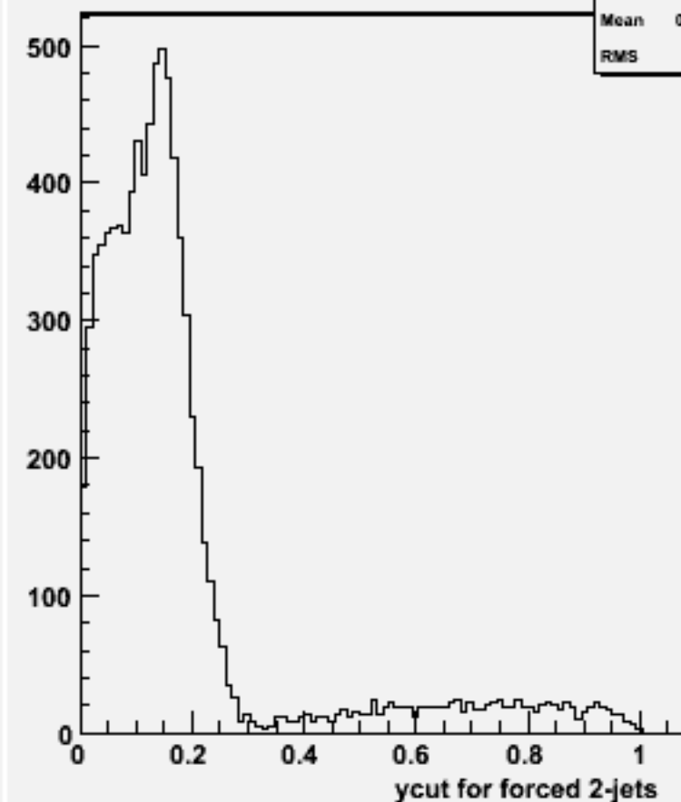
Ycut for 2-jets :w101313 n1n1n1e1sc_o
