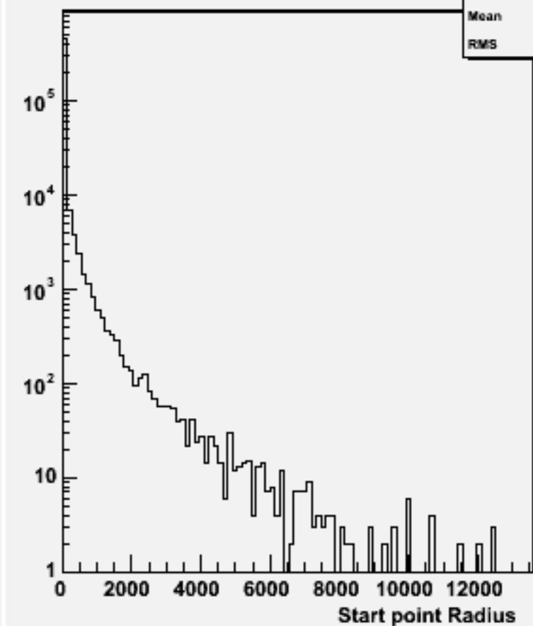
Start point R : w101313 n1n1n1e1sc_o
