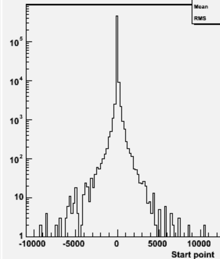
Start point Z : w101313 n1n1n1e1sc_o
