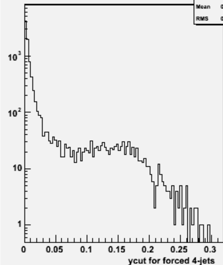
Ycut for 4-jets :w101313 n1n1n1e1sc_o
