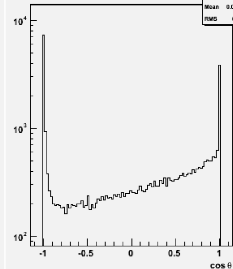
Jet cos \theta (All jets)w101311 n1n1n1e1sc_o
