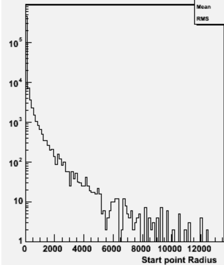
Start point R : w101311 n1n1n1e1sc_o
