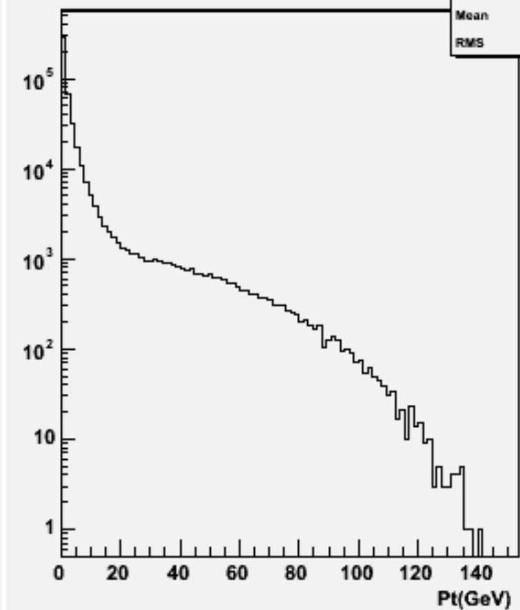
Particle Pt : w101311 n1n1n1e1sc_o
