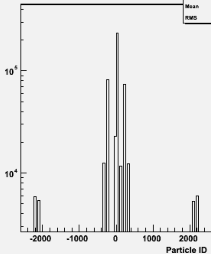
Particle ID : w101311 n1n1n1e1sc_o
