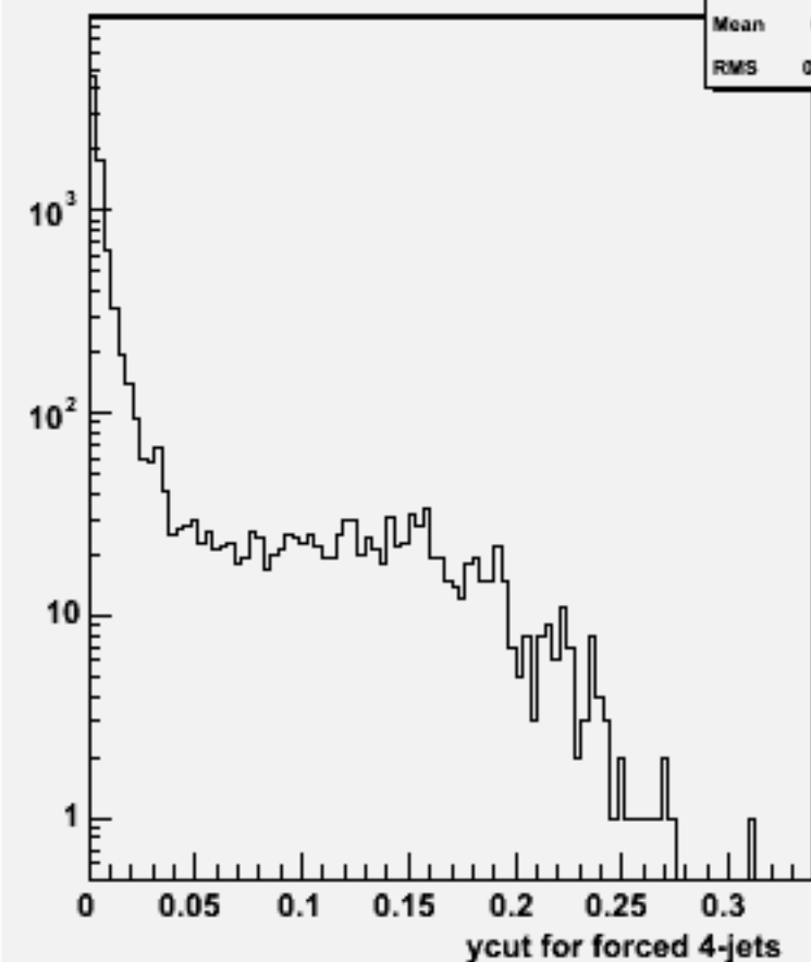
Ycut for 4-jets :w101311 n1n1n1e1sc_o
