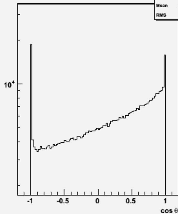
Particle cosθ : w101311 n1n1n1e1sc_o
