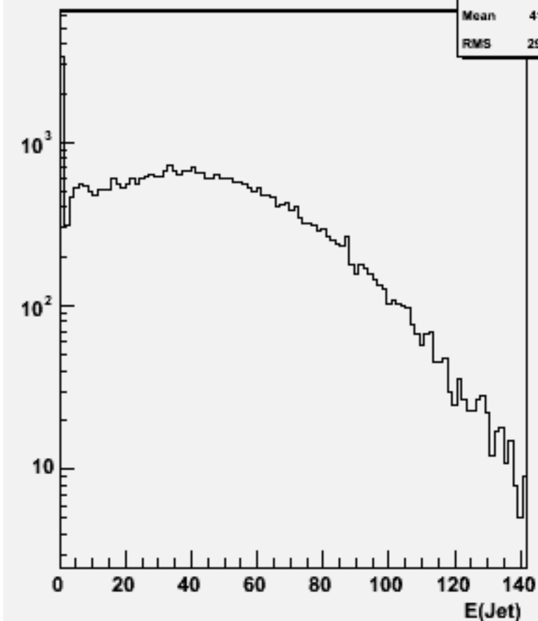
Jet energies(All jets)w101311 n1n1n1e1sc_o
