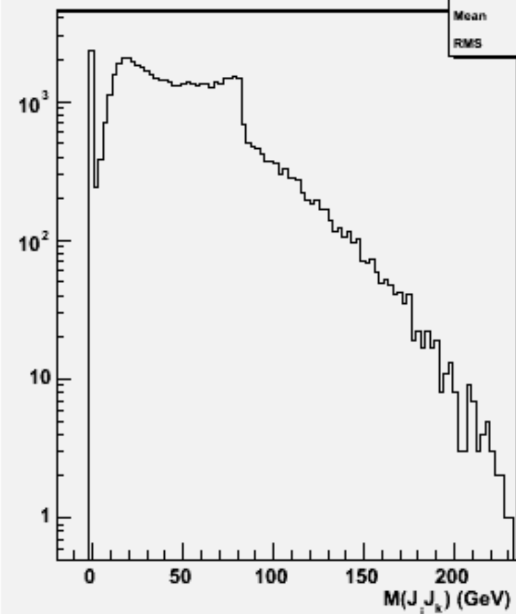
2jets mass(All comb)w101311 n1n1n1e1sc_o
