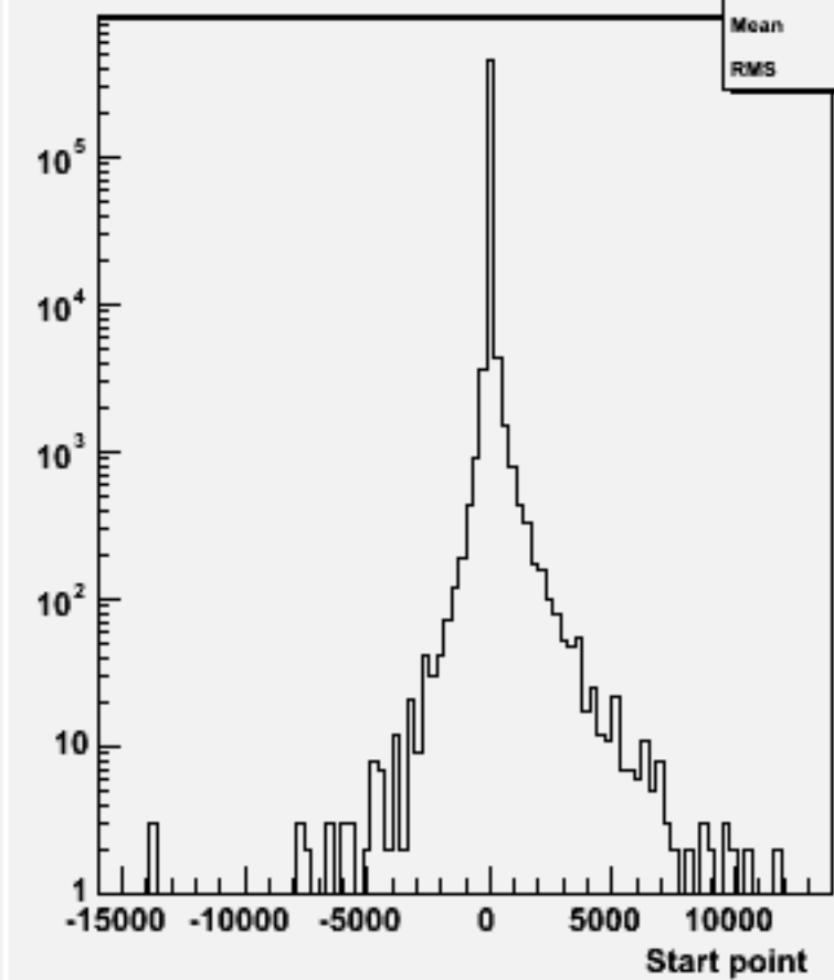
Start point Z : w101311 n1n1n1e1sc_o
