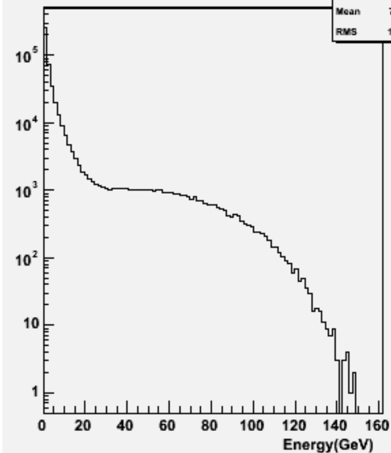
Particle Energy : w101311 n1n1n1e1sc_o
